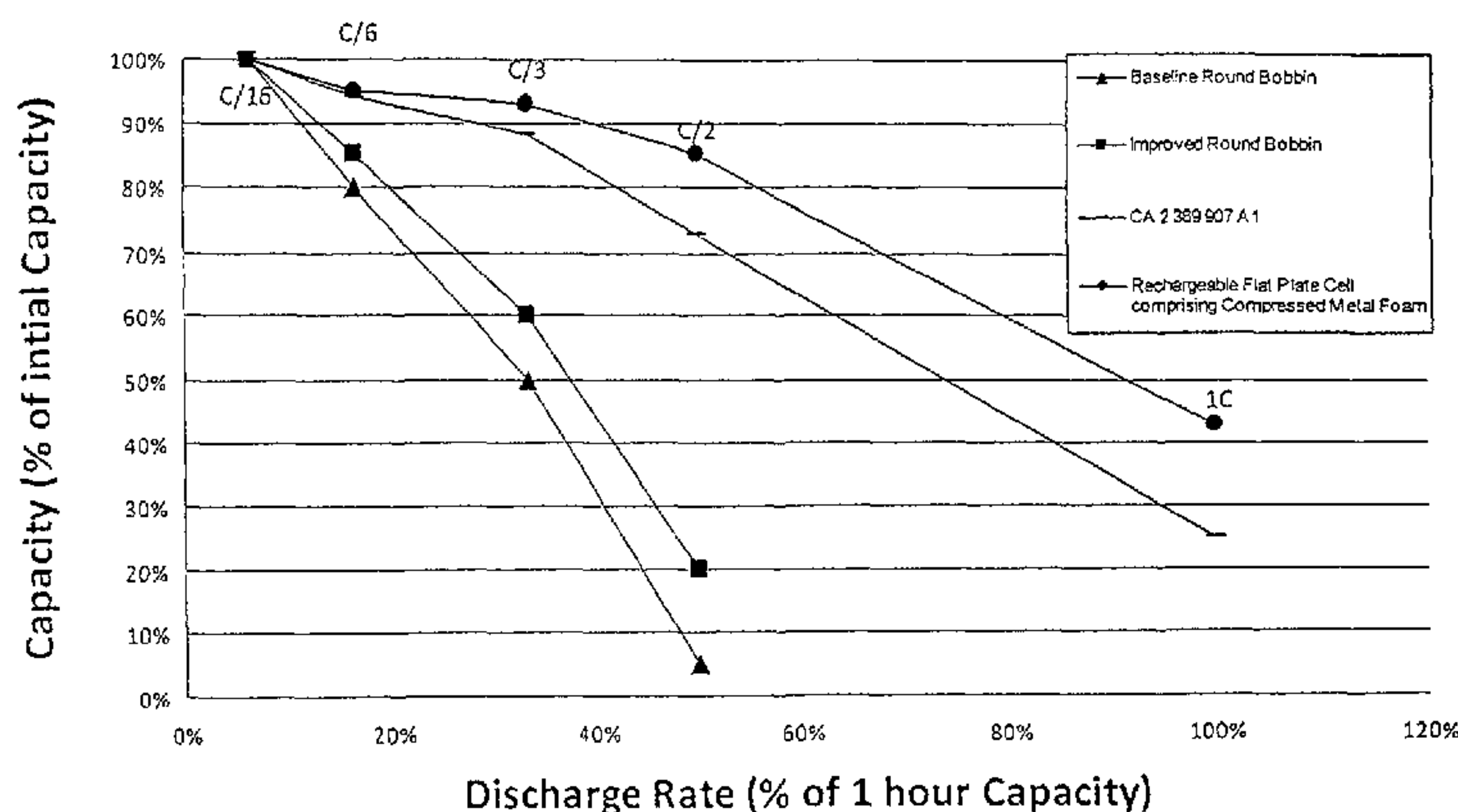
ZnMn(O 2 ) Cell Capacity Versus Discharge Rate
