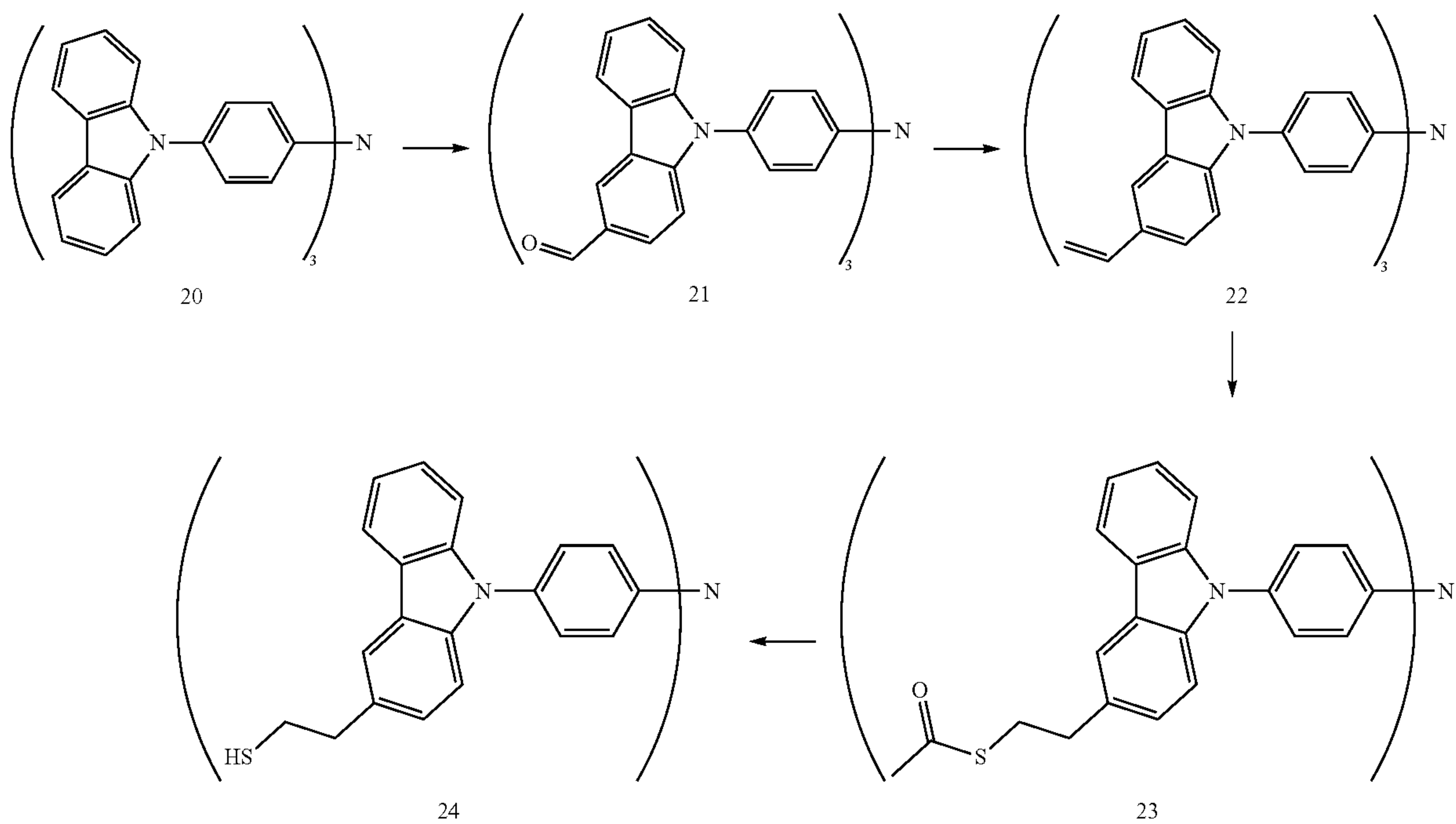
Scheme 1: Synthesis of 22 and 24 derivatives
