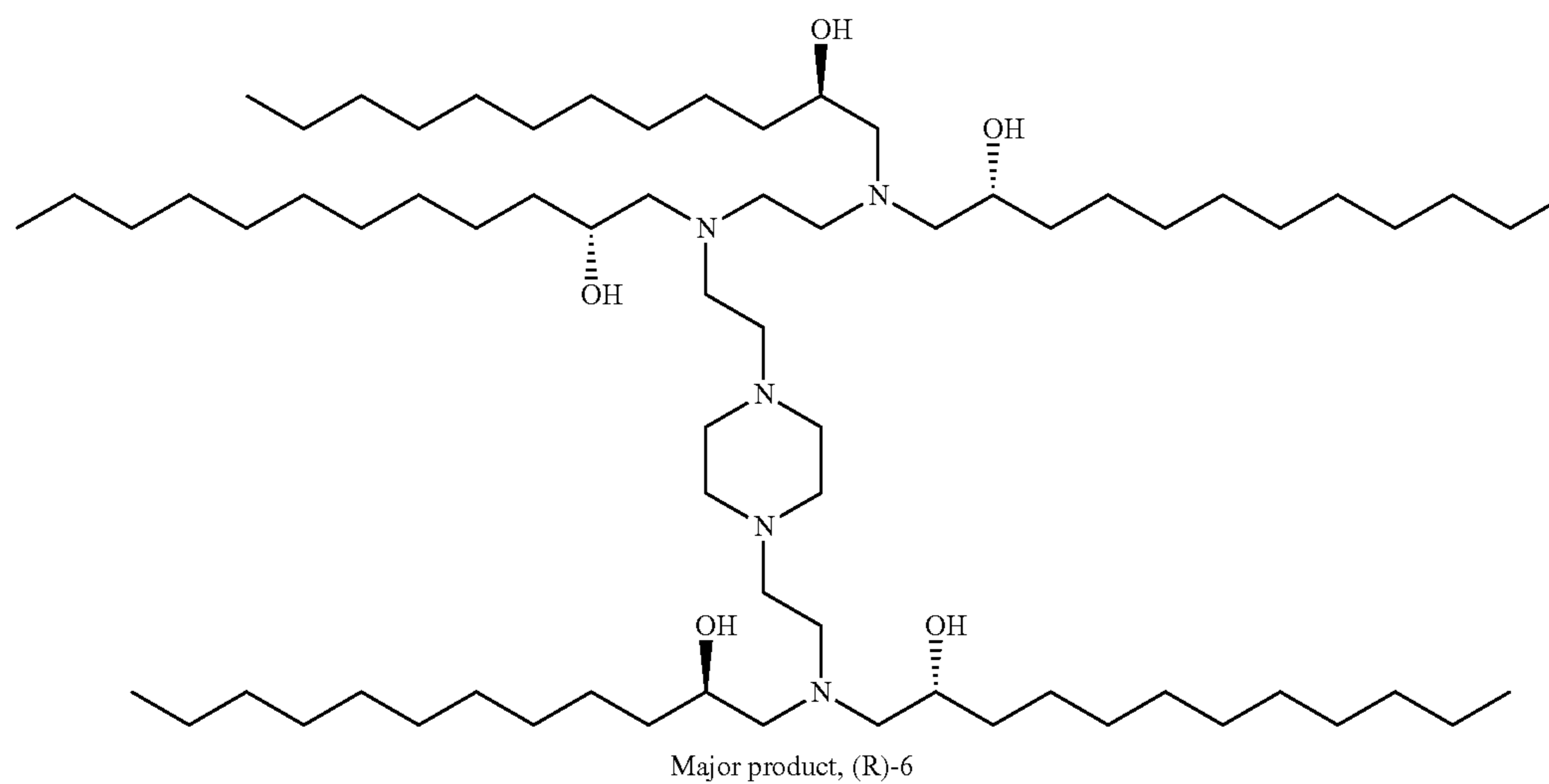
Scheme 7
