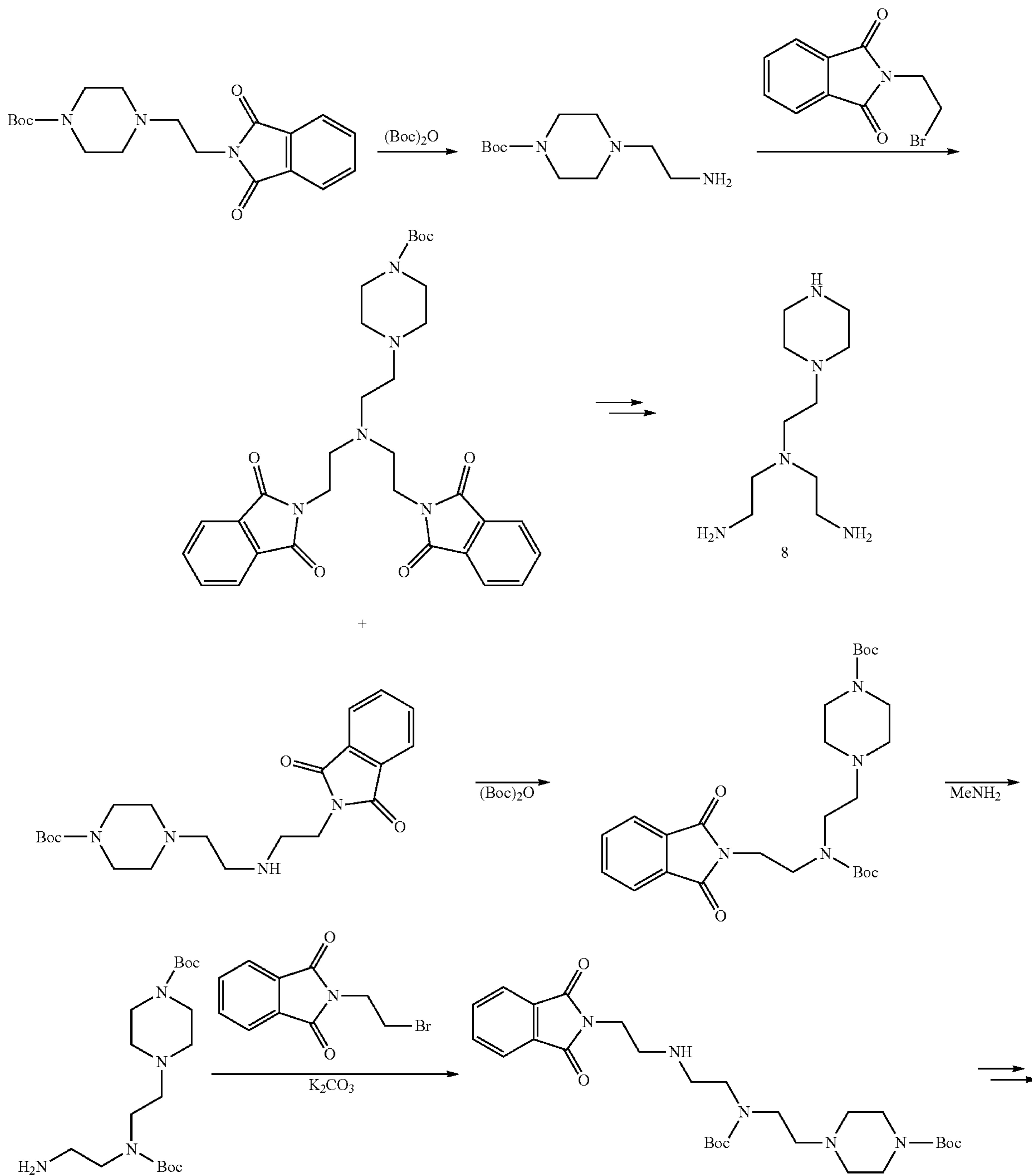
Scheme 2
