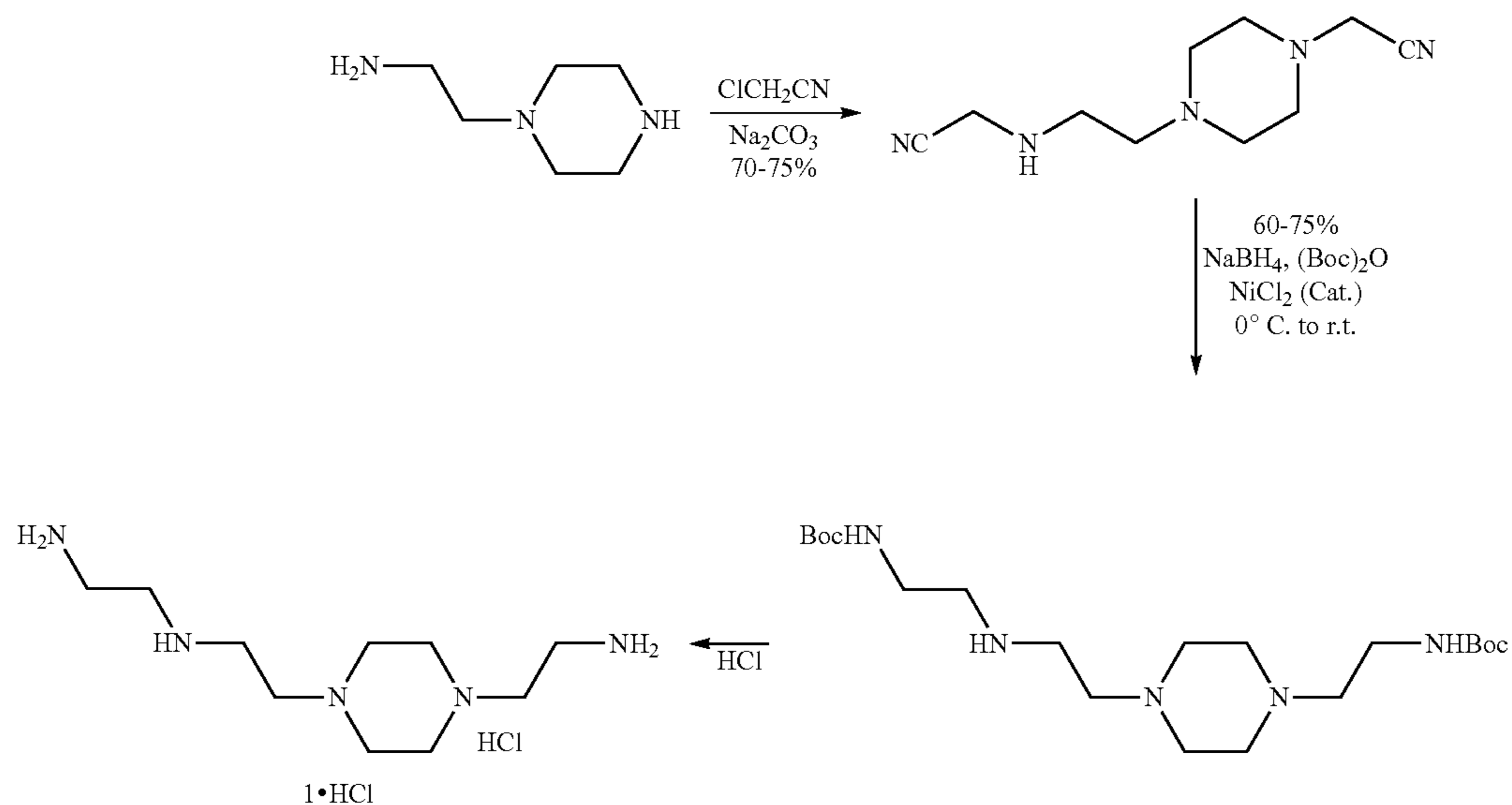
Scheme 5
