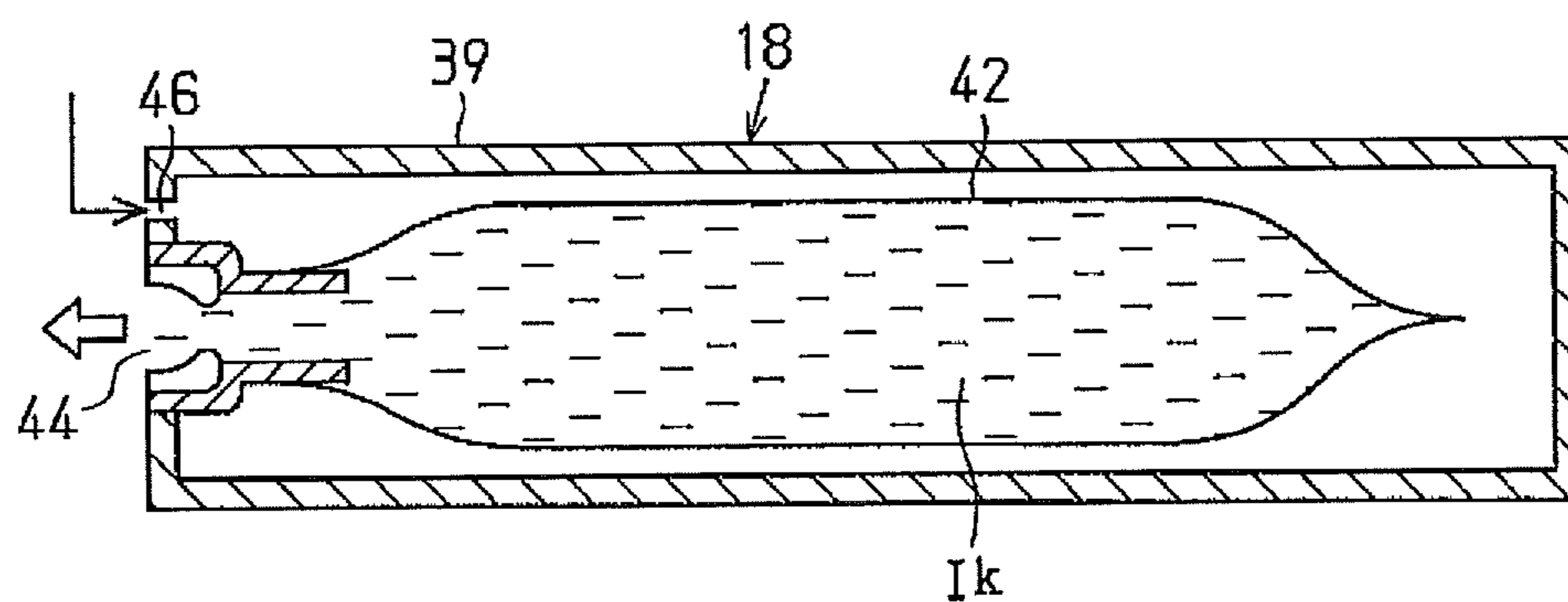
Fig. 25 (Prior Art)
