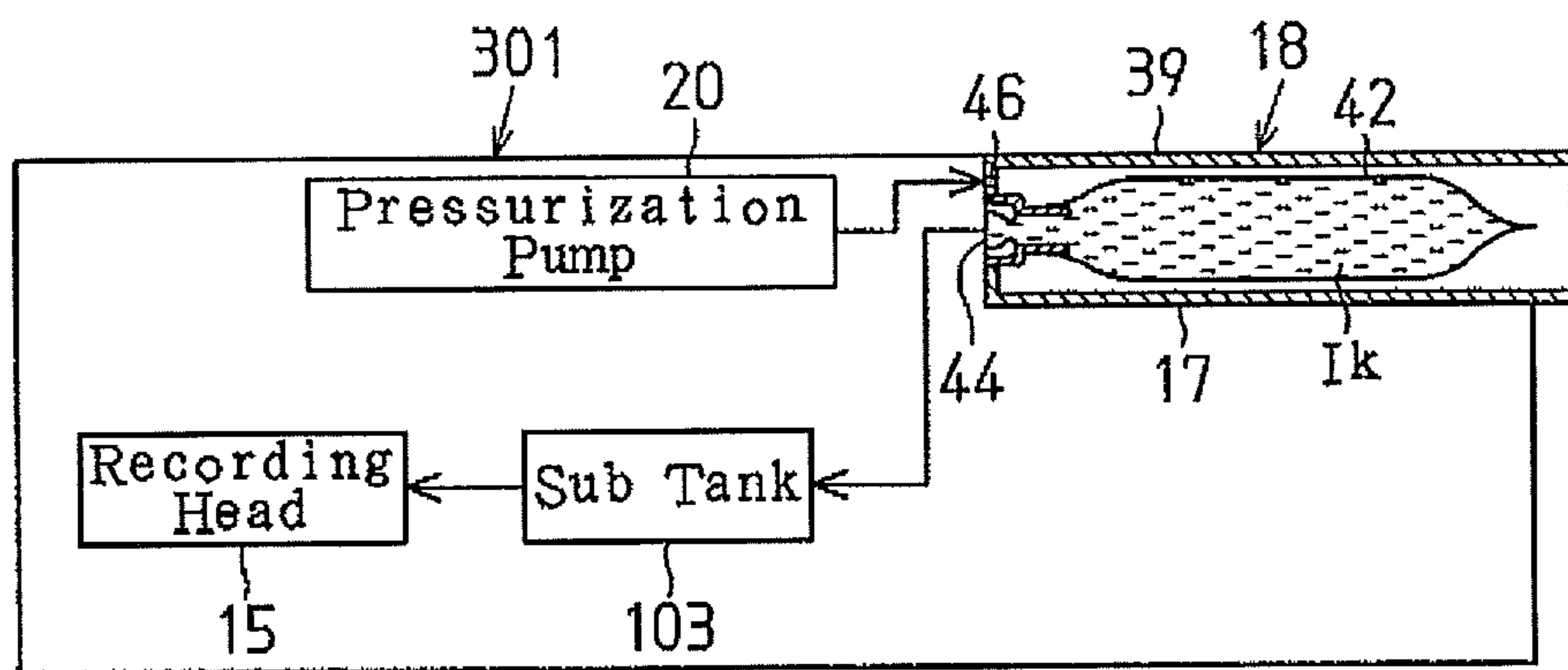
Fig. 24 (Prior Art)
