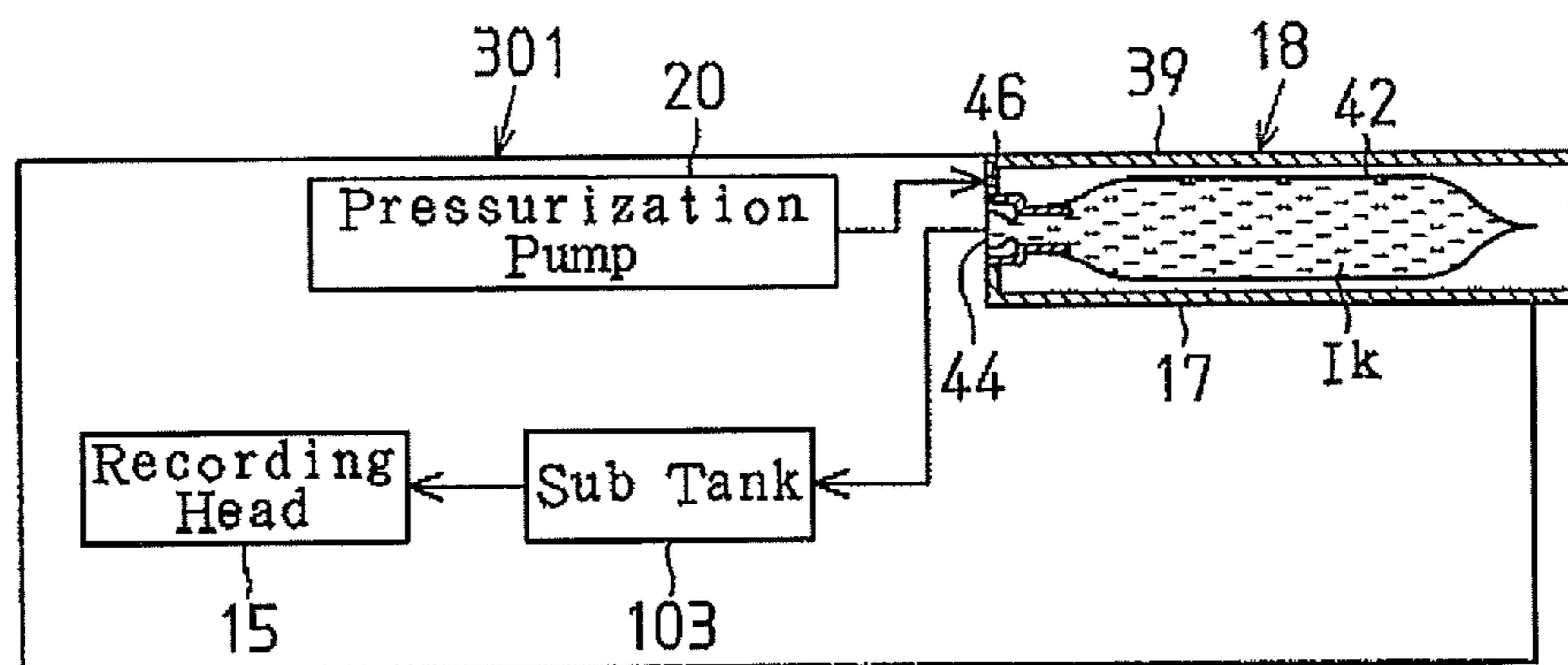
Fig. 24 (Prior Art)
