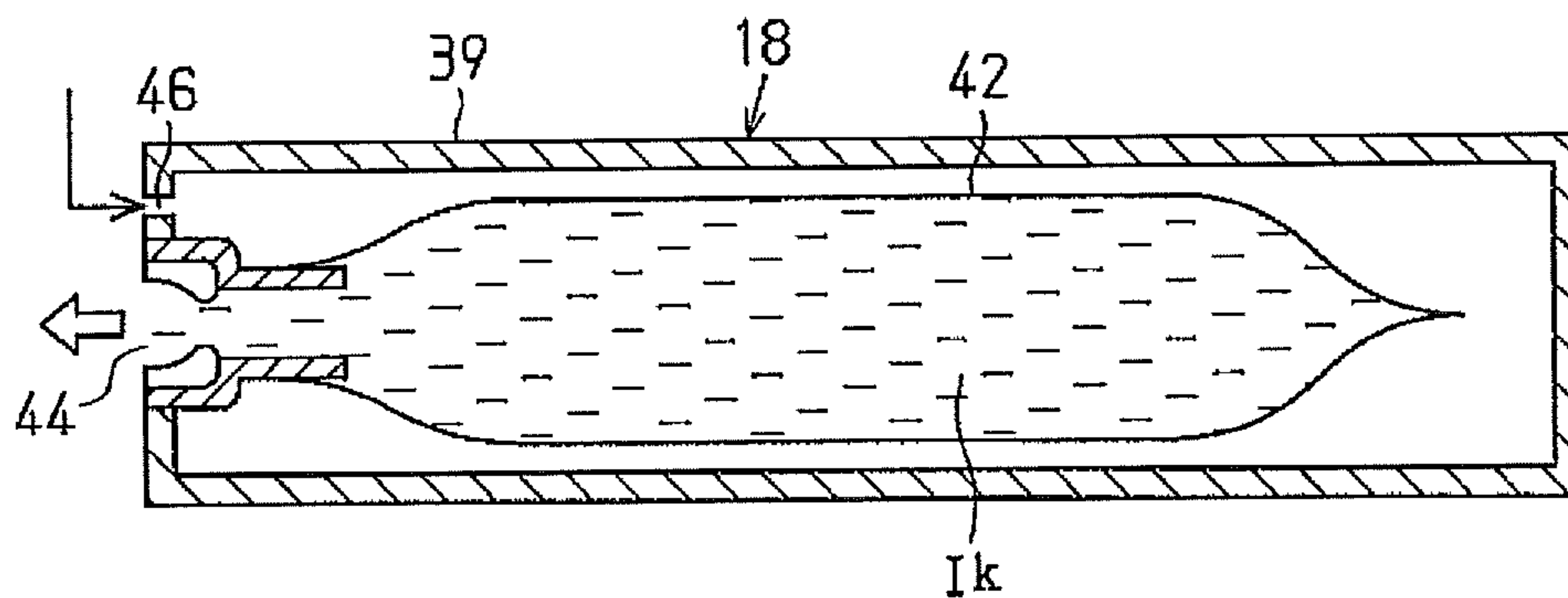
Fig. 25 (Prior Art)
