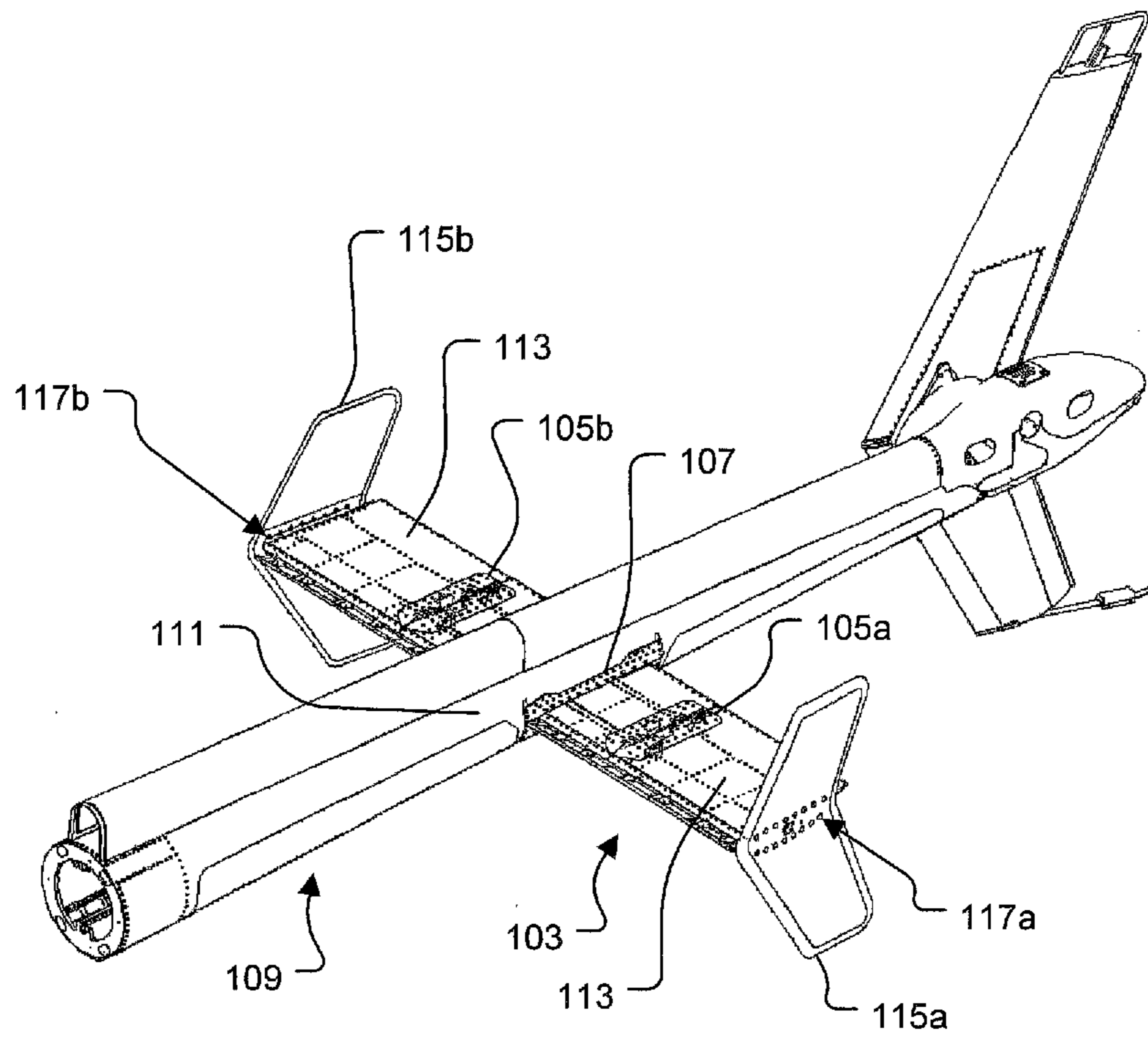
FIG. 2 (PRIOR ART)
