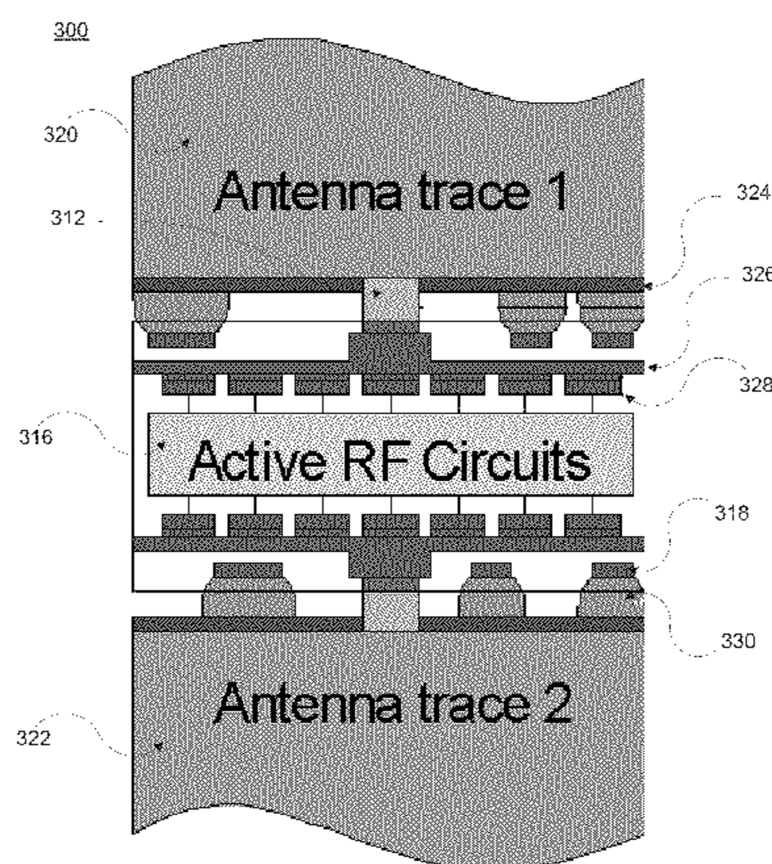
CONCEPTUAL DIAGRAM OF AN ASSEMBLED RFID TAG
