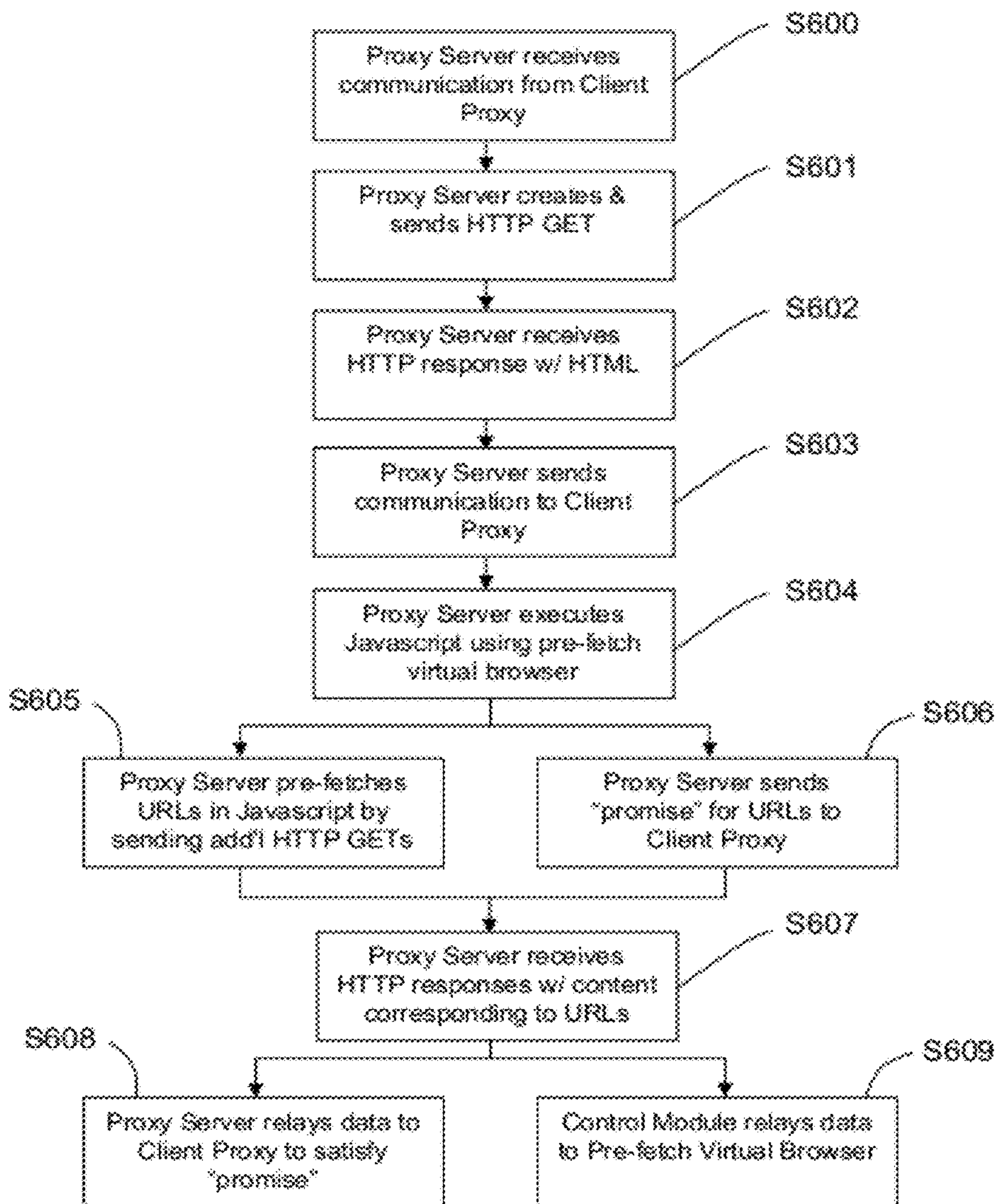
Fig. 6 Proxy Server Pre-Fetching
