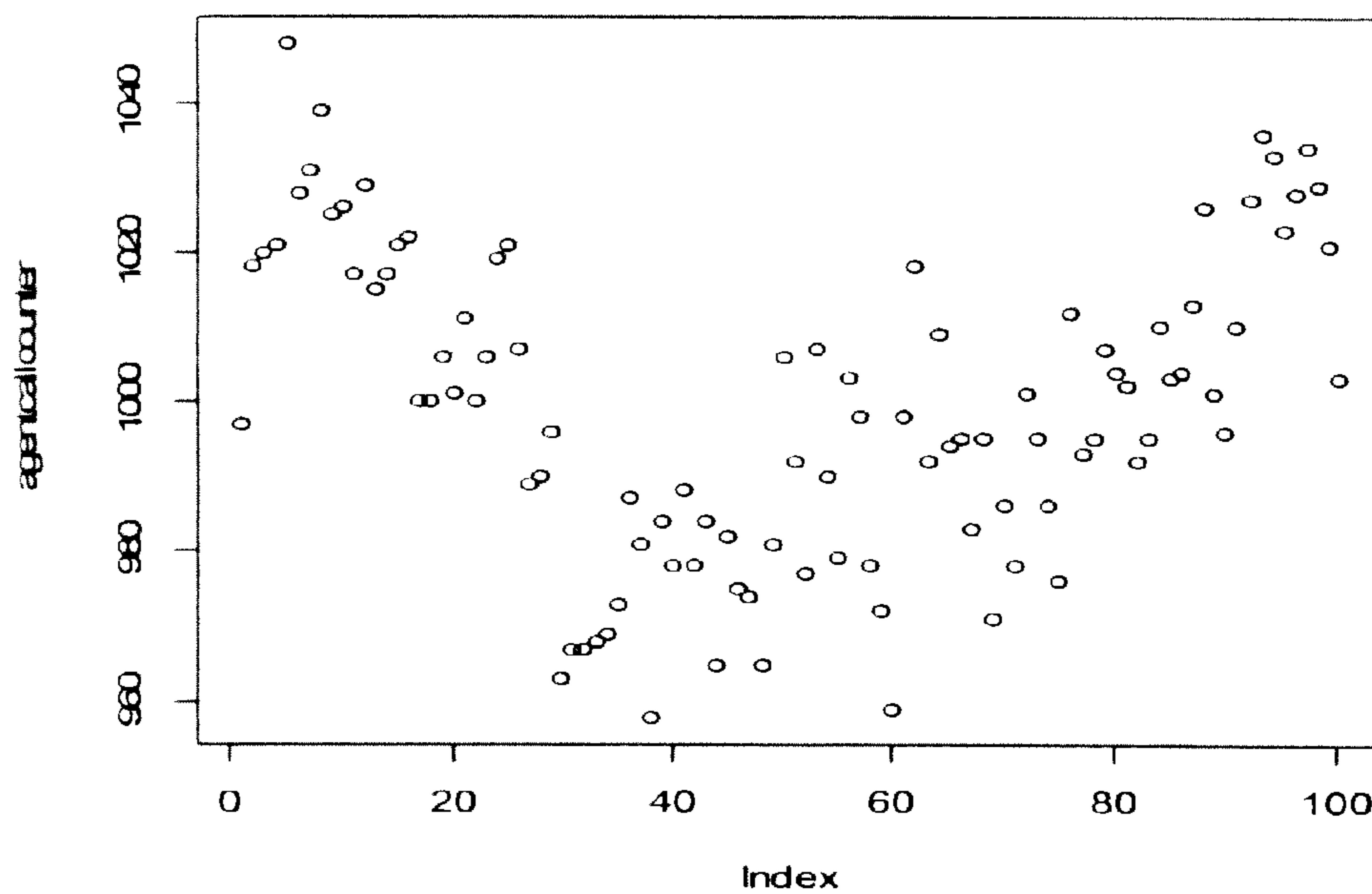
Agent Utilization
