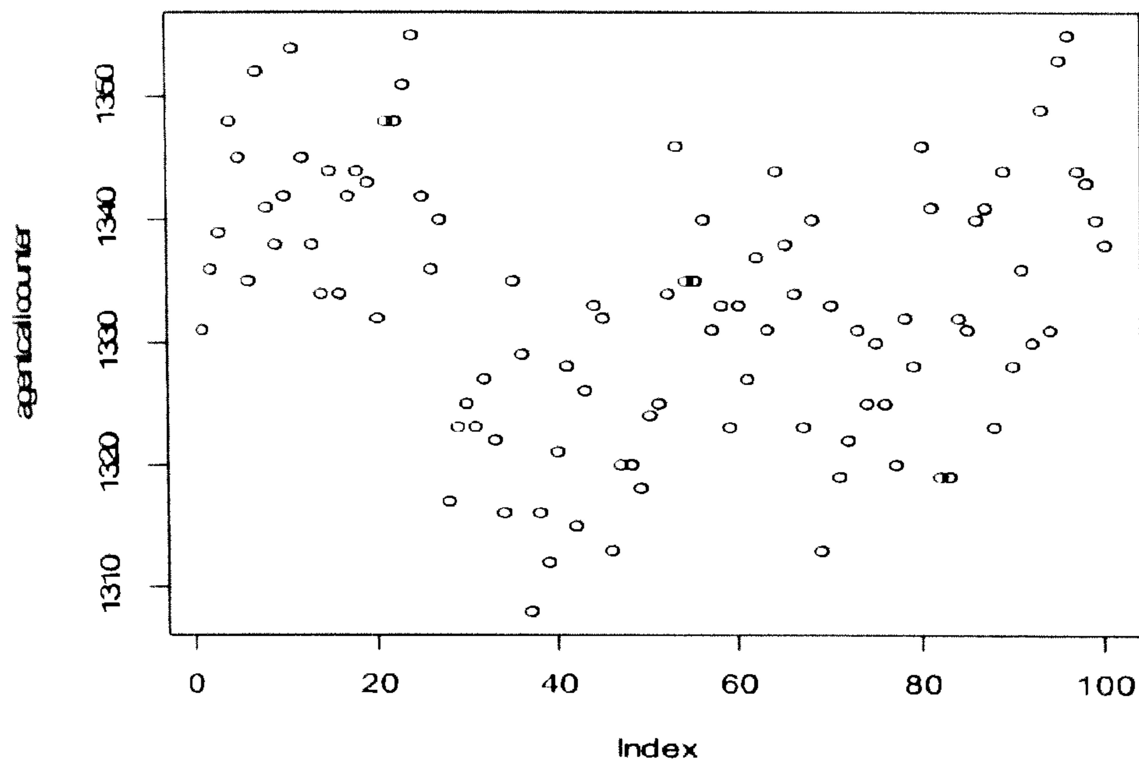
Agent Utilization
