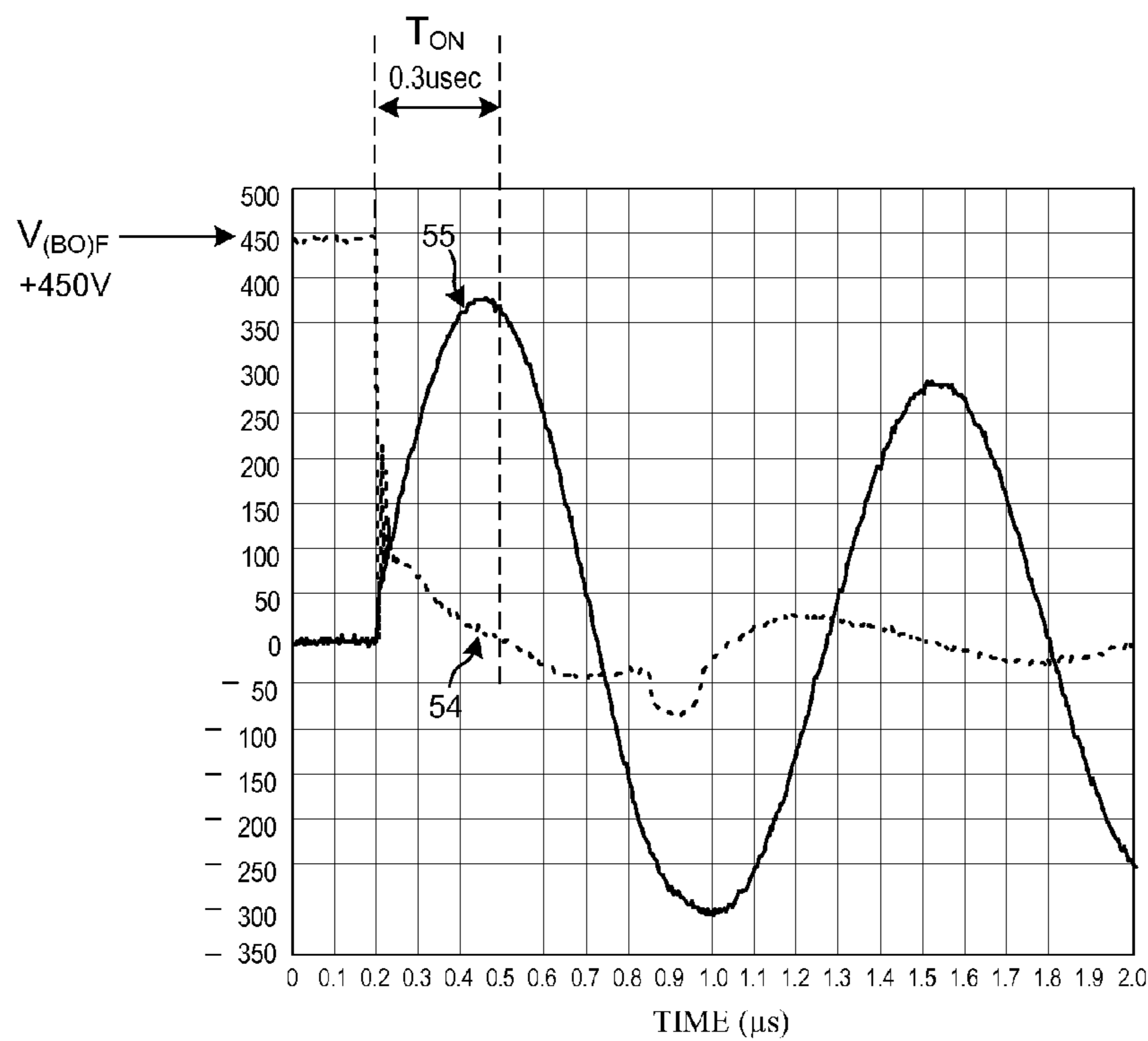
SWITCHING DIAGRAM OF THE BOD
