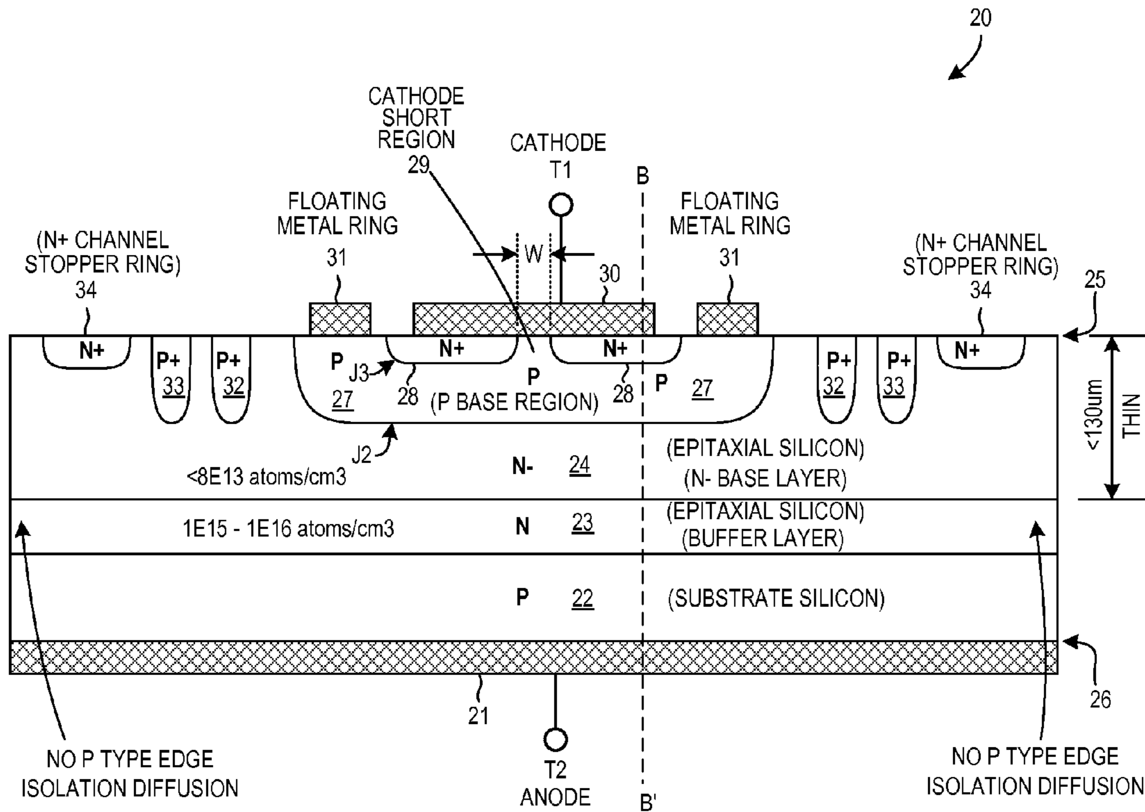
BREAKOVER DIODE DEVICE
