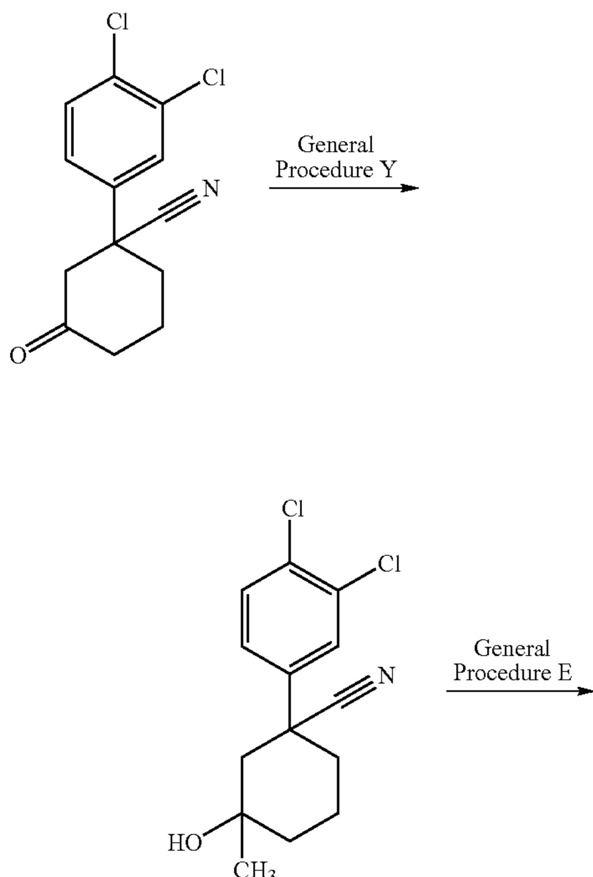
Scheme 31: Synthesis of 3-Disubstituted Cyclohexylamines
