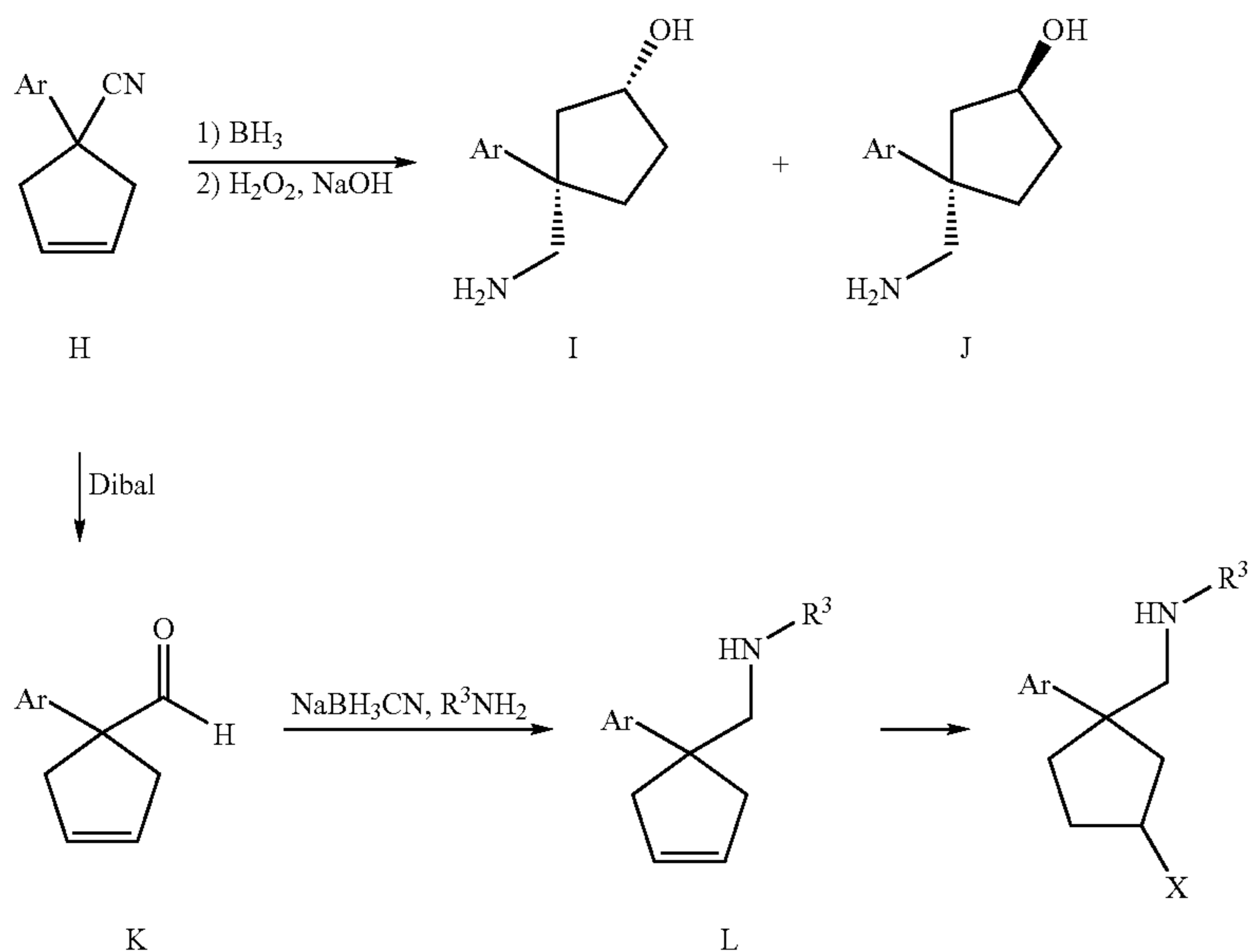
Scheme 4: Synthesis of Substituted Cyclopentyl Amines
