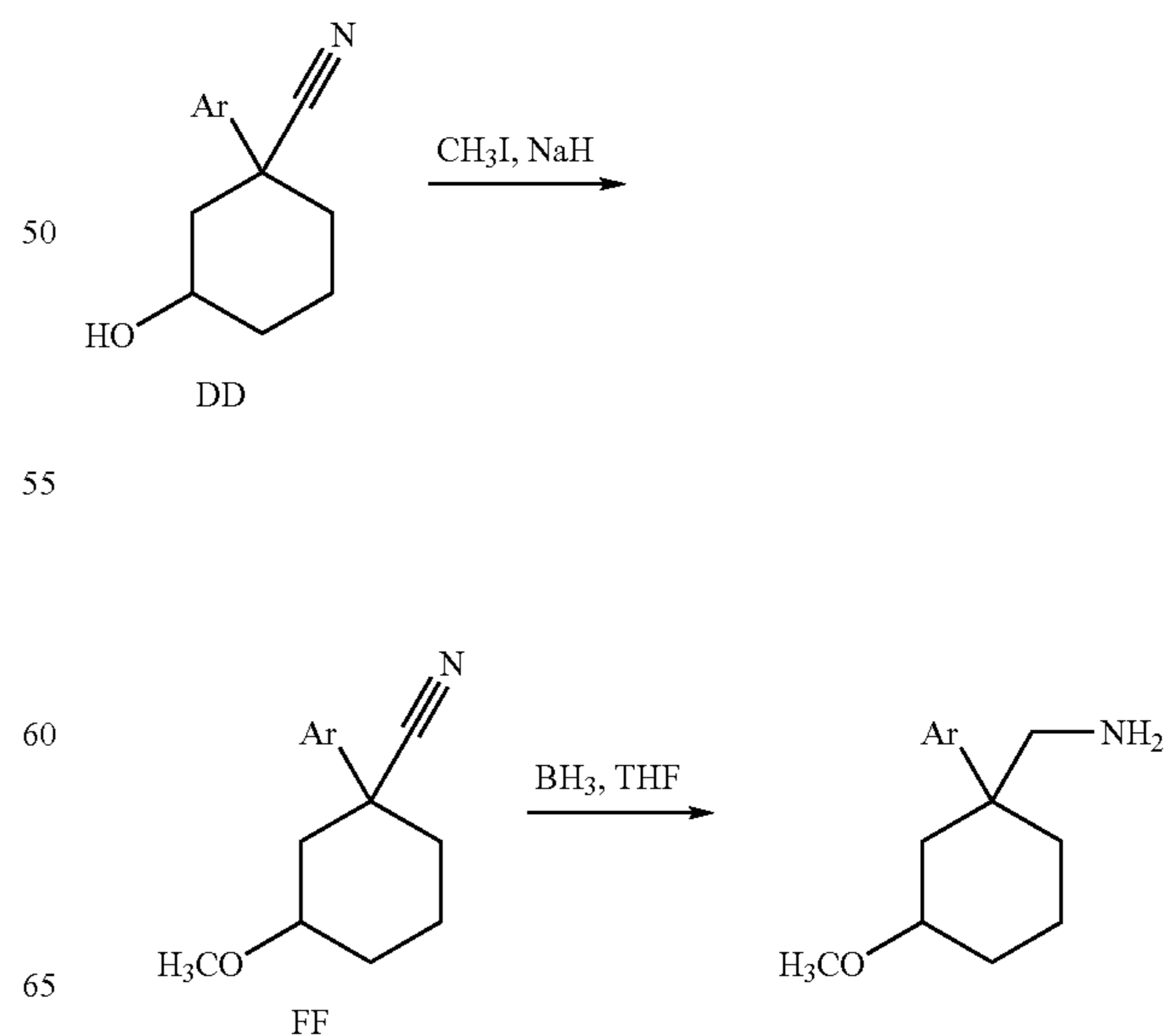
Scheme 13: Exemplary Synthesis of 3-Alkoxy-Cyclohexylamines
