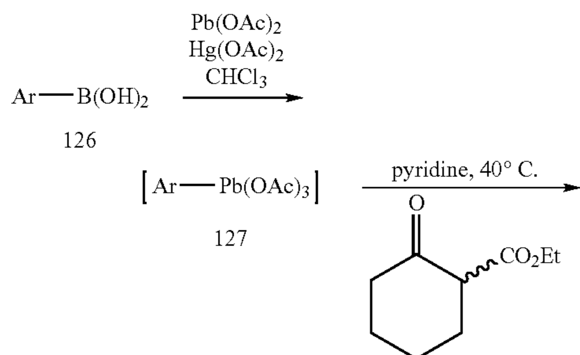
Scheme 27: Preparation of Arylhydroxyacids (130)
