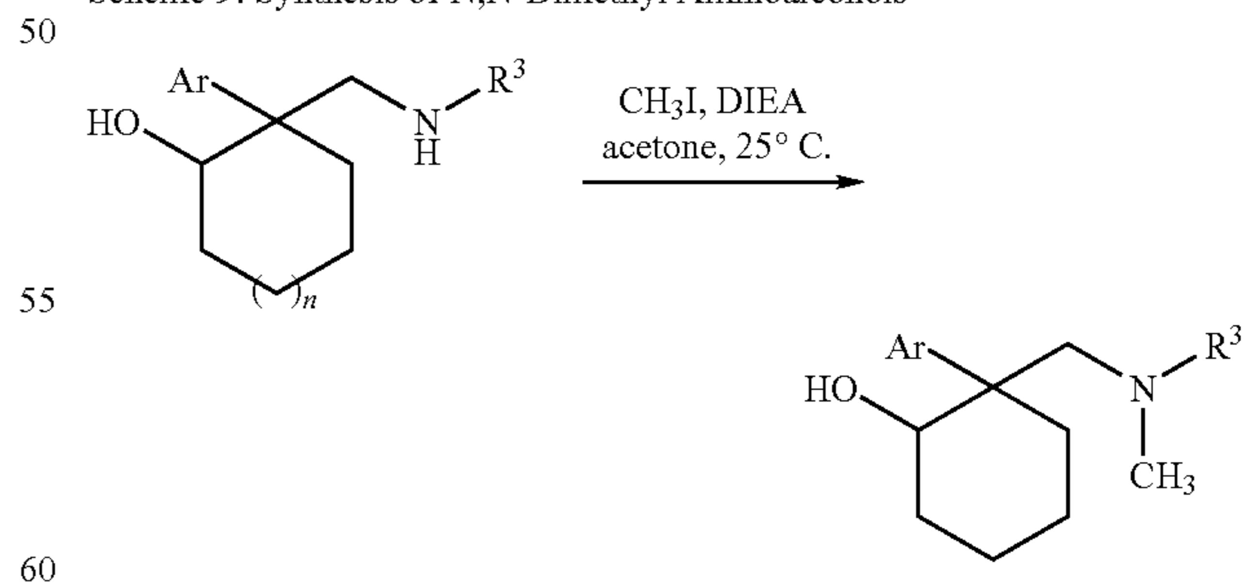
Scheme 9: Synthesis of N,N-Dimethyl Aminoalcohols
