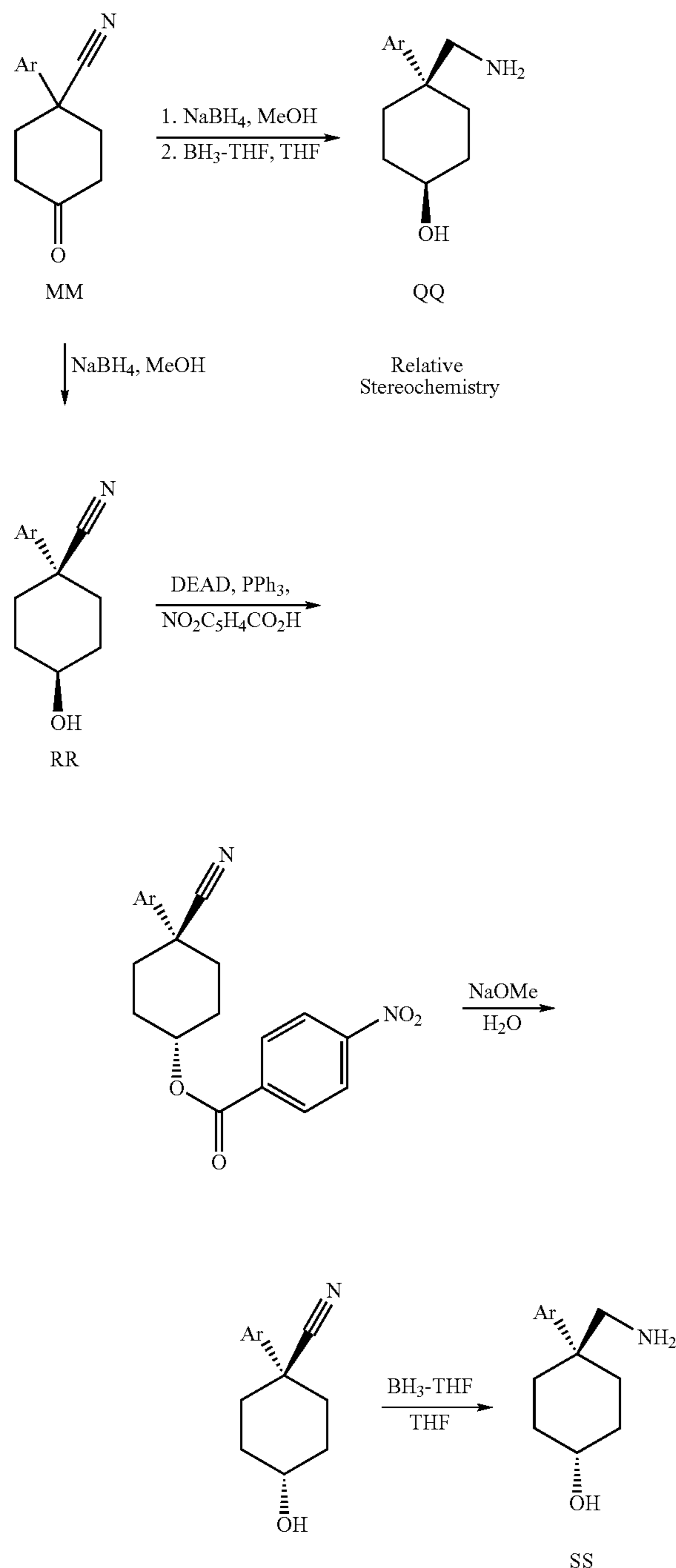
Scheme 17: Exemplary Synthesis of Chiral 4-OH-Cycloalkylamines
