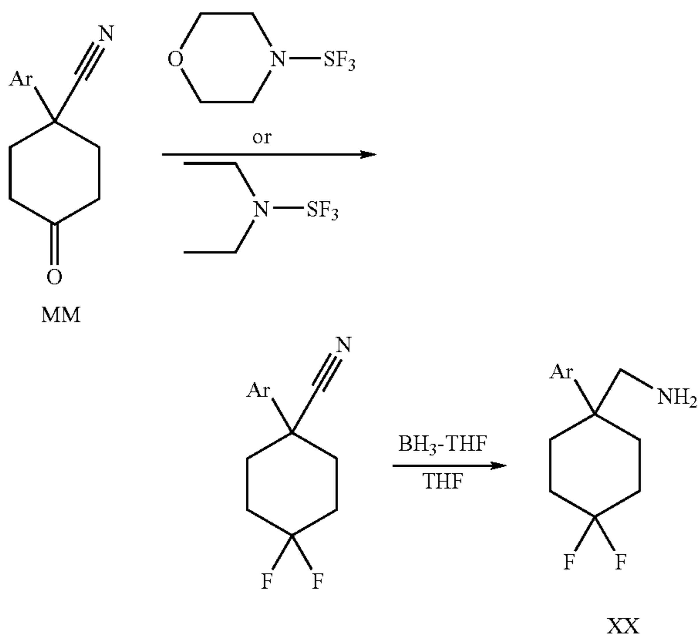
Scheme 20: Exemplary Synthesis of 4,4-Disubstituted Cycloalkylamines
