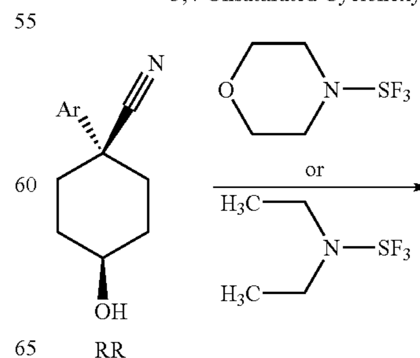
Scheme 19: Synthesis of 4-Fluoro-Cyclohexylamines and 3,4-Unsaturated Cyclohexylamines
