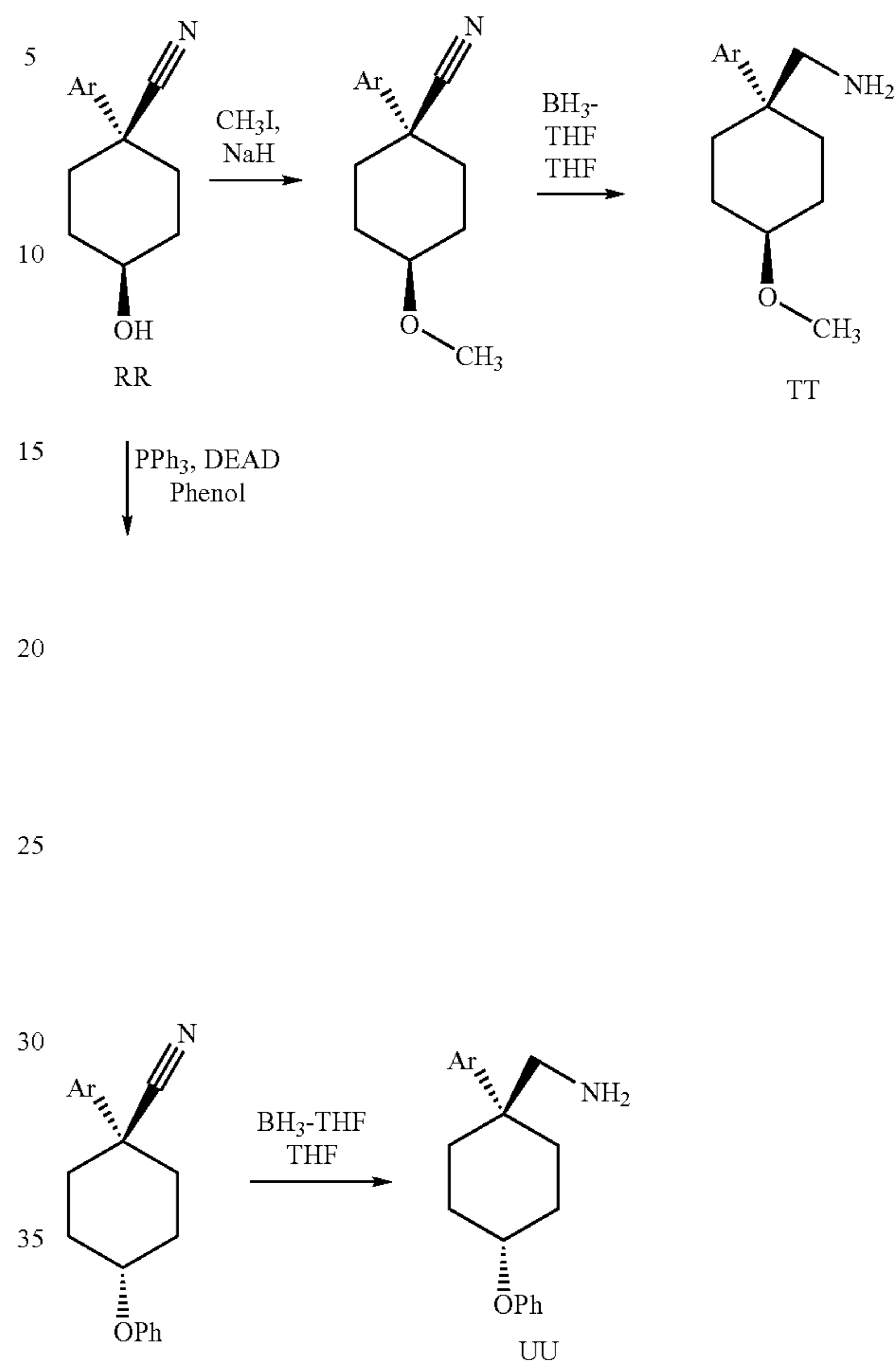
Scheme 18: Exemplary of 4-Alkoxy-Cyclohexylamines
