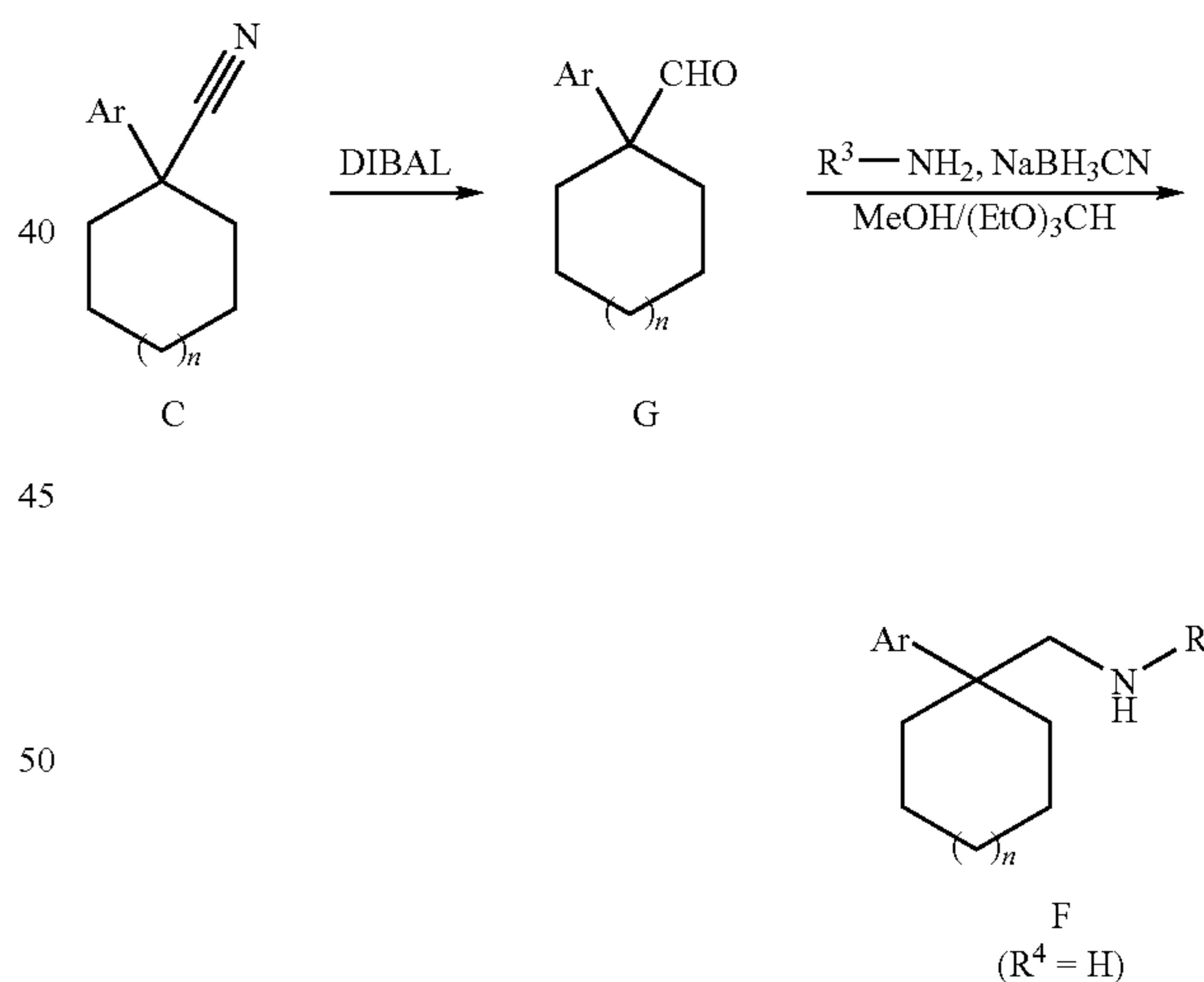
Scheme 3: Reduction of Nitriles to Aldehydes and Synthesis of Secondary Amines
