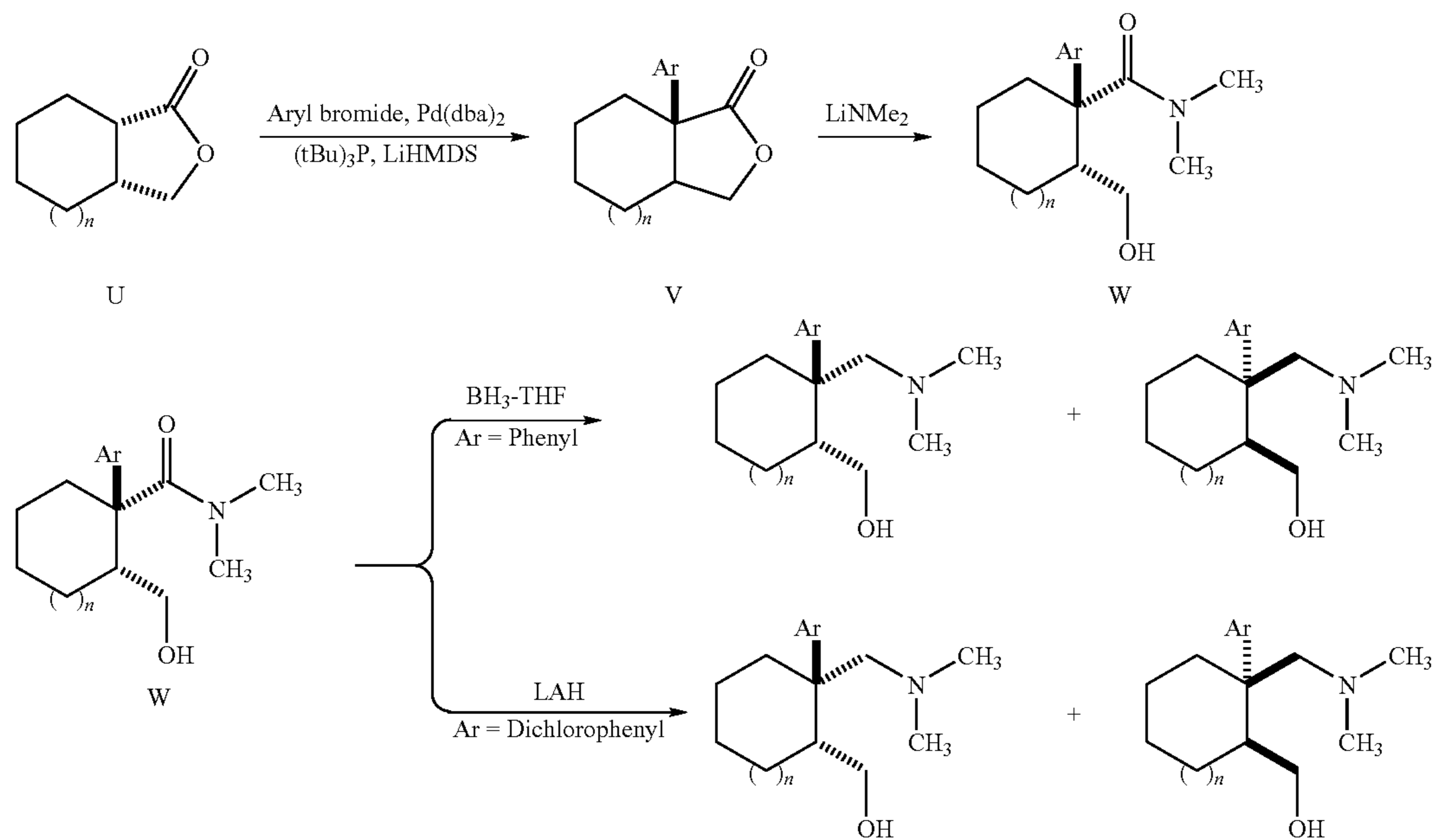
Scheme 10: Synthesis of 2-Hydroxymethyl Analogs
