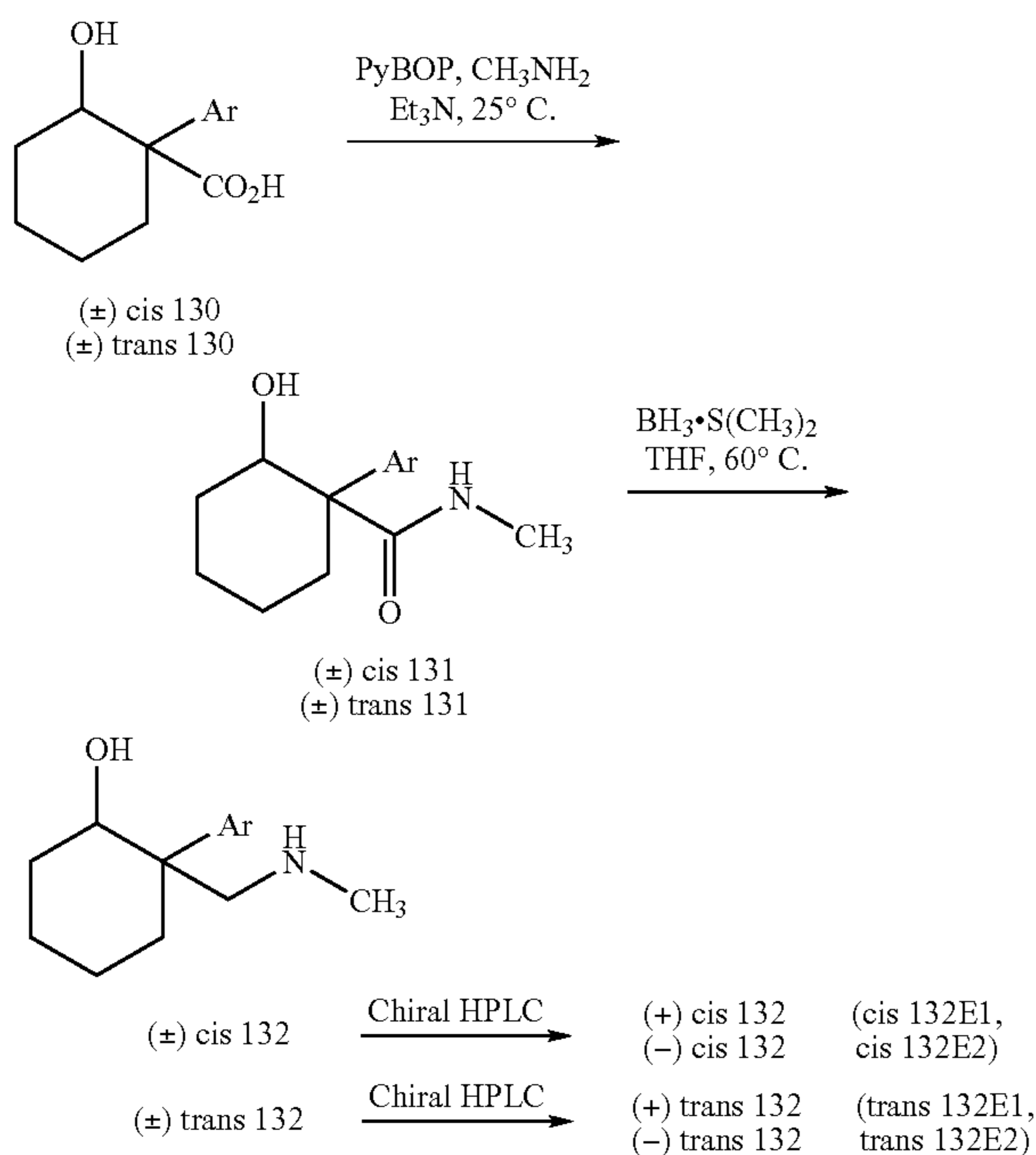
Scheme 28: Preparation of Chiral 2-Hydroxy-Cycloalkylamines
