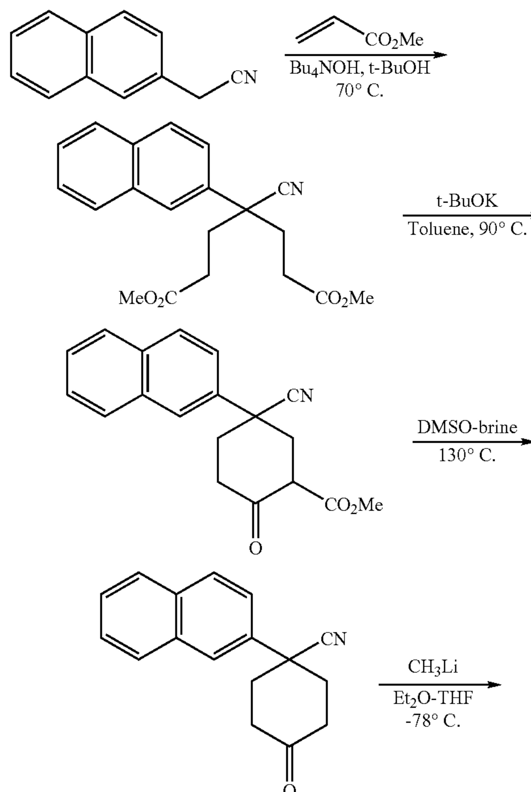
Scheme 33: Preparation of 225 hydrochloride
