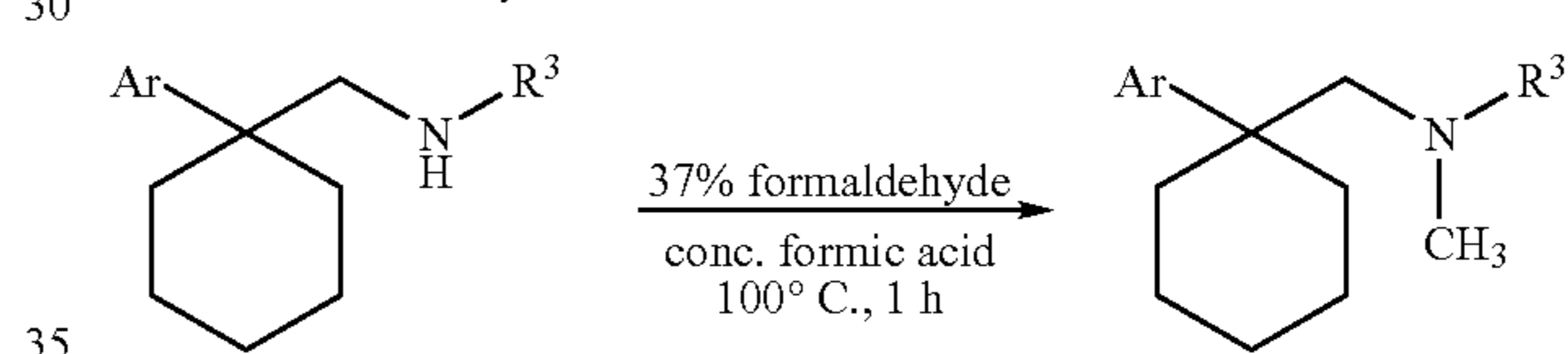
Scheme 6: Exemplary Synthesis of Tertiary Amines from Secondary Amines
