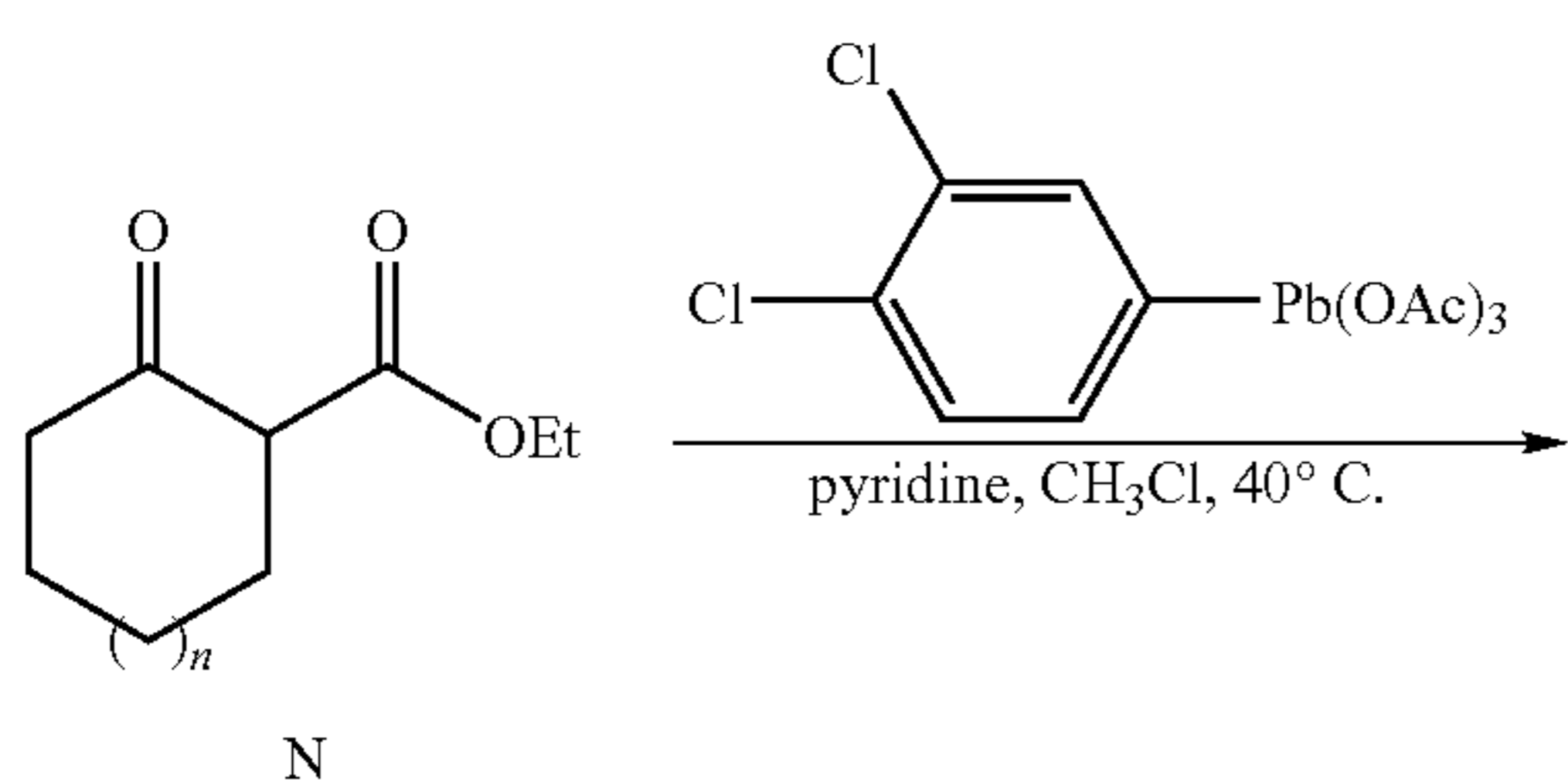
Scheme 8: Synthesis of 2-Substituted Cycloalkylamines
