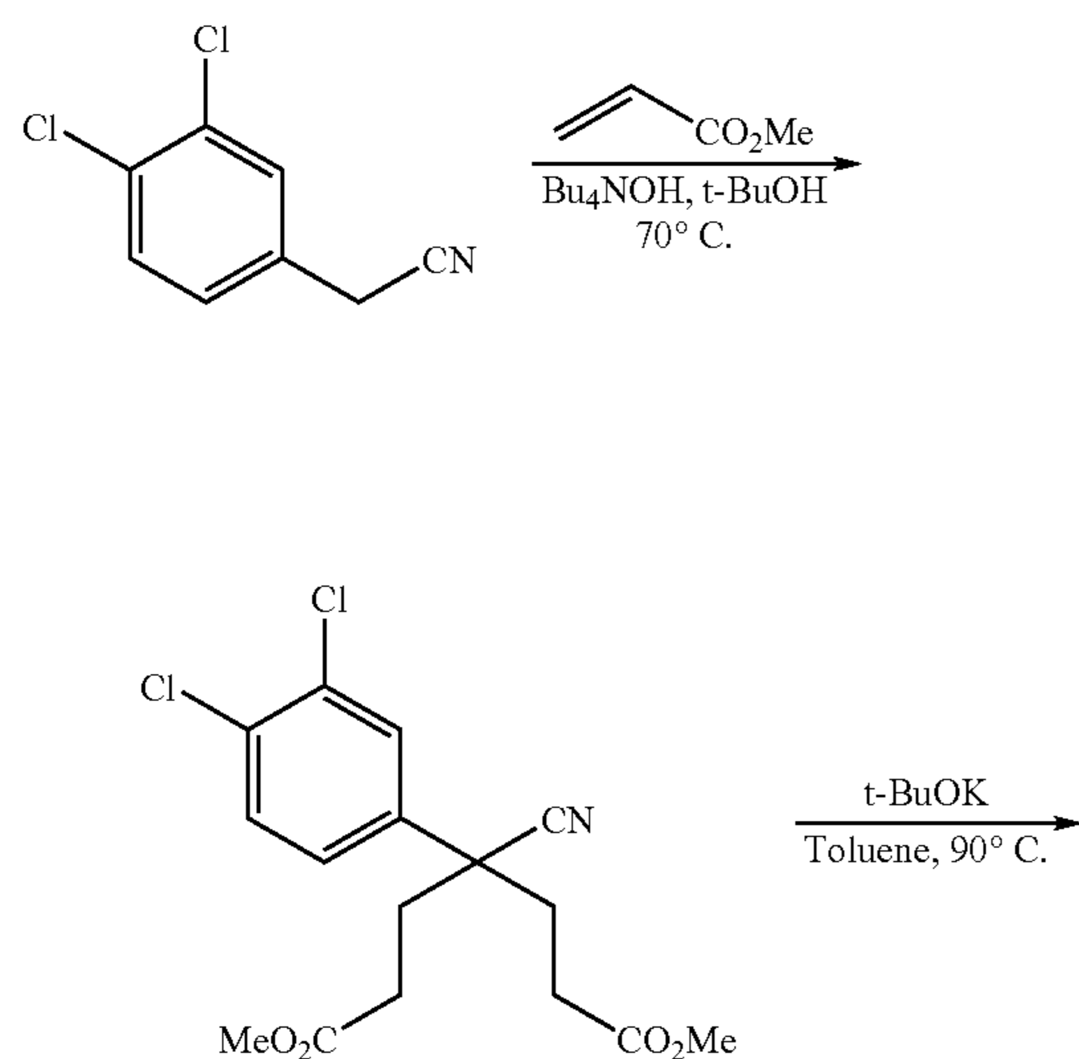
Scheme 36: Preparation of 277 Hydrochloride
