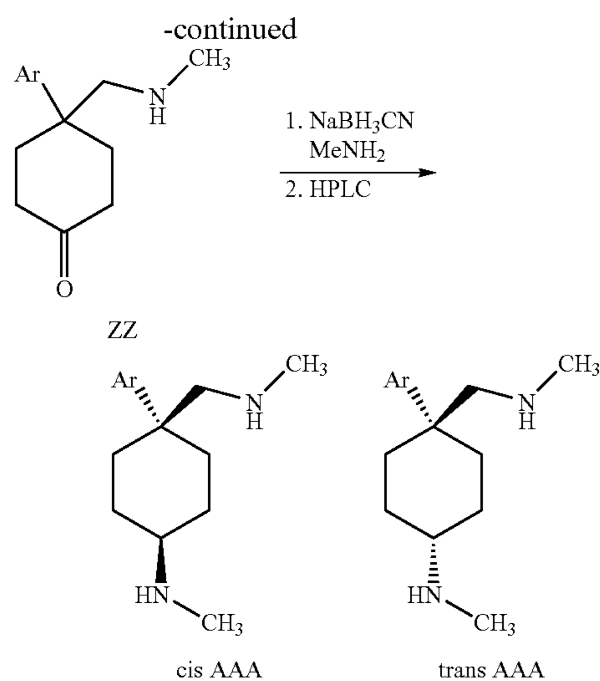
Scheme 24: Synthesis of Cycloalkyl-Pyrrolidine Analogs of the Invention
