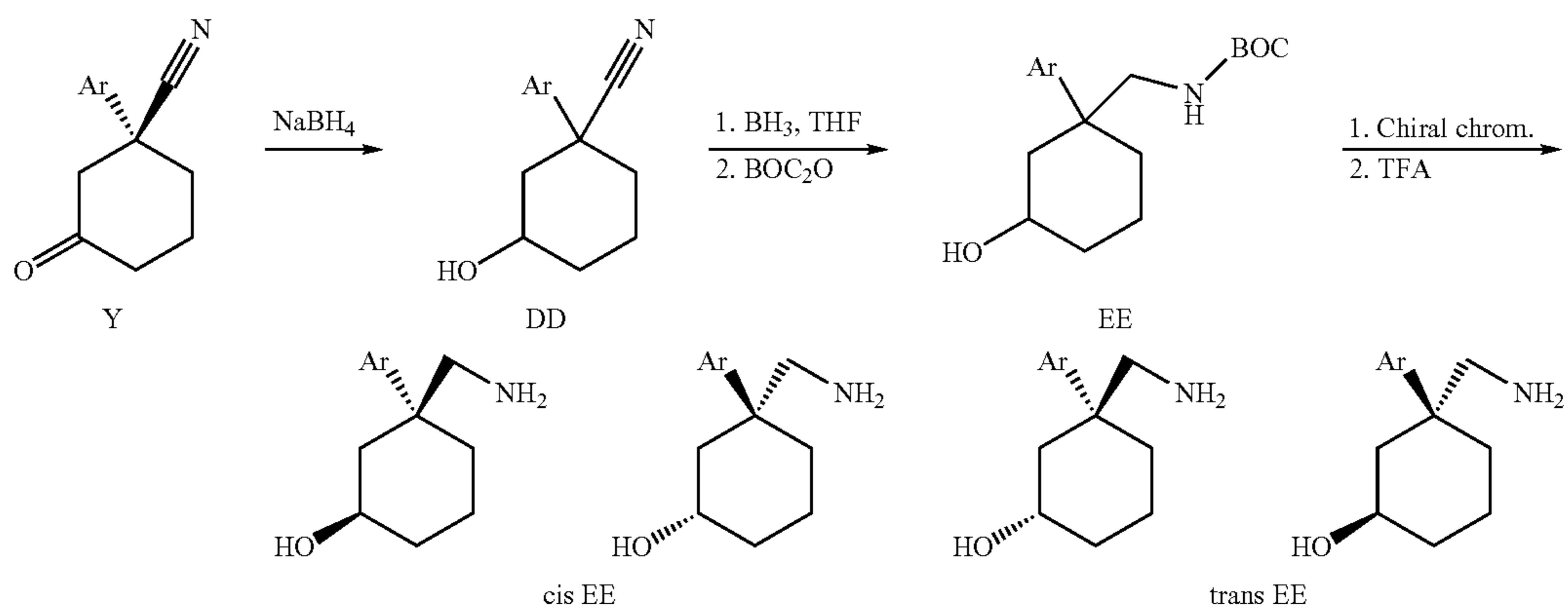
Scheme 12: Exemplary Synthesis of 3-OH-Substituted Cyclohexylamines
