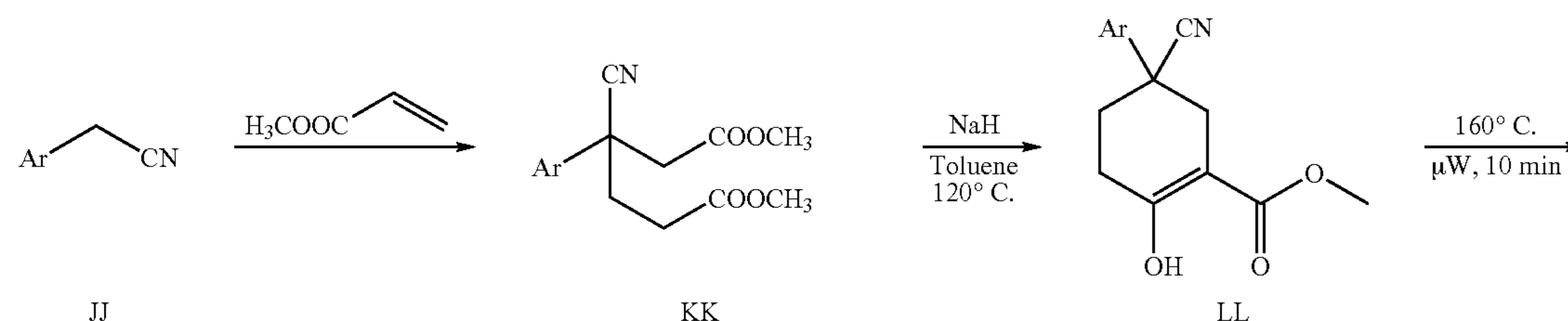
Scheme 15: Exemplary Synthesis of 4-OH-Cycloalkylamines
