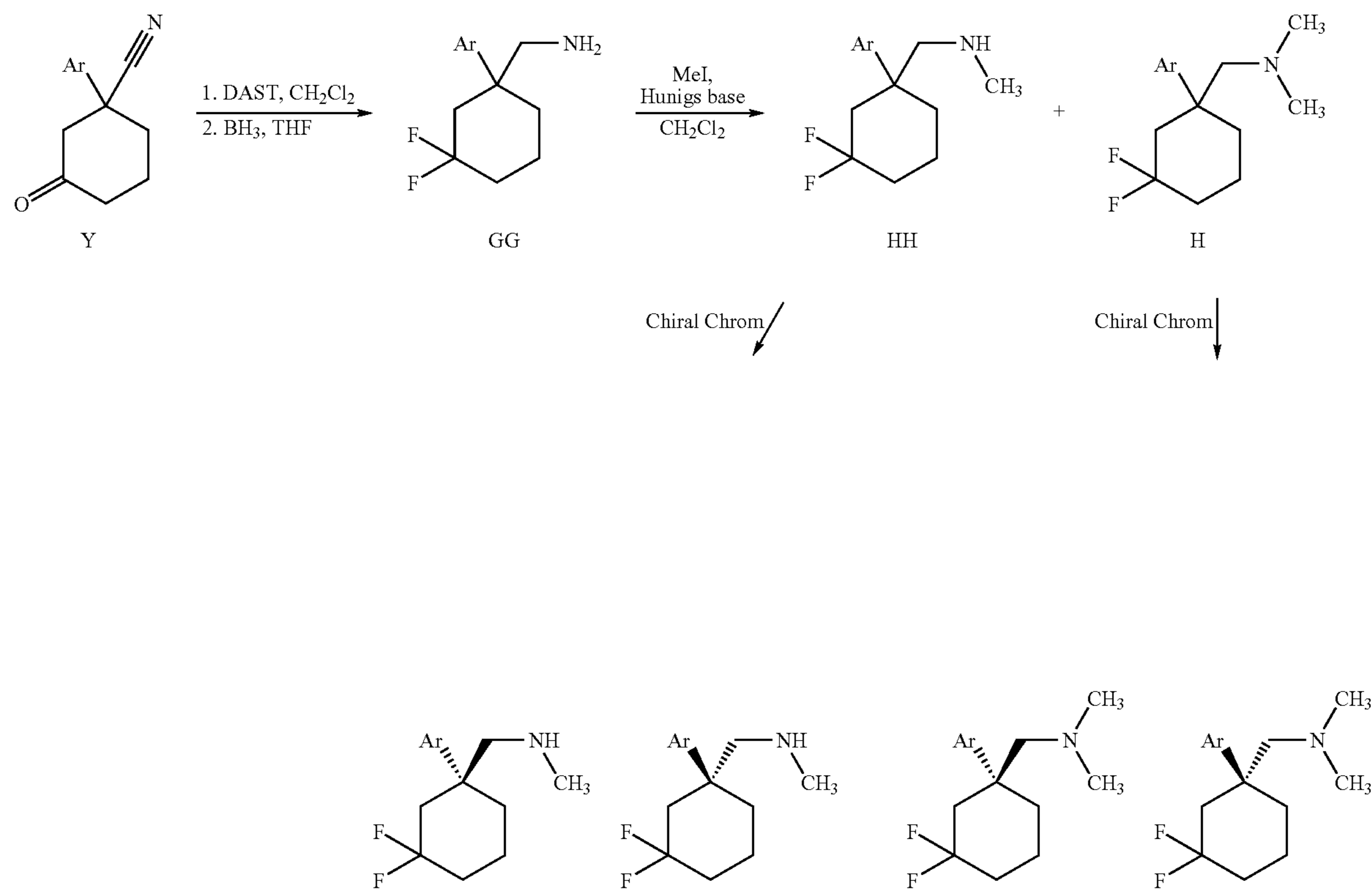
Scheme 14: Exemplary Preparation of 3,3-Difluoro Chiral Amines
