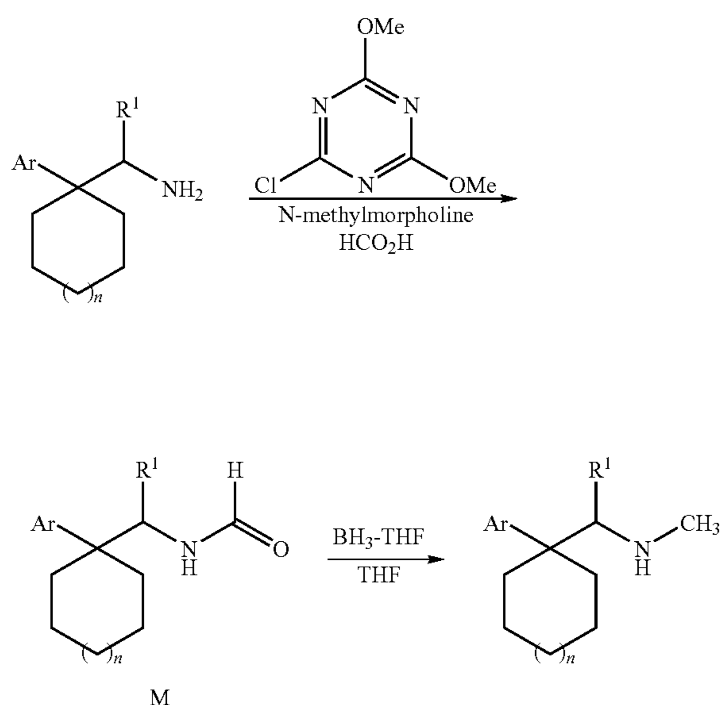
Scheme 5: Exemplary Synthesis of Secondary Amines
