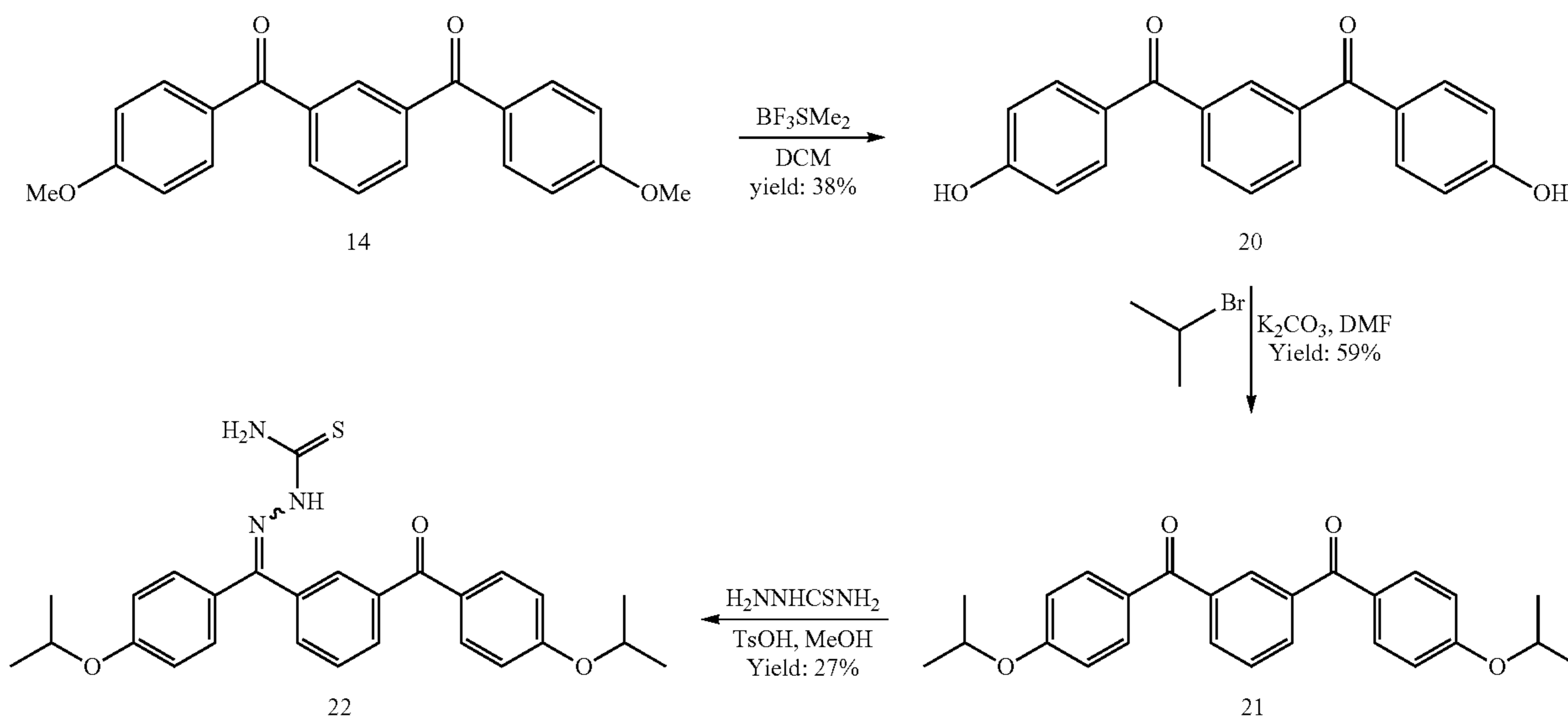
J. 1,3-bis-(4-isopropoxybenzoyl)benzene thiosemicarbazone (22)
