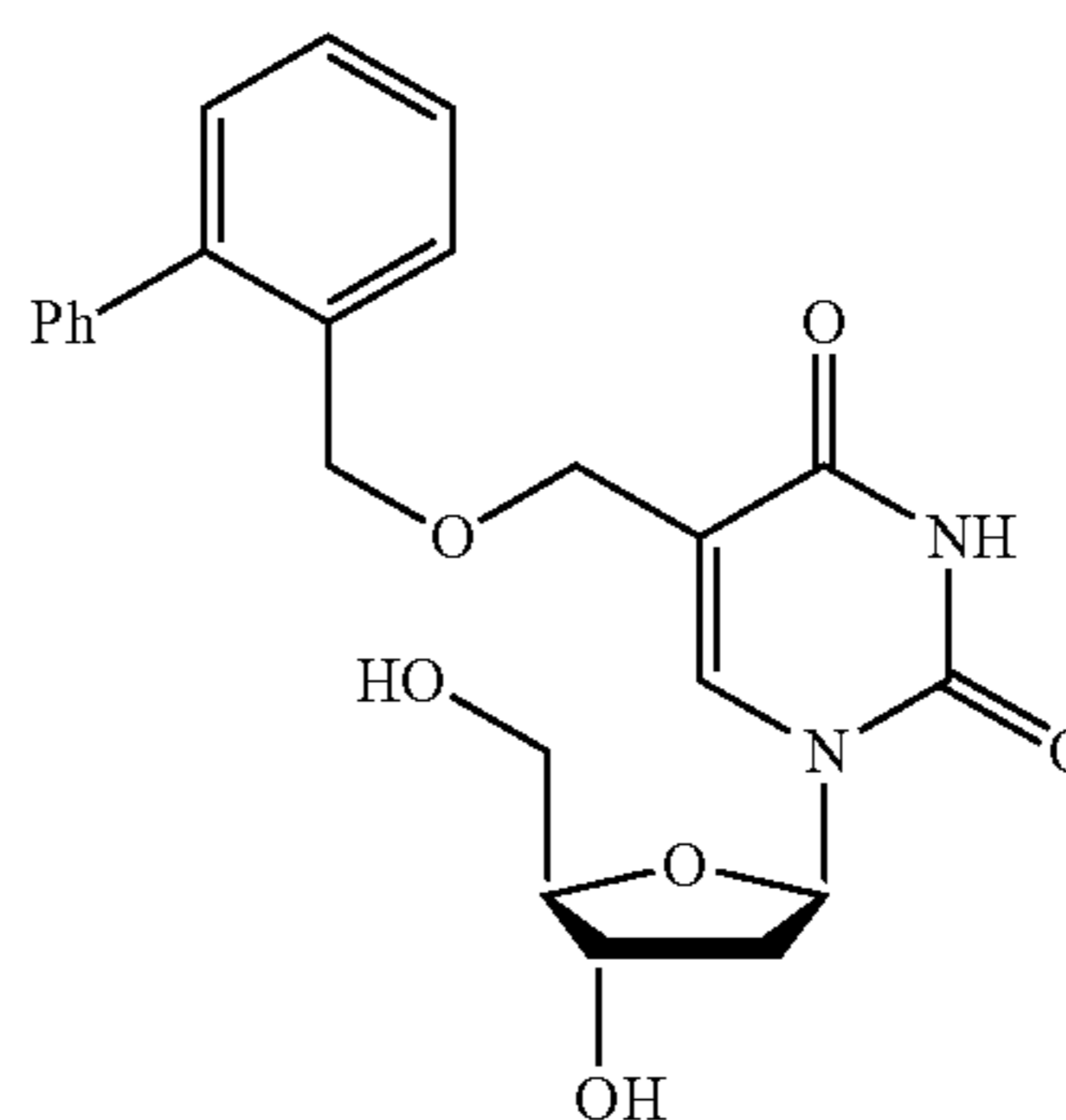
5-(2-phenylbenzyloxy)methyl-2'-deoxyuridine
