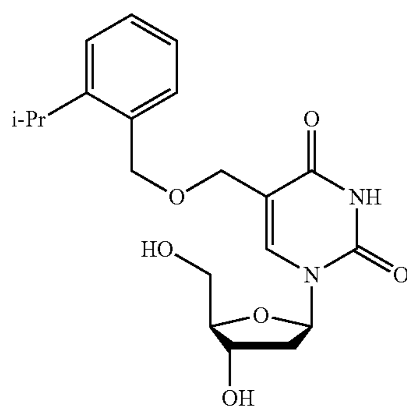
5-(2-isopropylbenzyloxy)methyl-2'-deoxyuridine
