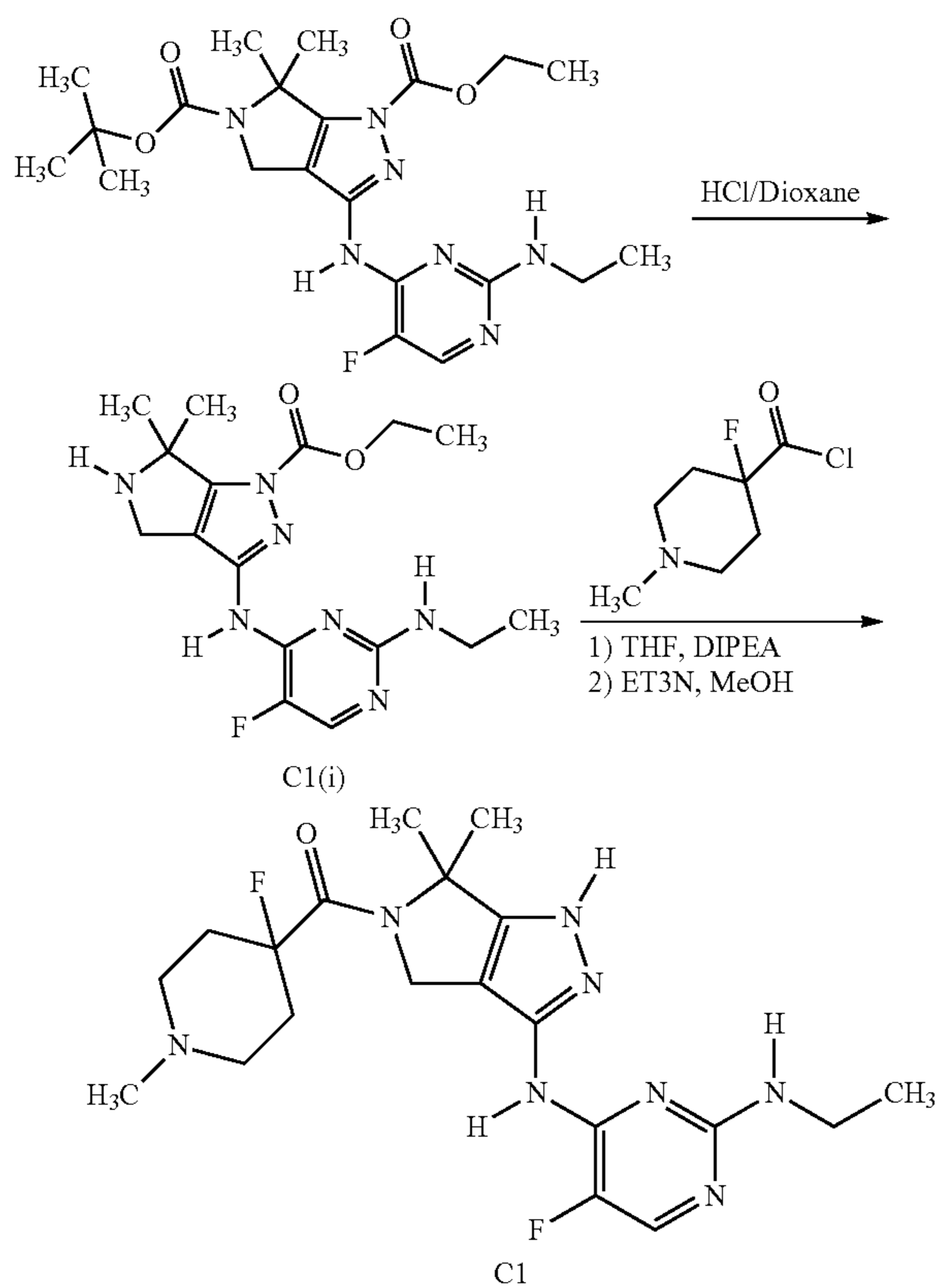
Intermediate C1(i)
