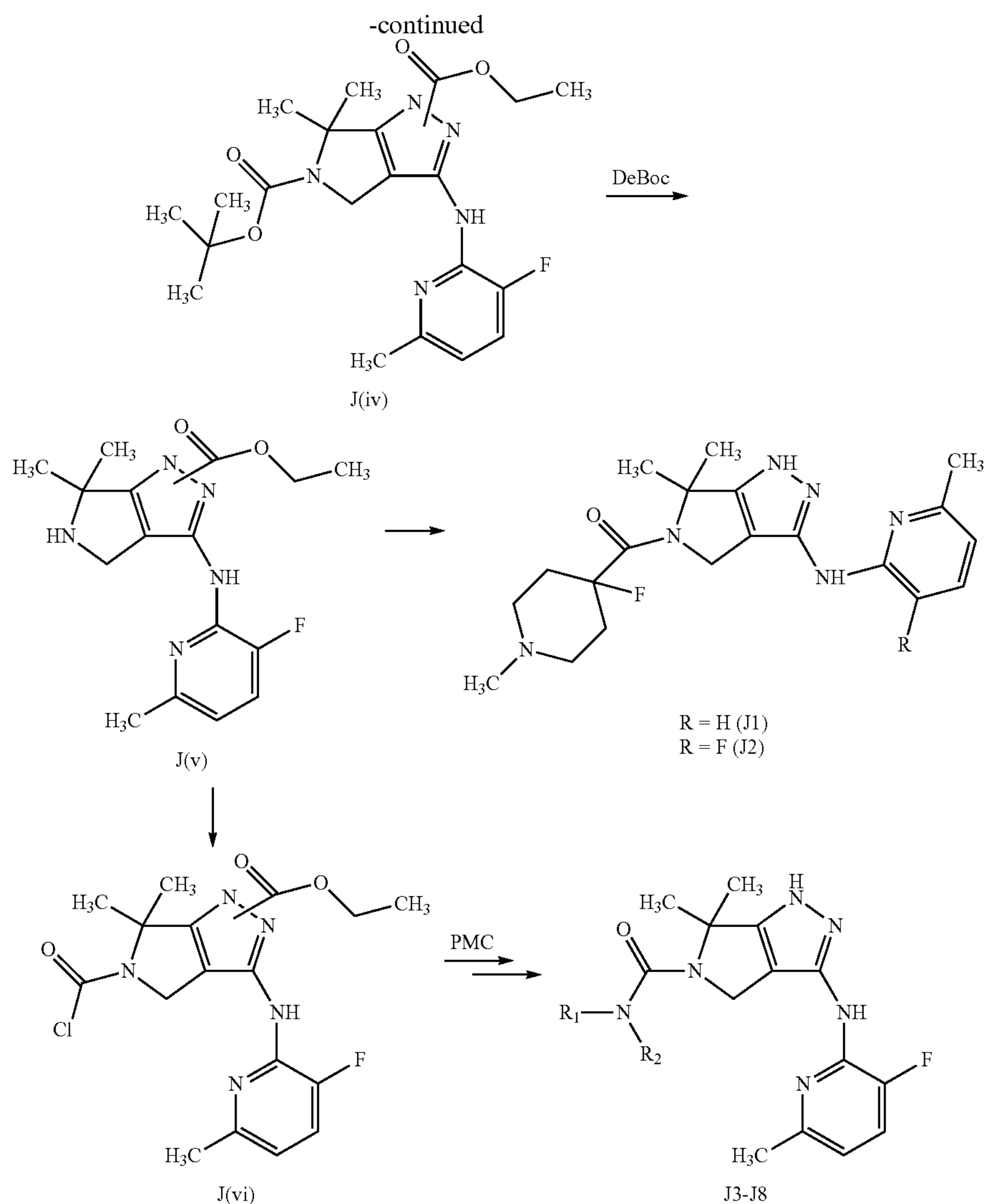
Intermediate J(i)
