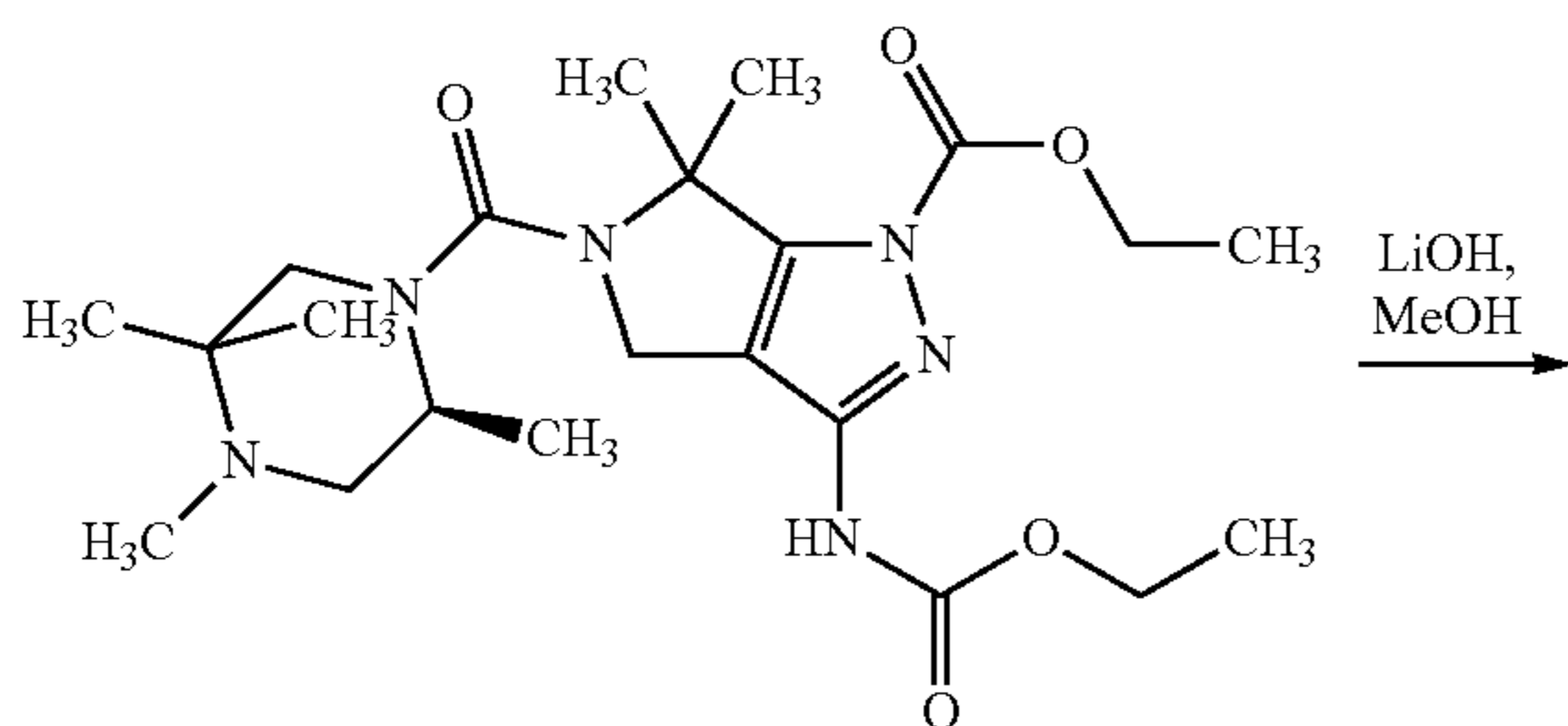
A1(iii)
