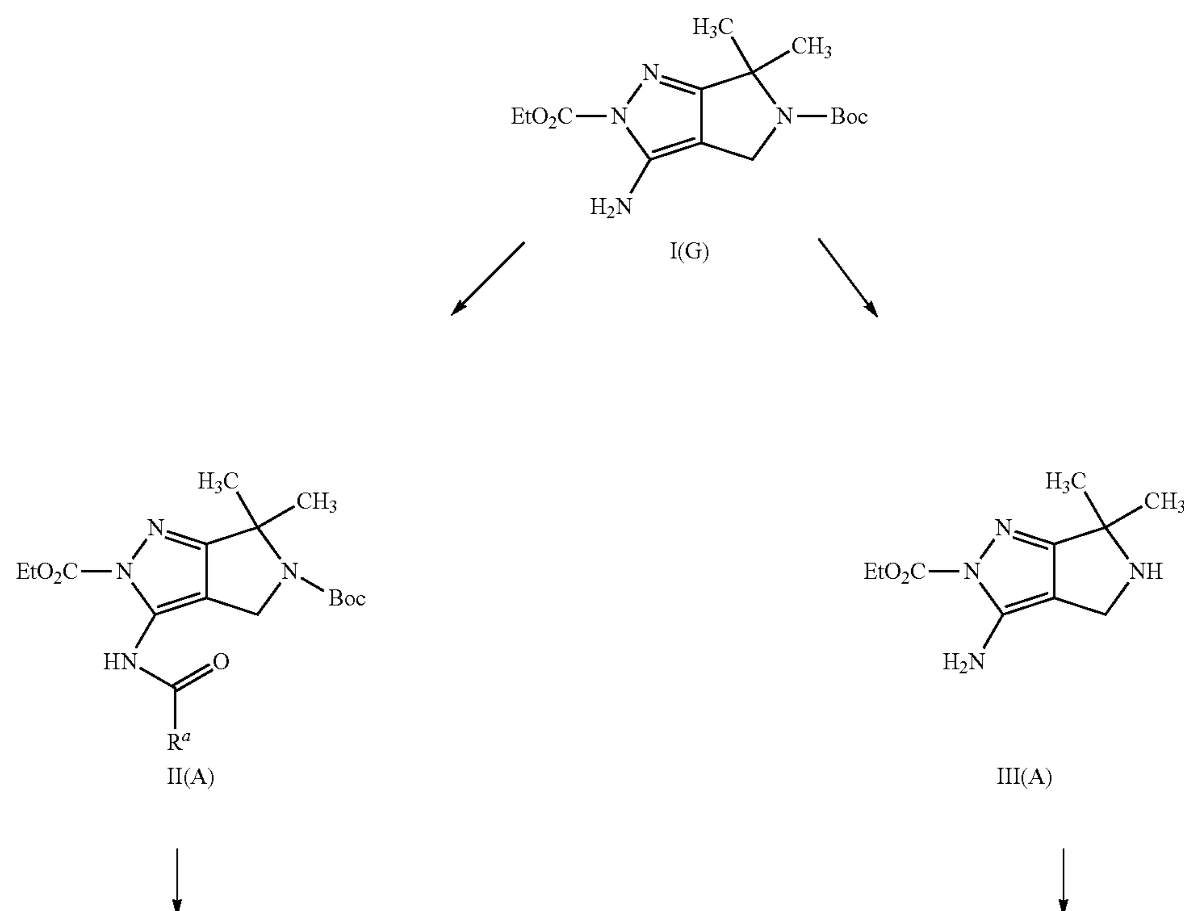
Scheme 2
