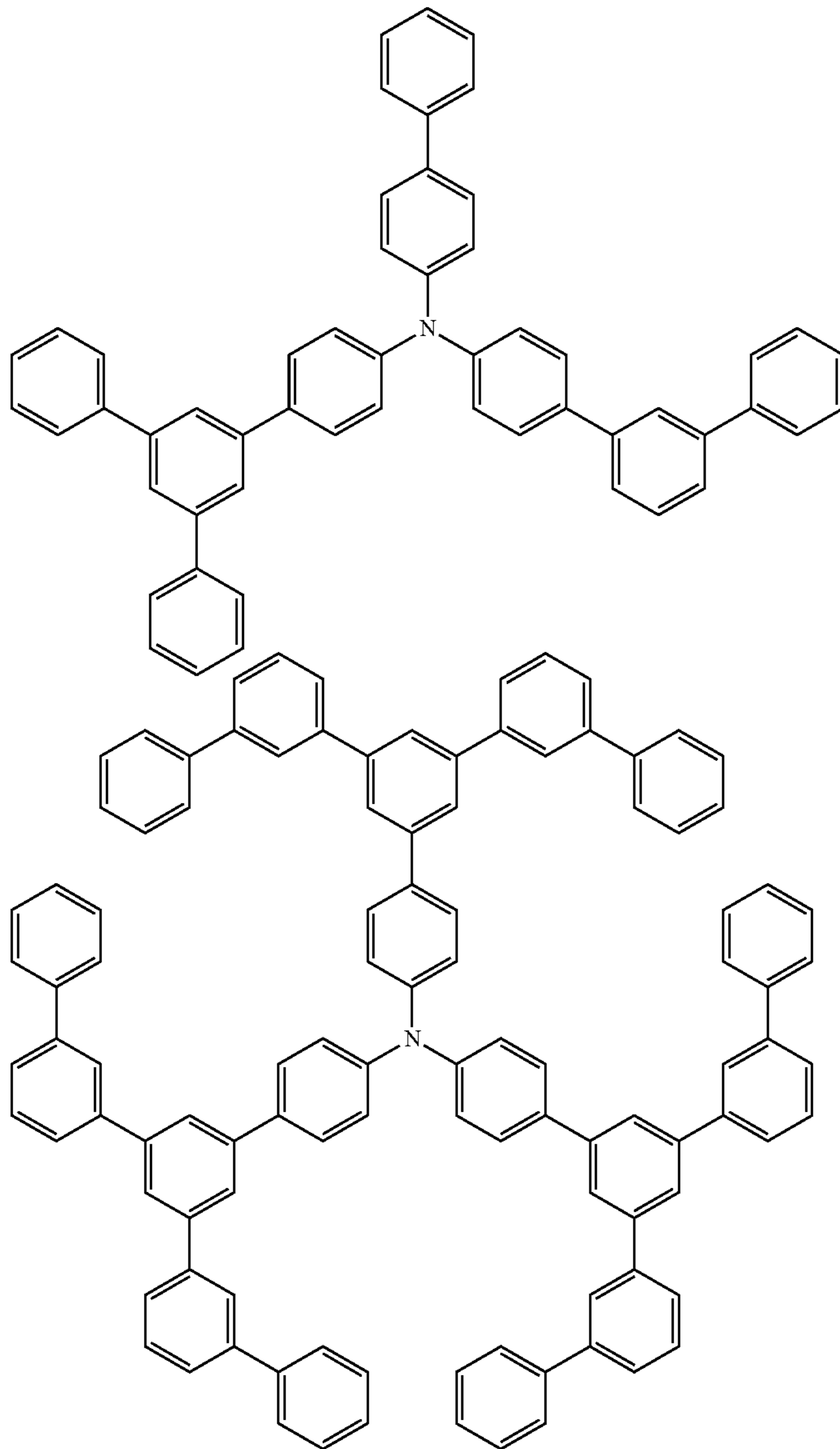
[Chem 24]
