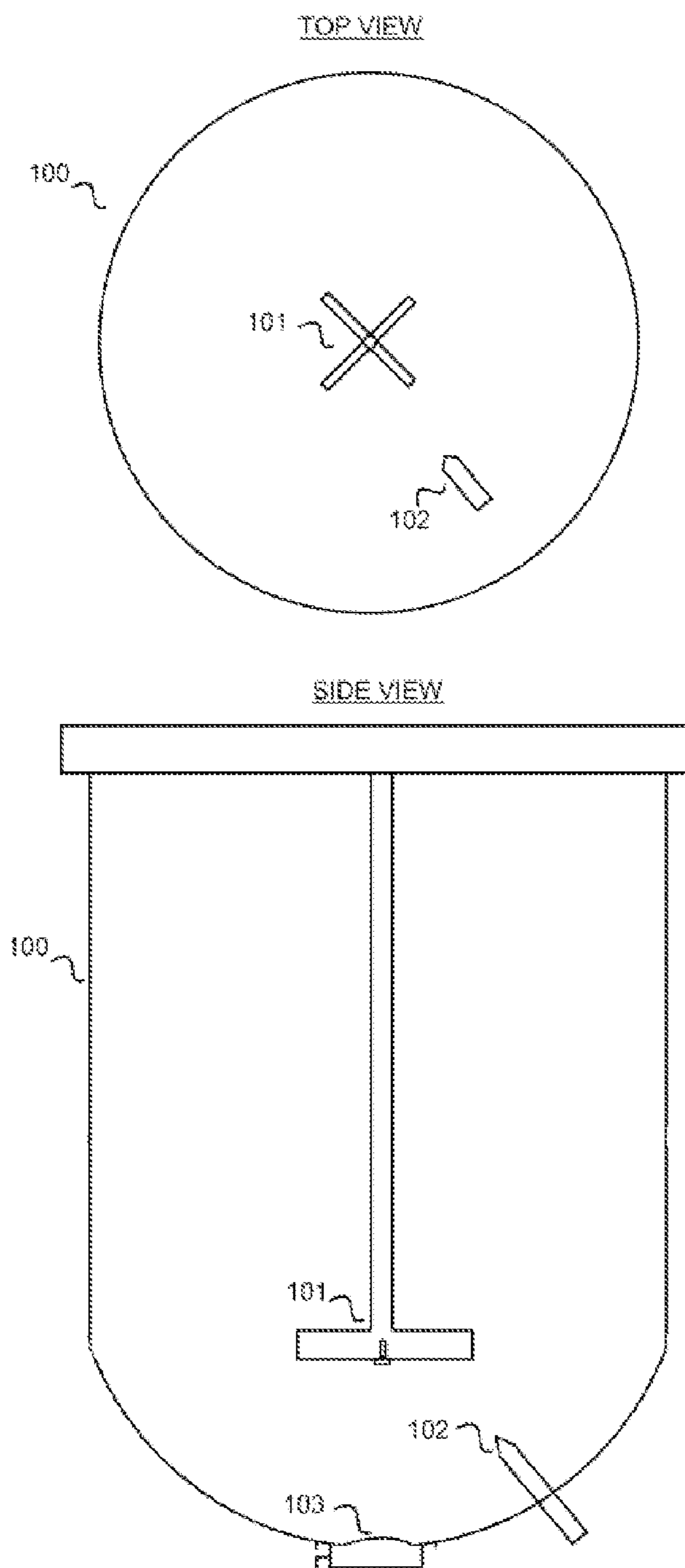
Fig. 17: 200-L reaction vessel with standard agitator arrangement.
