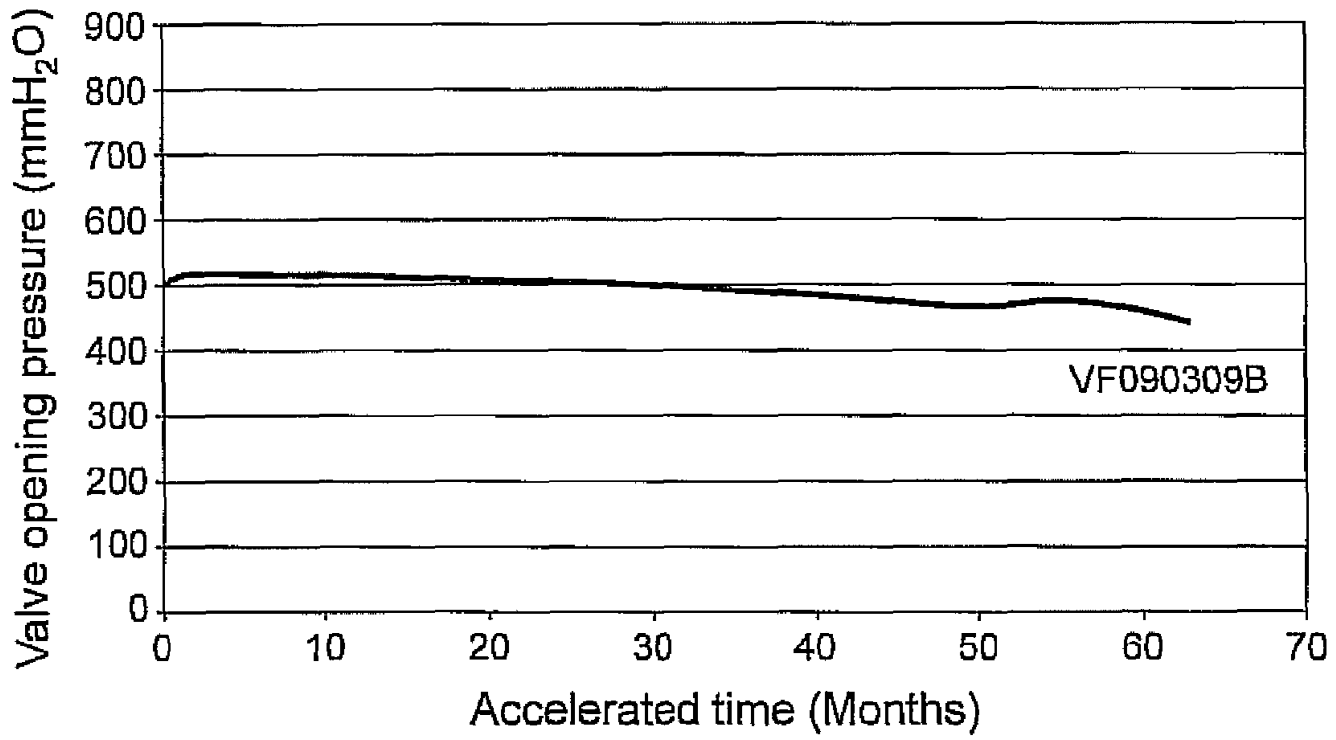
Valve Function stability in Simulated Gastric Fluid
