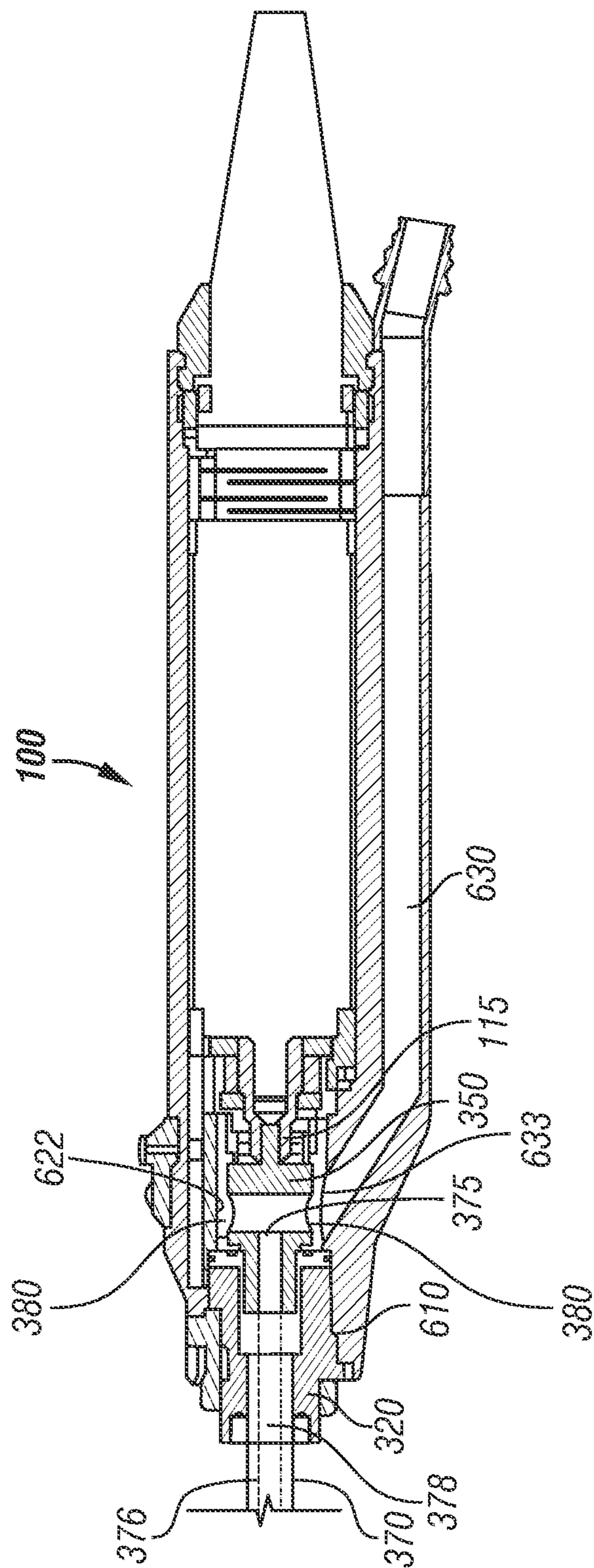
FIG. 2 (PRIOR ART)
