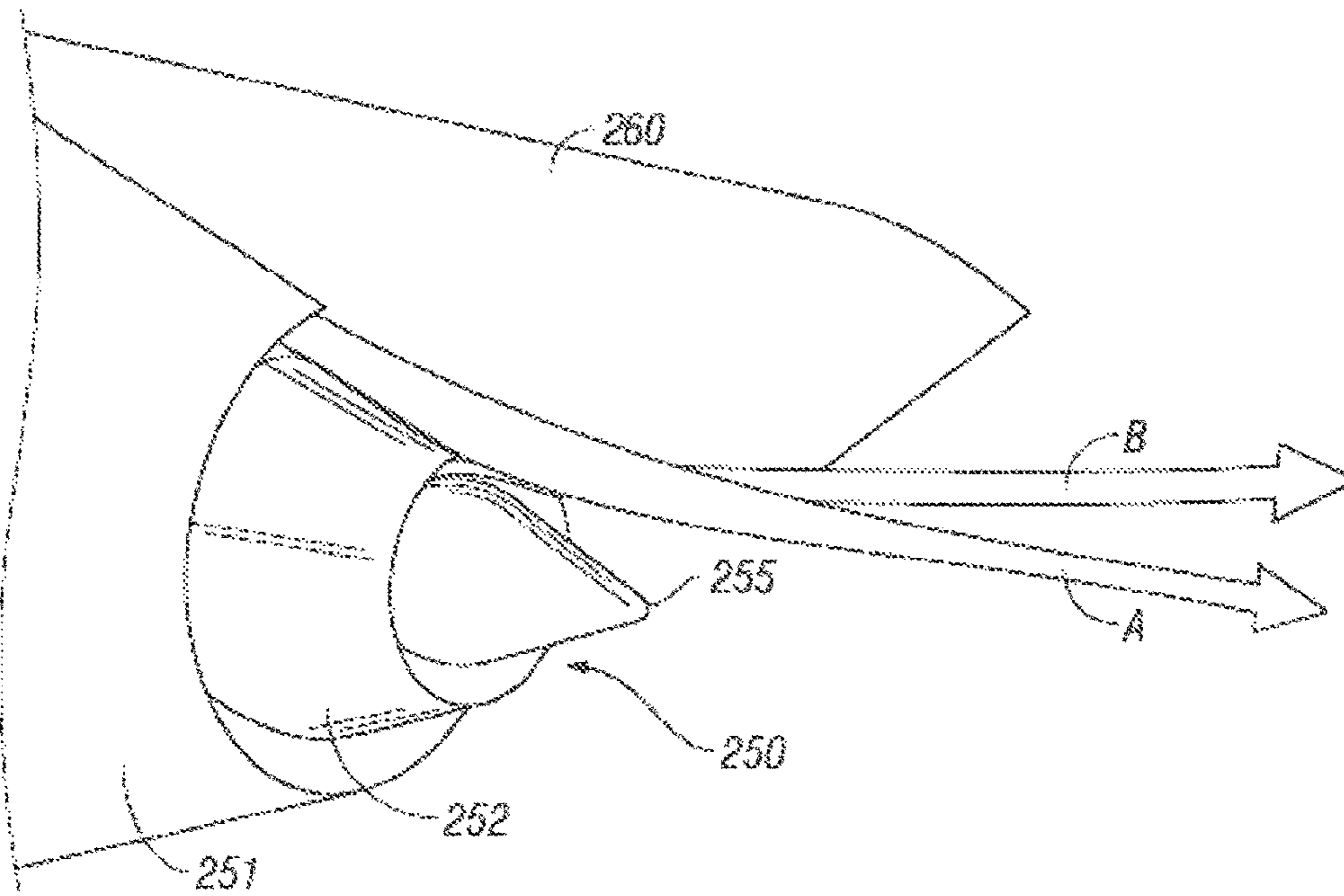
FIG. 4 (Prior Art)
