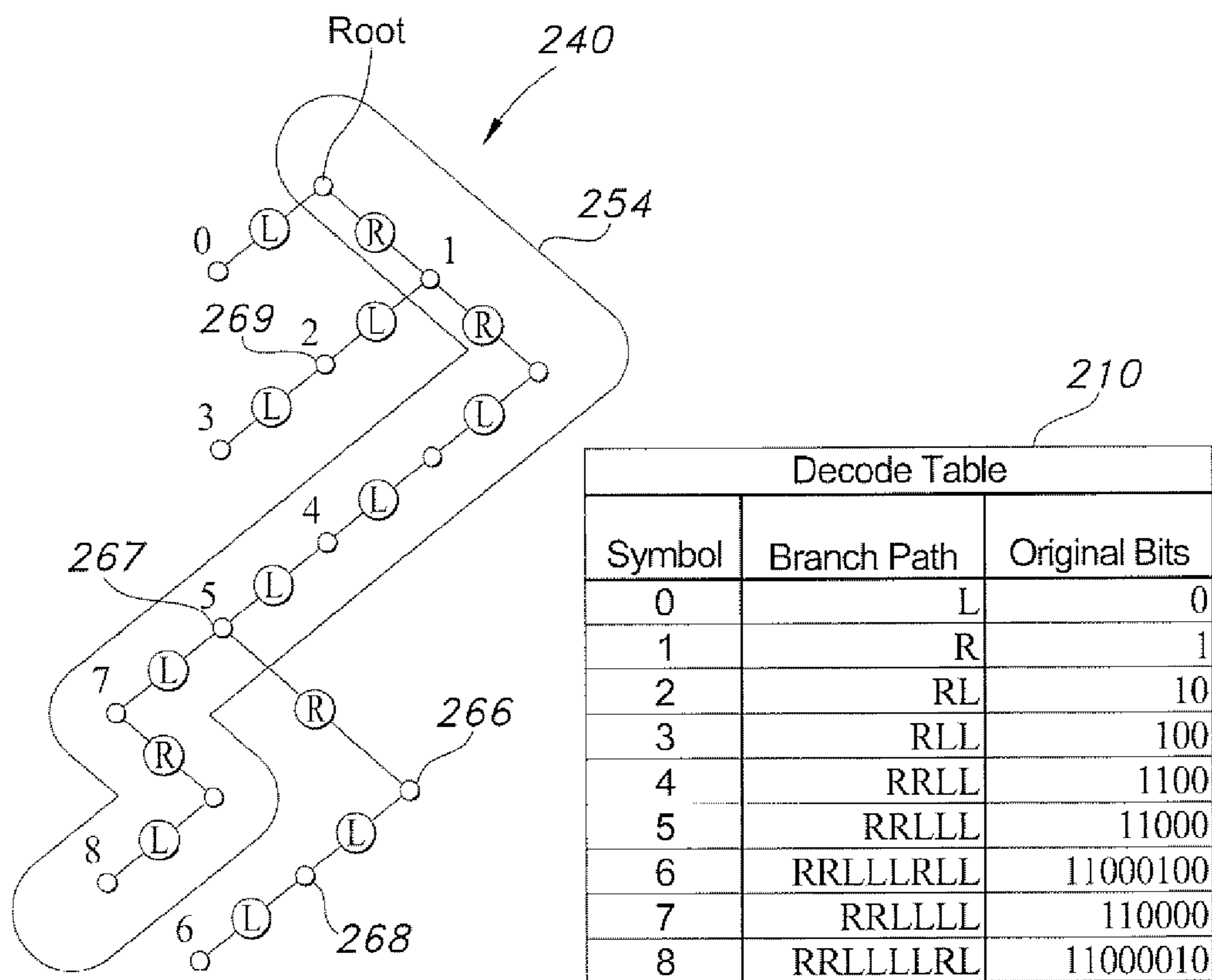
Decode Tree
