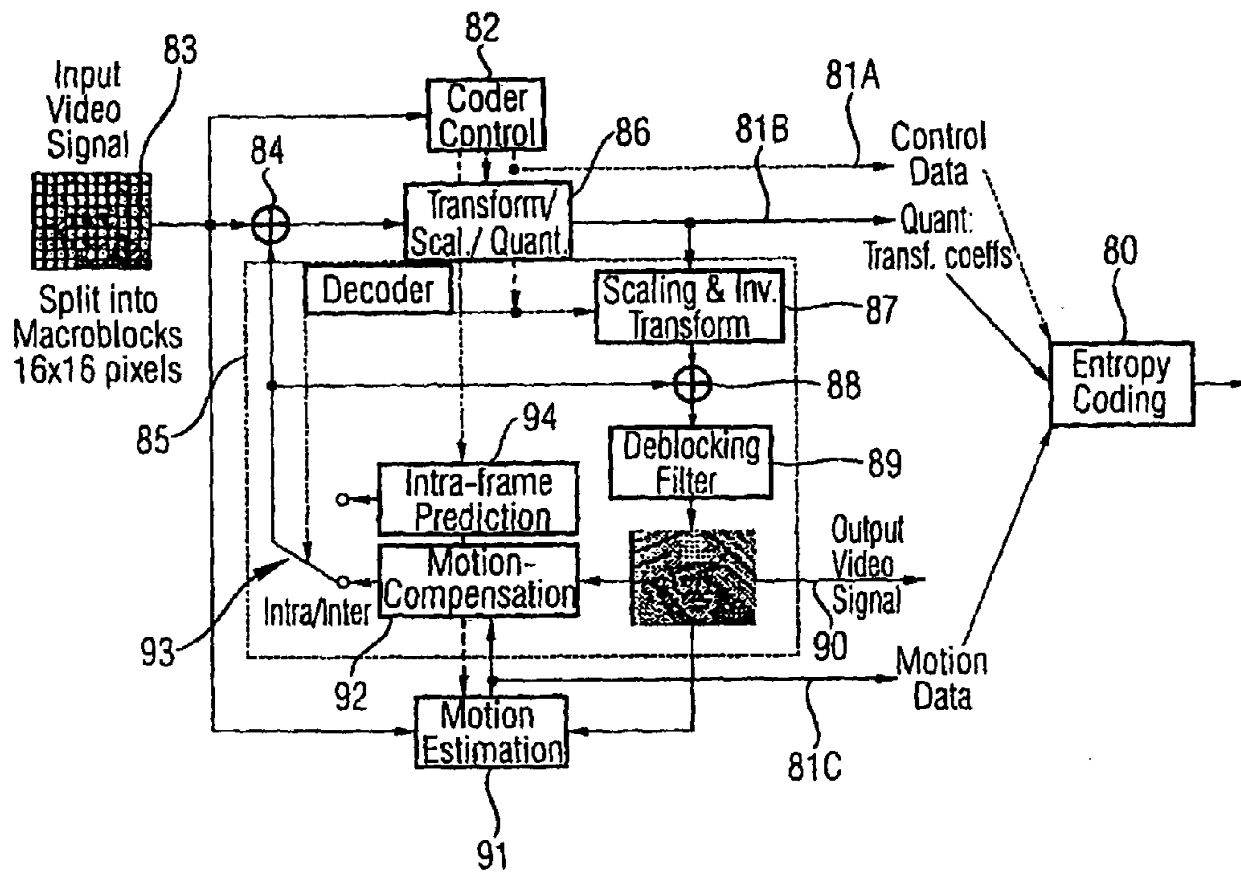
FIG. 9 (prior art)
