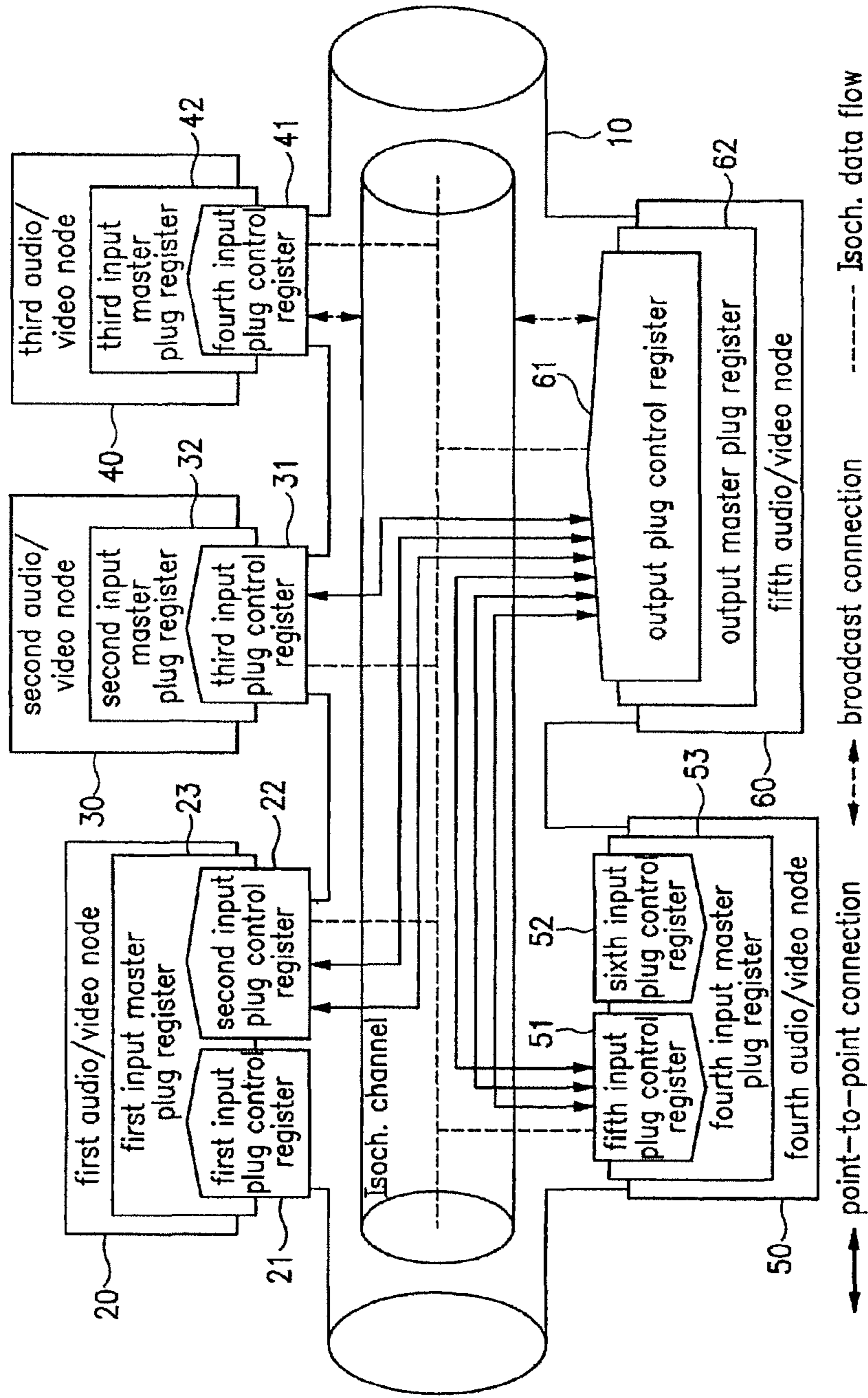
FIG. 1 Related Art
