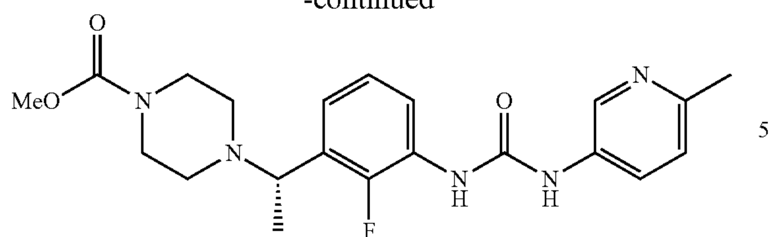
(S)-methyl 4-(1-(2-fluoro-3-(3-(6-methylpyridin-3-yl)ureido)phenyl)ethyl)piperazine-1-carboxylate
