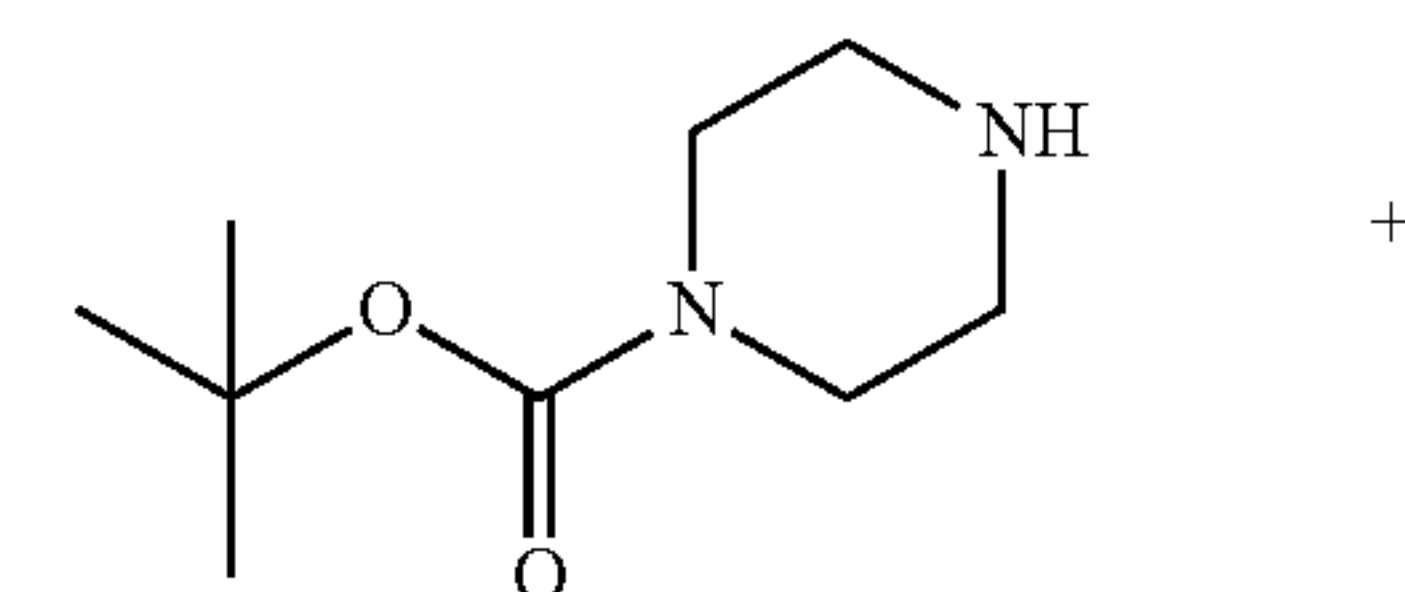
tert-butyl piperazine-1-carboxylate
