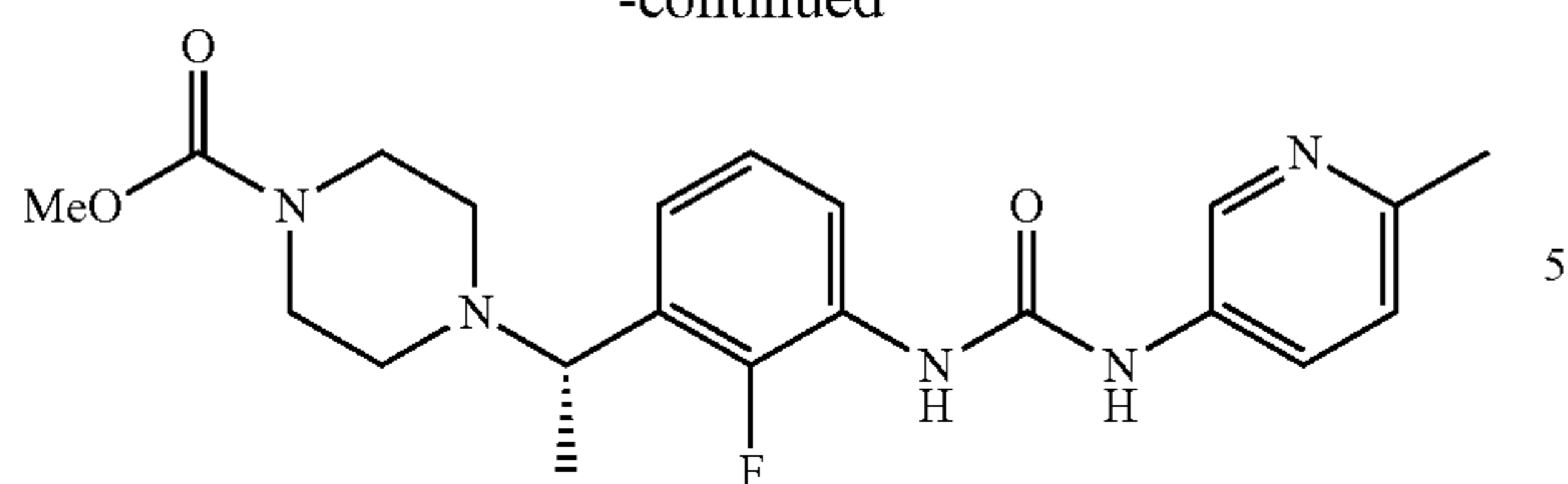
(S)-methyl 4-(1-(2-fluoro-3-(3-(6-methylpyridin-3-yl)ureido)phenyl)ethyl)piperazine-1-carboxylate
