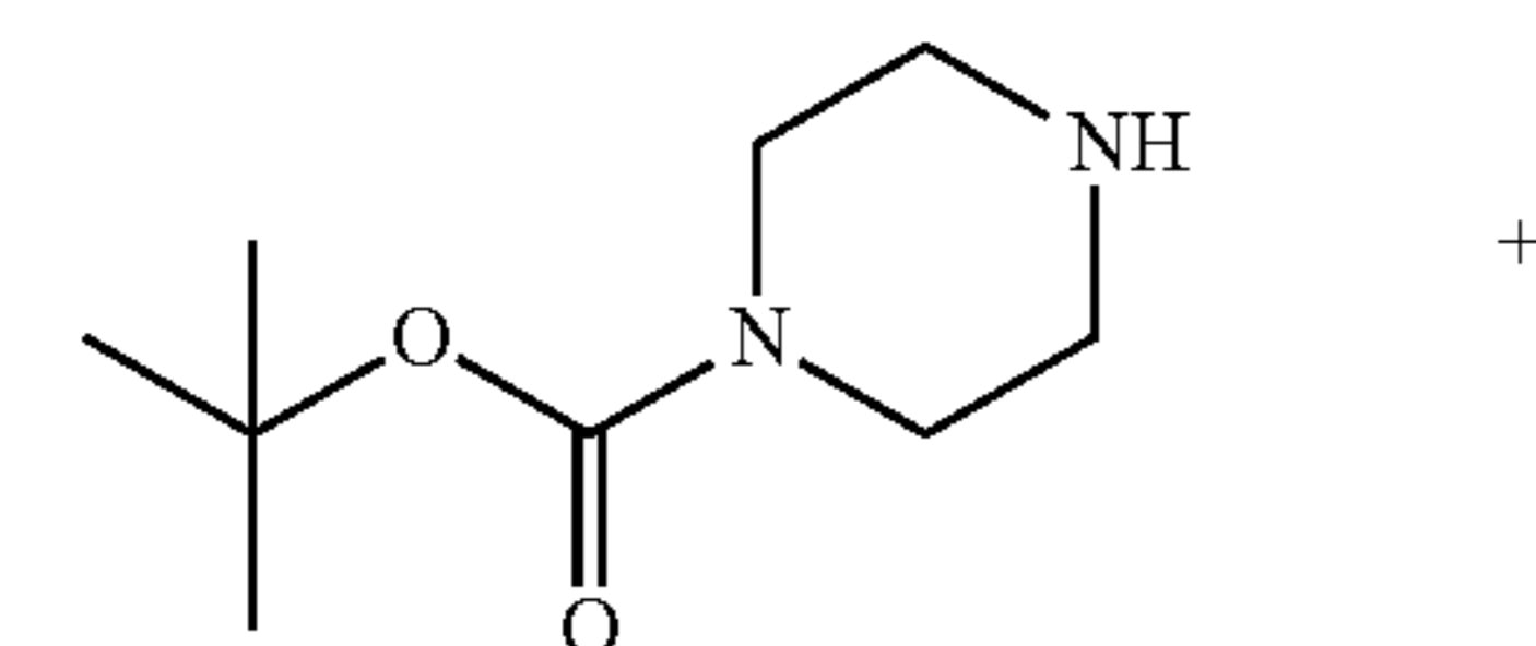
tert-butyl piperazine-1-carboxylate
