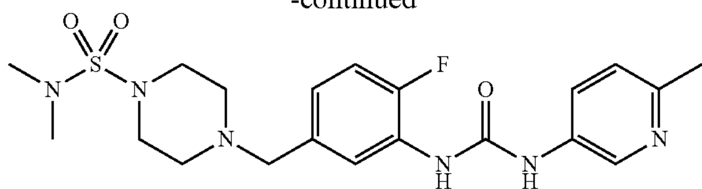
4-(4-fluoro-3-(3-(6-methylpyridin-3-yl)ureido)benzyl)-N,N-dimethylpiperazine-1-sulfonamide
