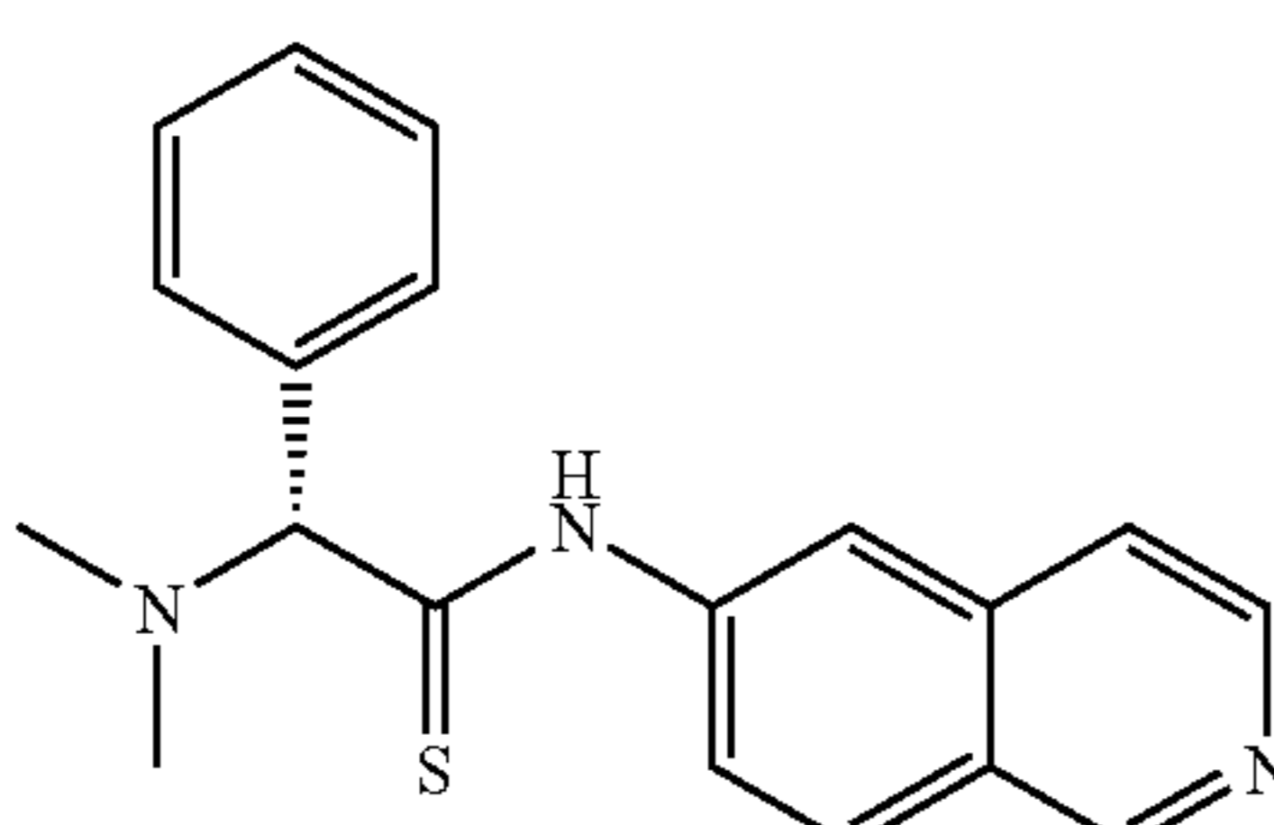
(R)-2-(dimethylamino)-N-(isoquinolin-6-yl)-2-phenylethanethioamide
