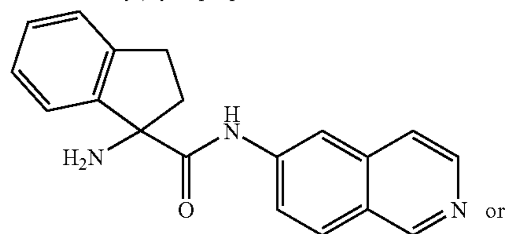
1-amino-N-(isoquinolin-6-yl)-2,3-dihydro-1H-indene-1-carboxamide
