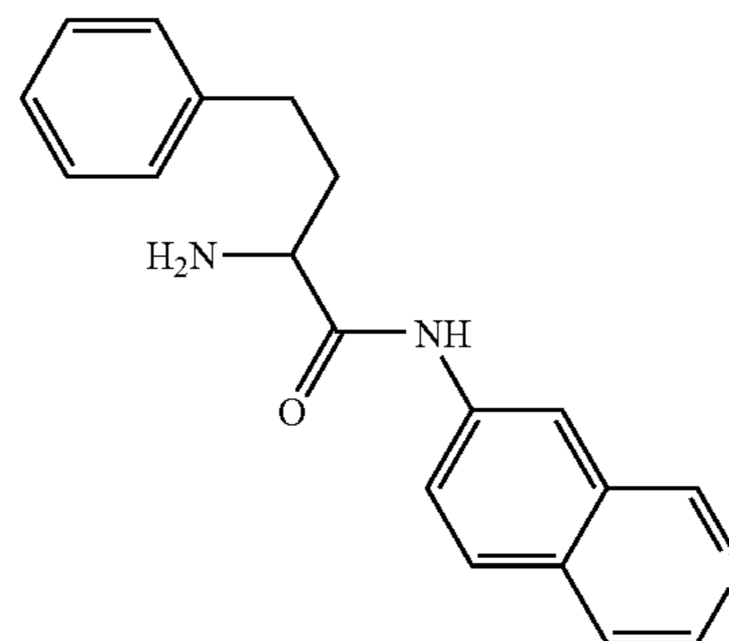
2-amino-N-(isoquinolin-7-yl)-4-phenylbutanamide
