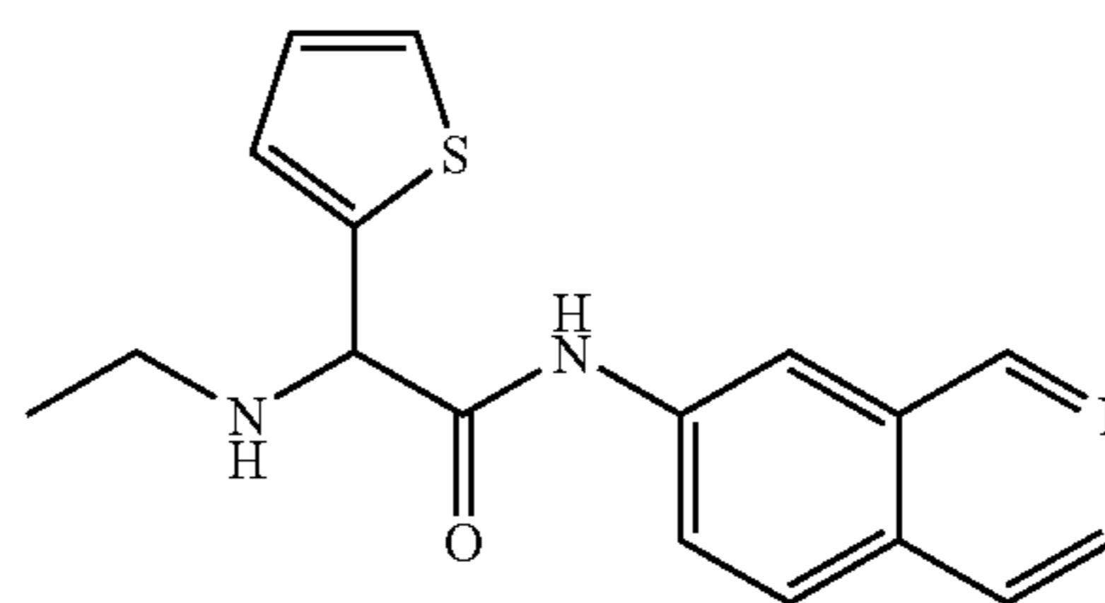
2-(ethylamino)-N-(isoquinolin-7-yl)-2-(thiophen-2-yl)acetamide
