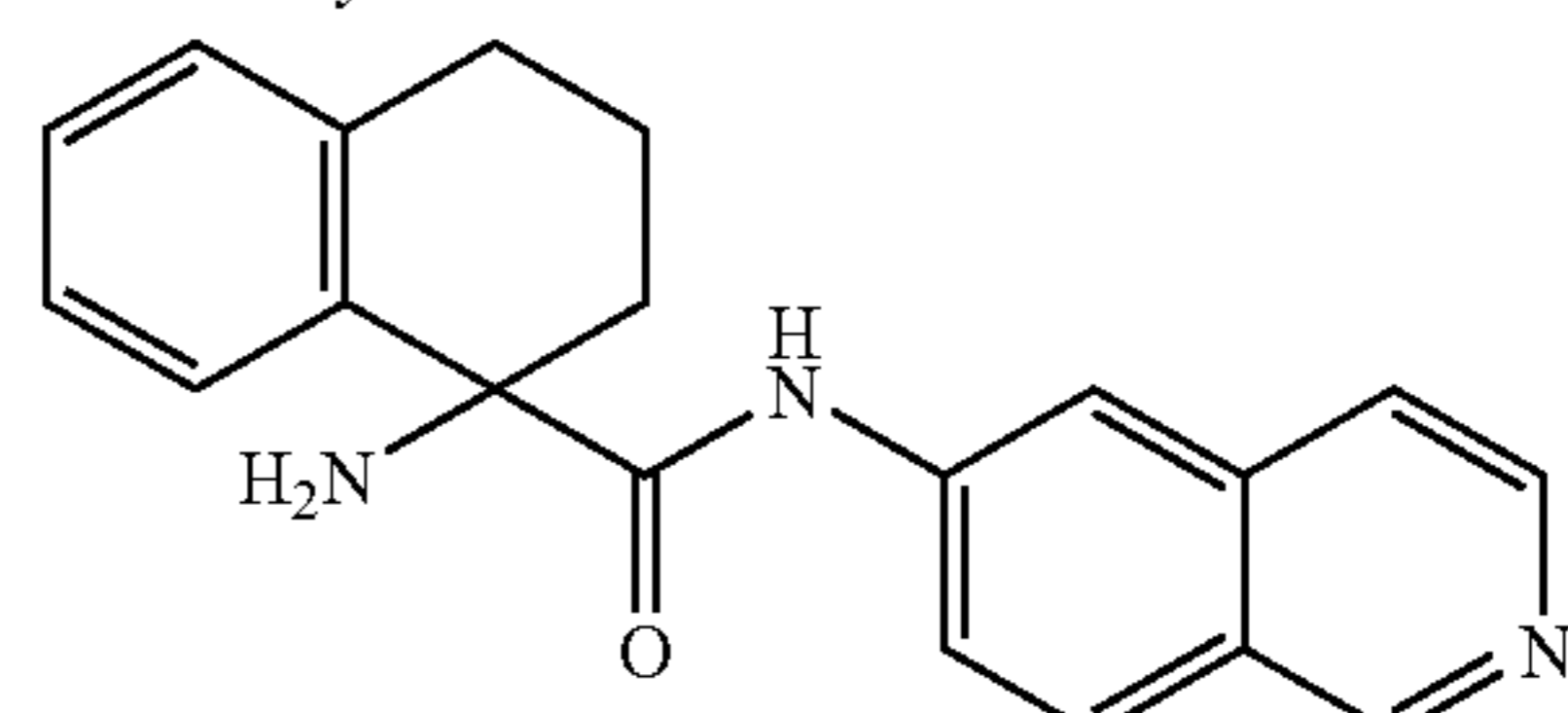
1-amino-N-(isoquinolin-6-yl)-1,2,3,4-tetrahydronaphthalene-1-carboxamide
