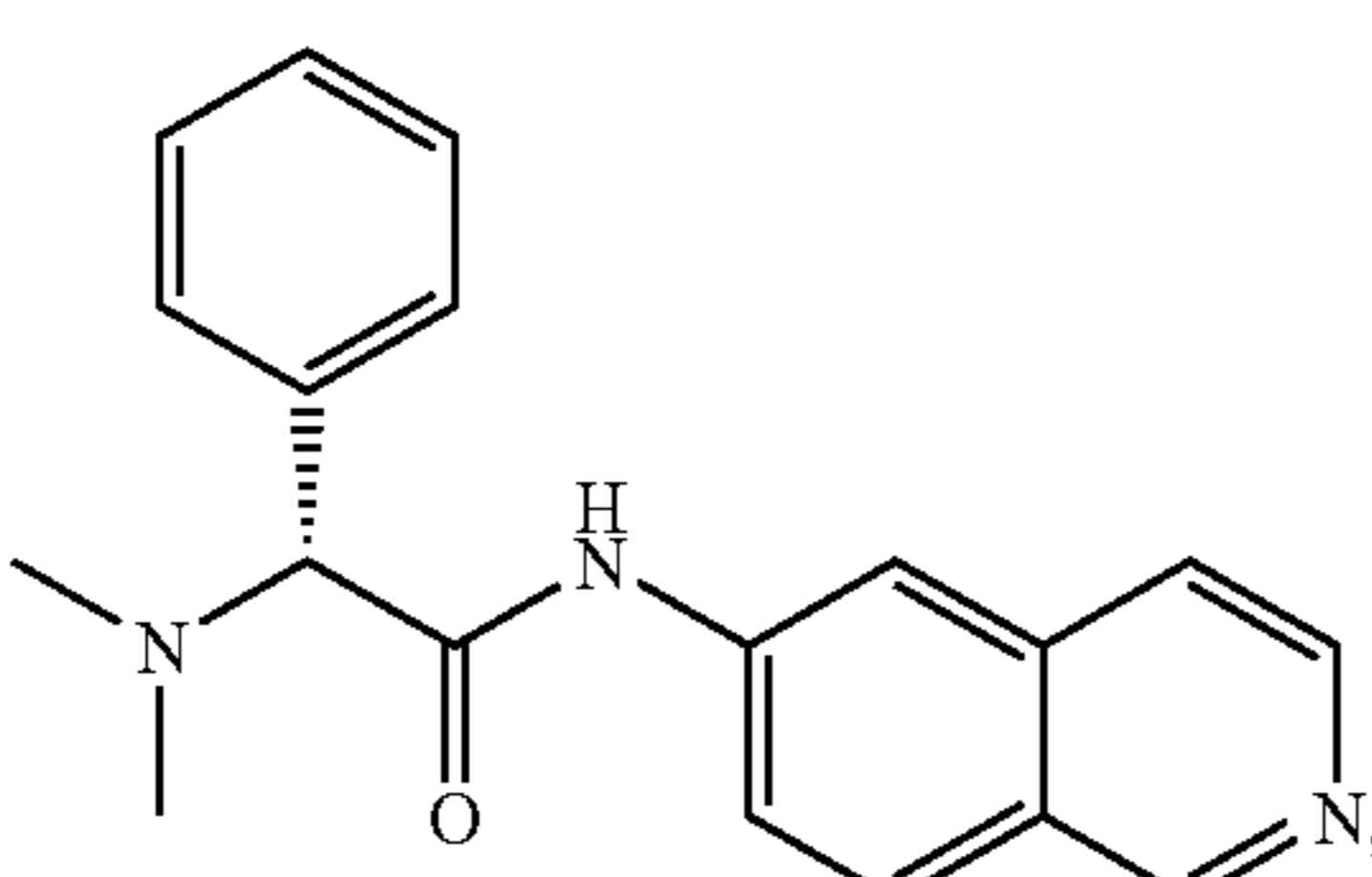
(R)-2-(dimethylamino)-N-(isoquinolin-6-yl)-2-phenylacetamide
