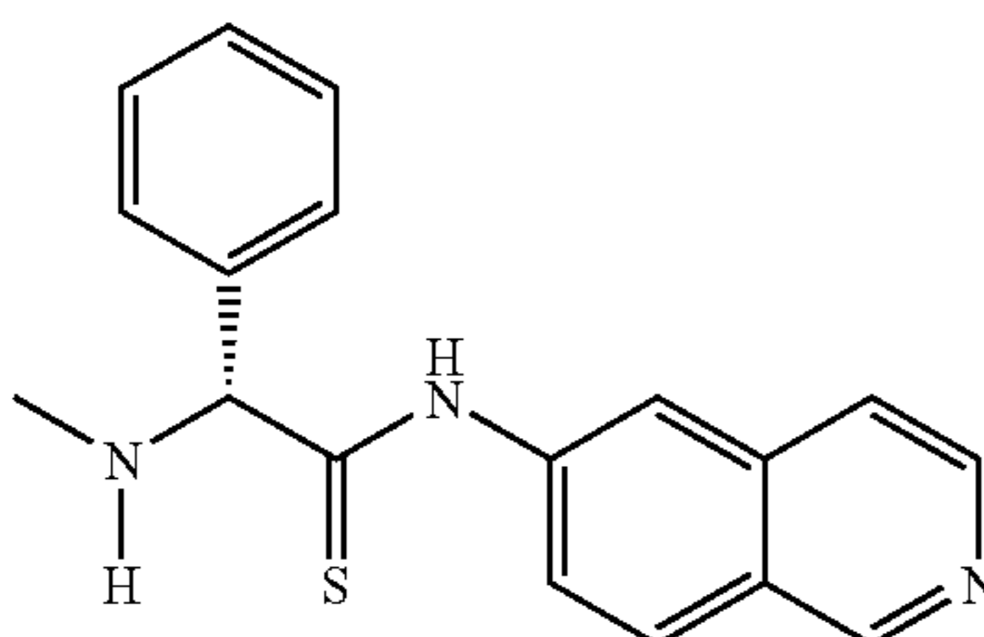
(R)-N-(isoquinolin-6-yl)-2-(methylamino)-2-phenylethanethioamide
