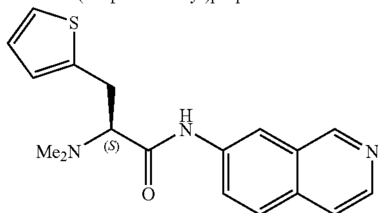
(S)-2-(dimethylamino)-N-(isoquinolin-7-yl)-3-(thiophen-2-yl)propanamide
