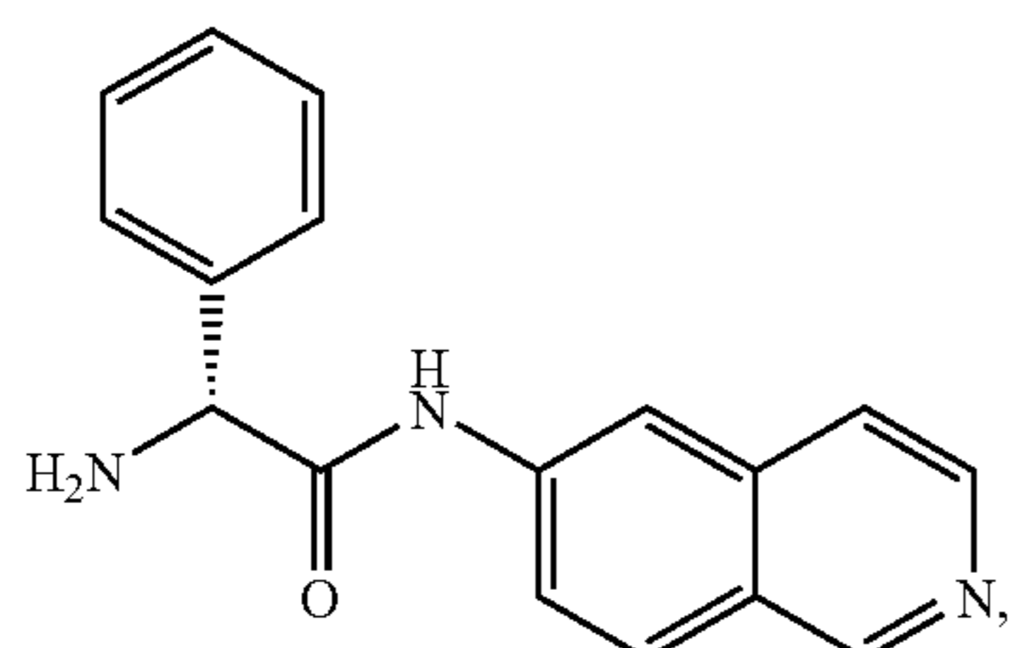
(R)-2-amino-N-(isoquinolin-6-yl)-2-phenylacetamide
