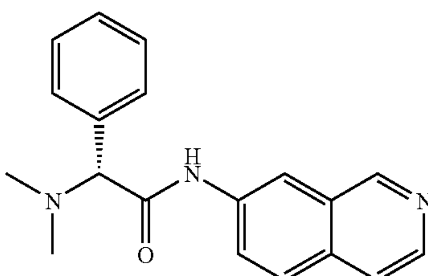
(R)-2-(dimethylamino)-N-(isoquinolin-7-yl)-2-phenylacetamide
