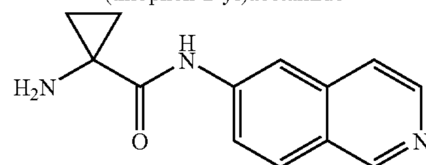
1-amino-N-(isoquinolin-6-yl)cyclopropanecarboxamide
