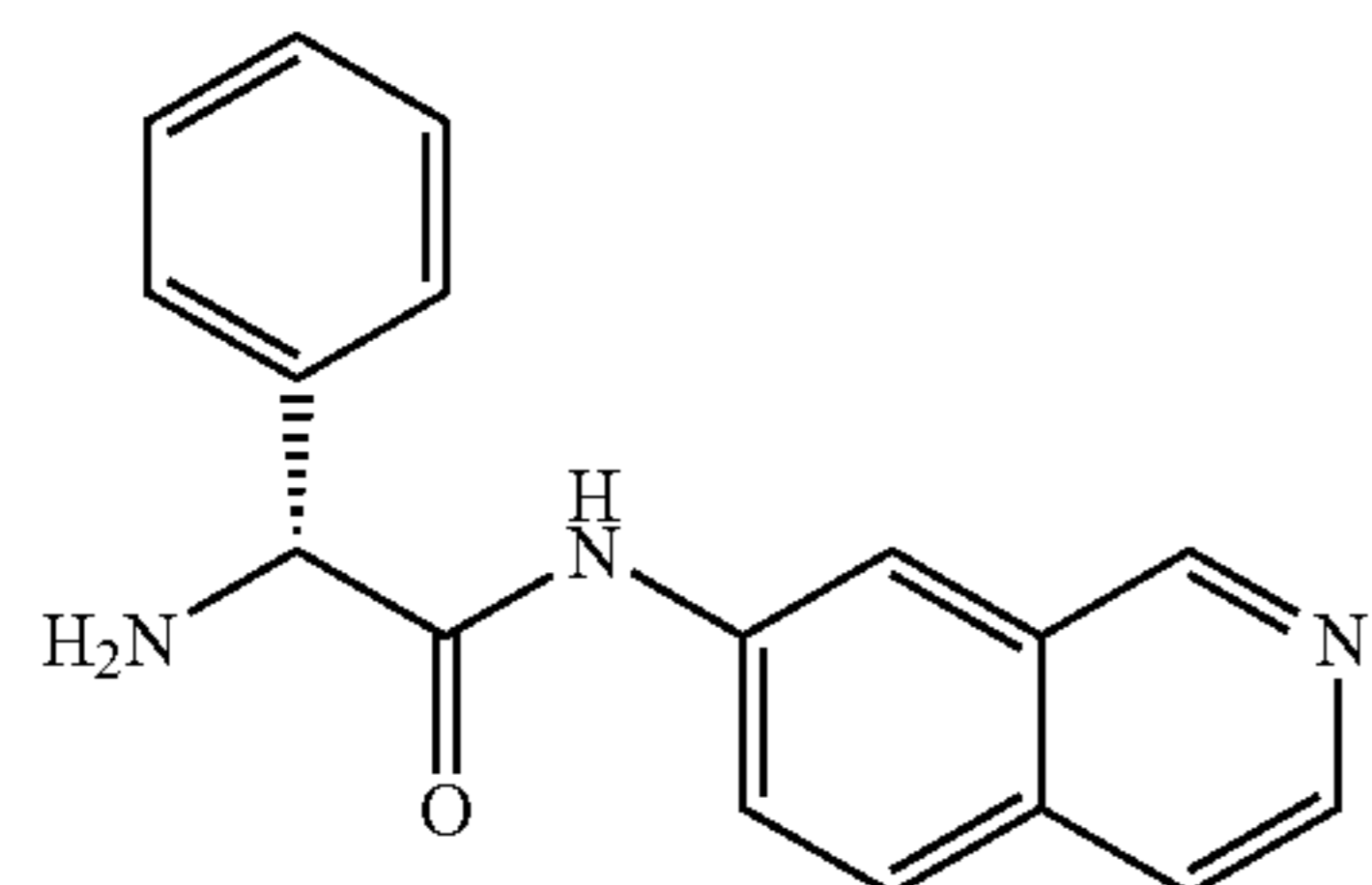
(R)-2-amino-N-(isoquinolin-7-yl)-2-phenylacetamide
