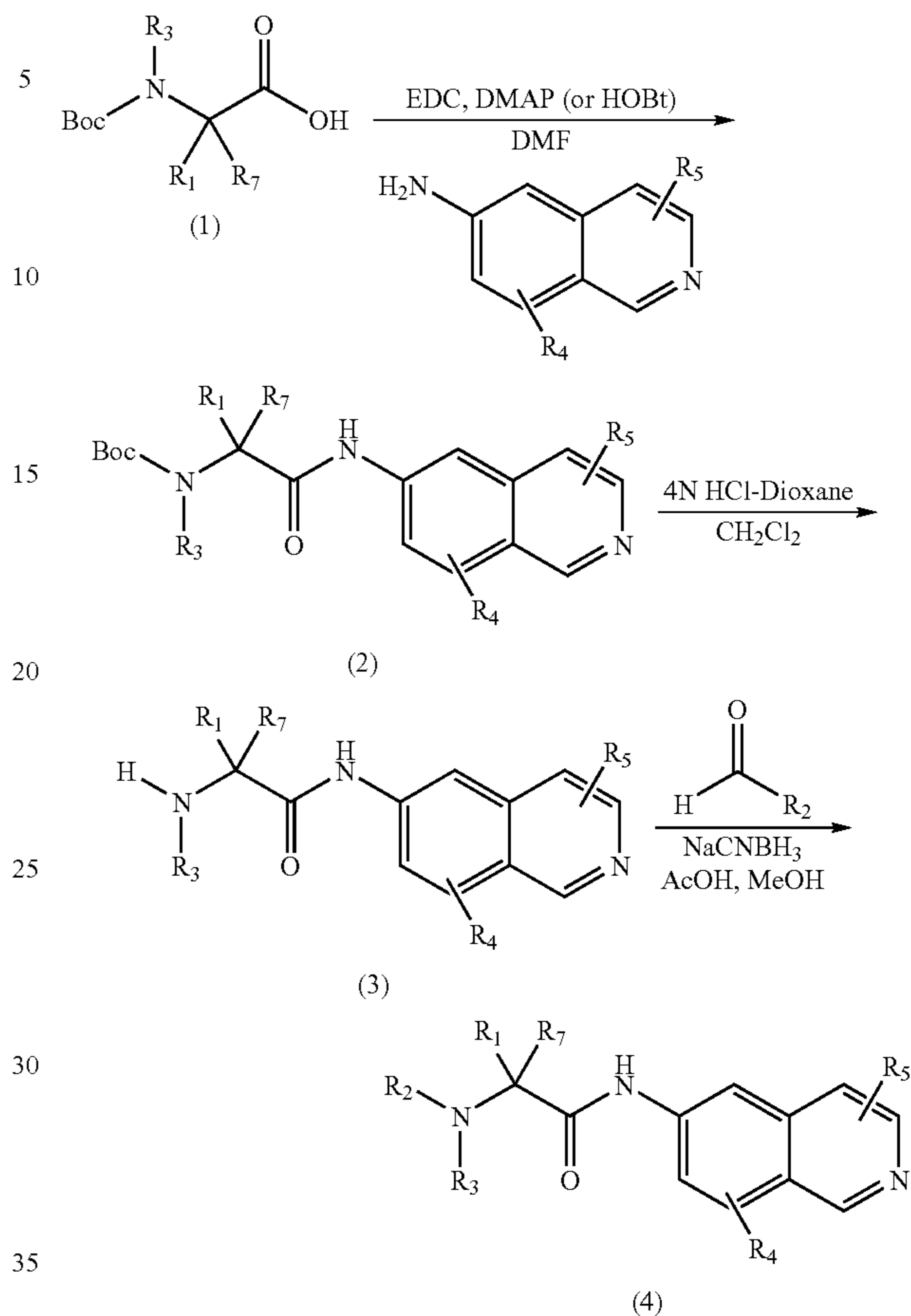
Scheme One
