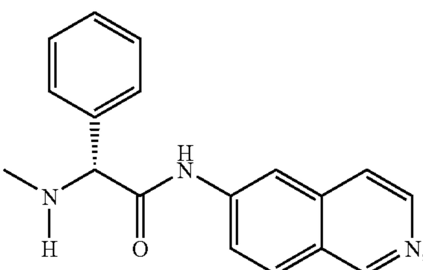
(R)-N-(isoquinolin-6-yl)-2-(methylamino)-2-phenylacetamide
