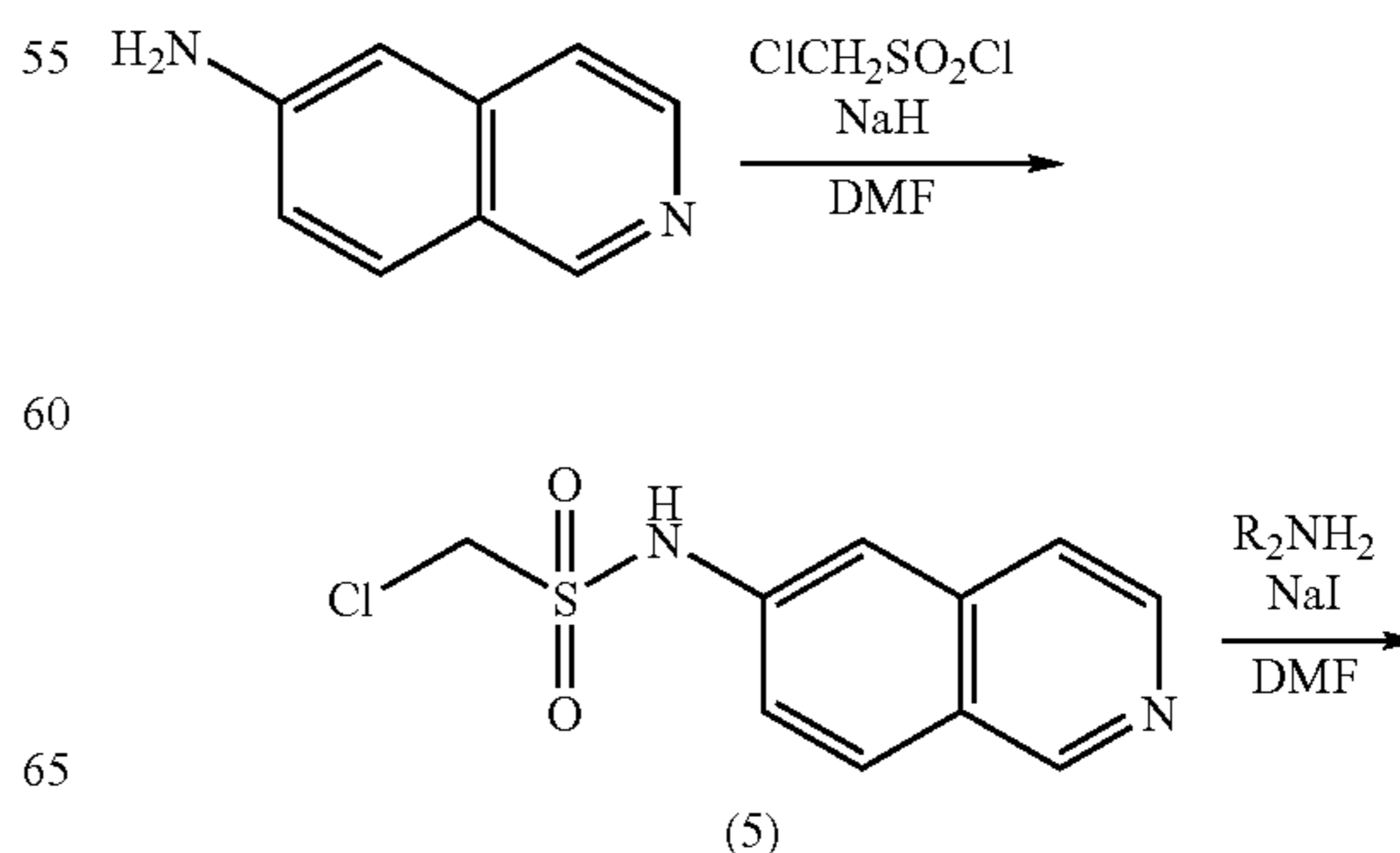
Scheme Two
