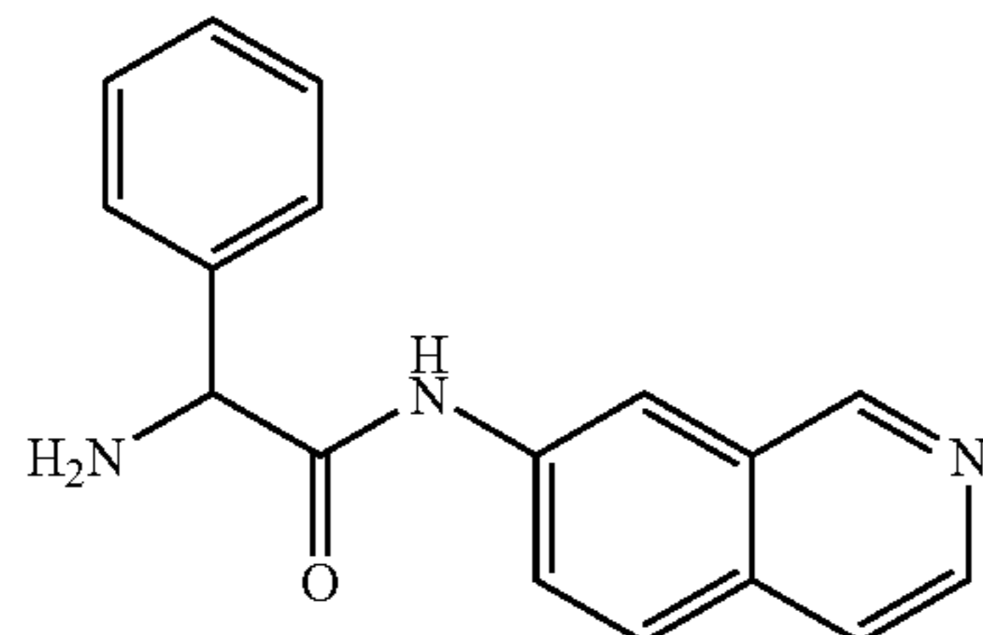
2-amino-N-(isoquinolin-7-yl)-2-phenylacetamide
