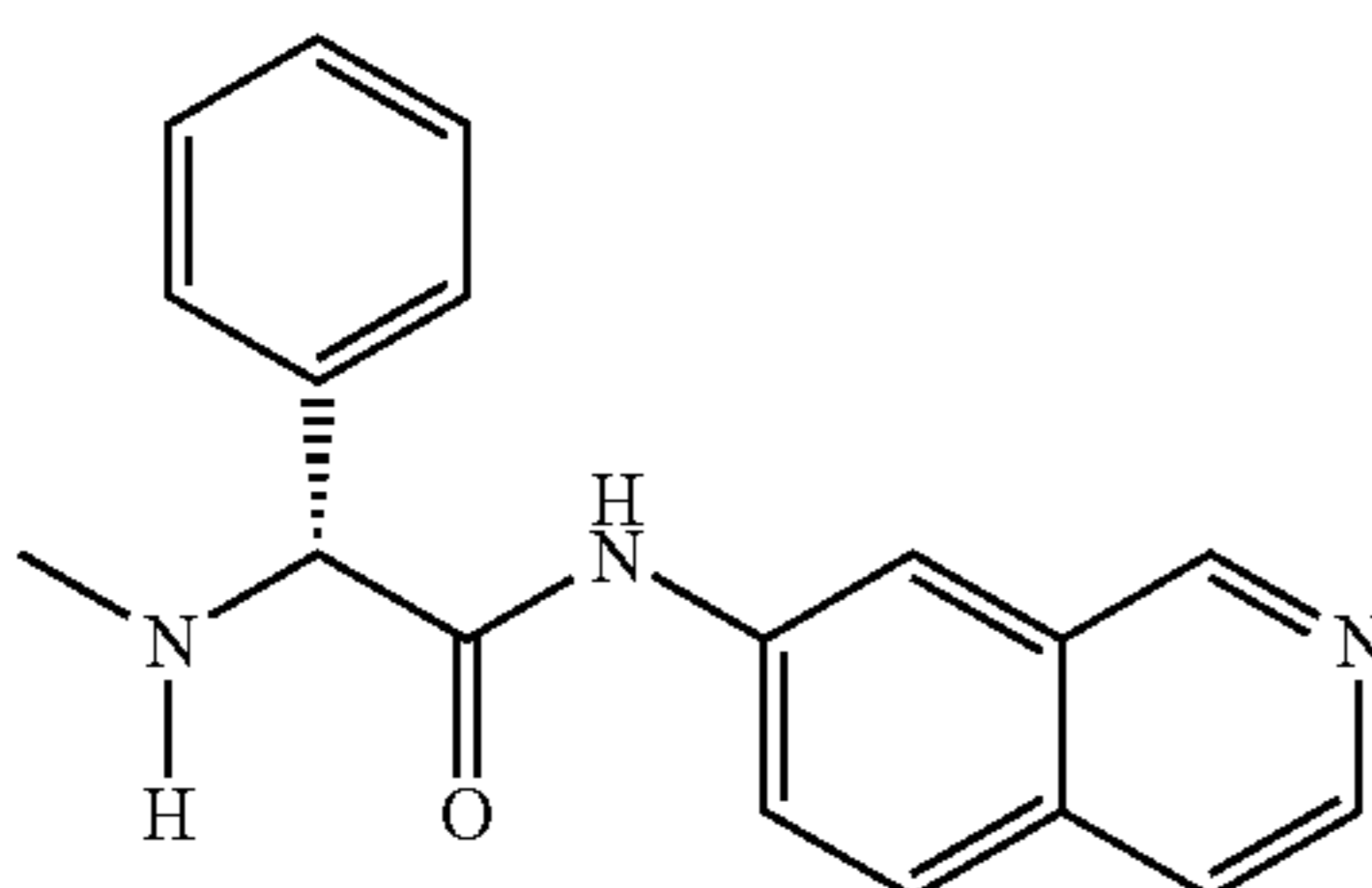
(R)-N-(isoquinolin-7-yl)-2-(methylamino)-2-phenylacetamide
