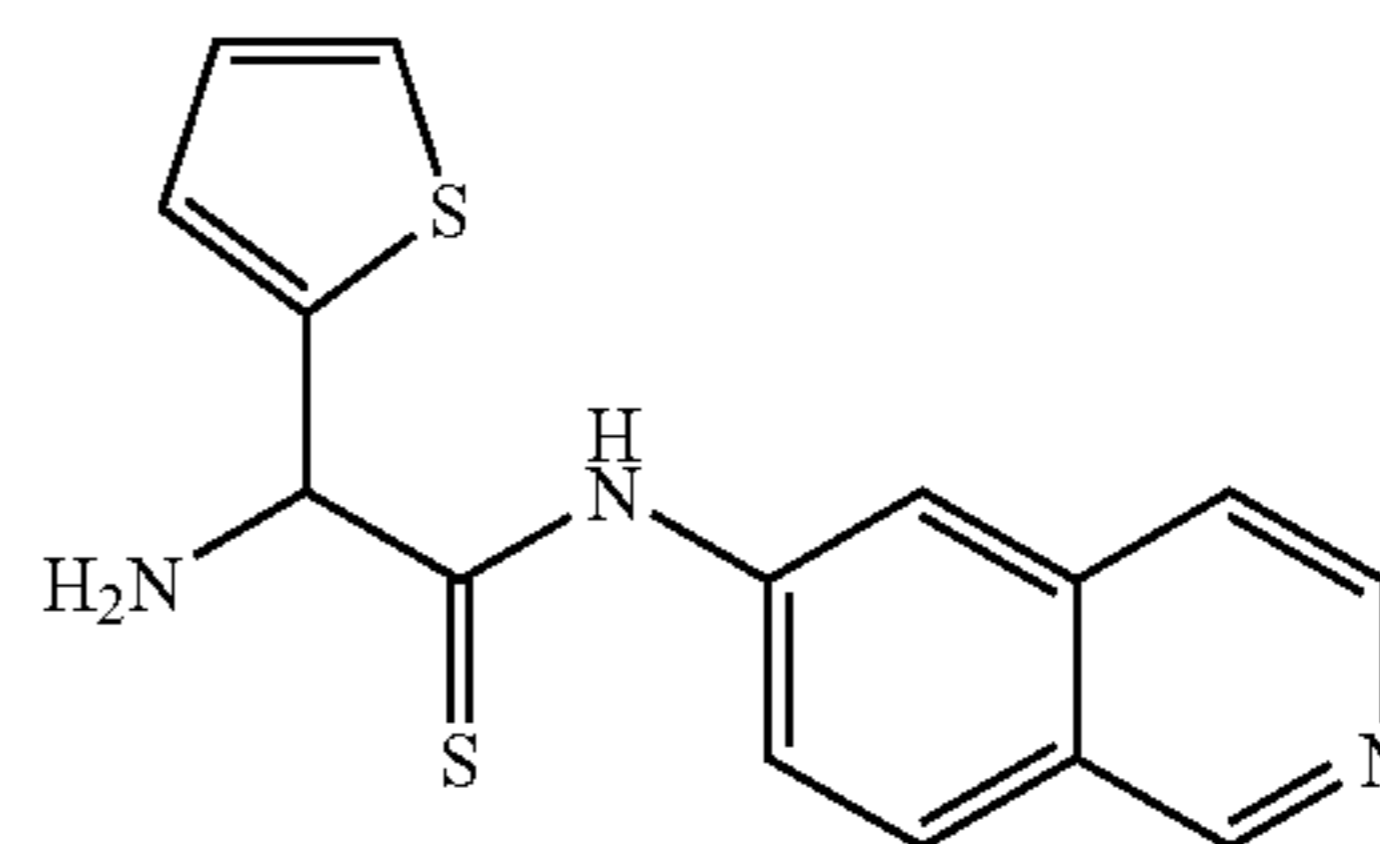
2-amino-N-(isoquinolin-6-yl)-2-(thiophen-2-yl)ethanethioamide
