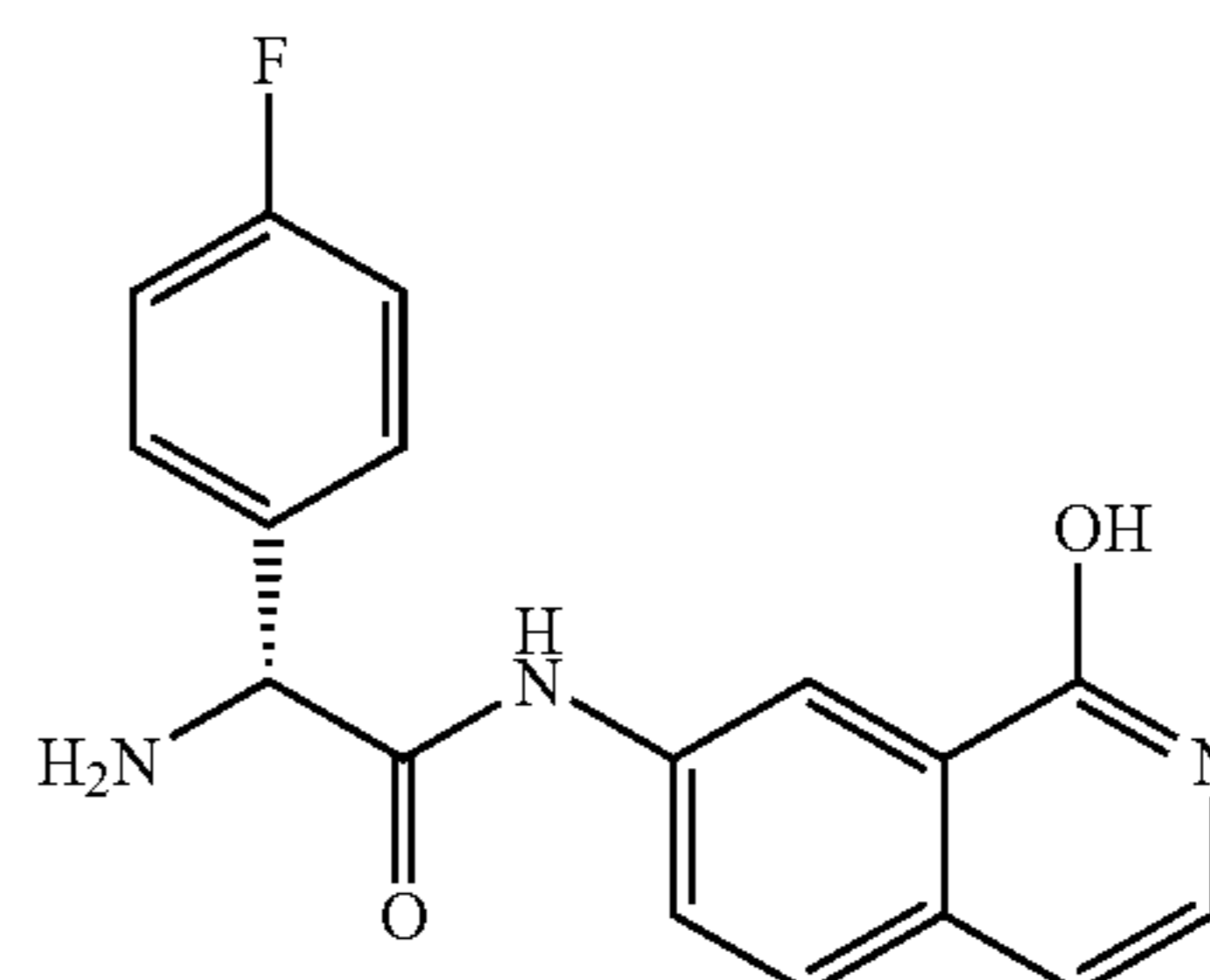
(R)-2-amino-2-(4-fluorophenyl)-N-(1-hydroxyisoquinolin-7-yl)acetamide
