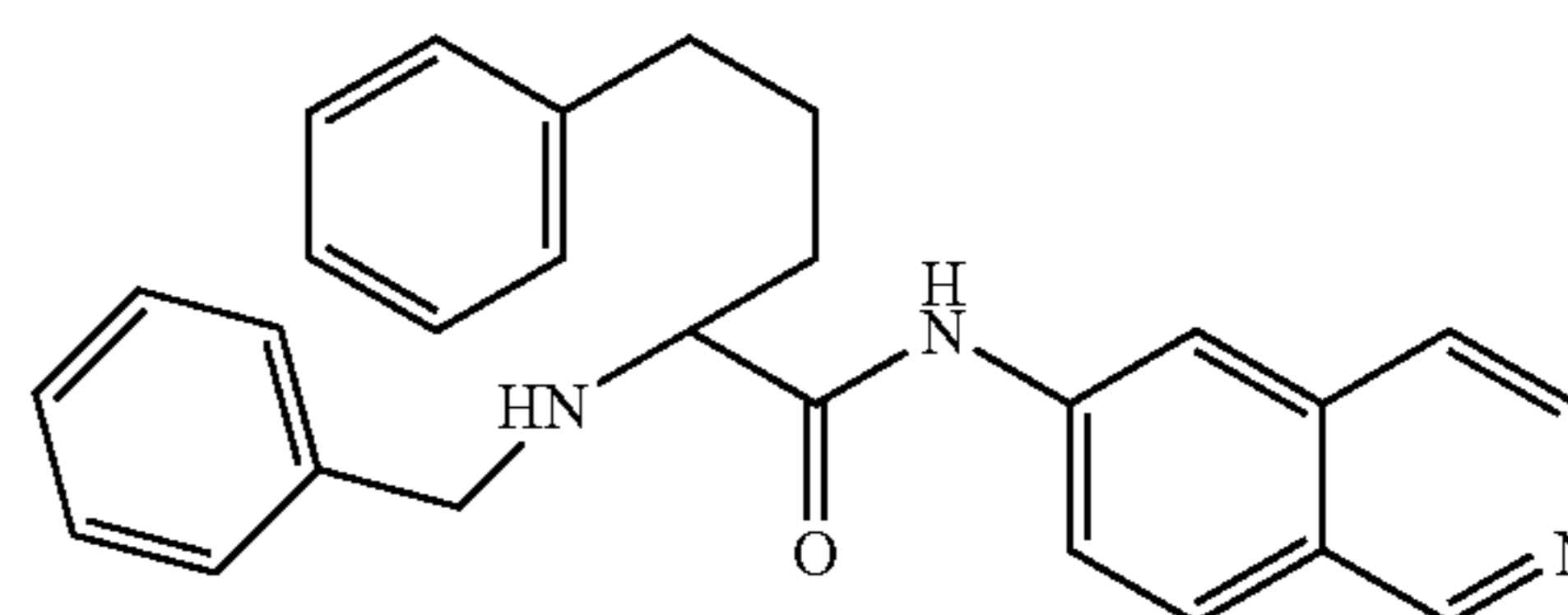
2-(benzylamino)-N-(isoquinolin-7-yl)-5-phenylpentanamide
