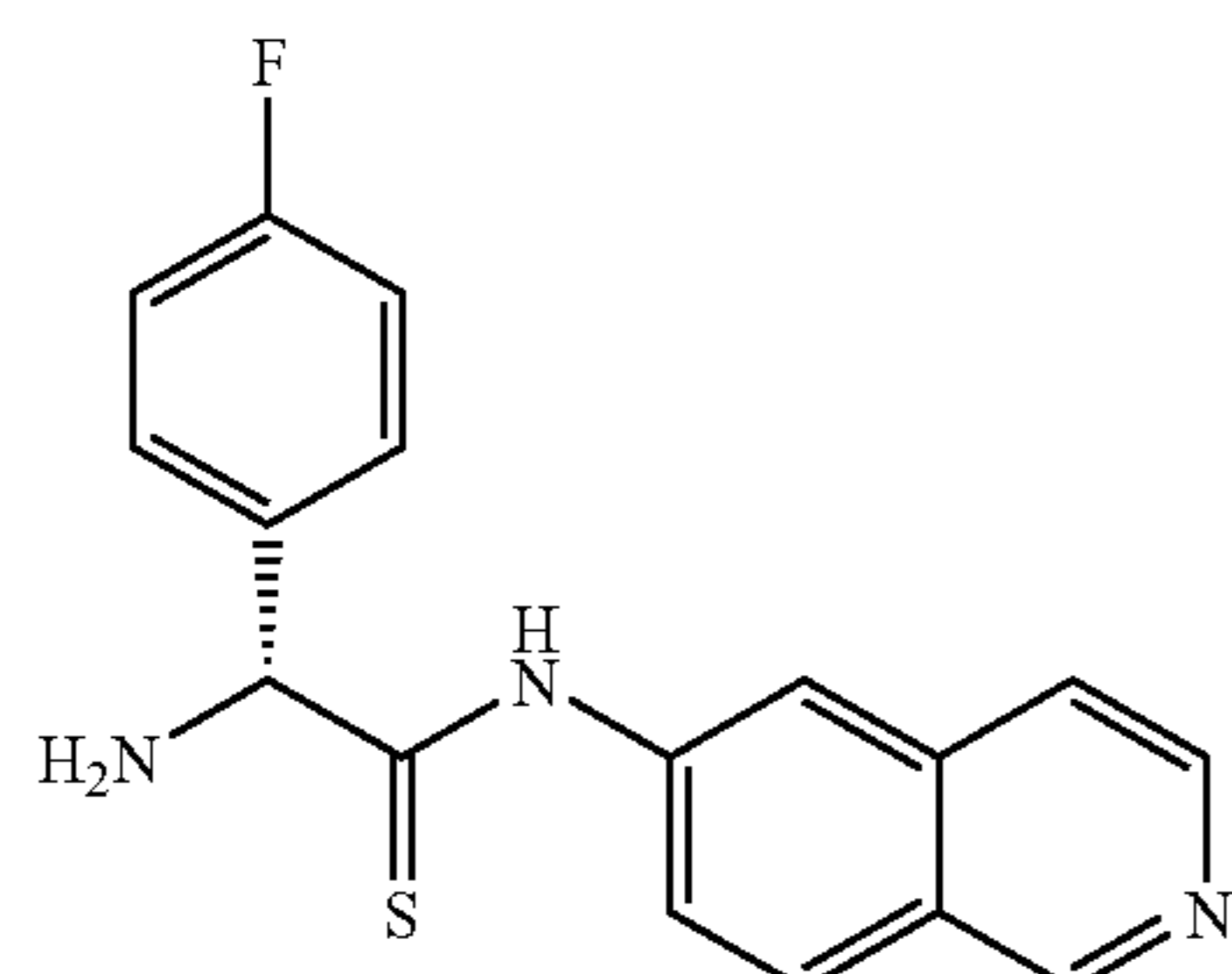
(R)-2-amino-2-(4-fluorophenyl)-N-(isoquinolin-6-yl)ethanethioamide
