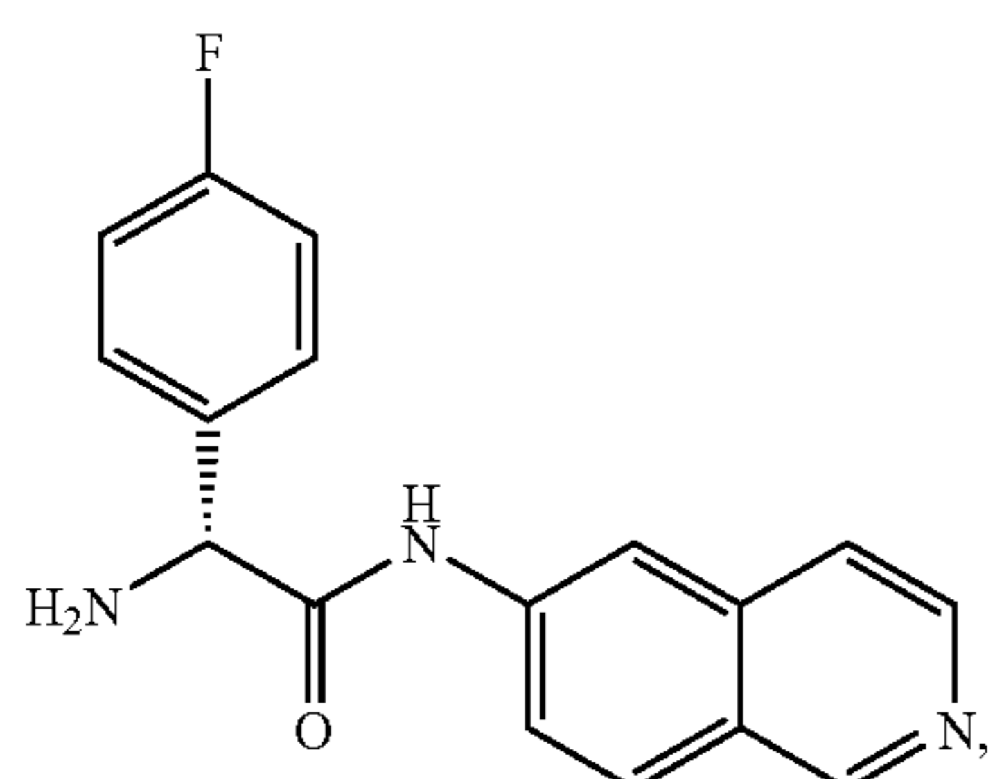
(R)-2-amino-2-(4-fluorophenyl)-N-(isoquinolin-6-yl)acetamide
