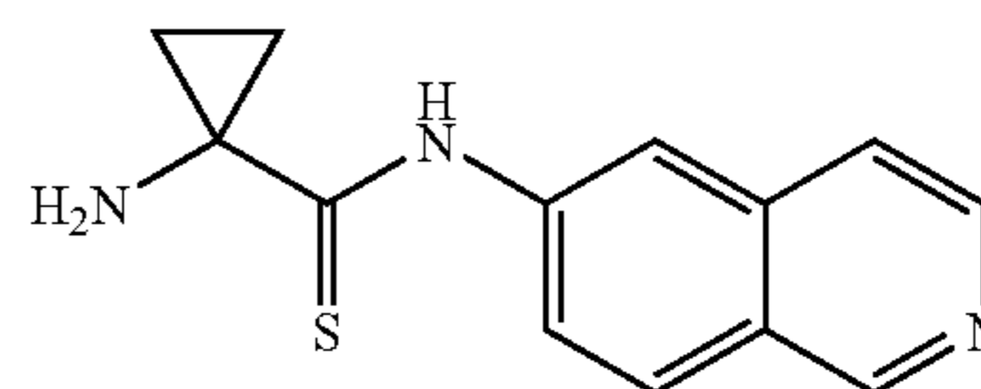
1-amino-N-(isoquinolin-6-yl)cyclopropanecarbothioamide
