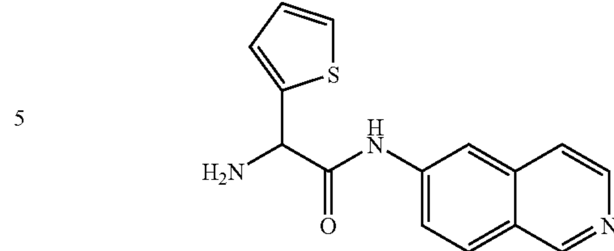
2-amino-N-(isoquinolin-6-yl)-2-(thiophen-2-yl)acetamide
