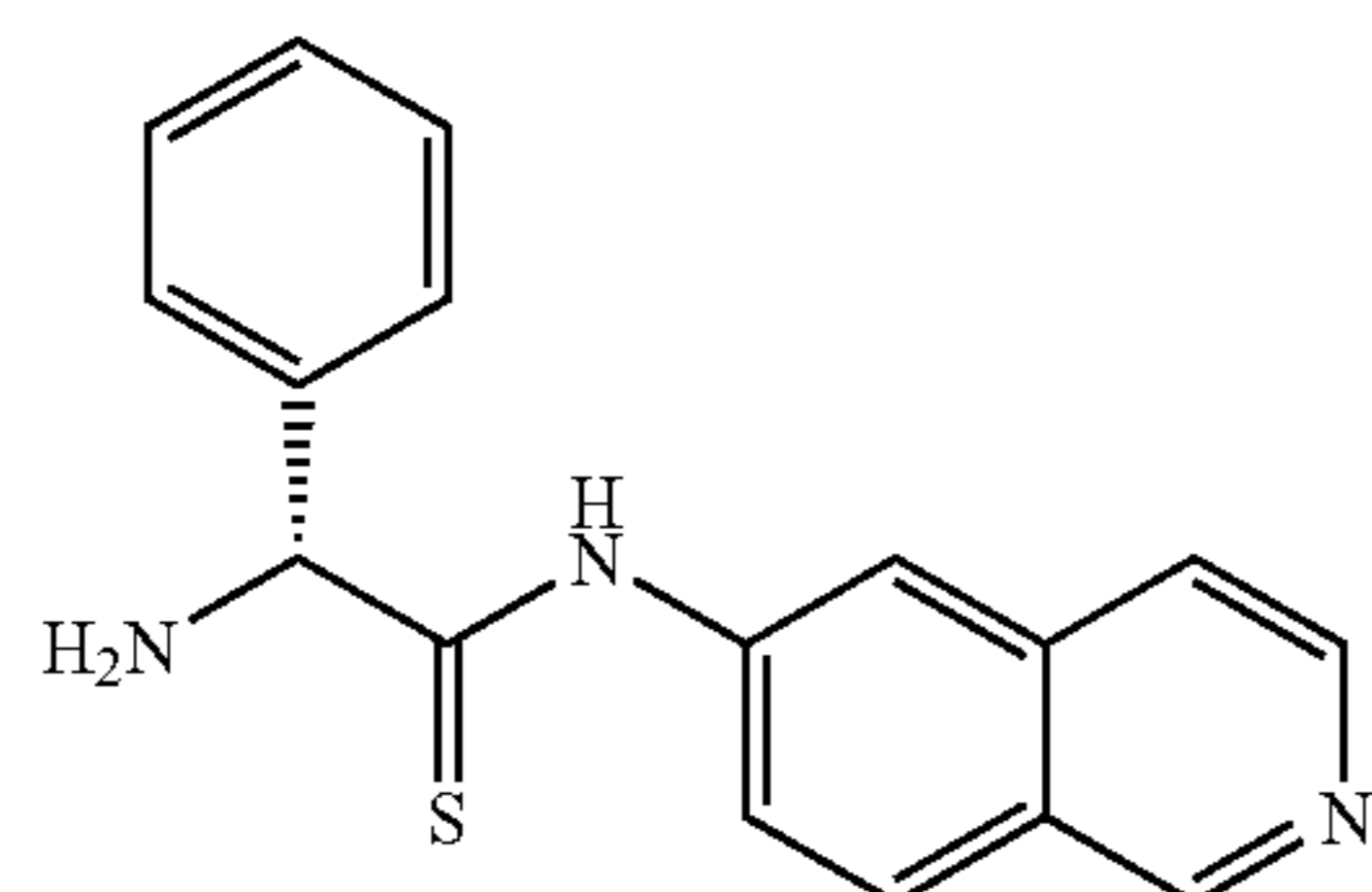
(R)-2-amino-N-(isoquinolin-6-yl)-2-phenylethanethioamide
