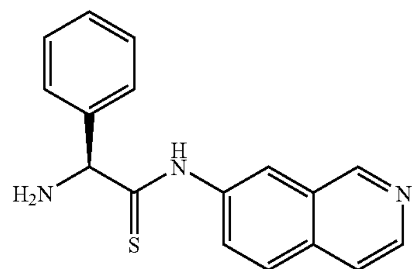
(S)-2-amino-N-(isoquinolin-7-yl)-2-phenylethanethioamide
