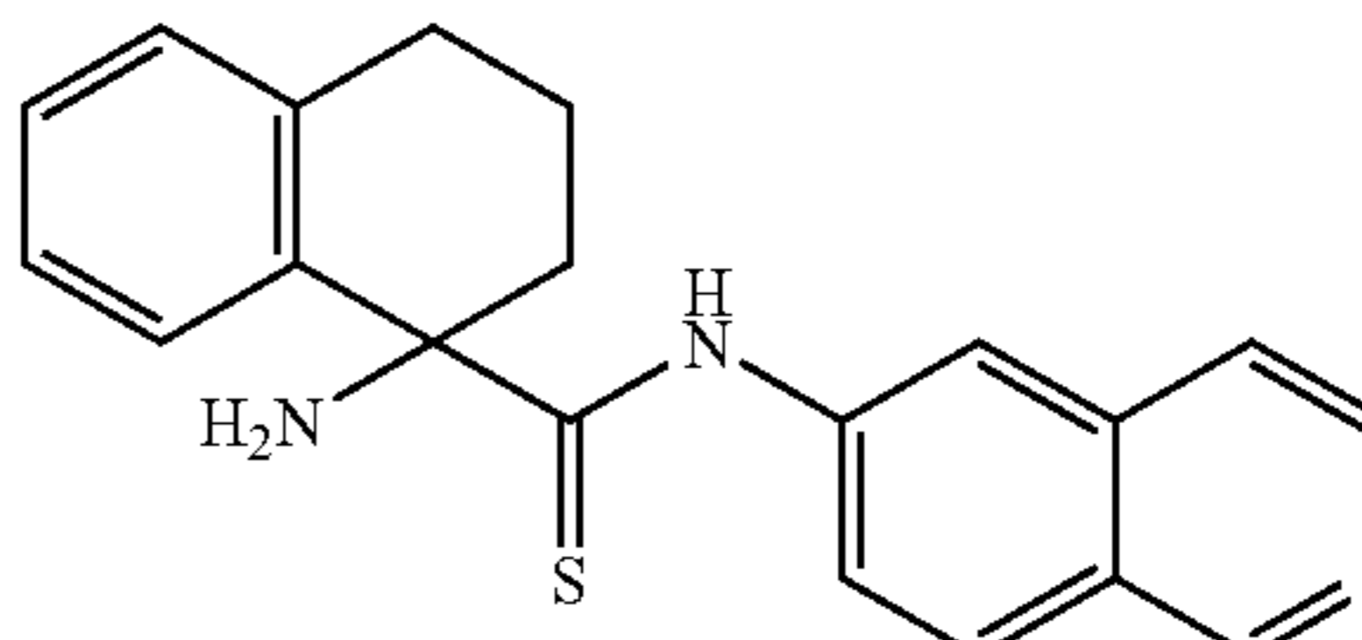
1-amino-N-(isoquinolin-6-yl)-1,2,3,4-tetrahydronaphthalene-1-carbothioamide
