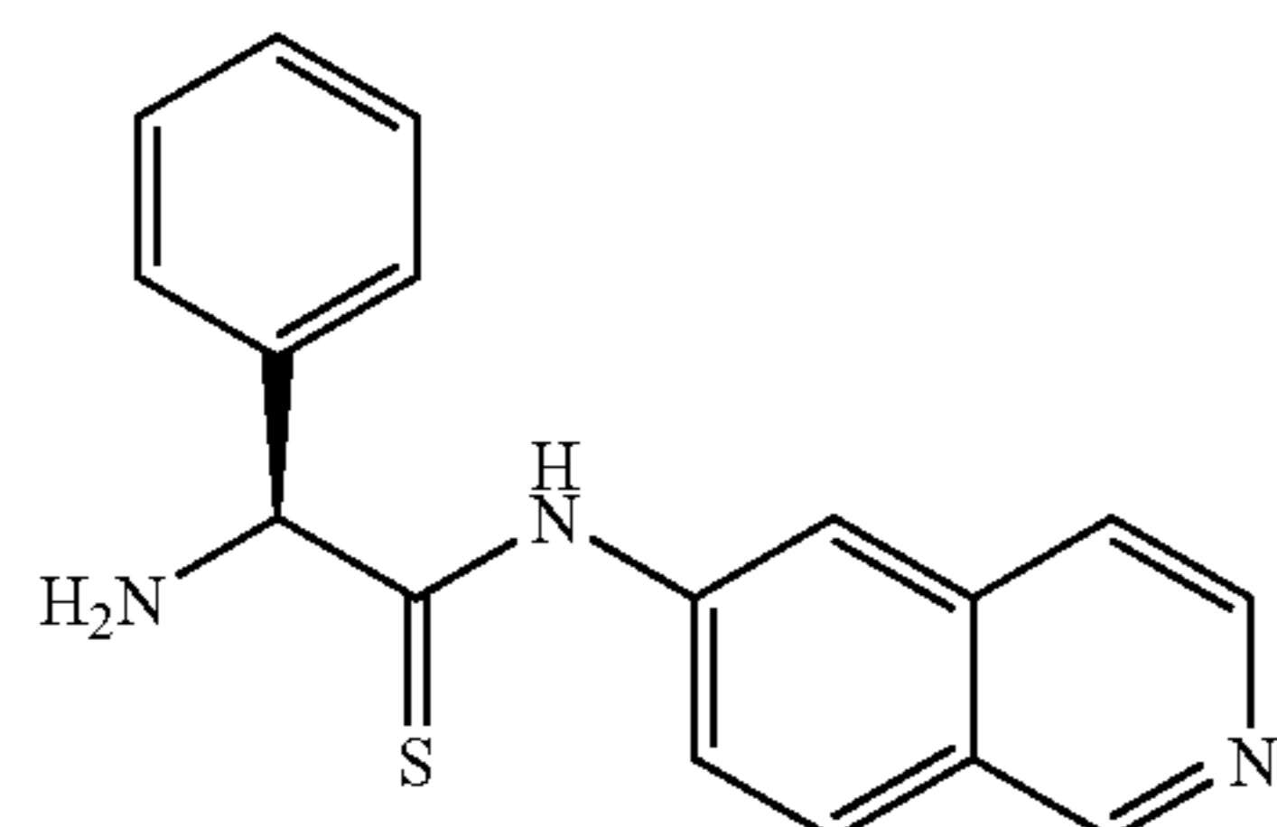
(S)-2-amino-N-(isoquinolin-6-yl)-2-phenylethanethioamide
