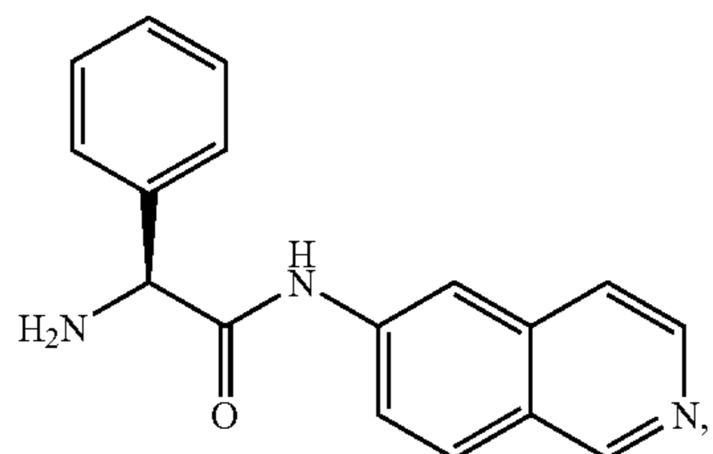
(S)-2-amino-N-(isoquinolin-6-yl)-2-phenylacetamide
