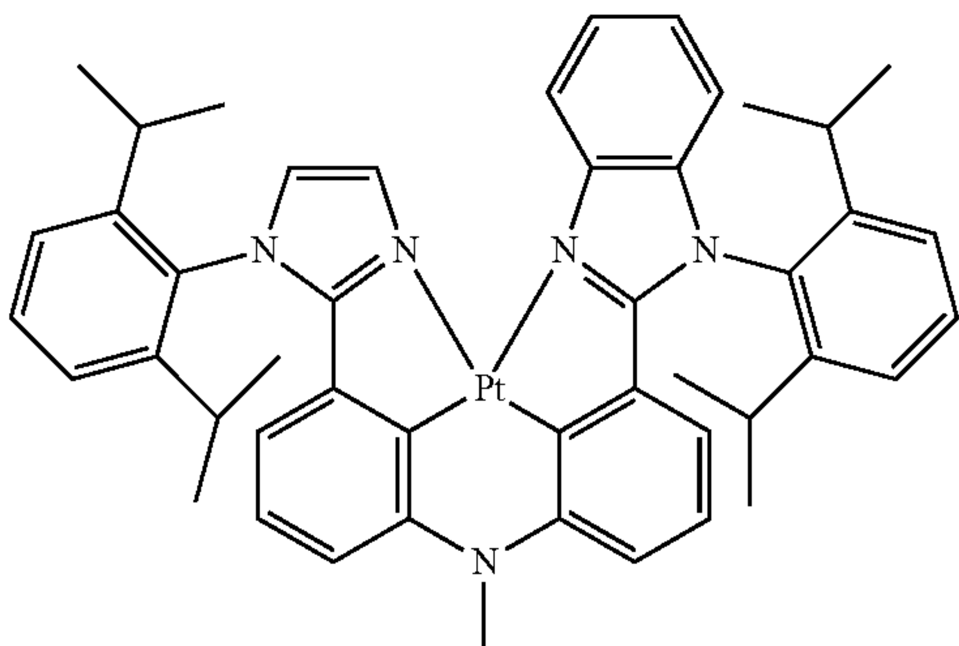
Compound 22
