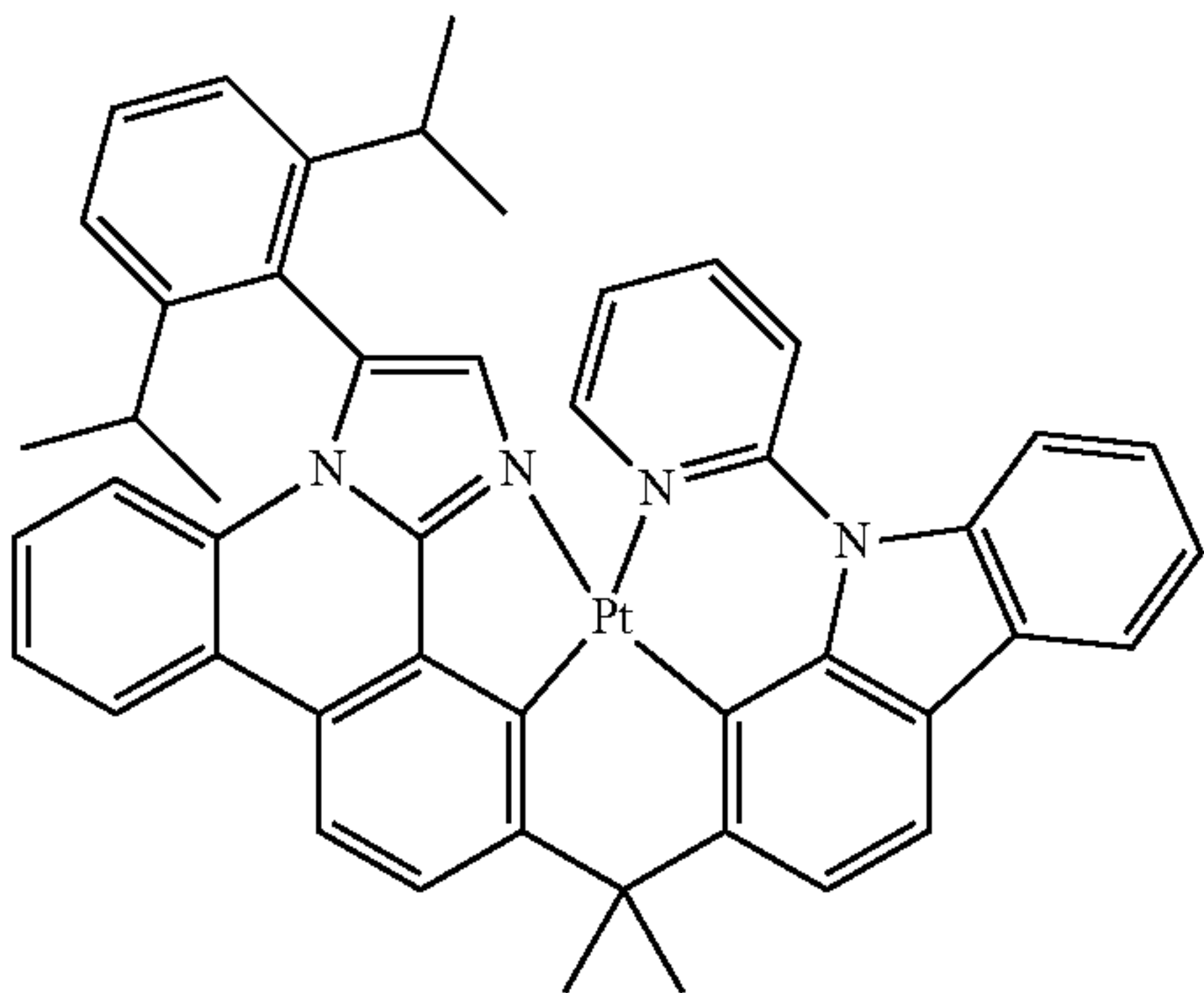
Compound 45'
