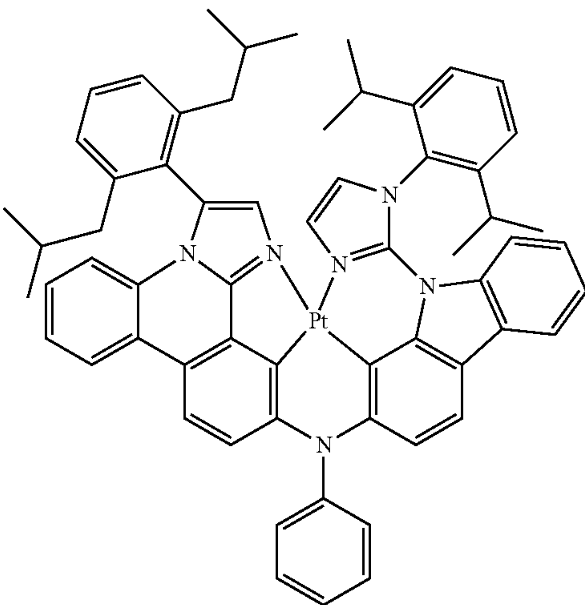
Compound 144'
