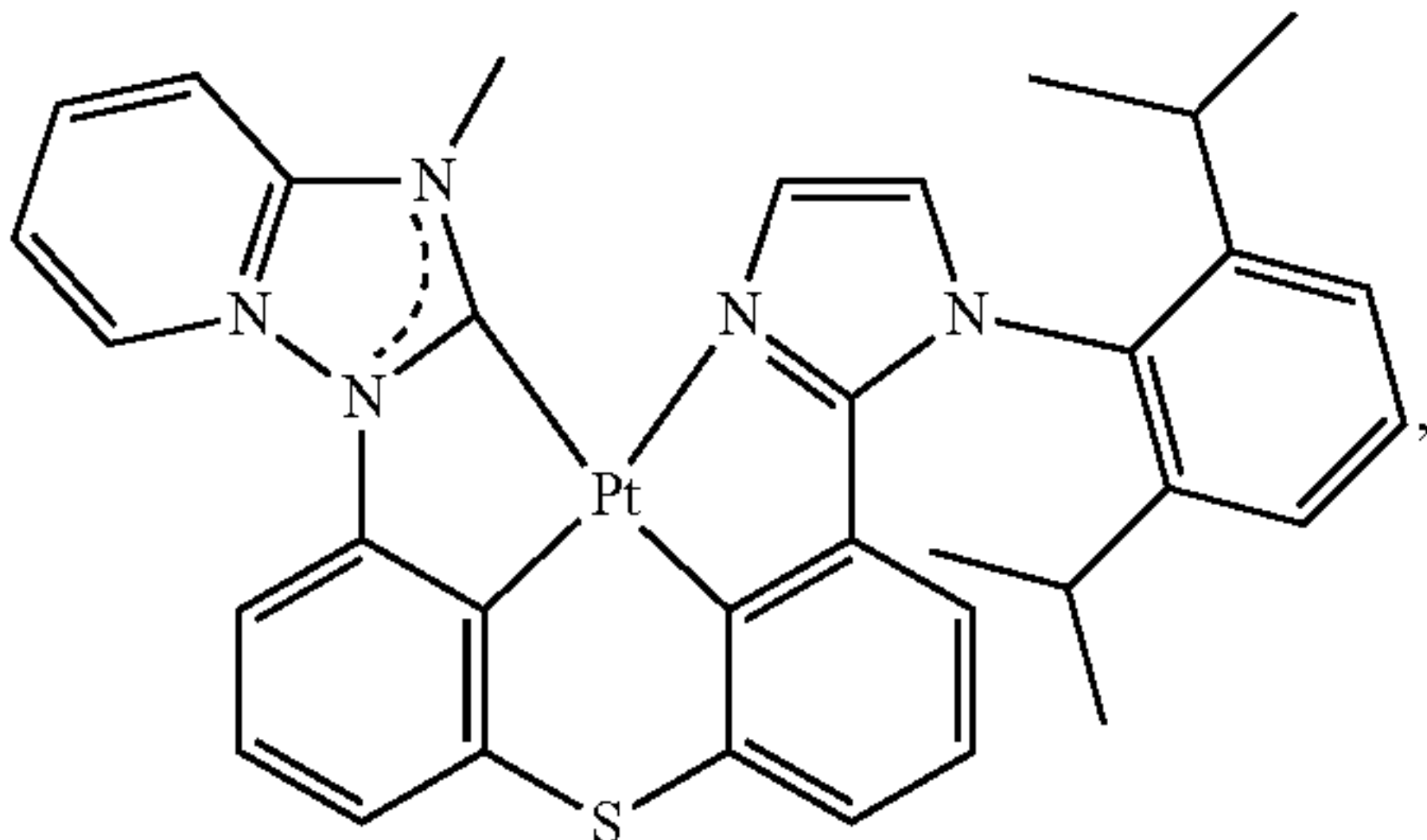
Compound 143
