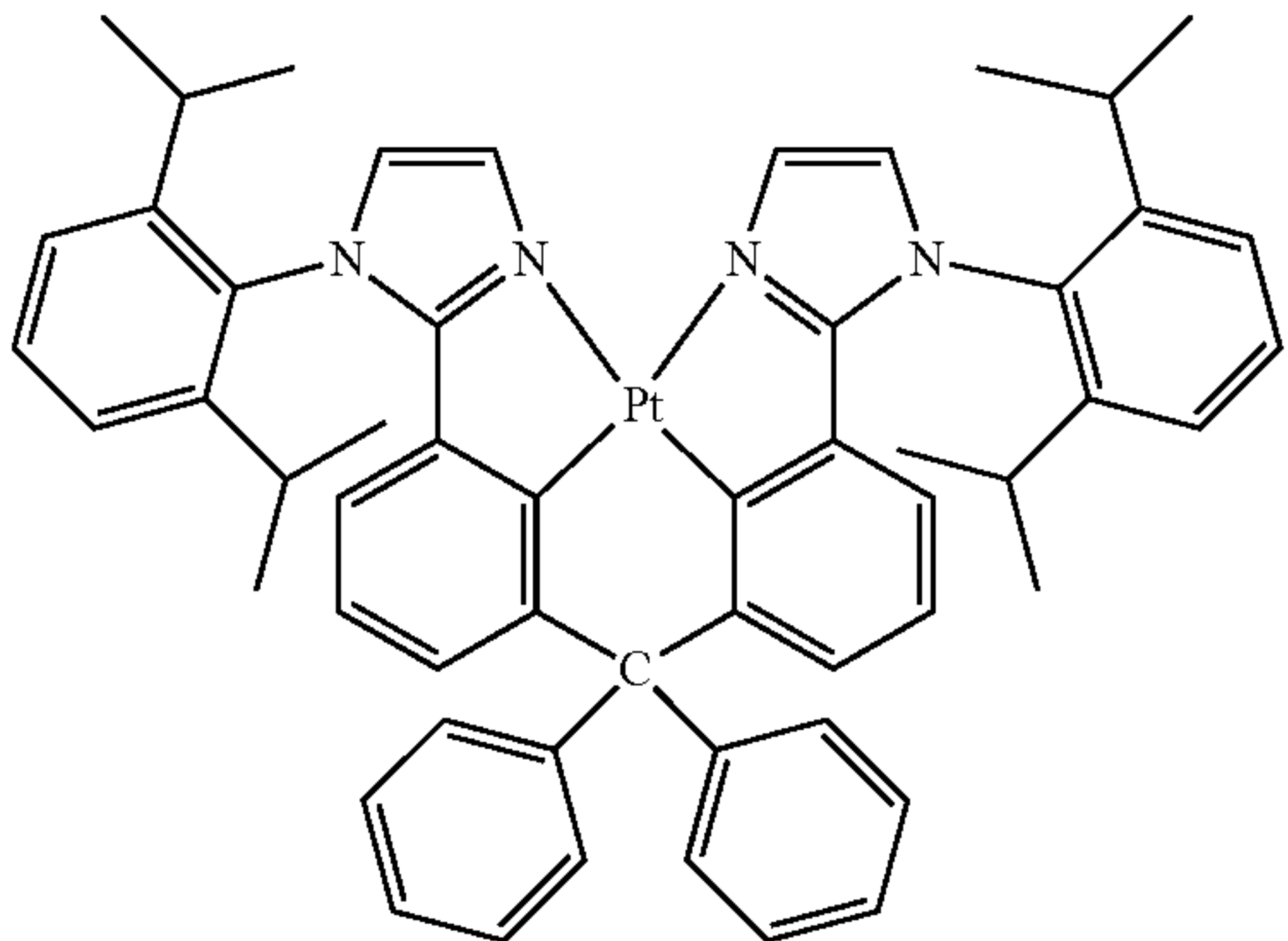
Compound 8
