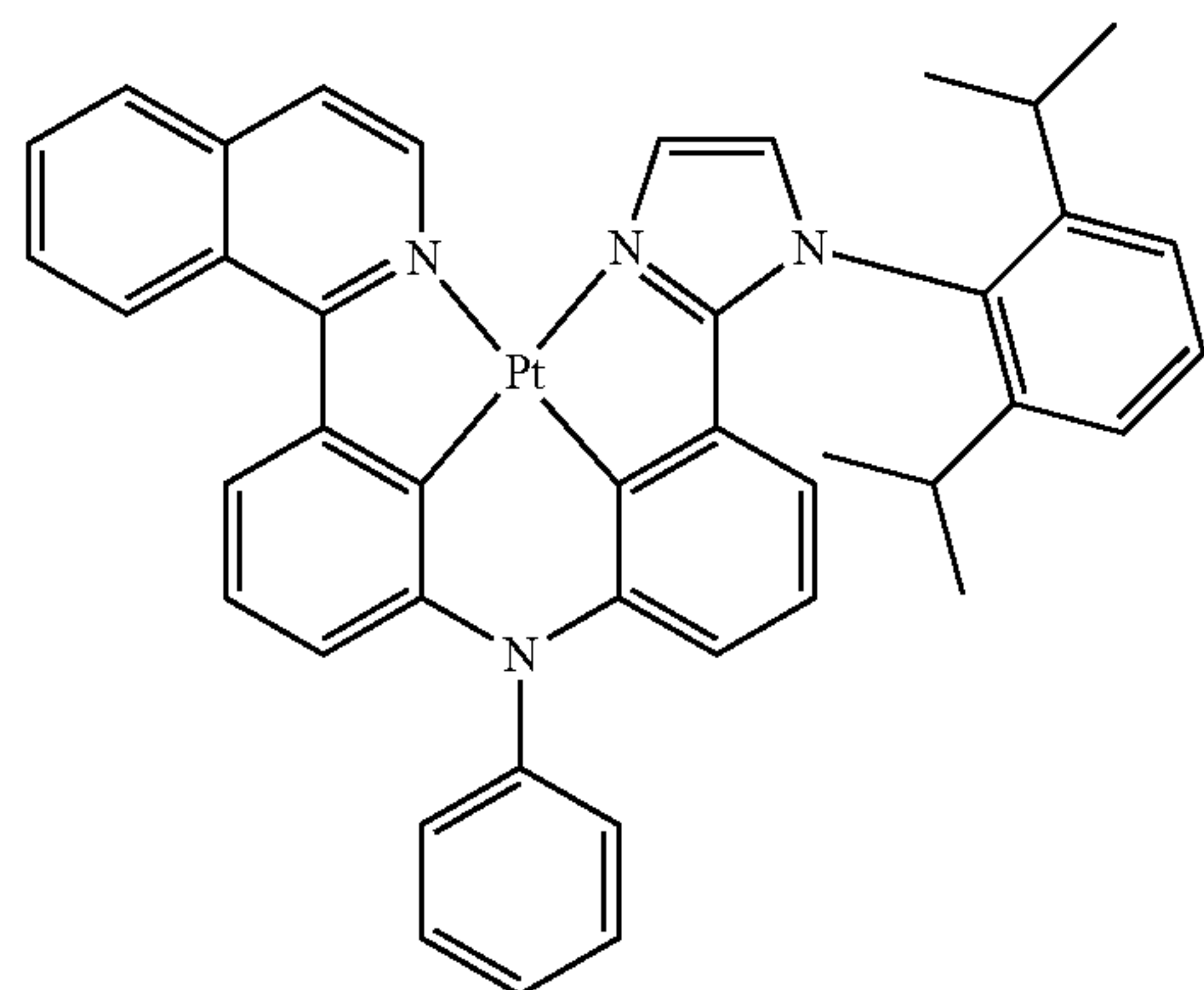
Compound 36
