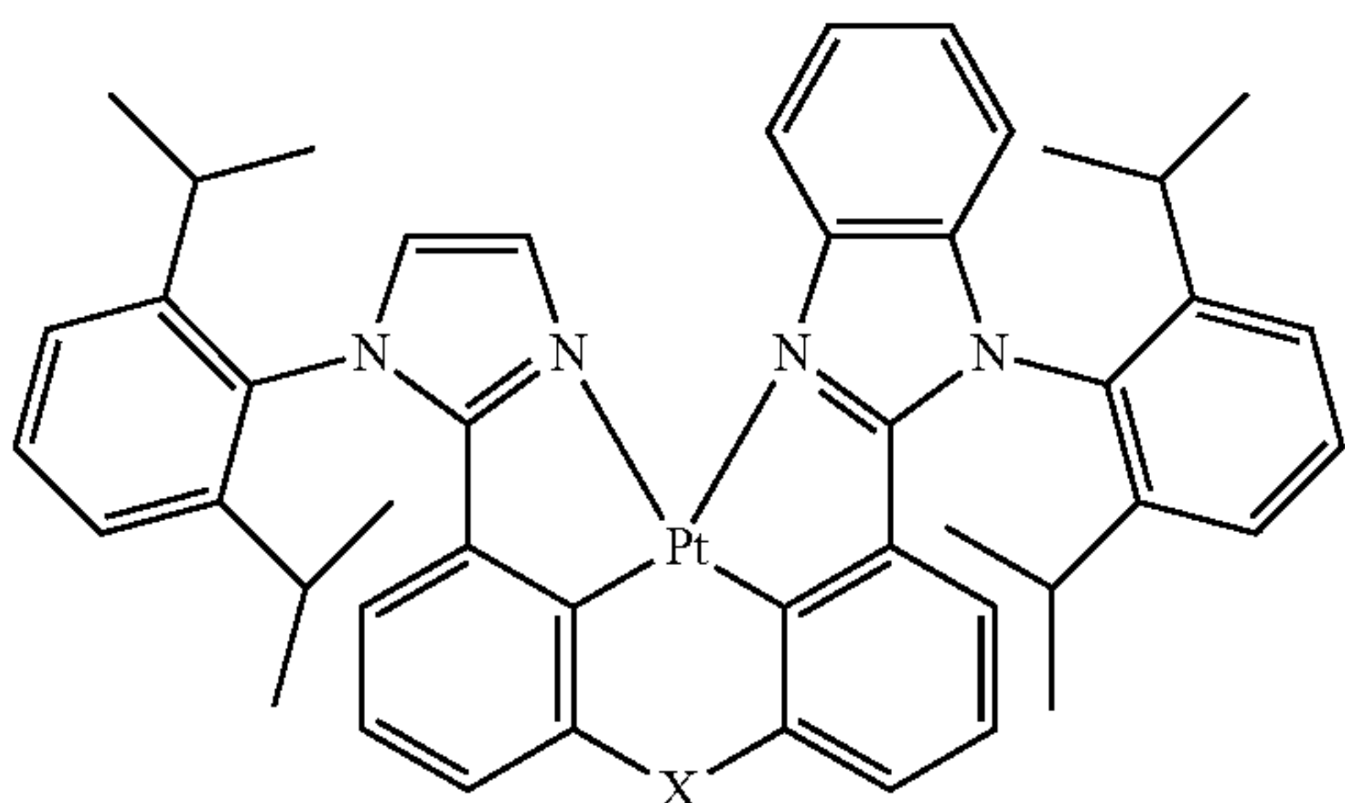
Compound 8G
