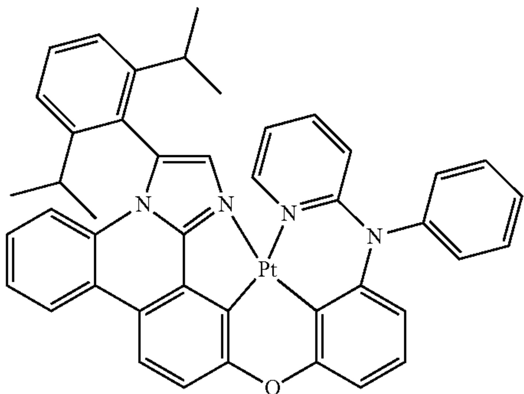
Compound 48'
