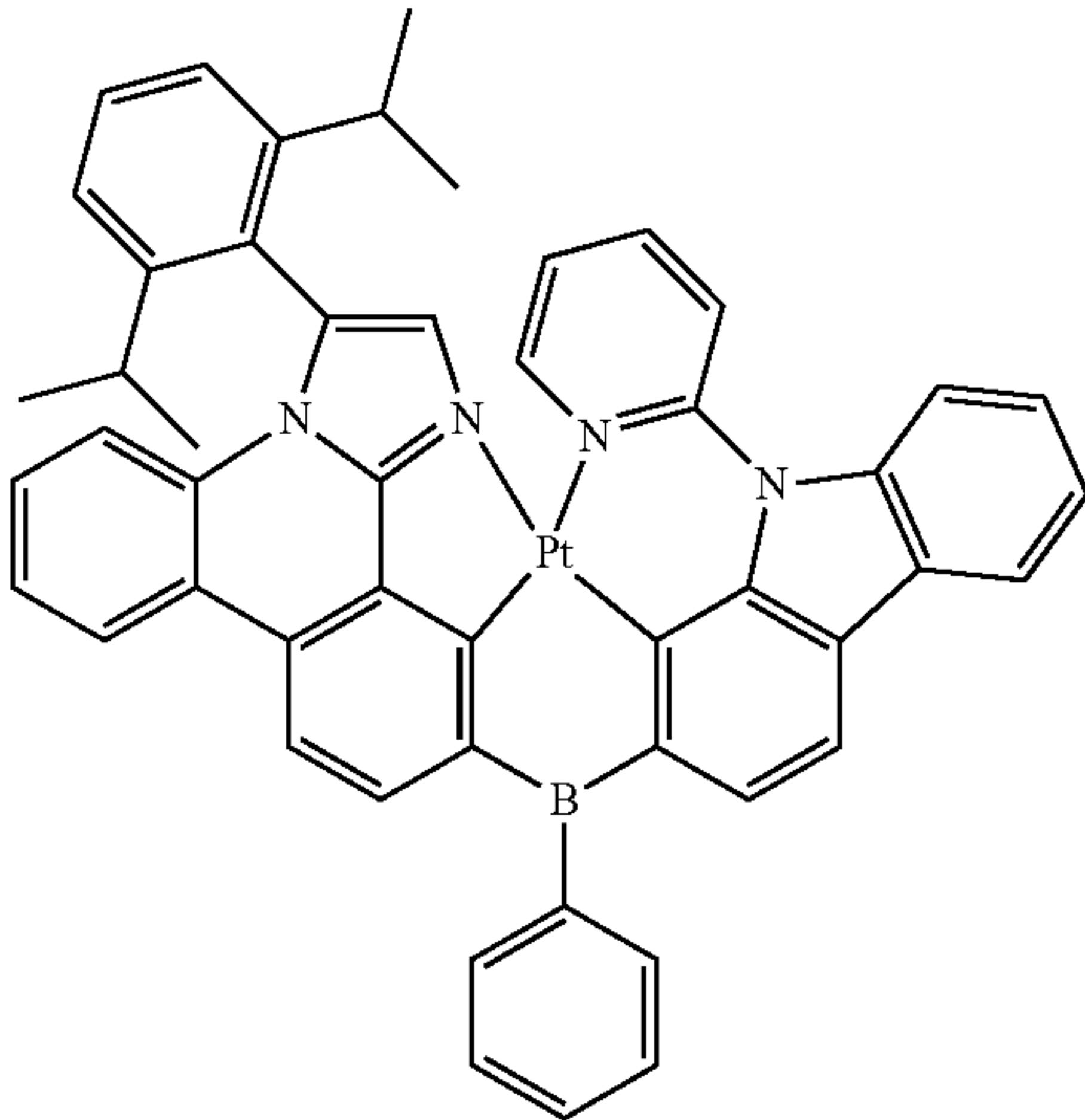
Compound 36'
