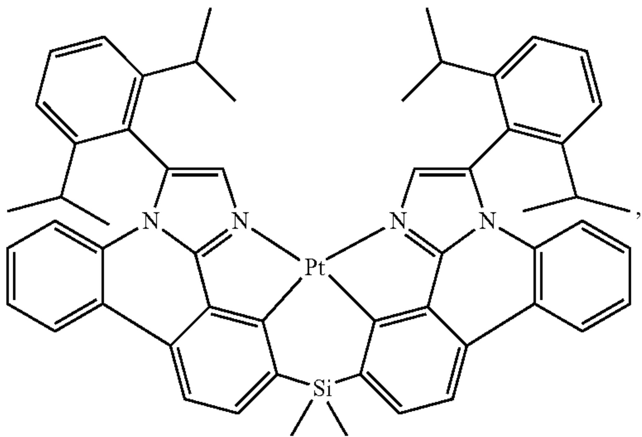
Compound 131
