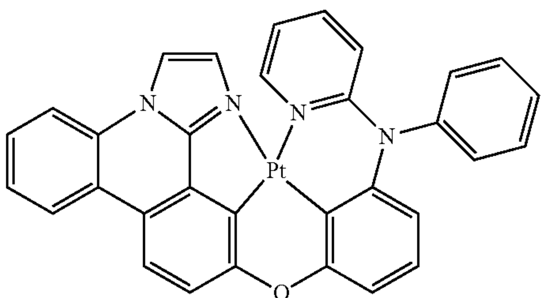
Compound 46'
