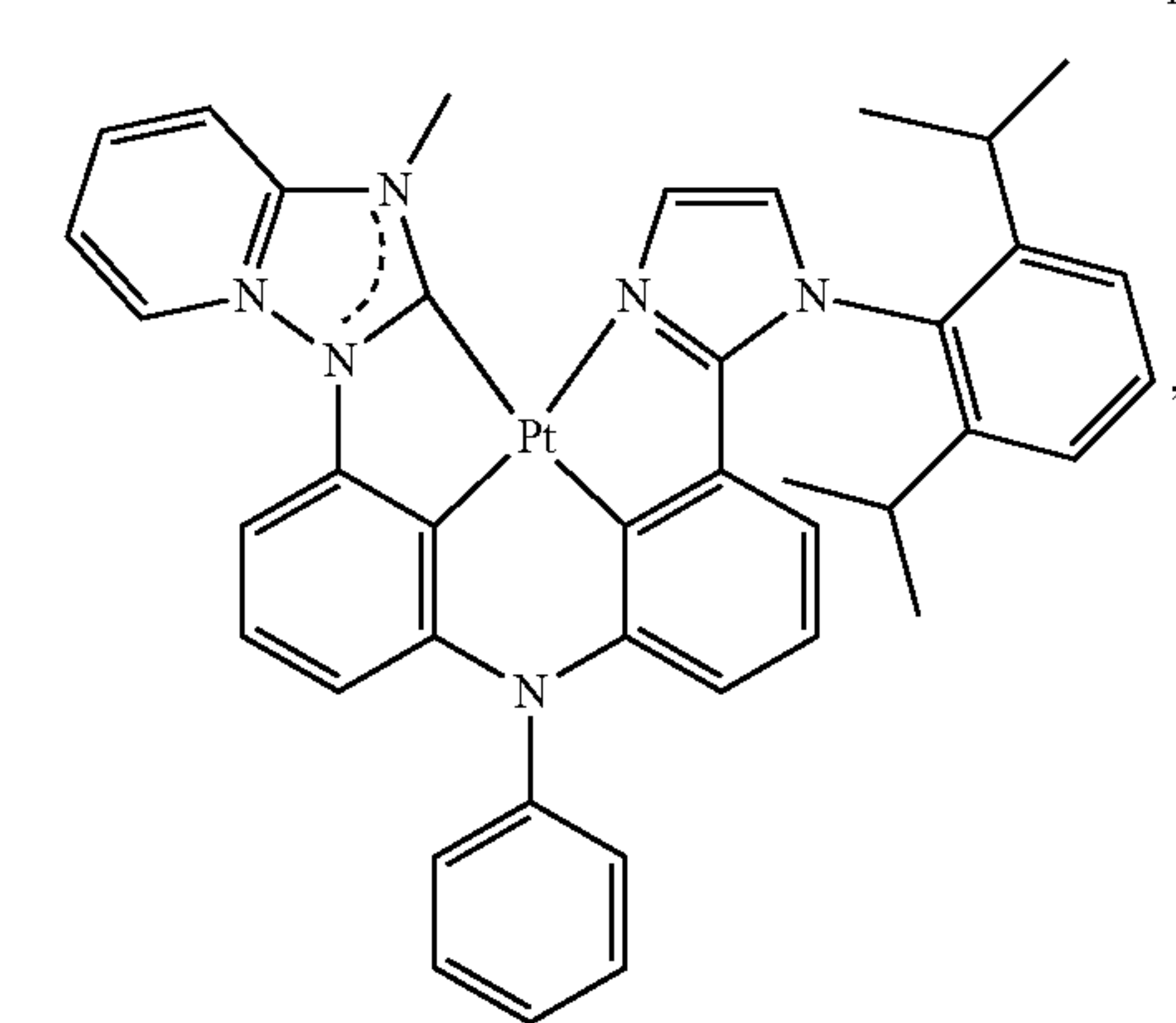
Compound 140
