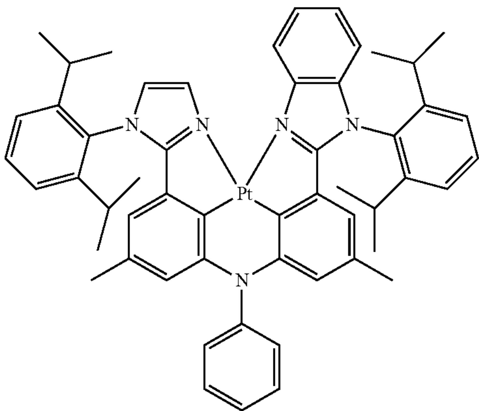
Compound 21
