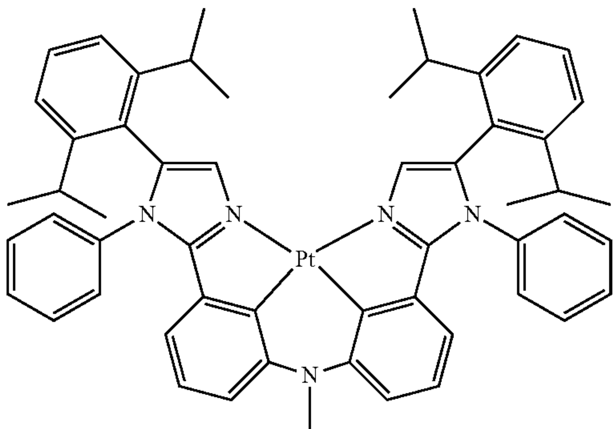
Compound 118
