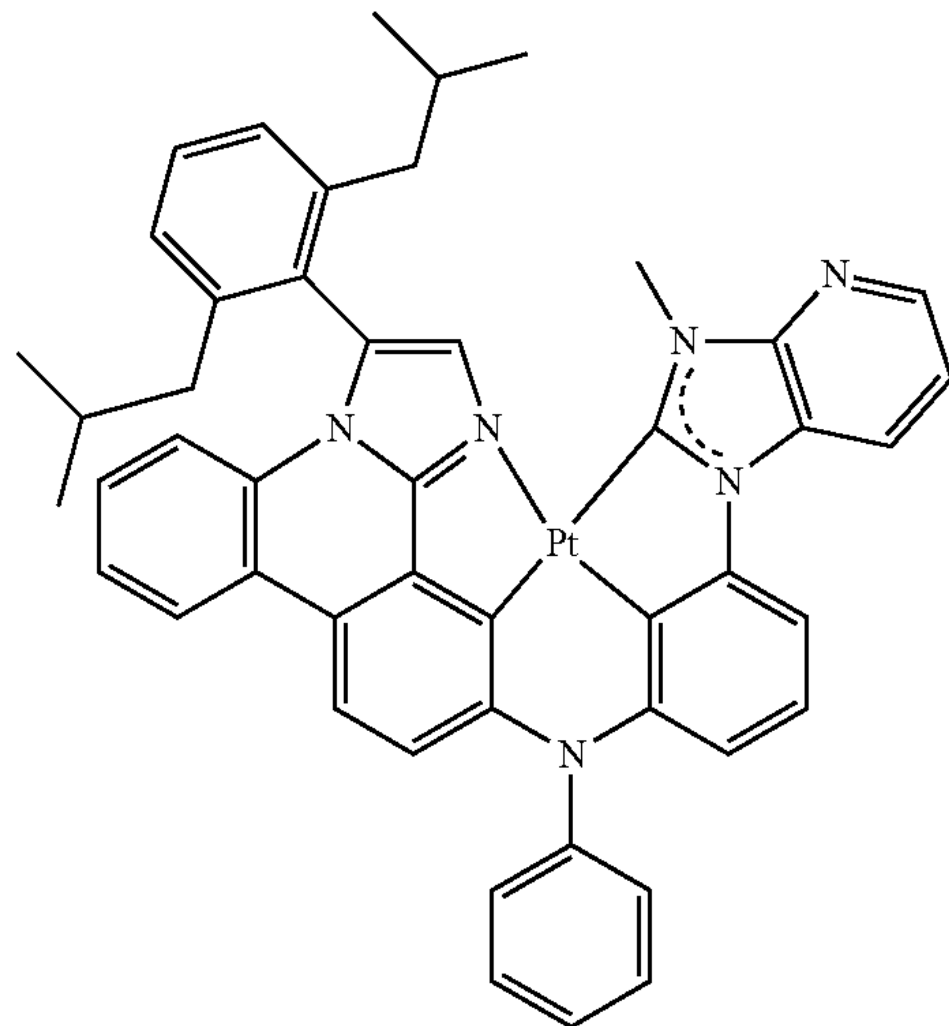
Compound 193'
