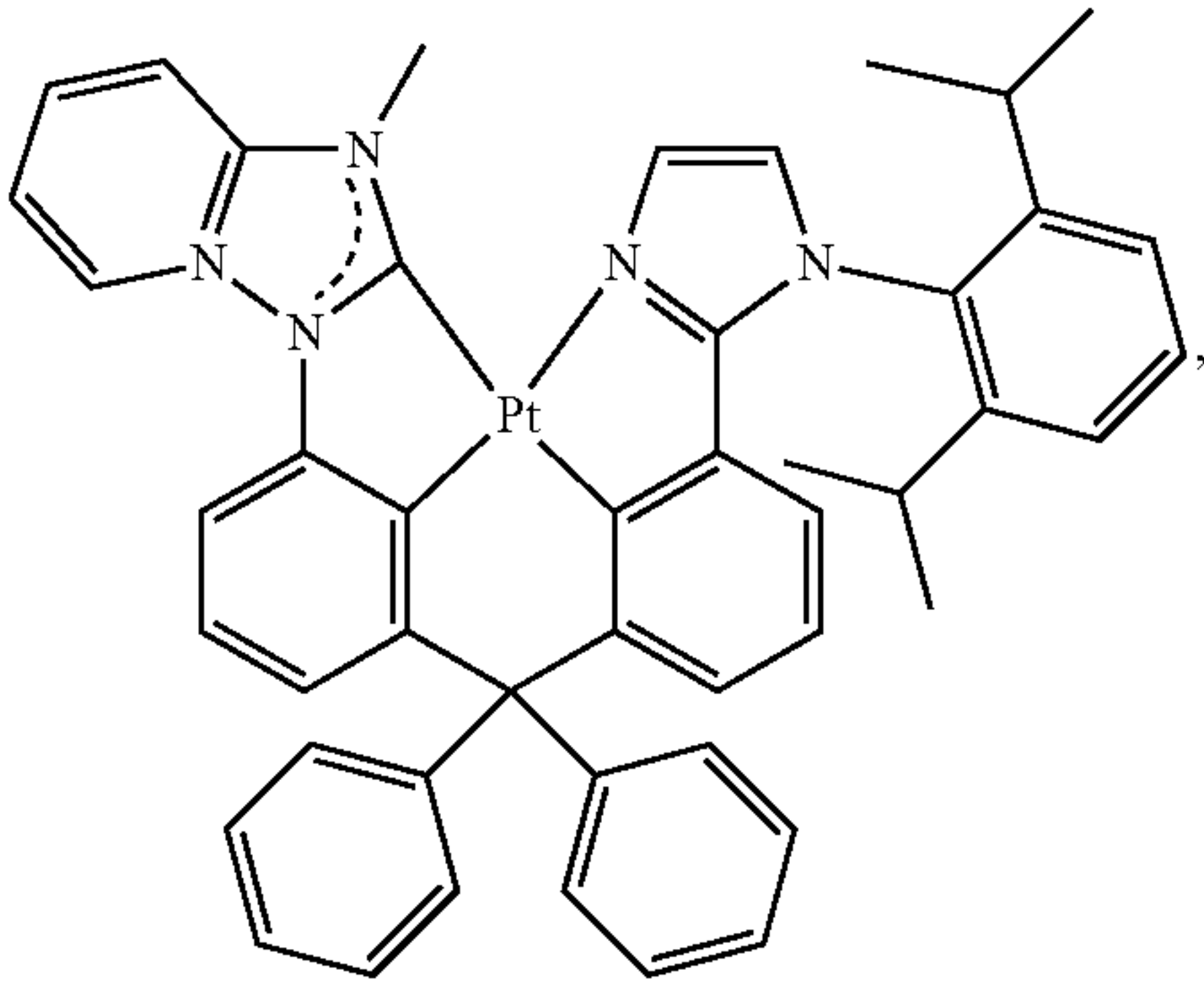
Compound 145
