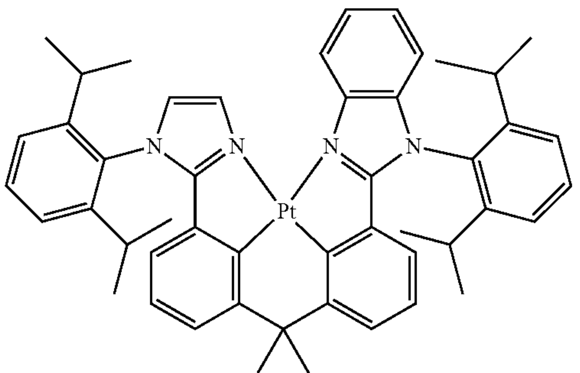
Compound 25
