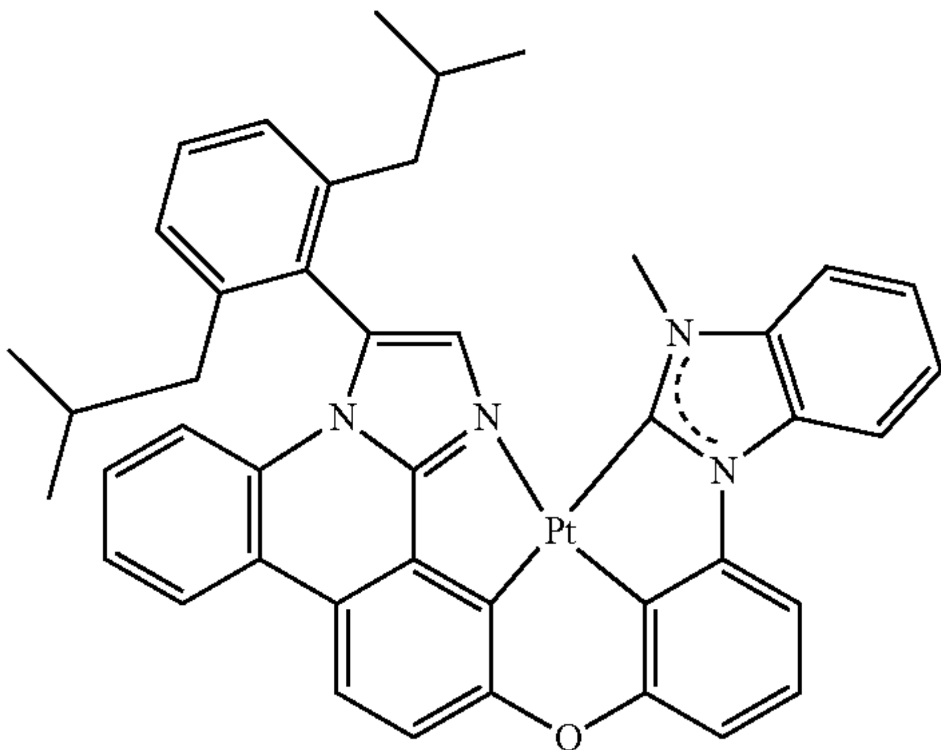
Compound 156'
