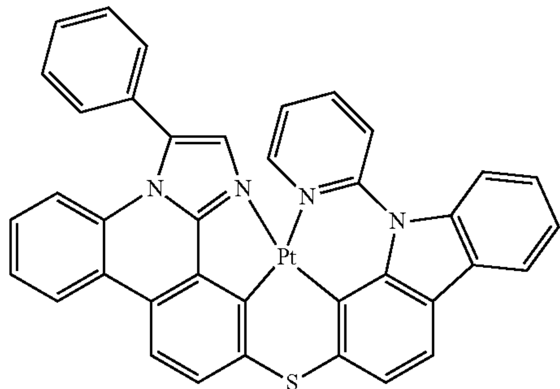
Compound 32'
