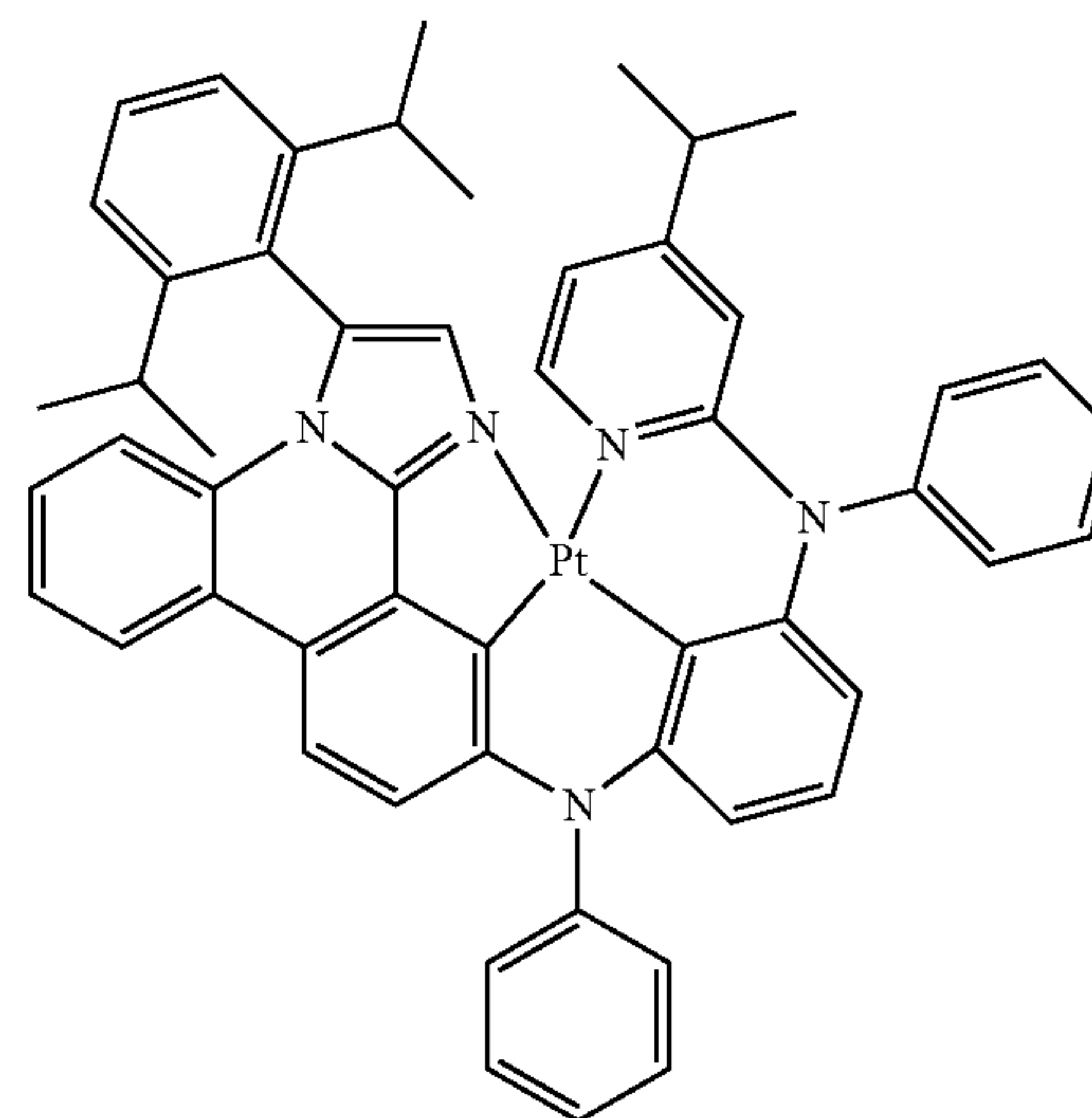
Compound 57'
