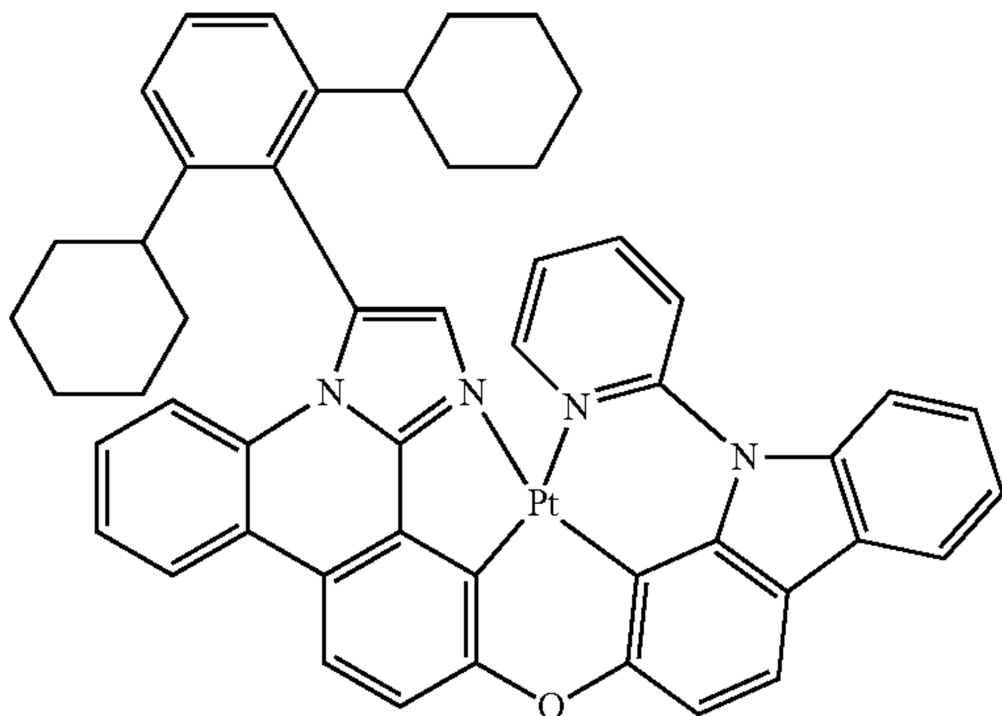
Compound 15'
