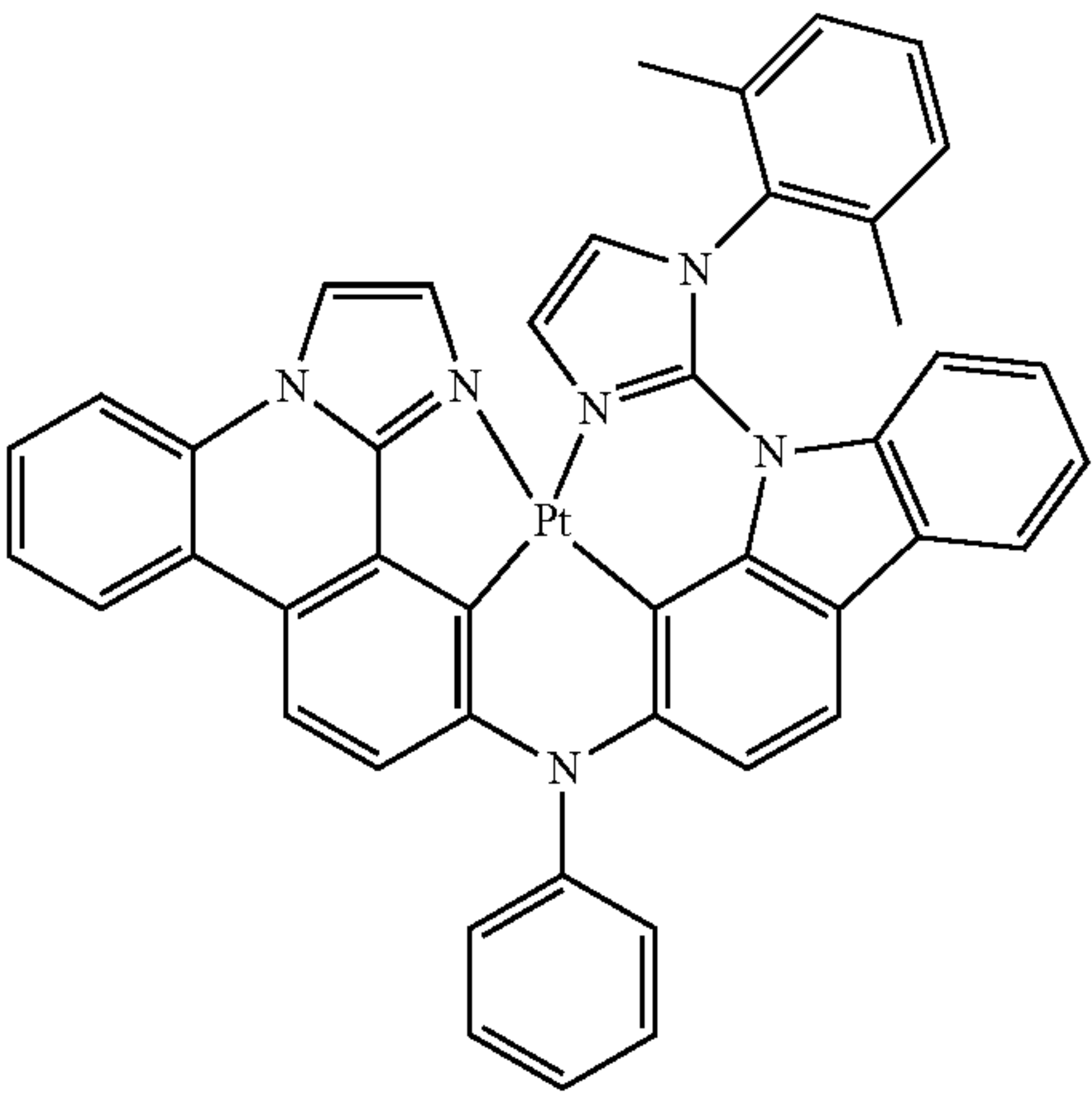
Compound 133'
