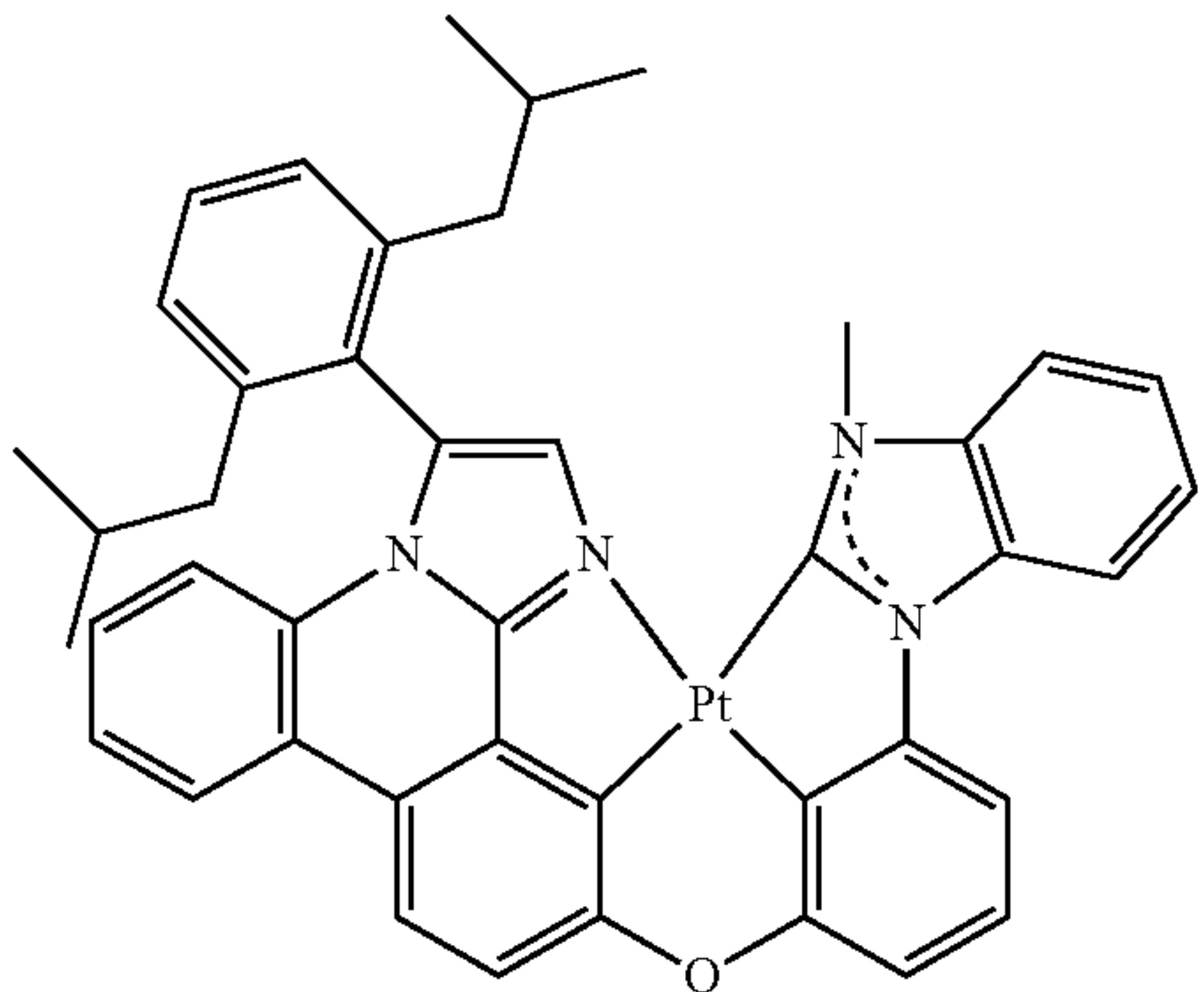
Compound 157'
