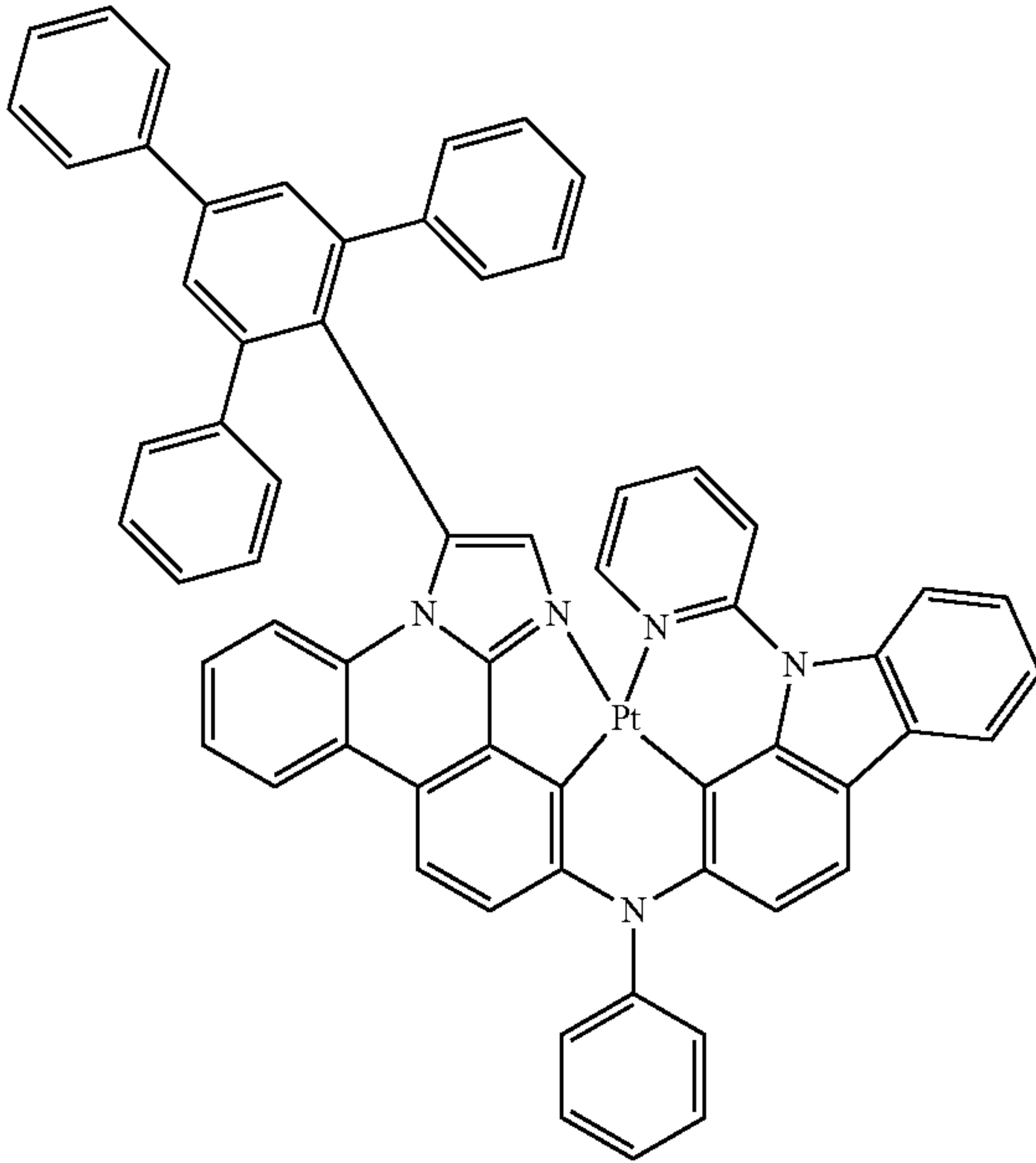
Compound 30'
