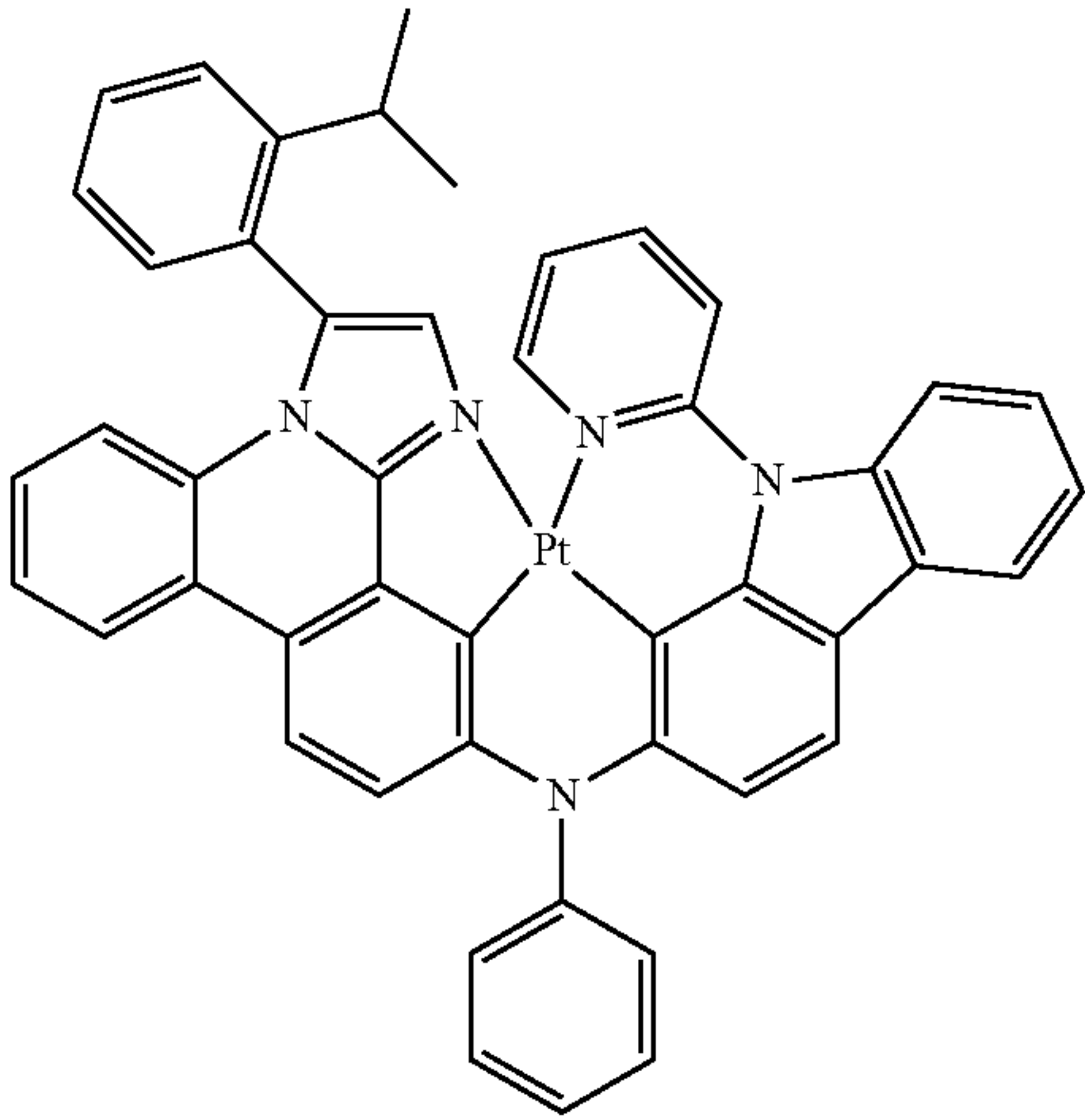
Compound 27'
