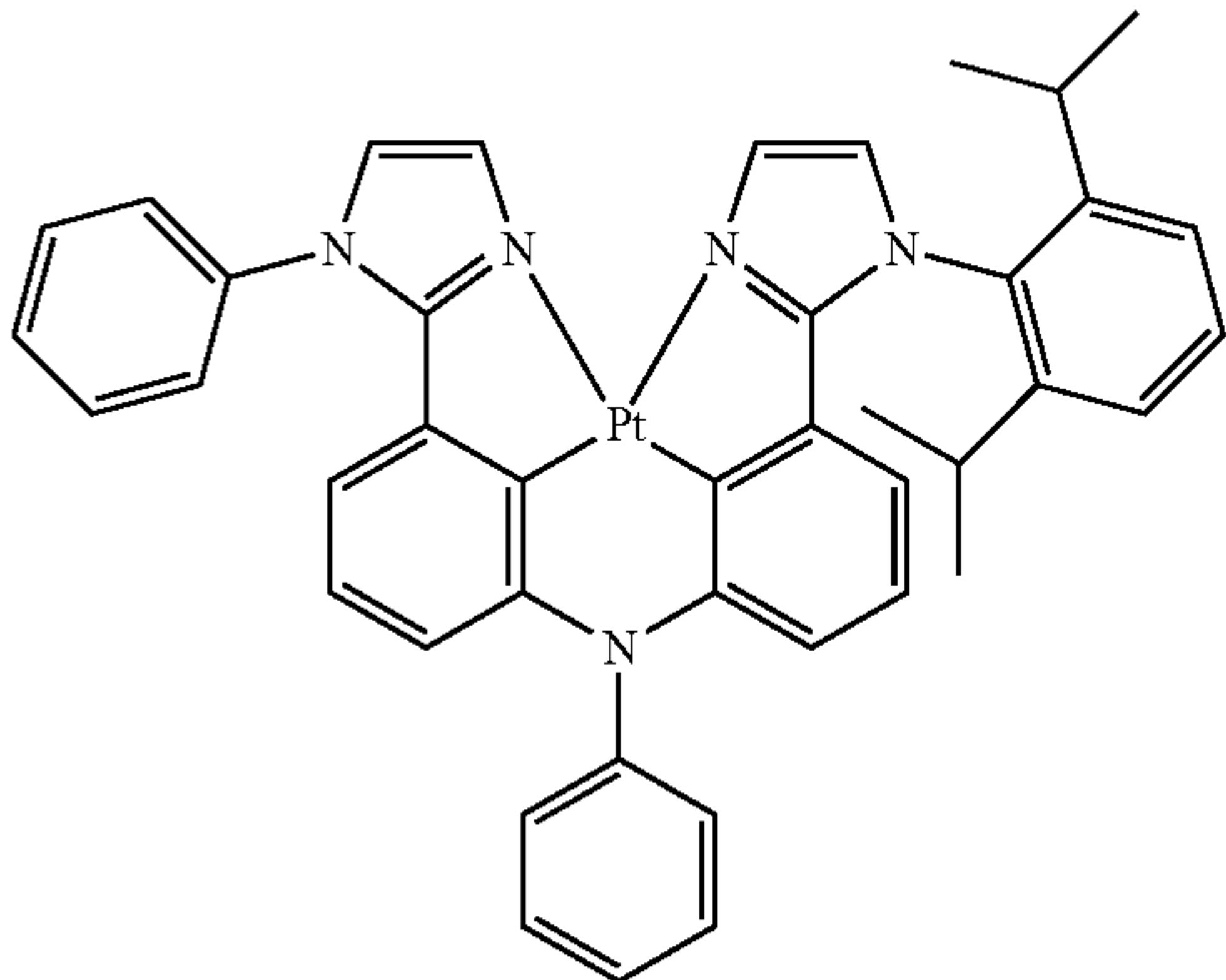
Compound 57
