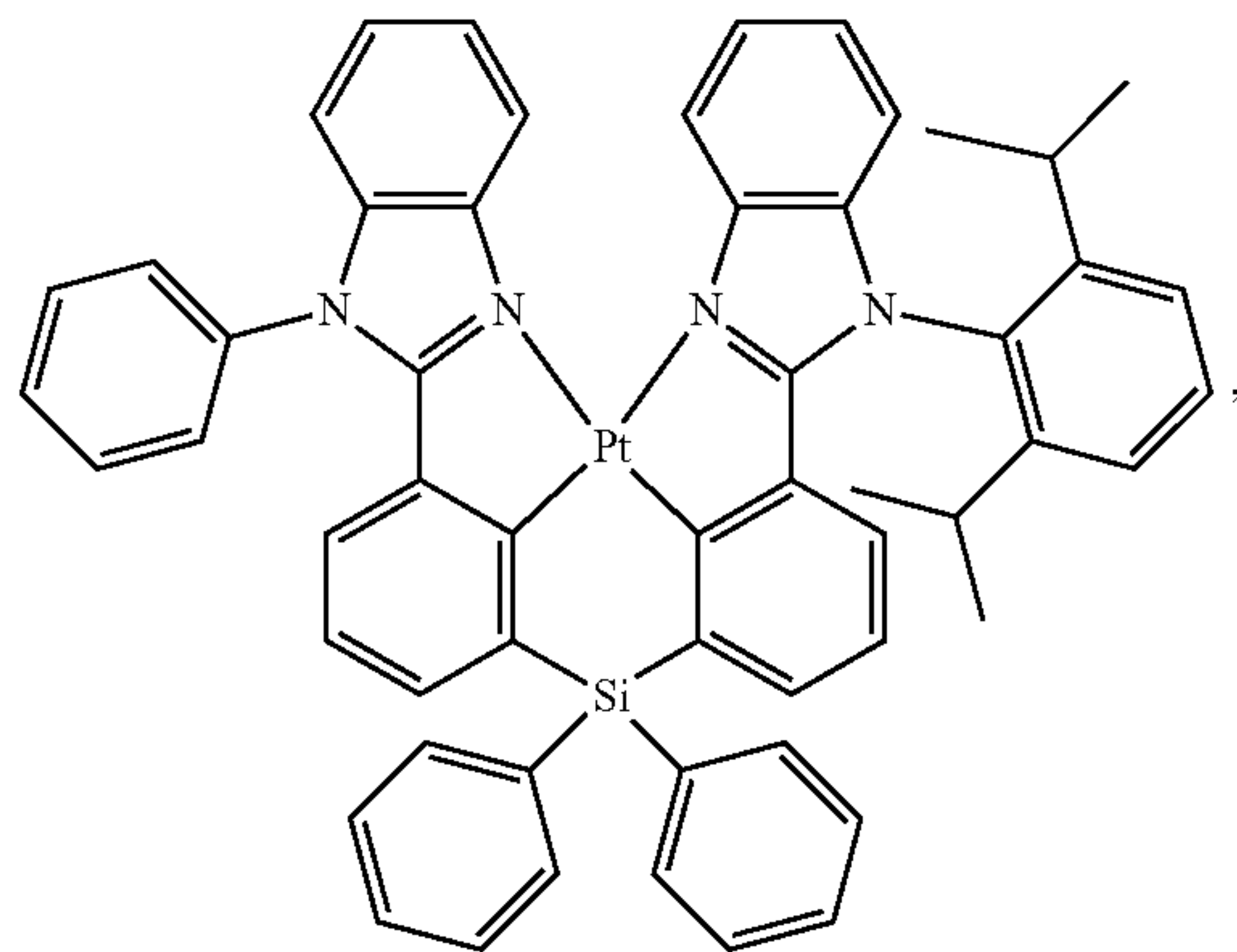
Compound 117
