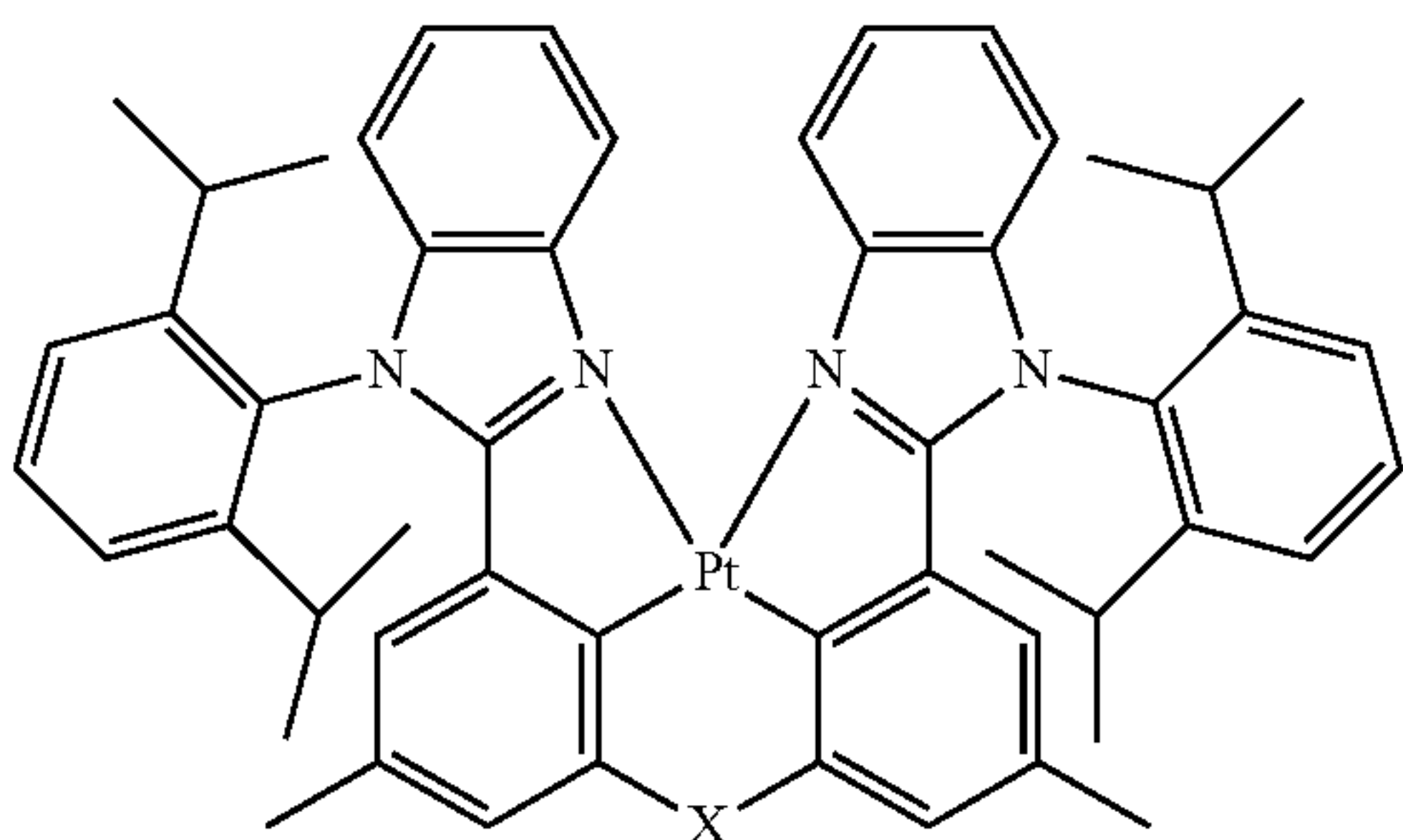
Compound 8G
