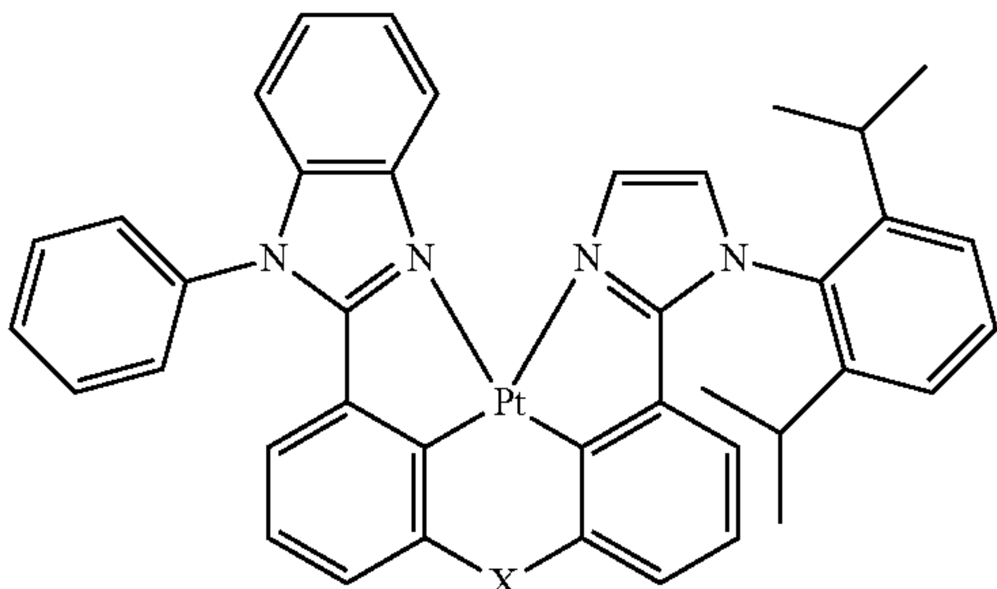
Compound 14G
