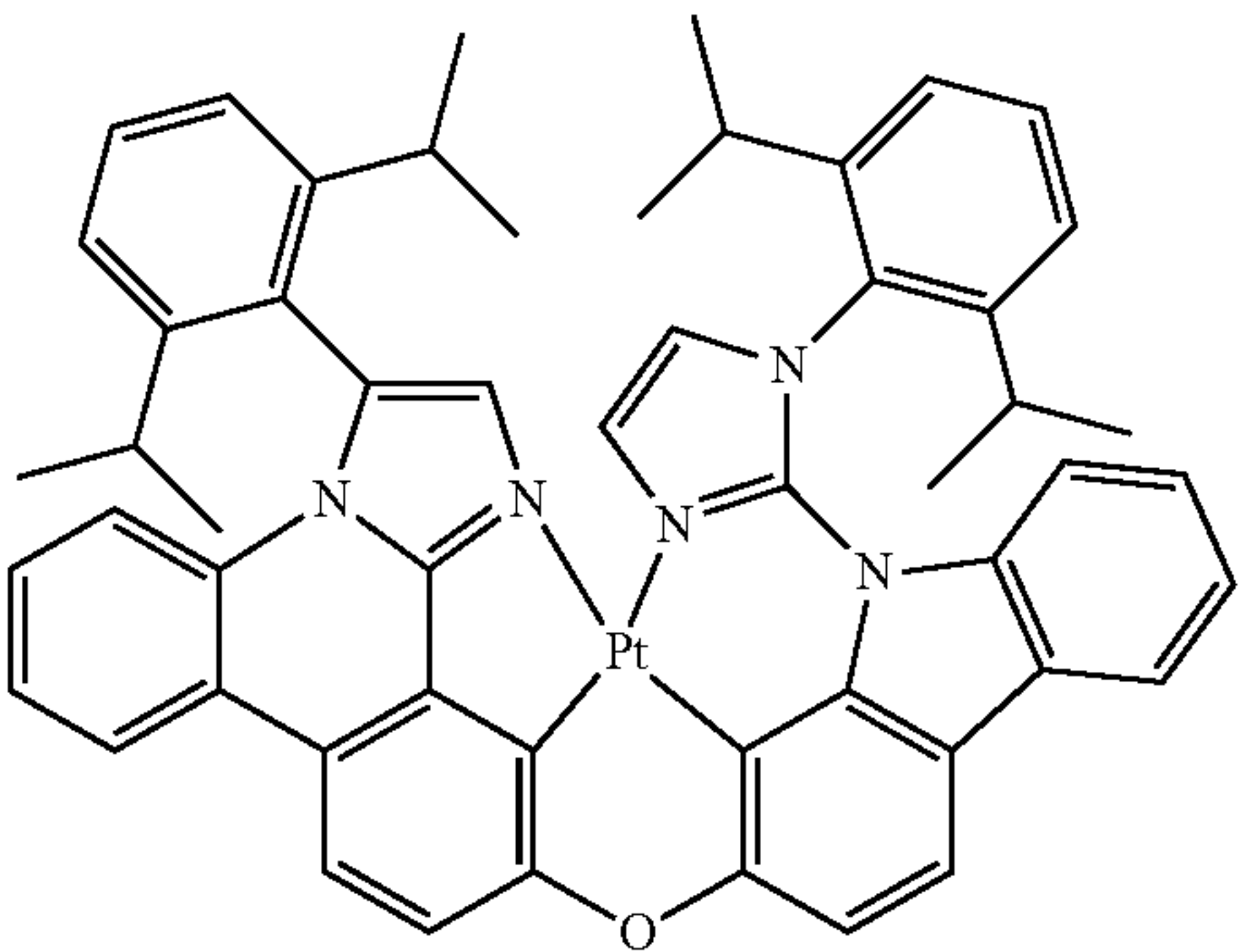
Compound 132'
