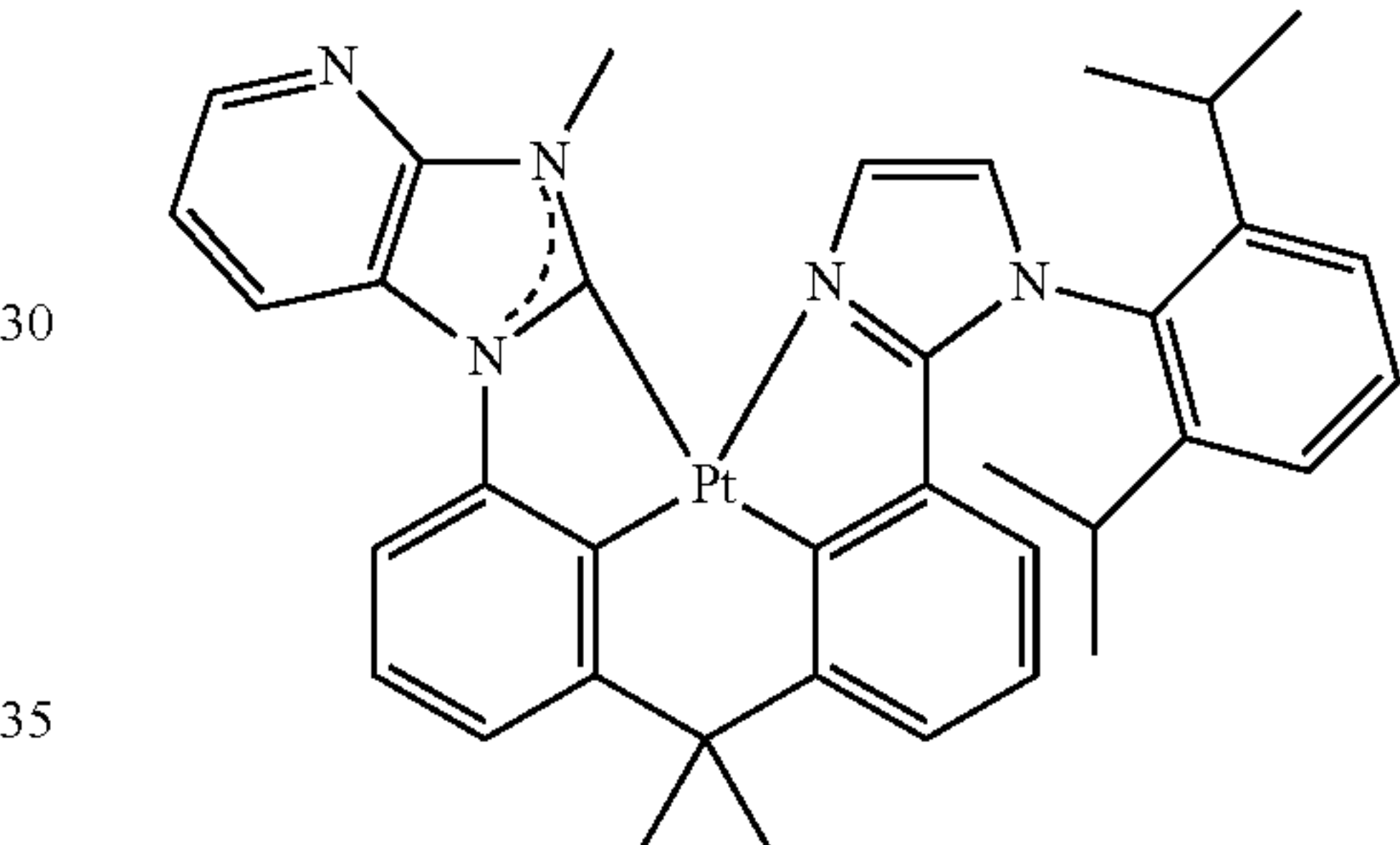
Compound 153
