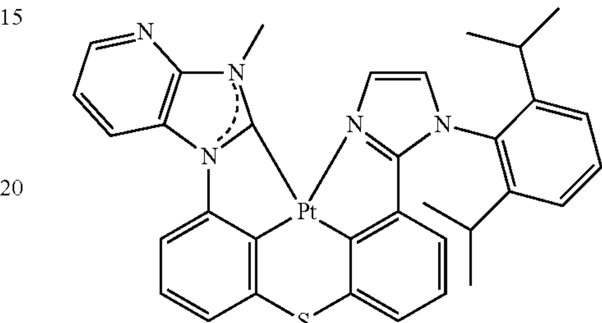
Compound 152
