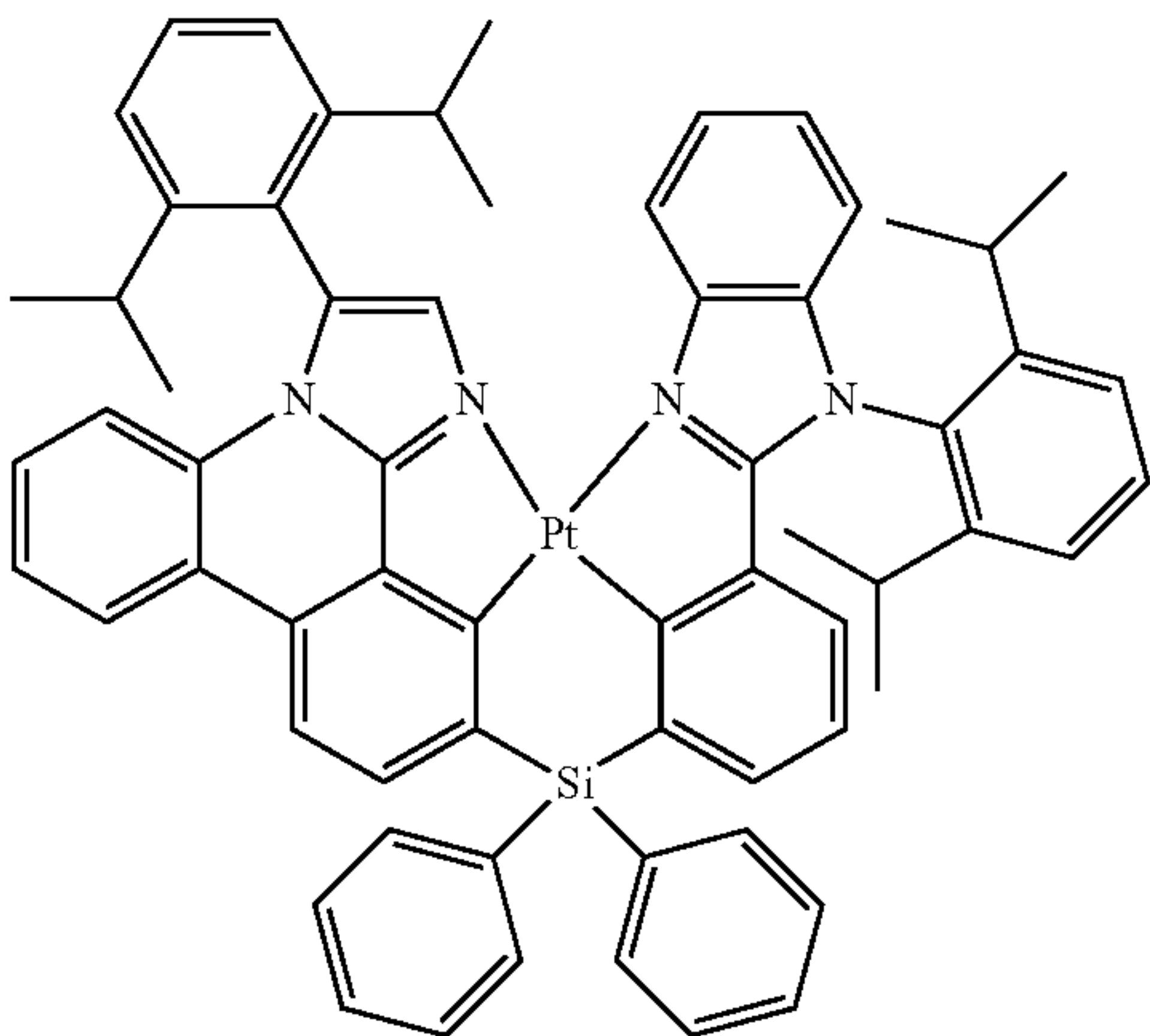
Compound 120'
