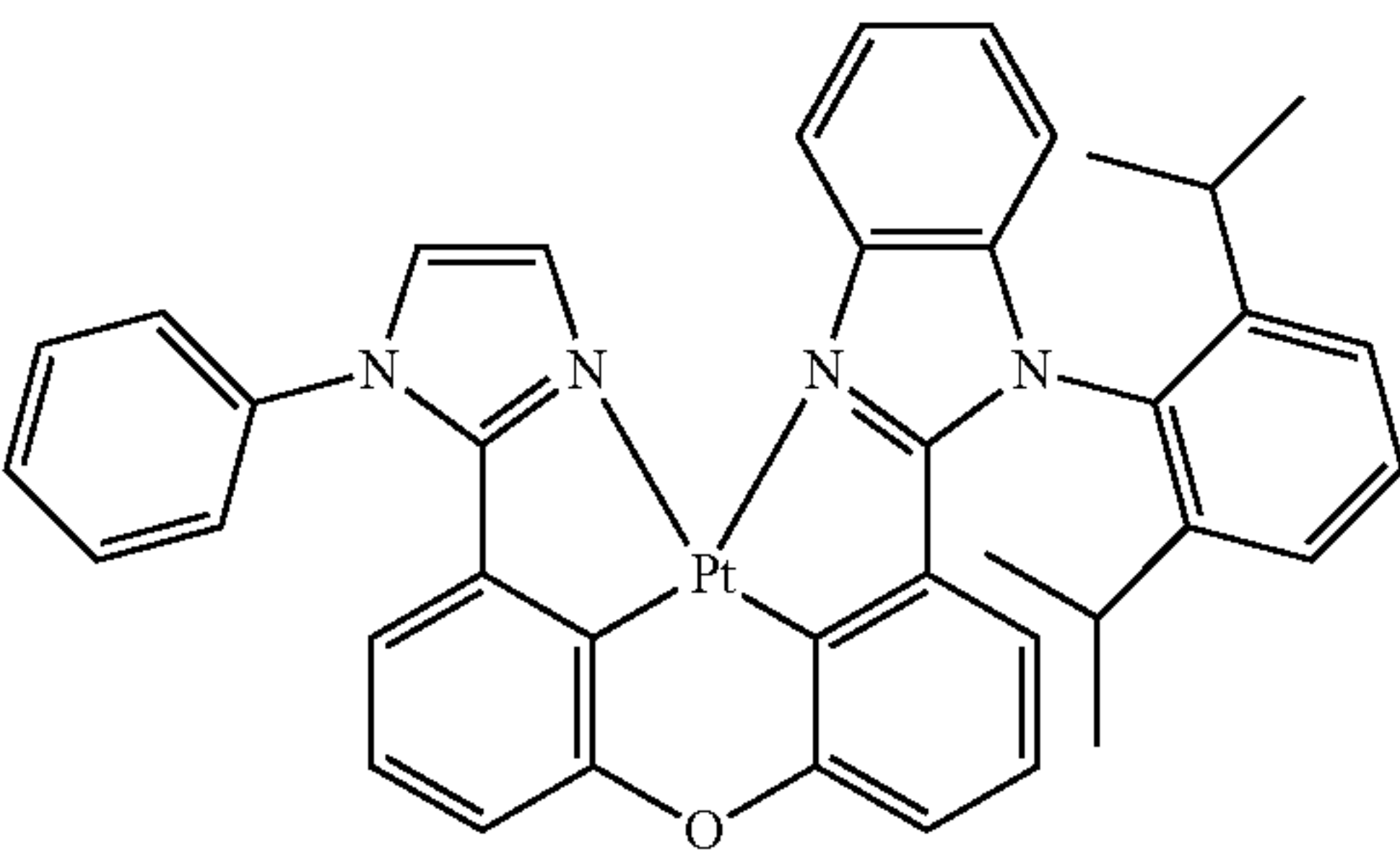
Compound 103
