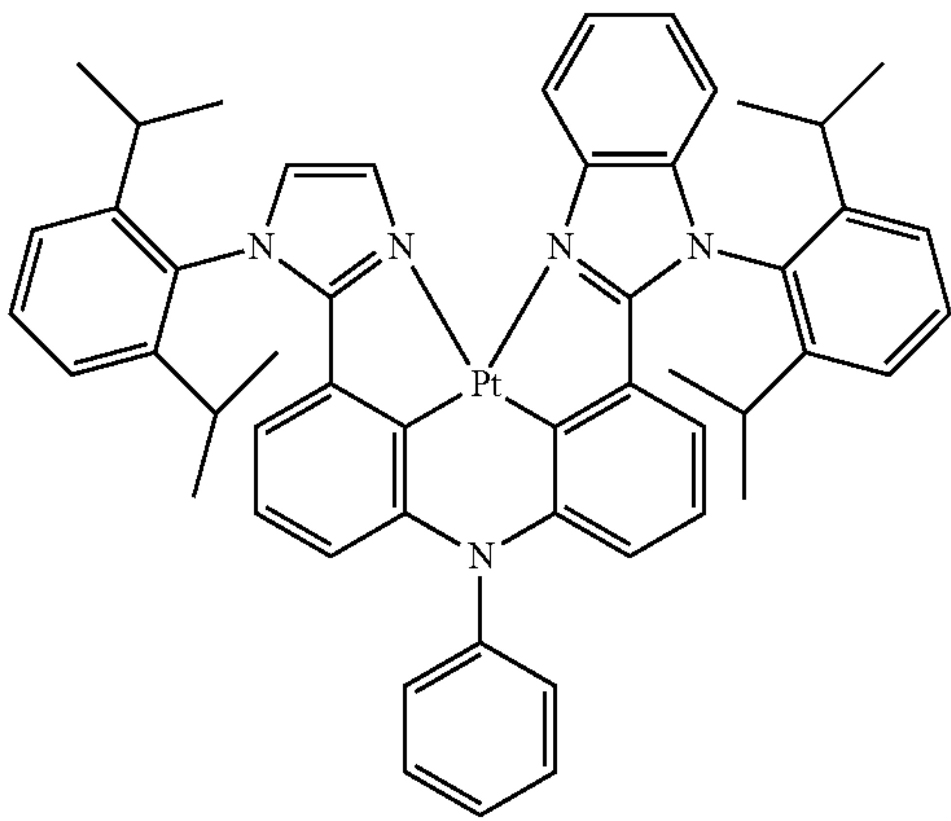
Compound 20
