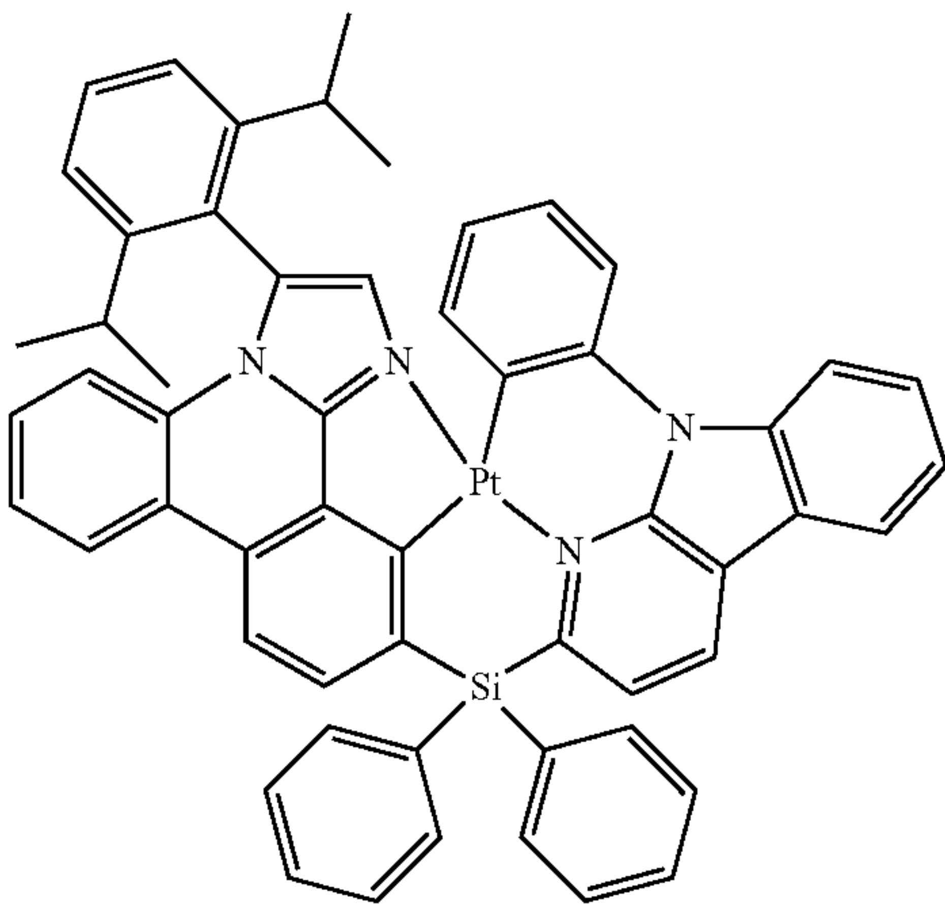
Compound 231'
