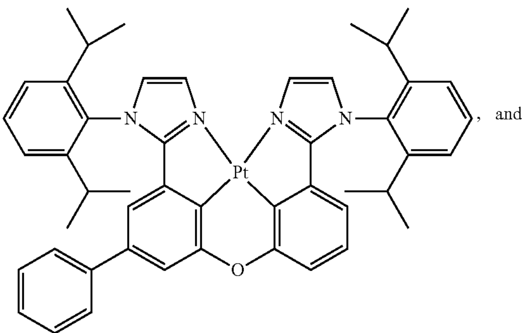
Compound 164
