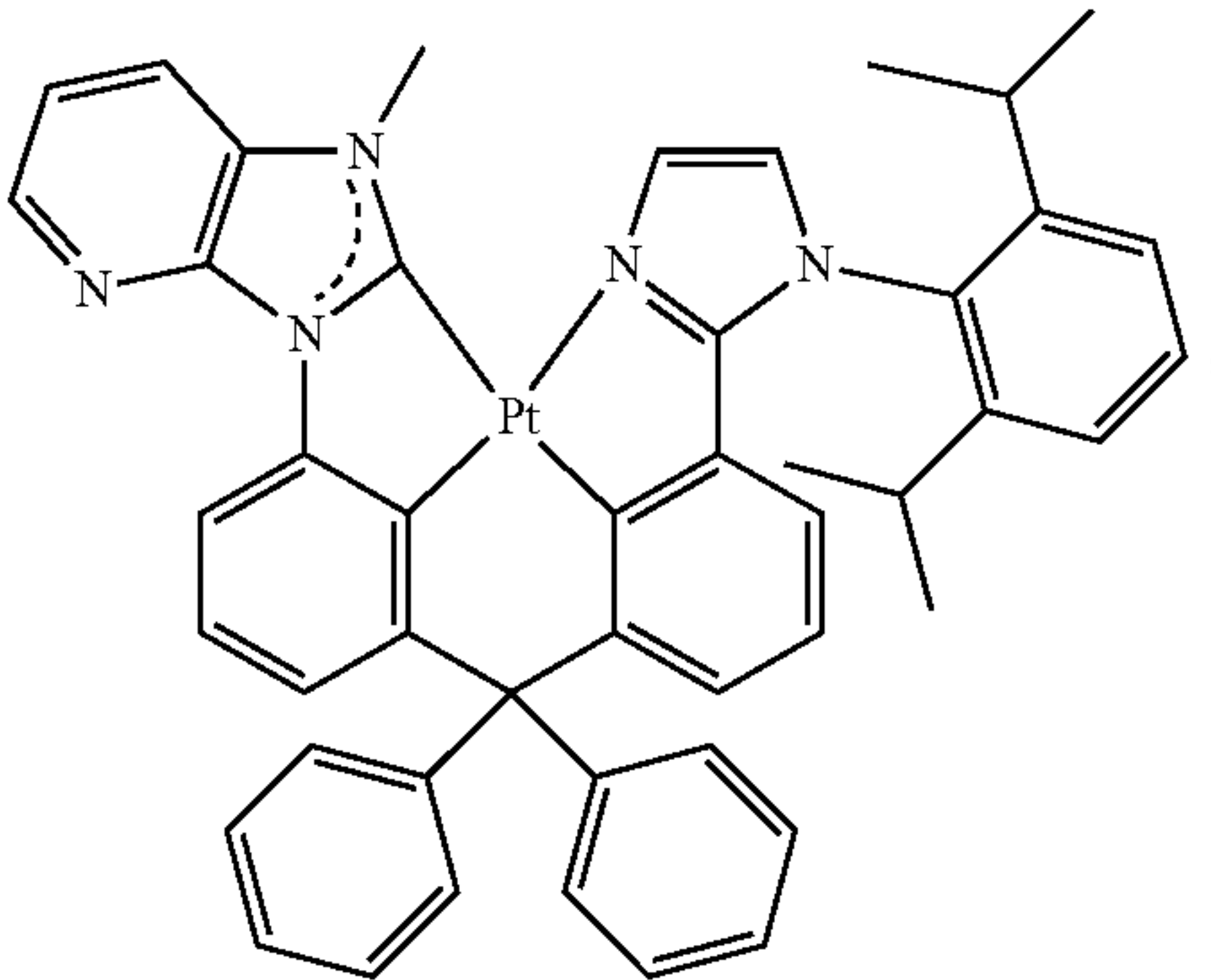
Compound 151
