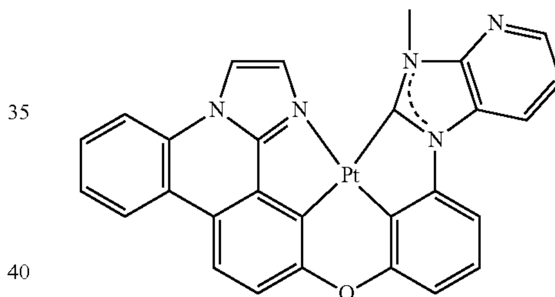
Compound 159'
