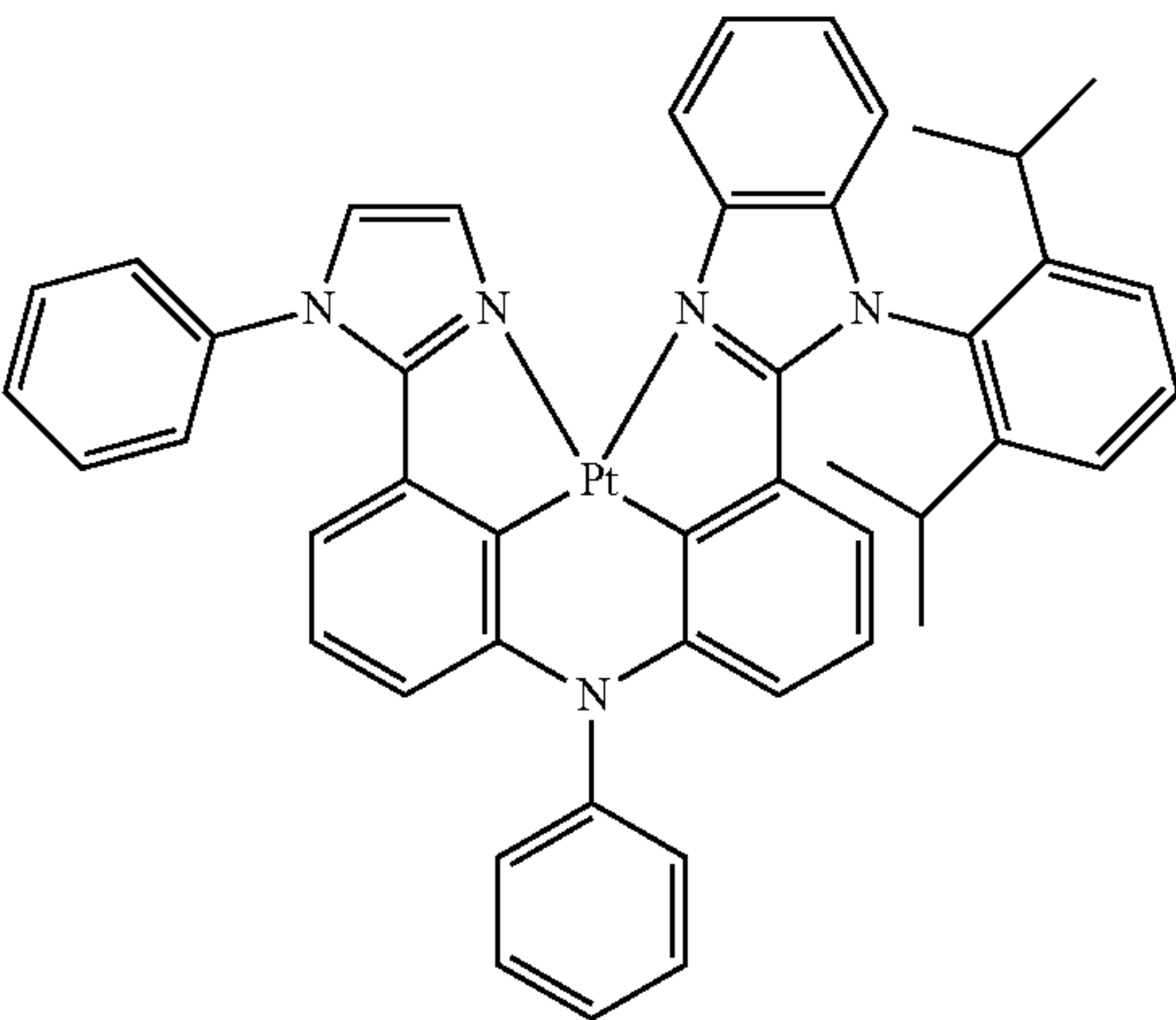
Compound 101
