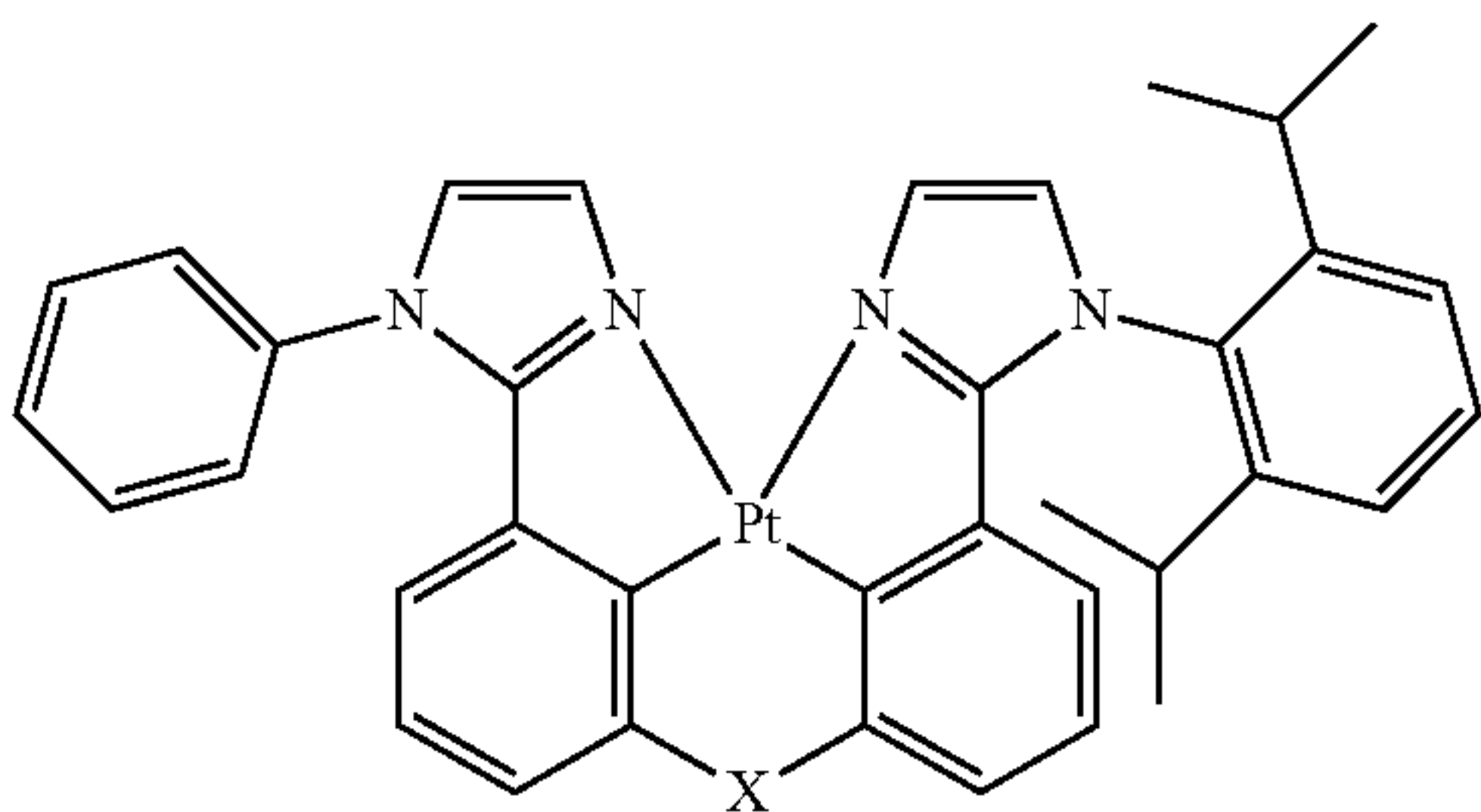
Compound 13G
