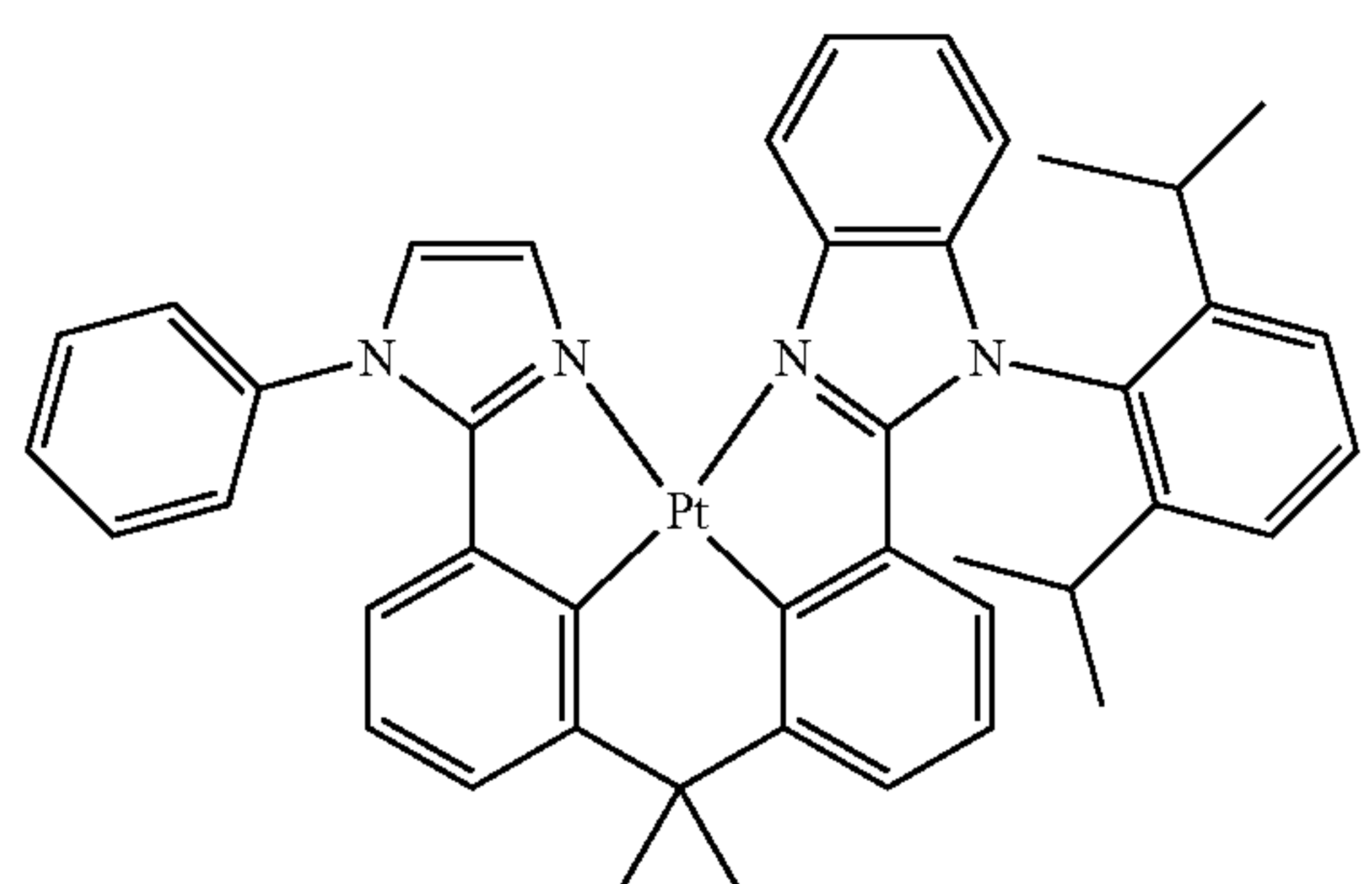
Compound 105
