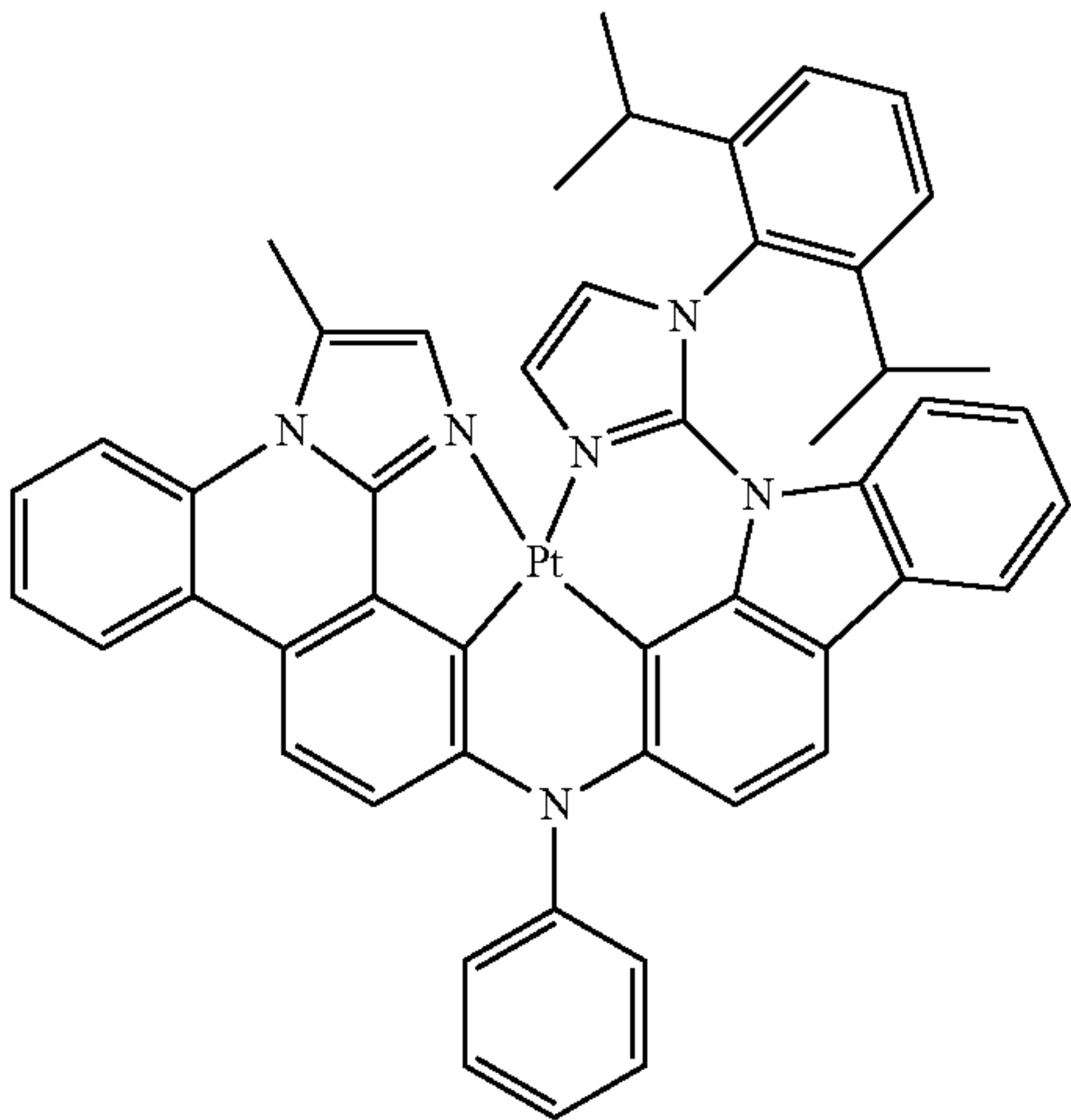
Compound 140'
