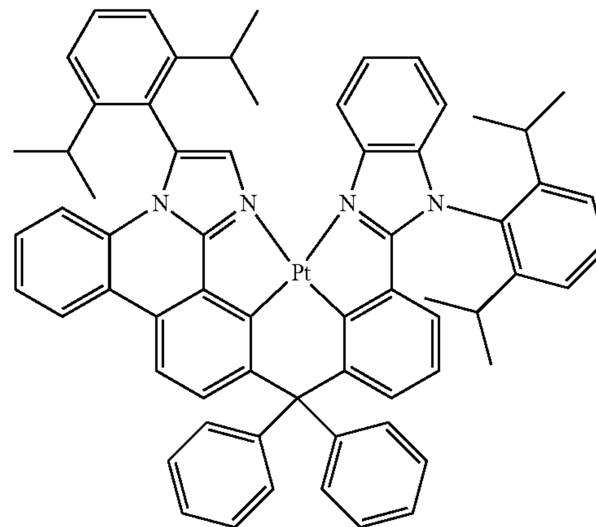
Compound 119'
