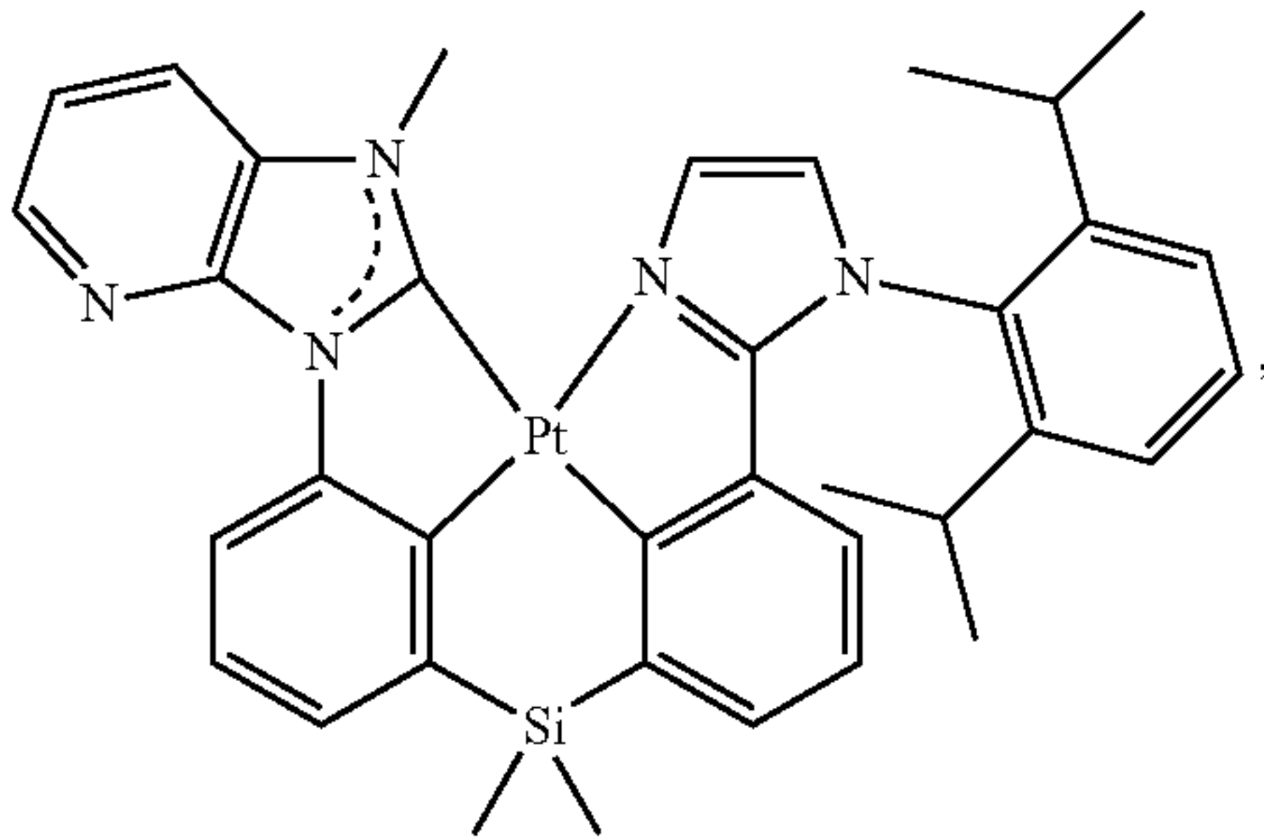
Compound 152
