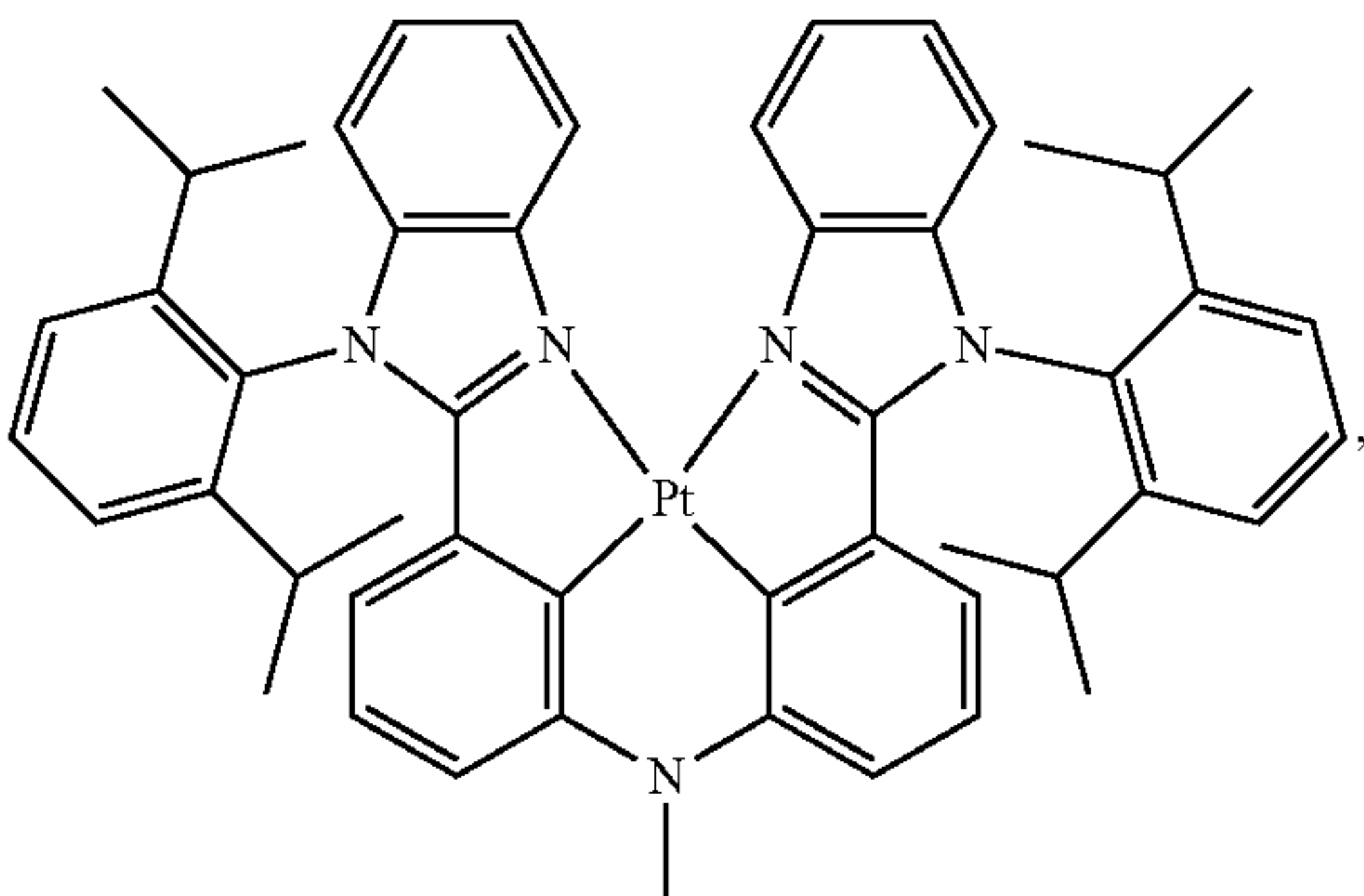
Compound 13
