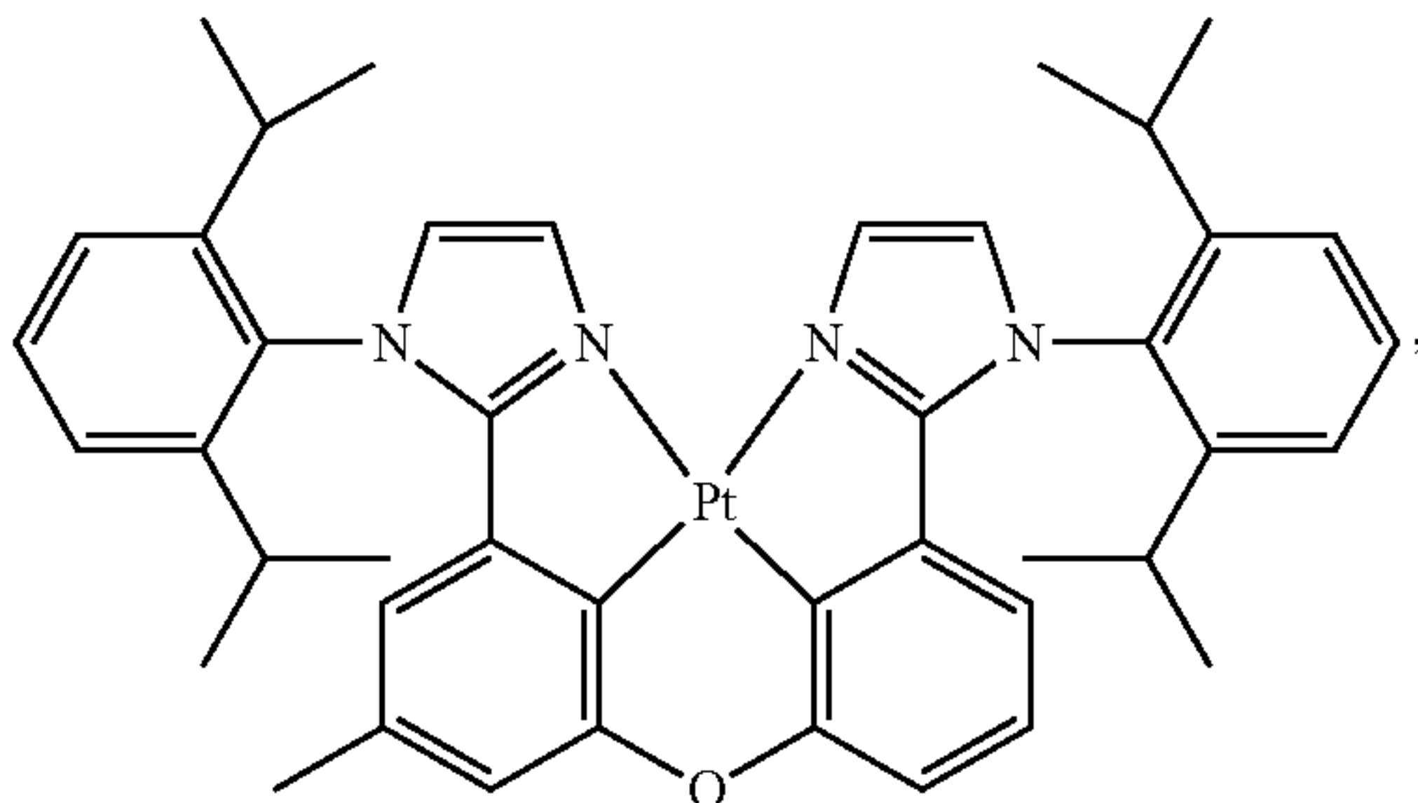
Compound 163
