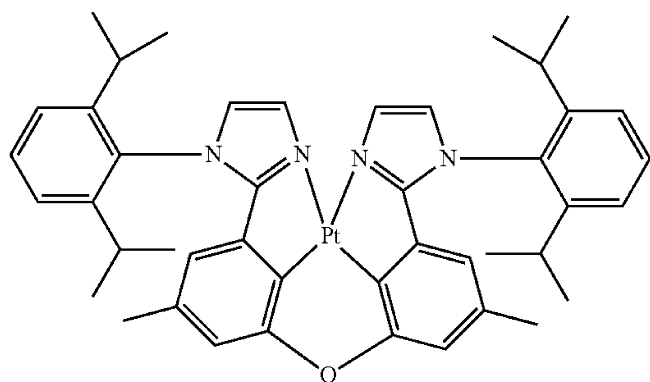
Compound 161
