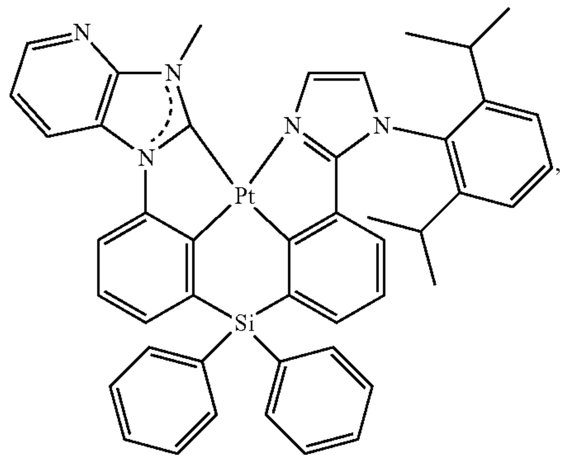
Compound 160
