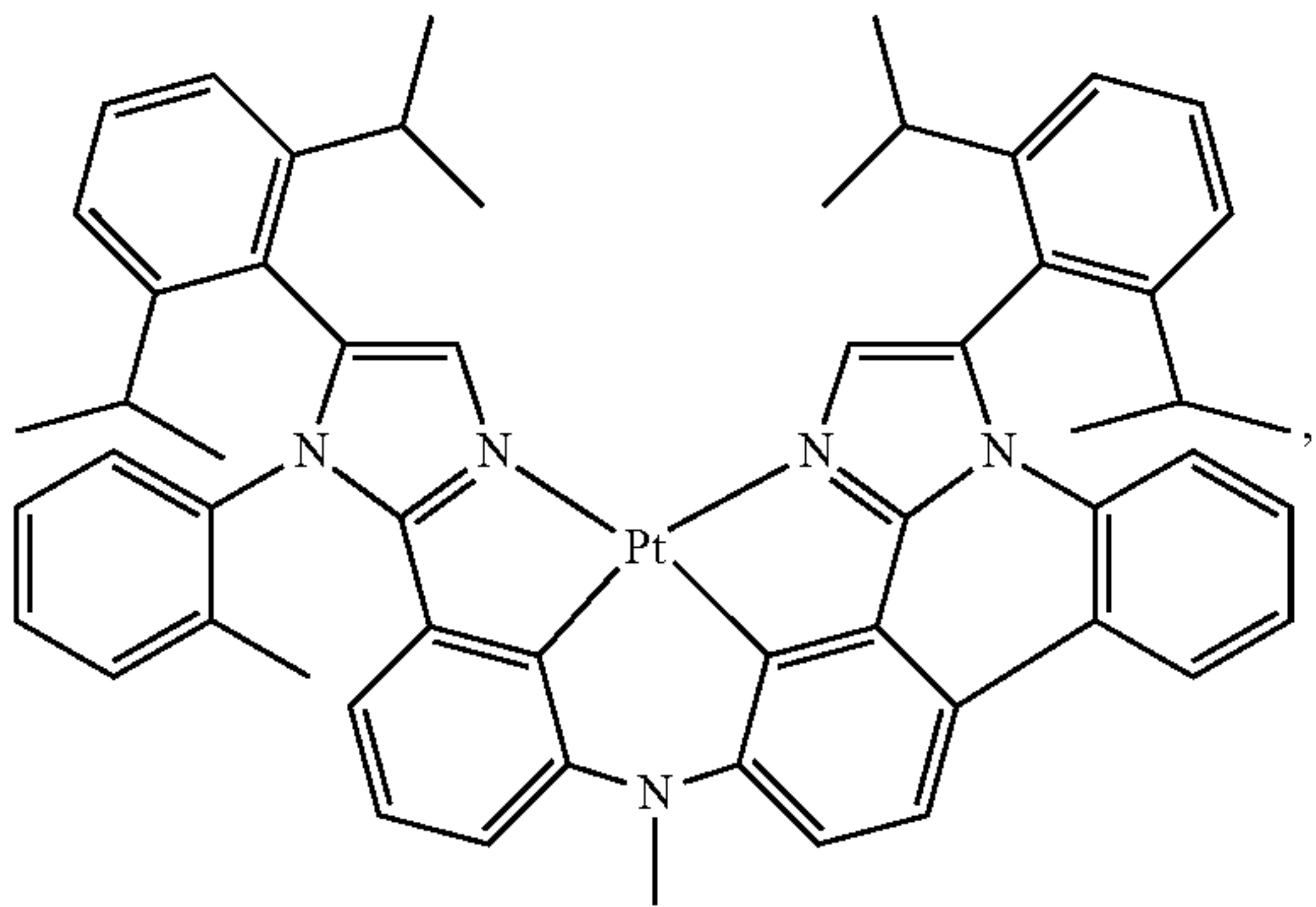
Compound 127
