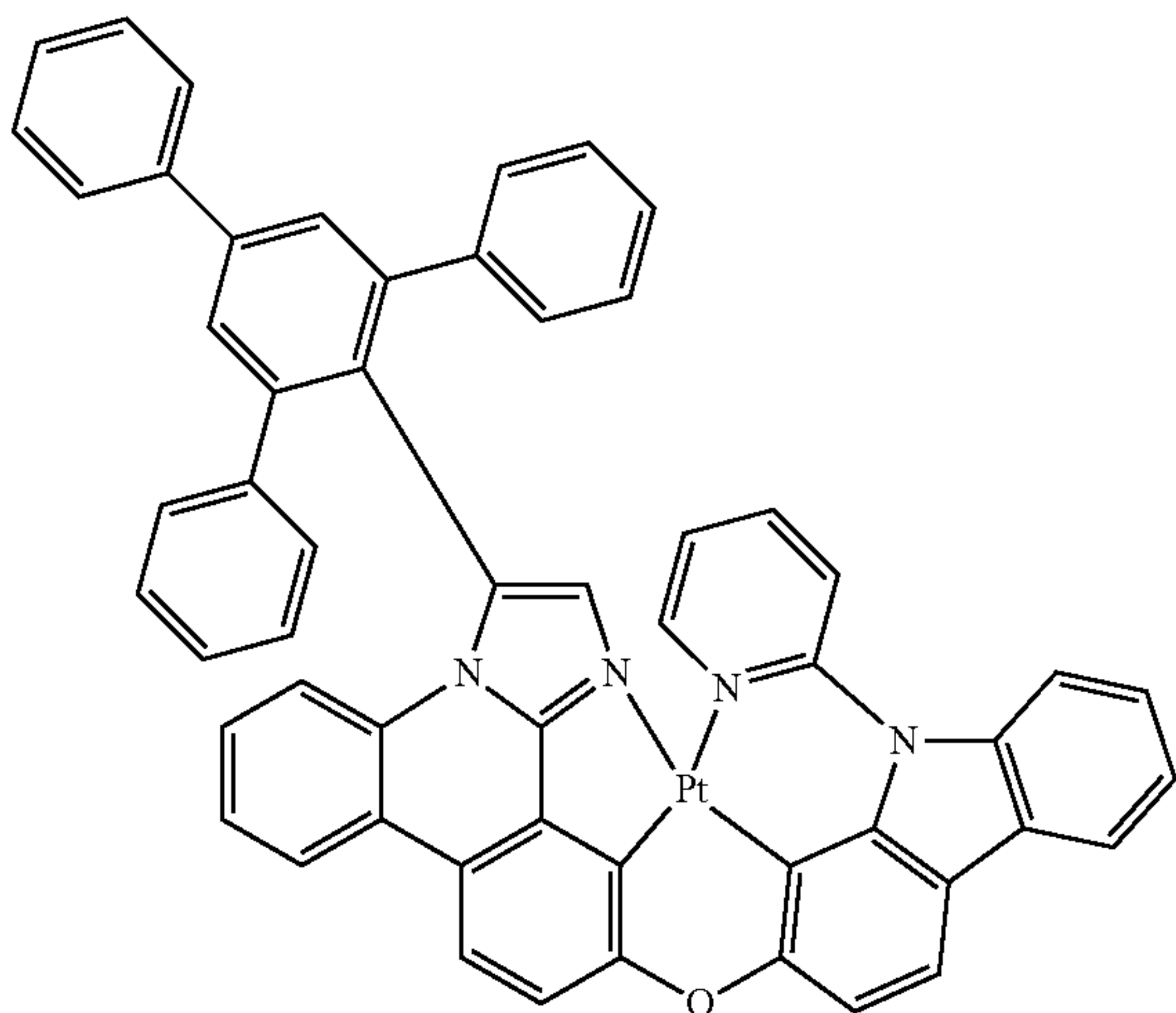
Compound 15'
