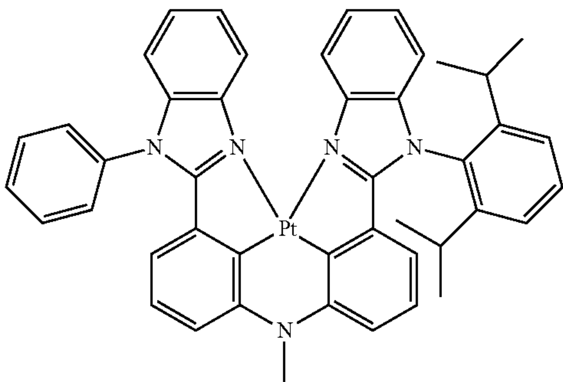
Compound 110
