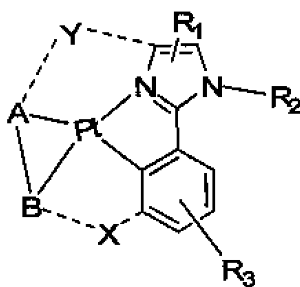
Formula I
