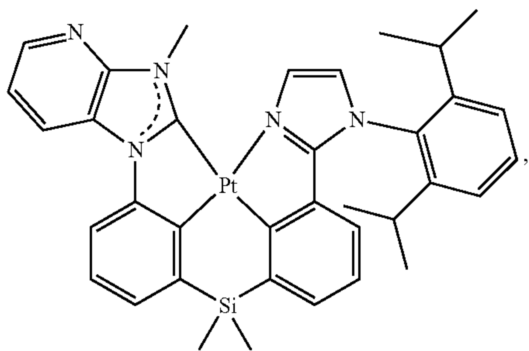
Compound 159
