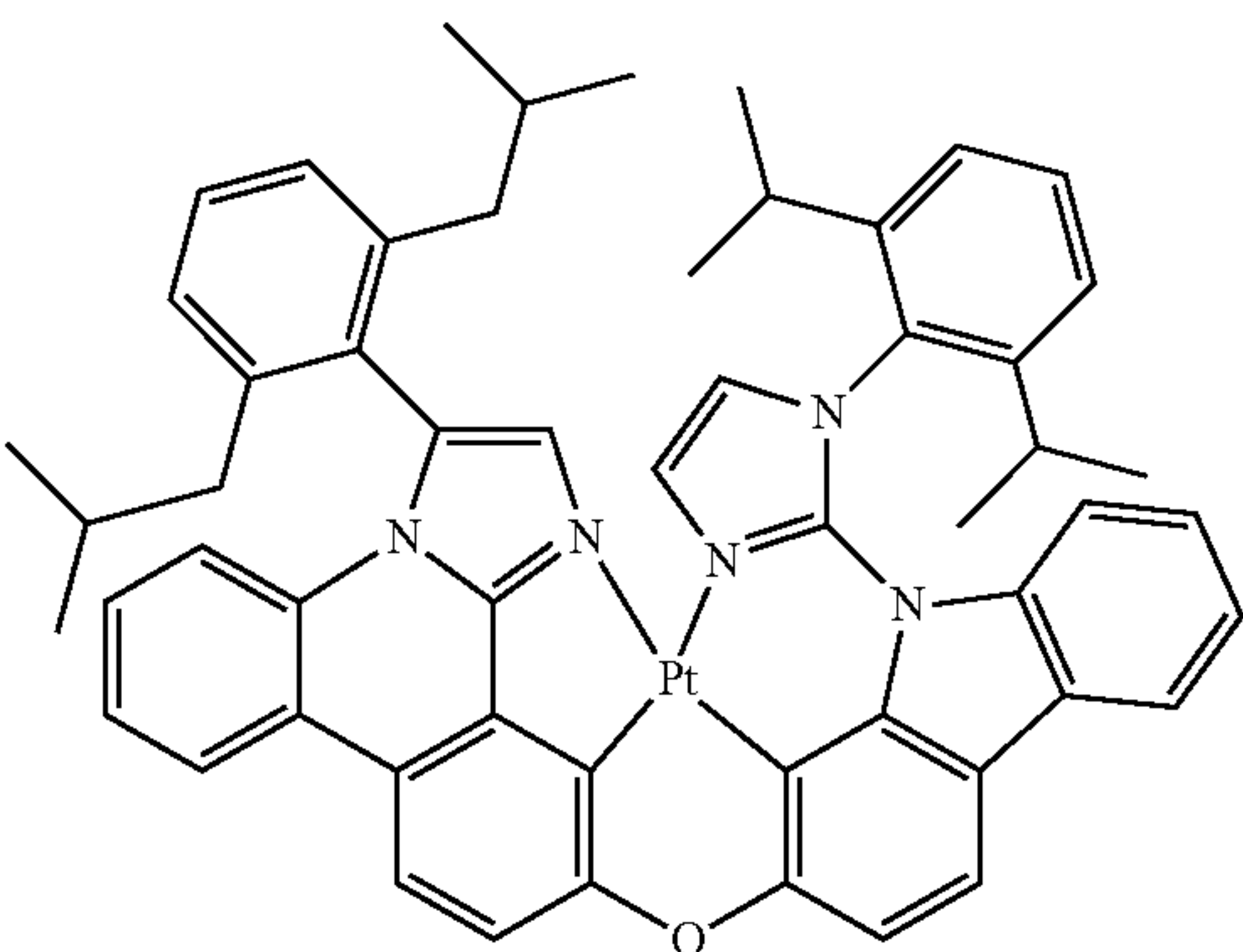
Compound 132'
