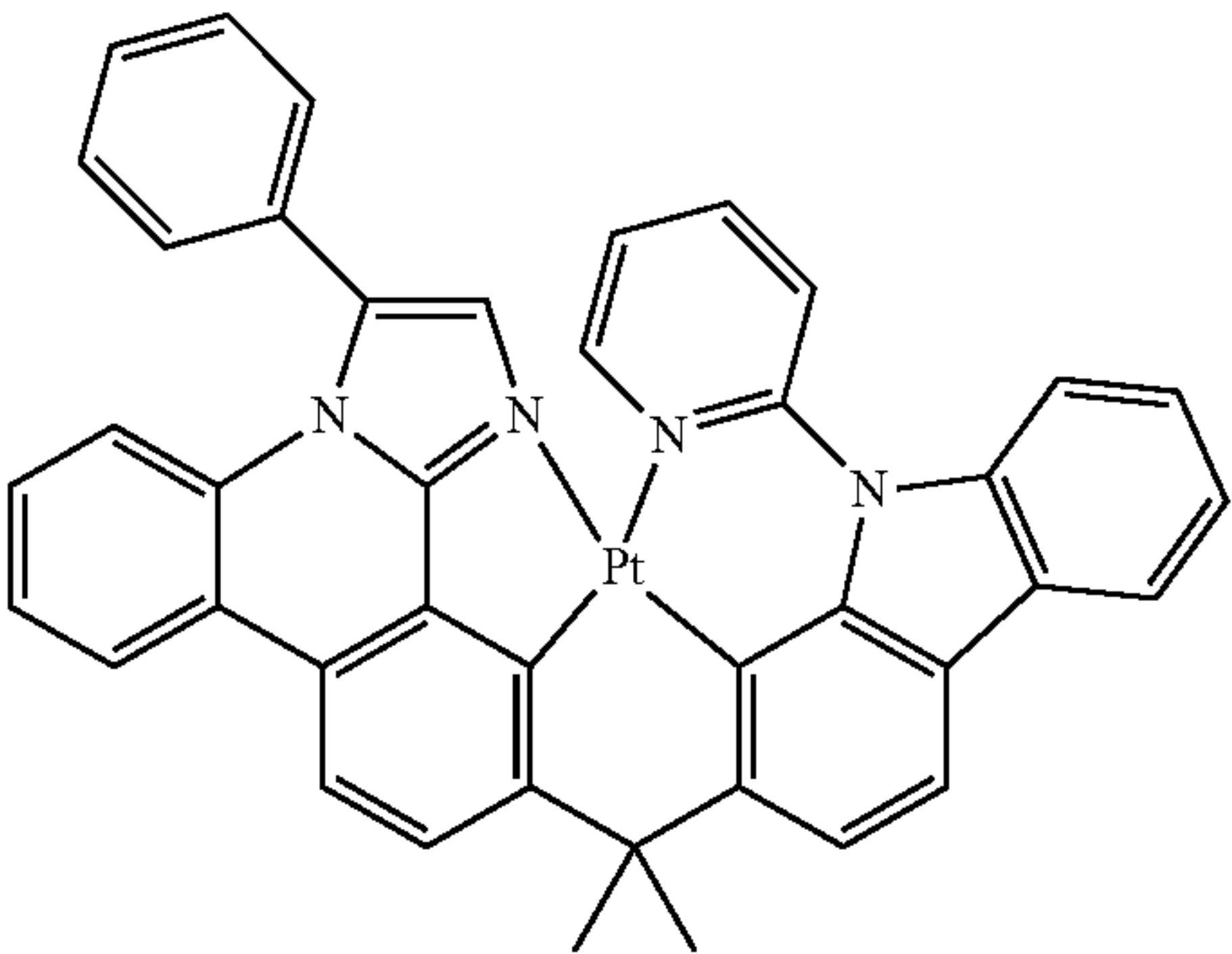
Compound 44'
