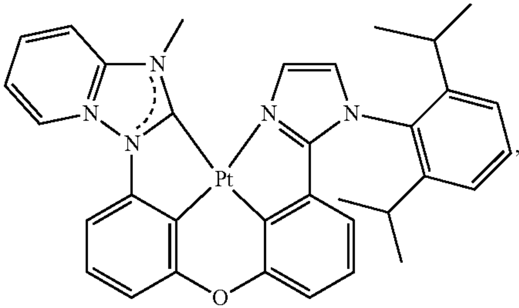
Compound 142
