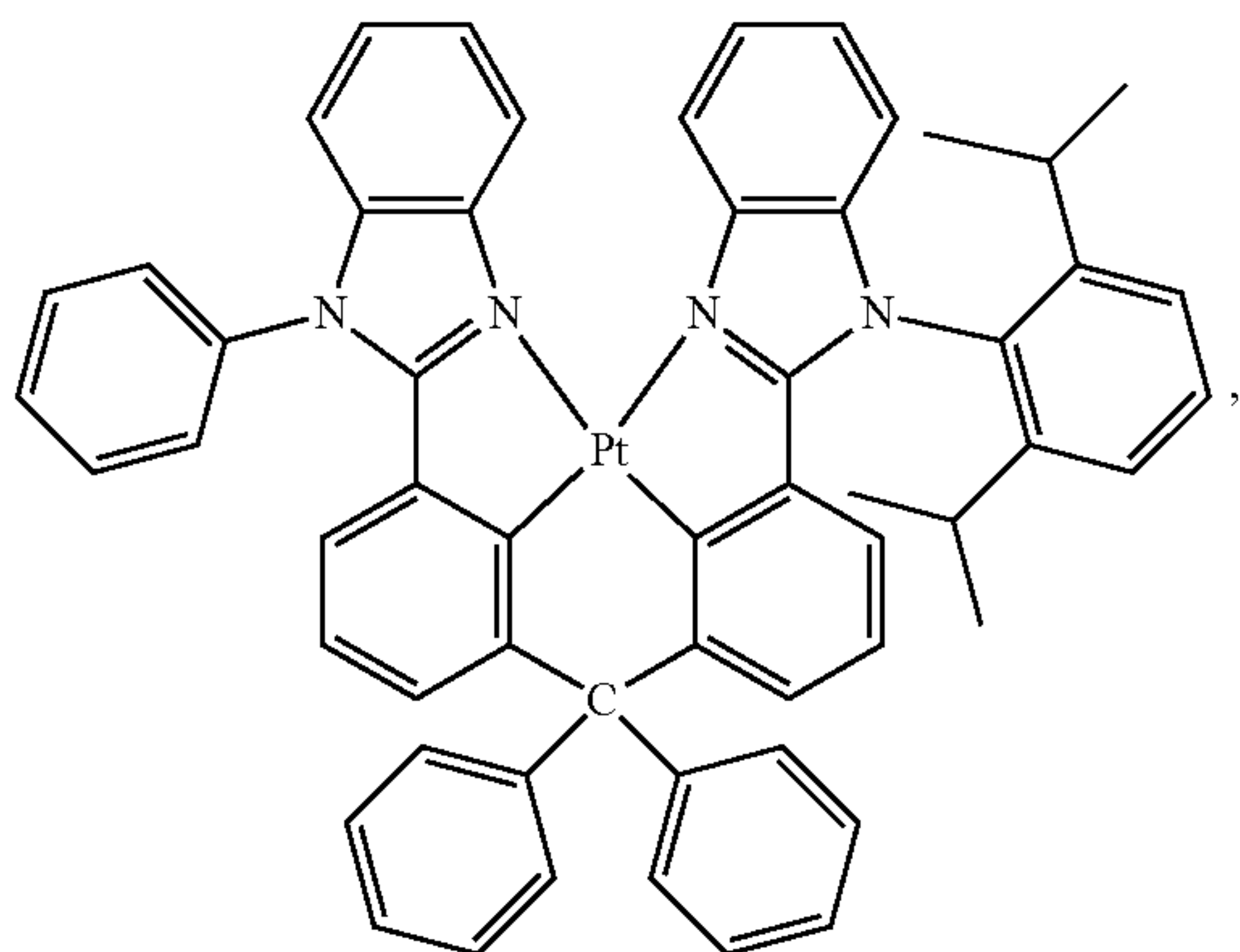
Compound 114
