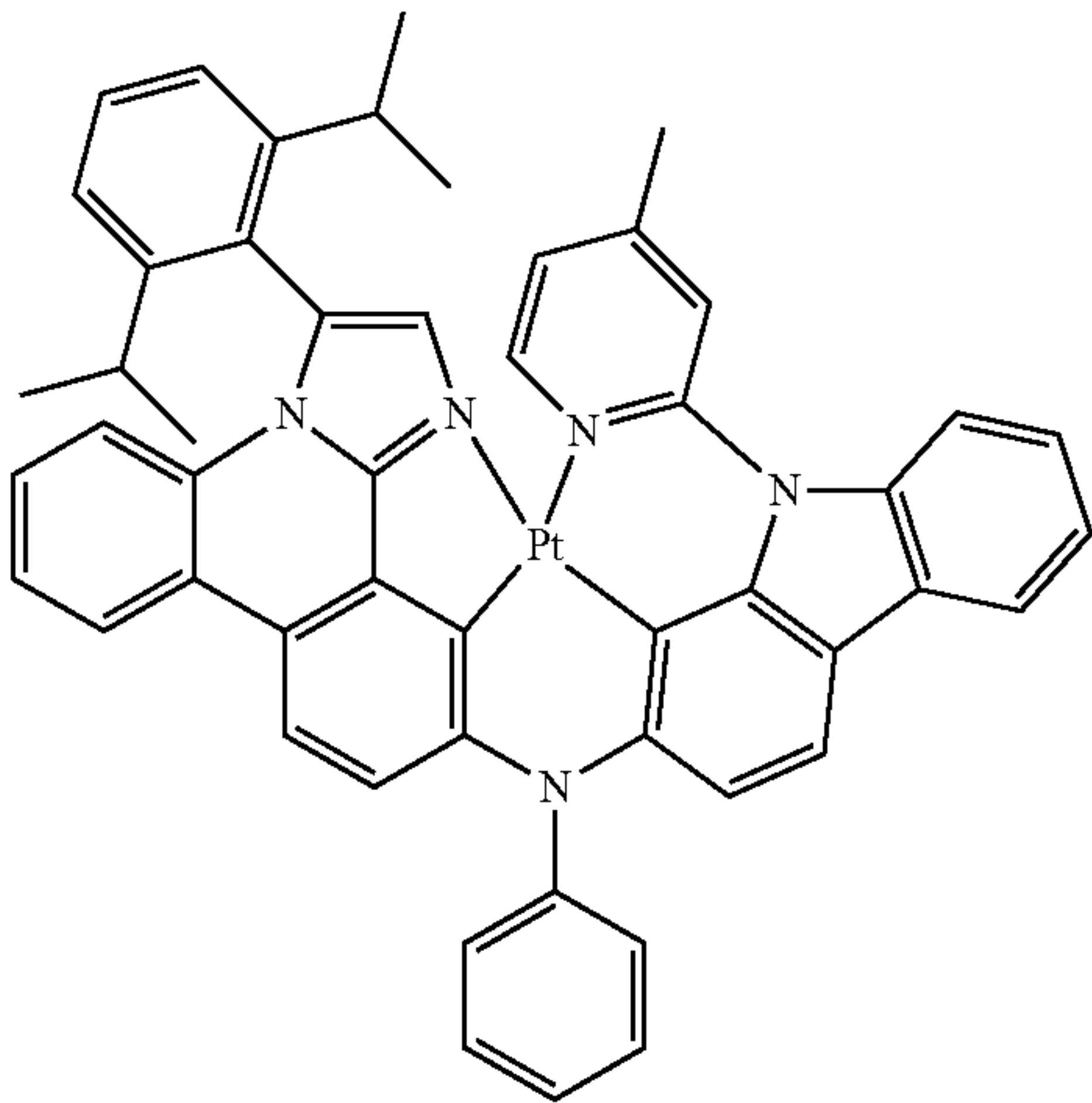
Compound 19'
