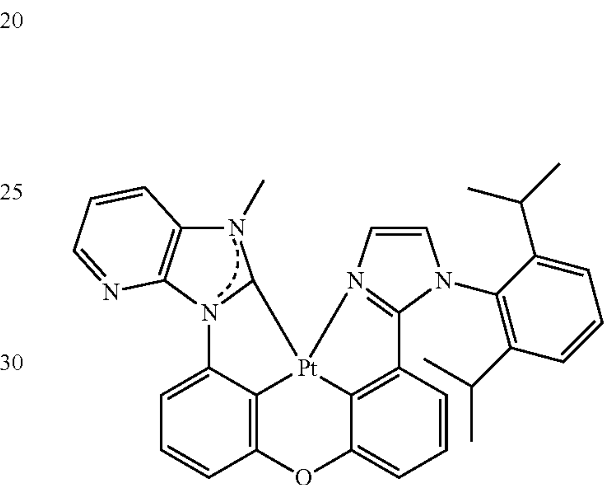
Compound 148
