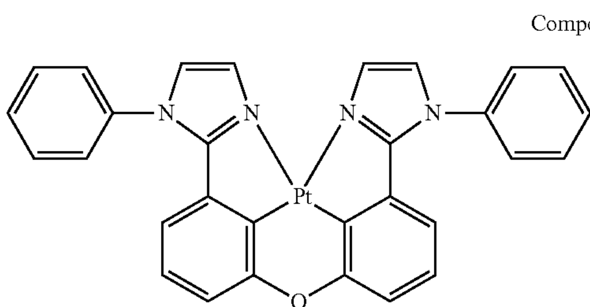
Compound E
