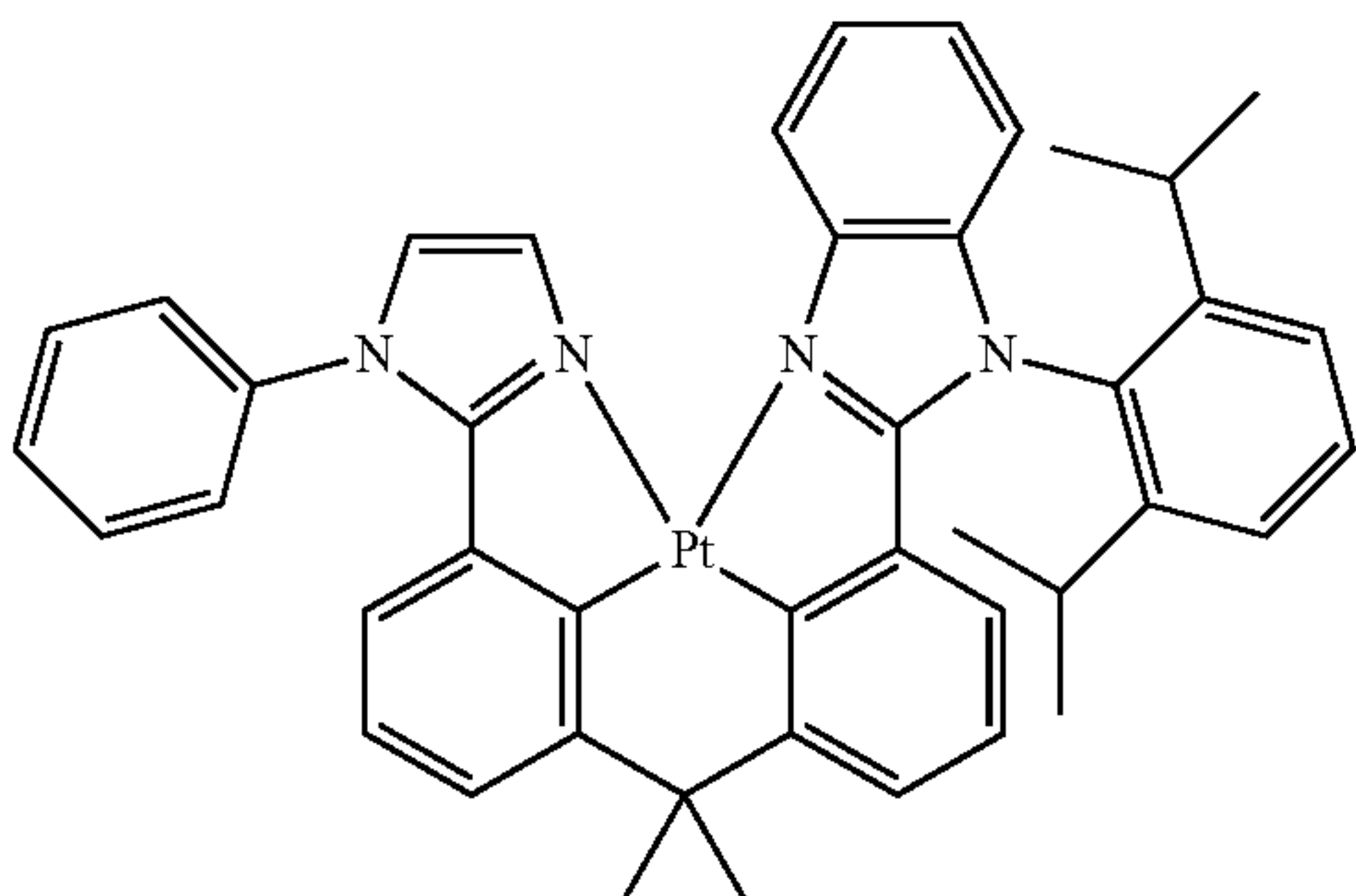
Compound 105
