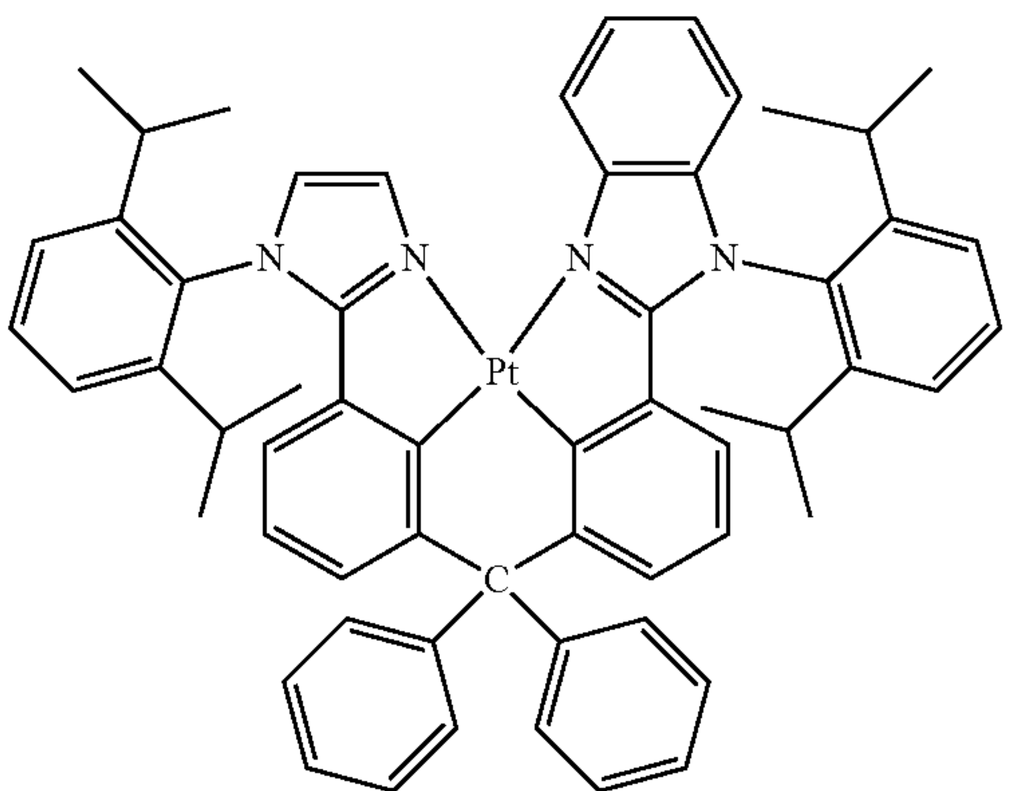
Compound 26
