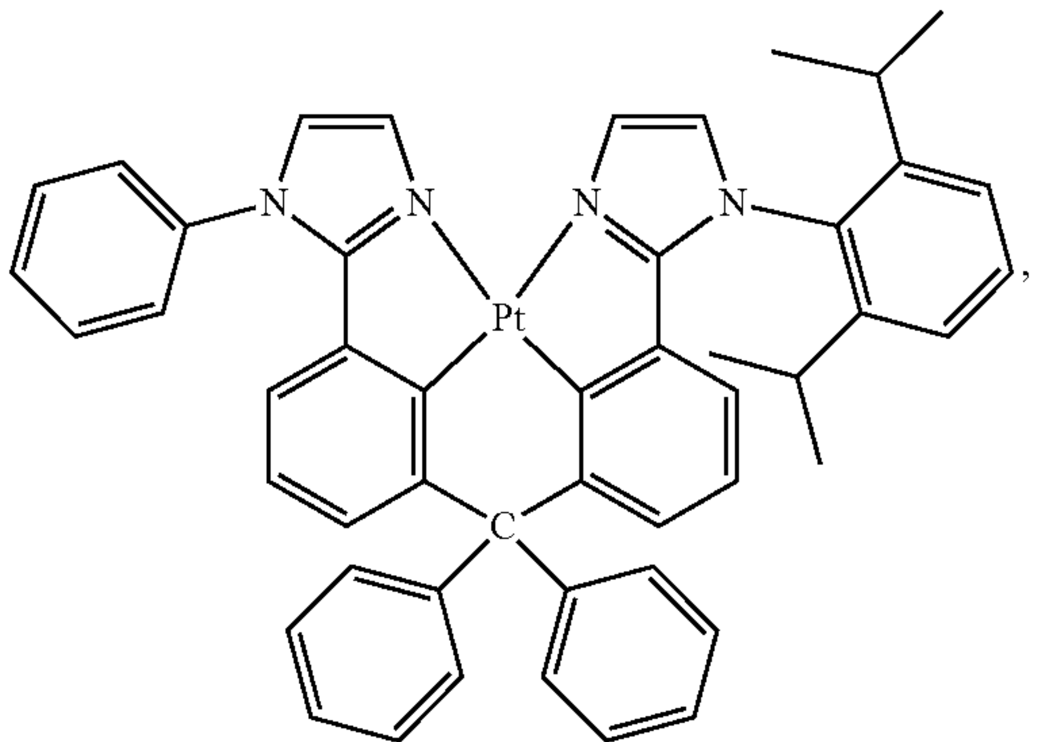
Compound 63
