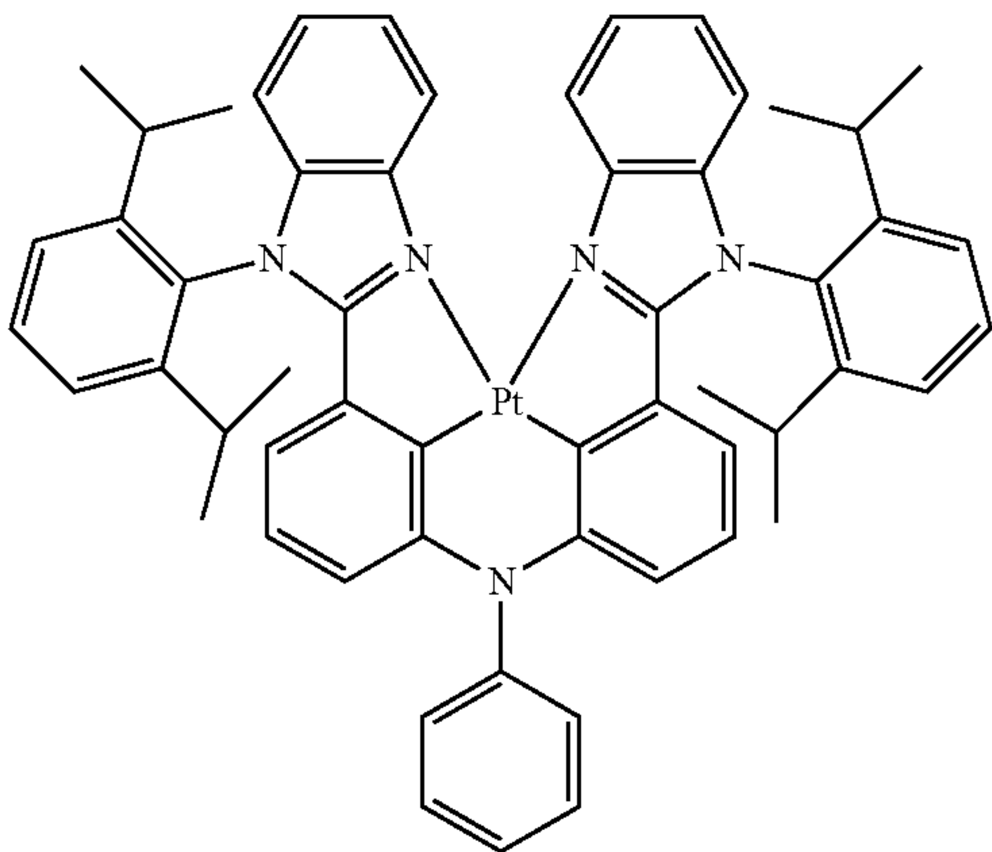
Compound 11
