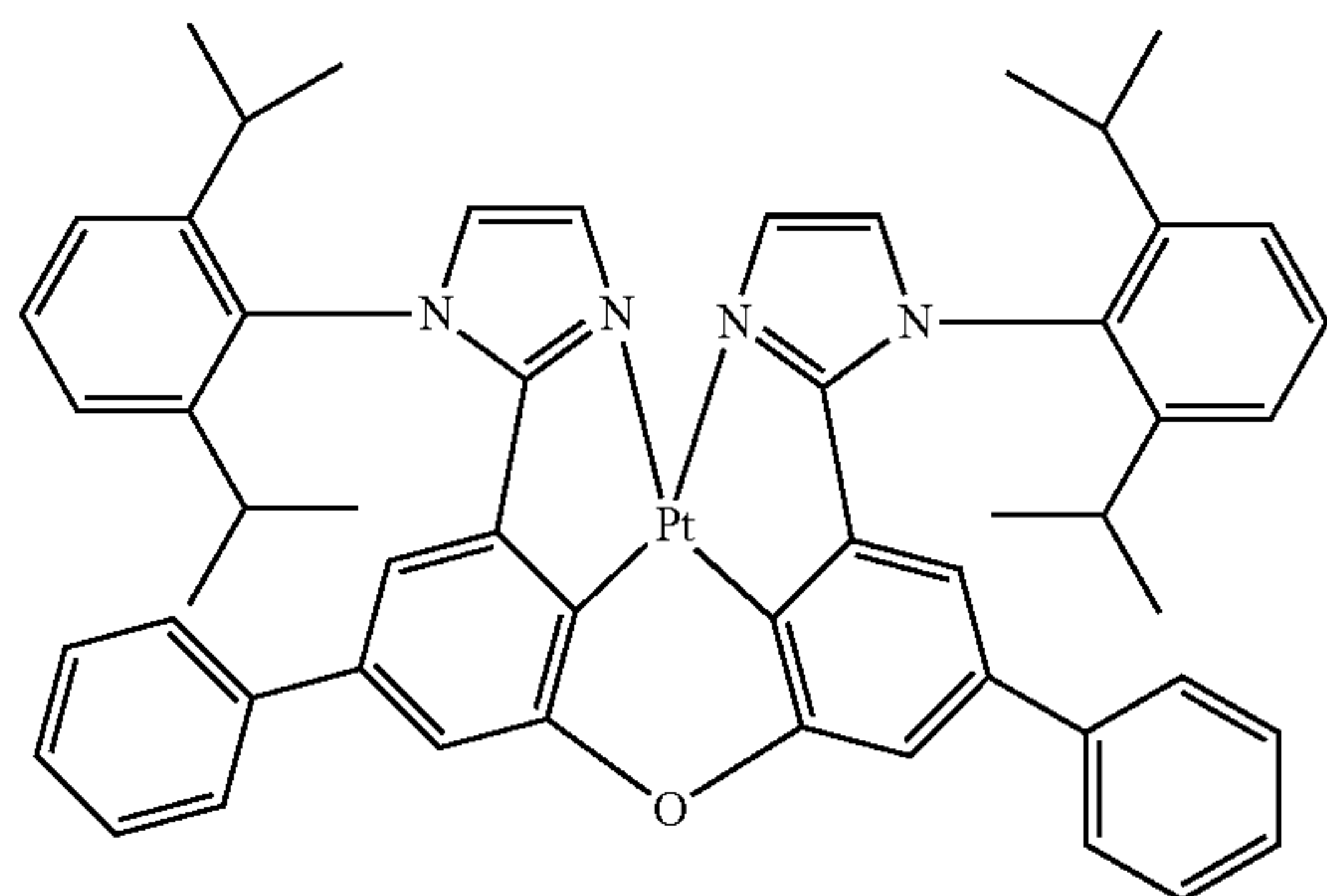
Compound 163
