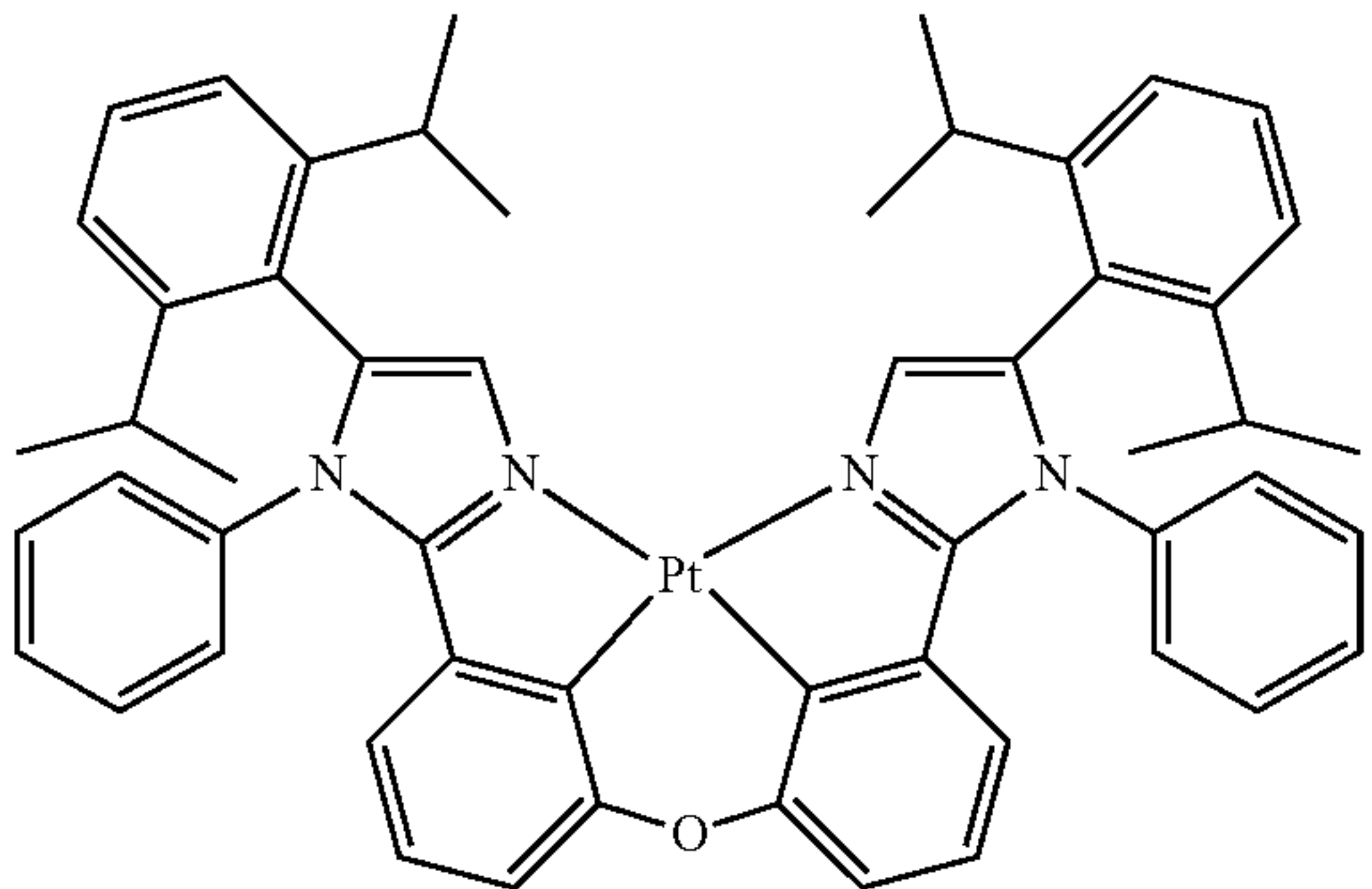
Compound 119
