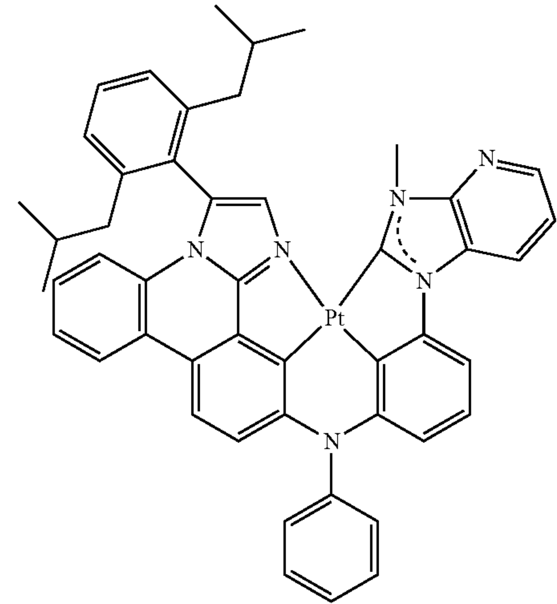
Compound 193'
