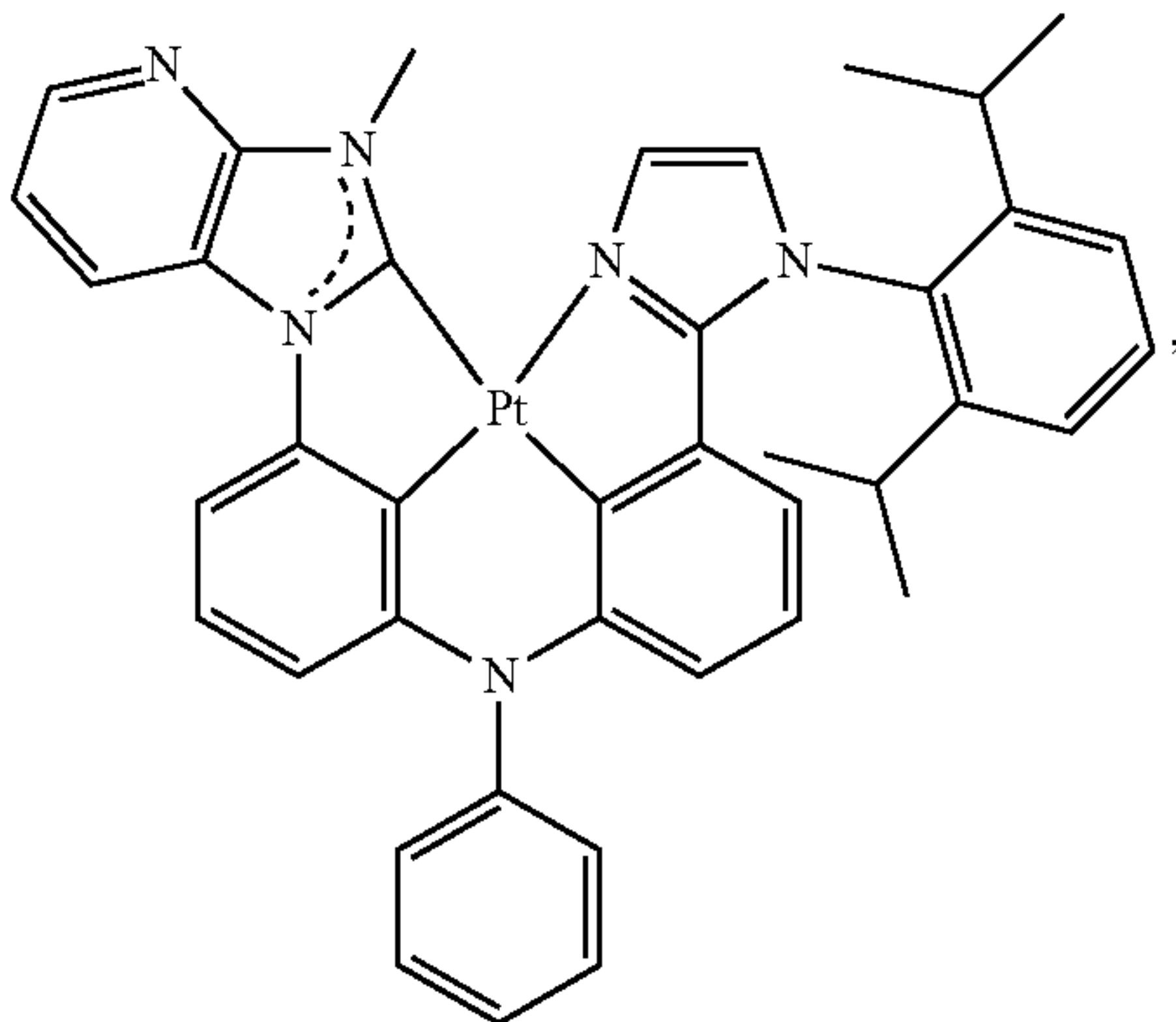
Compound 154
