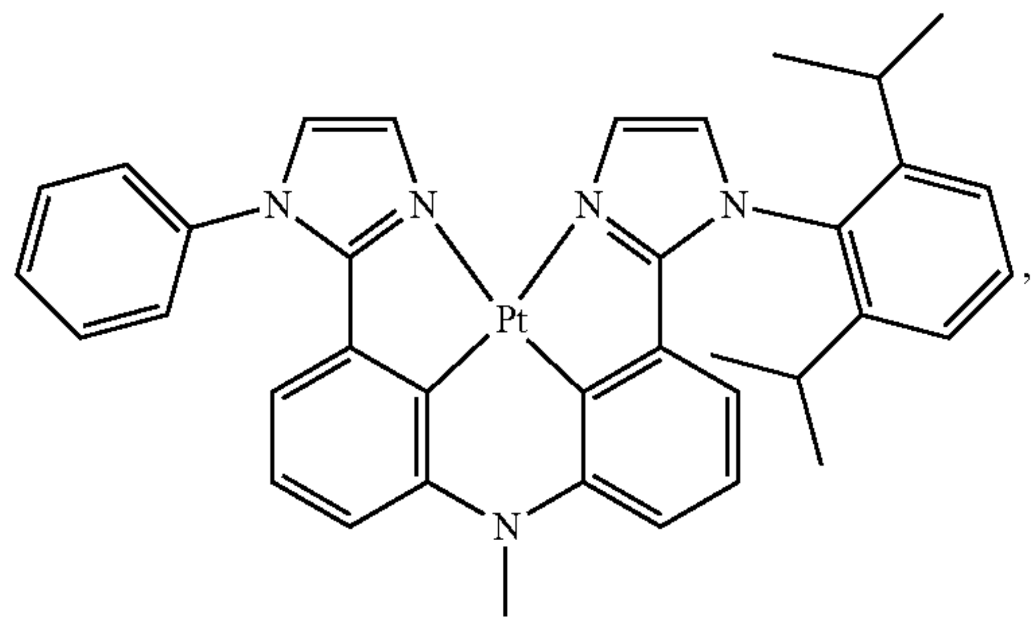
Compound 58
