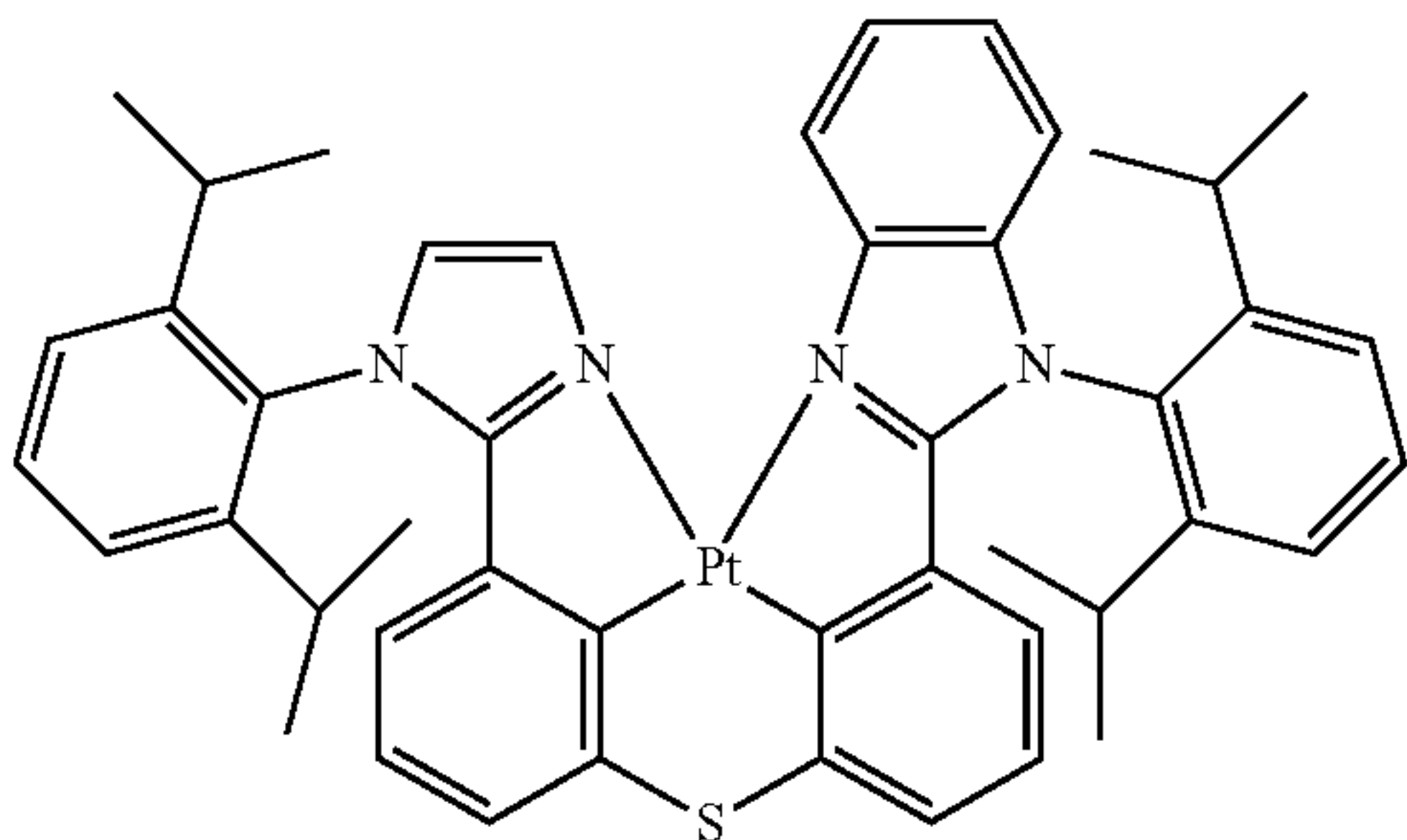
Compound 24
