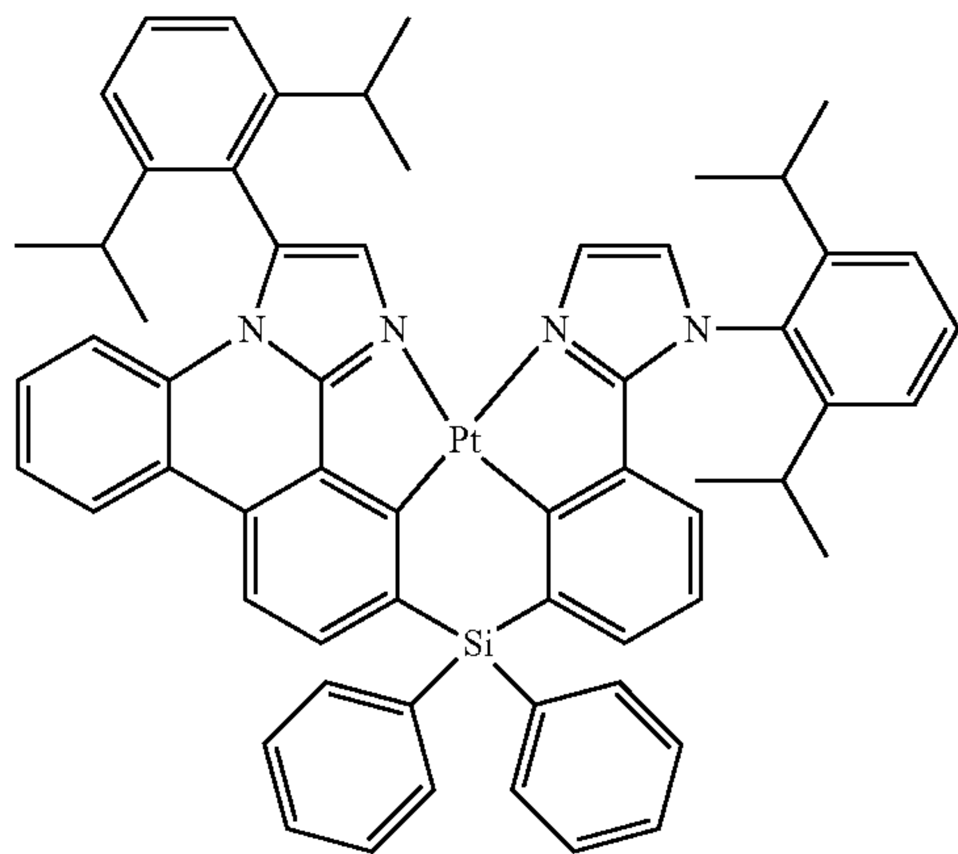
Compound 111'
