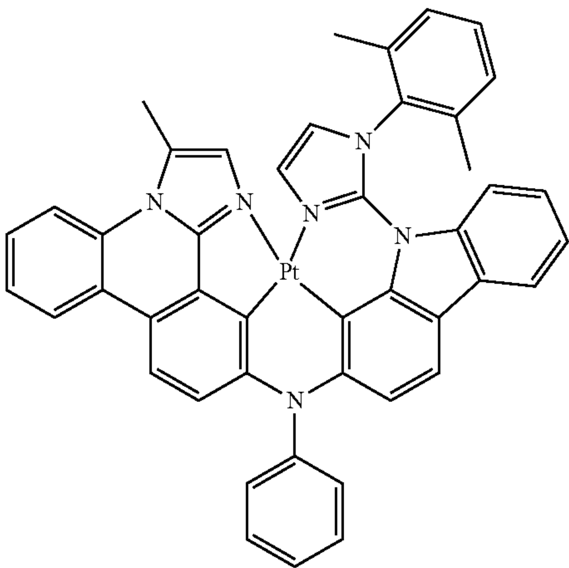
Compound 134'
