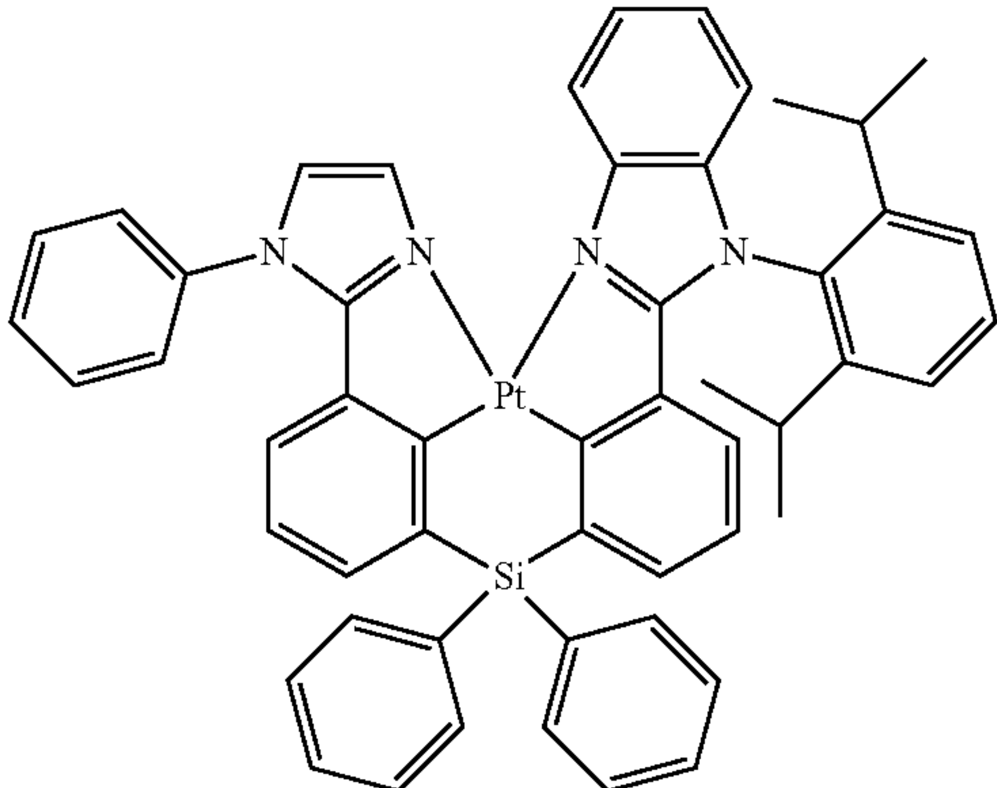
Compound 109
