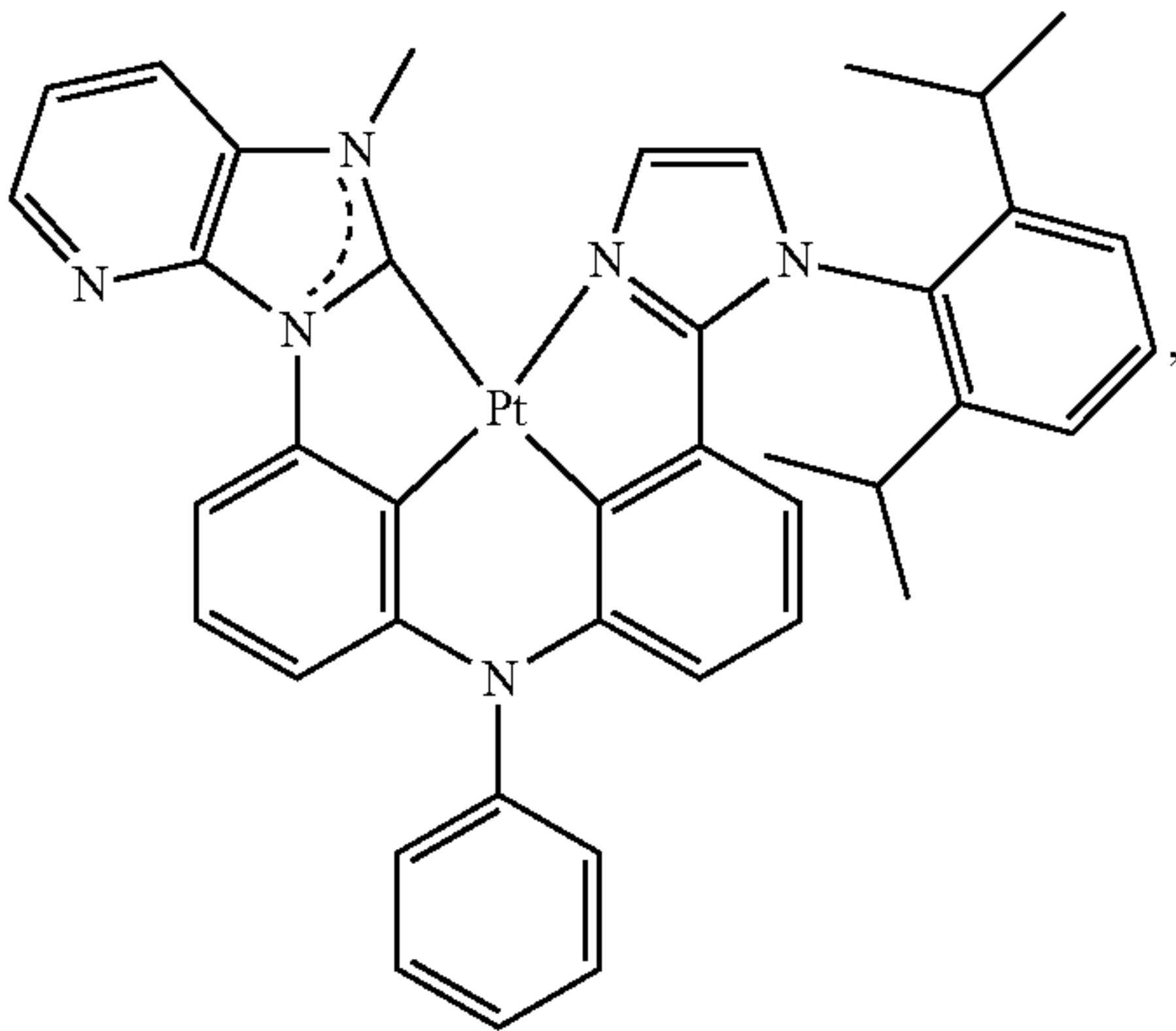
Compound 147
