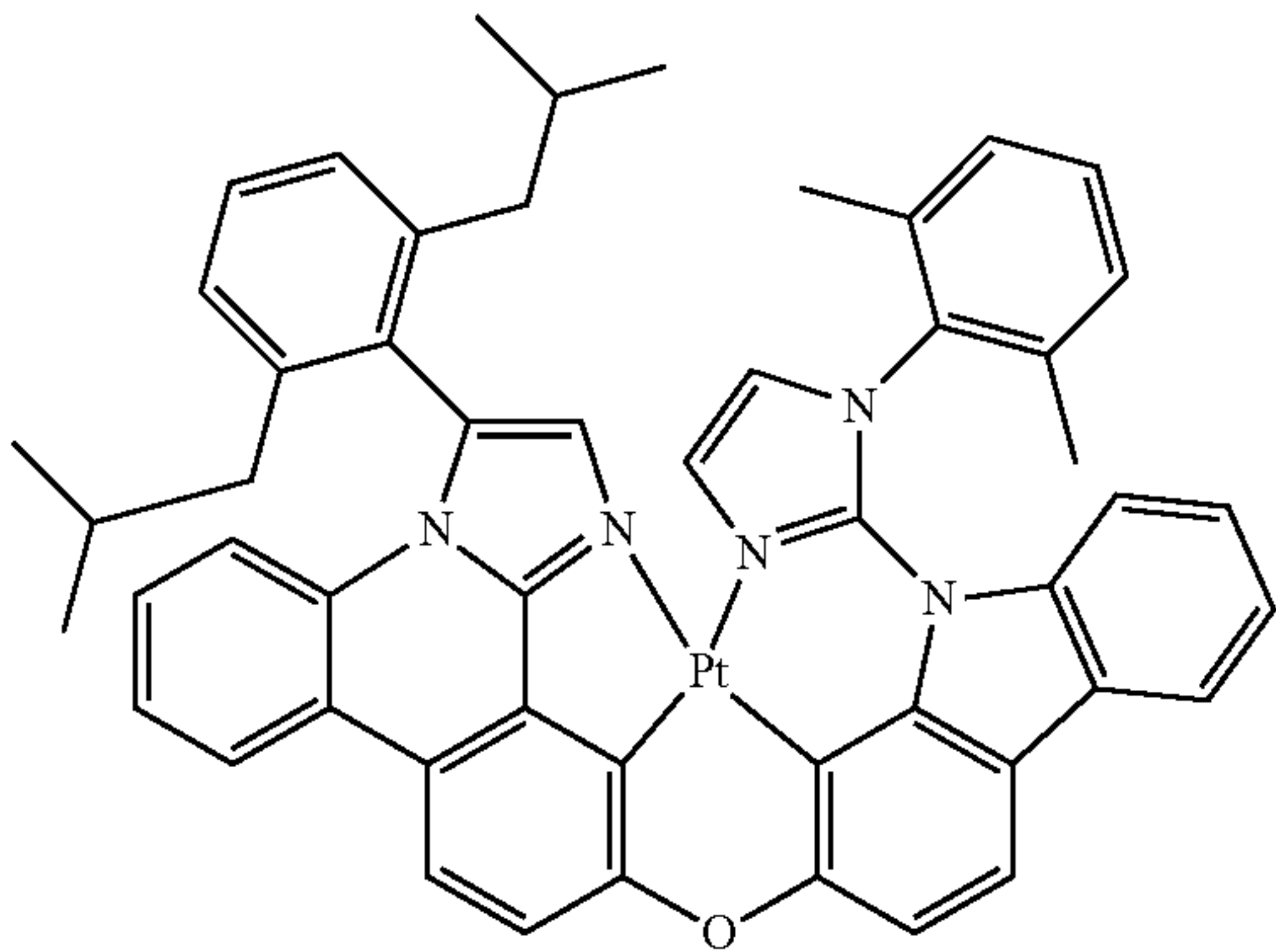
Compound 127'
