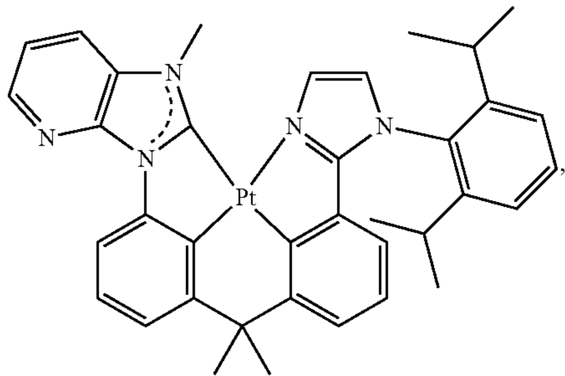
Compound 150
