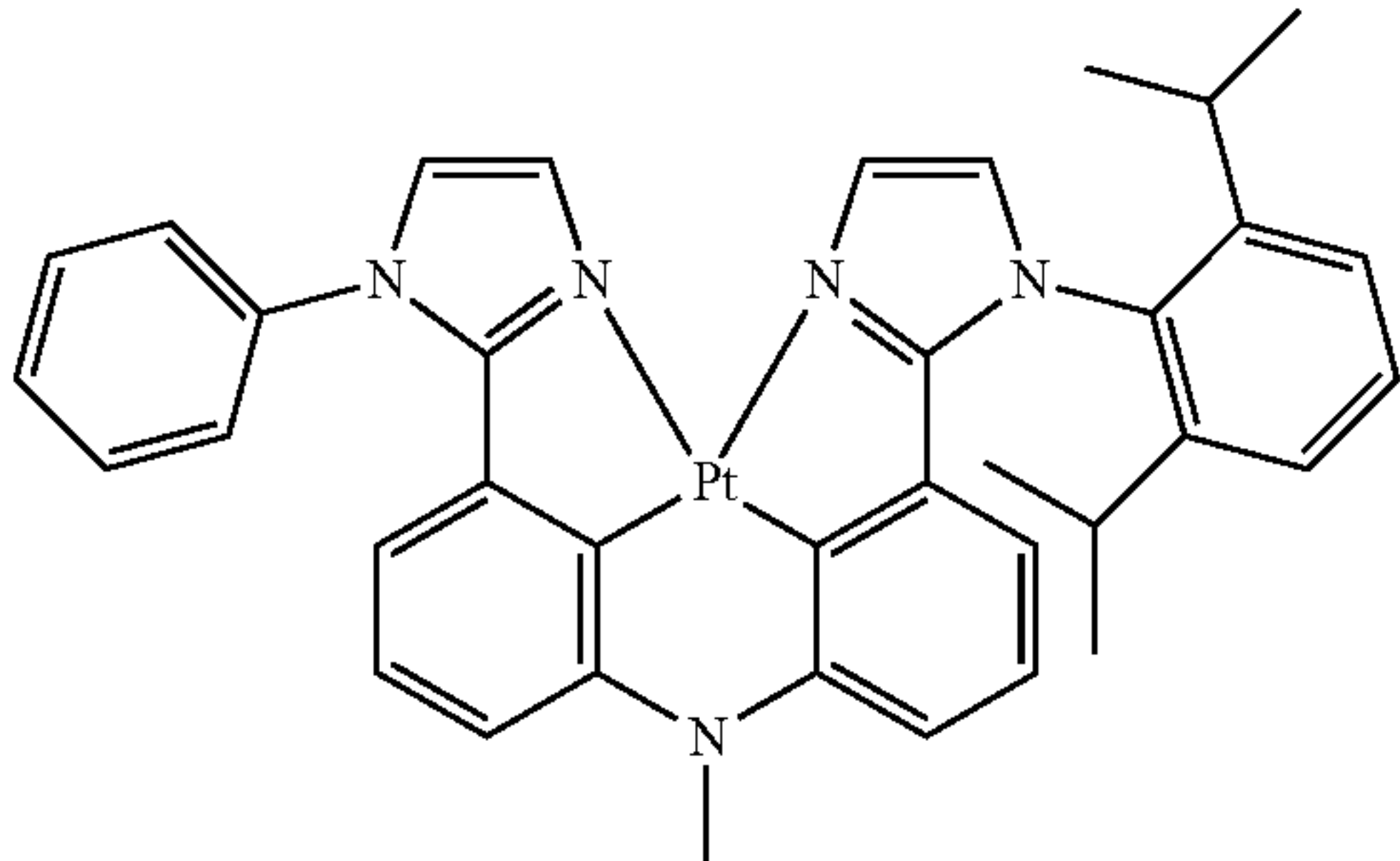
Compound 58
