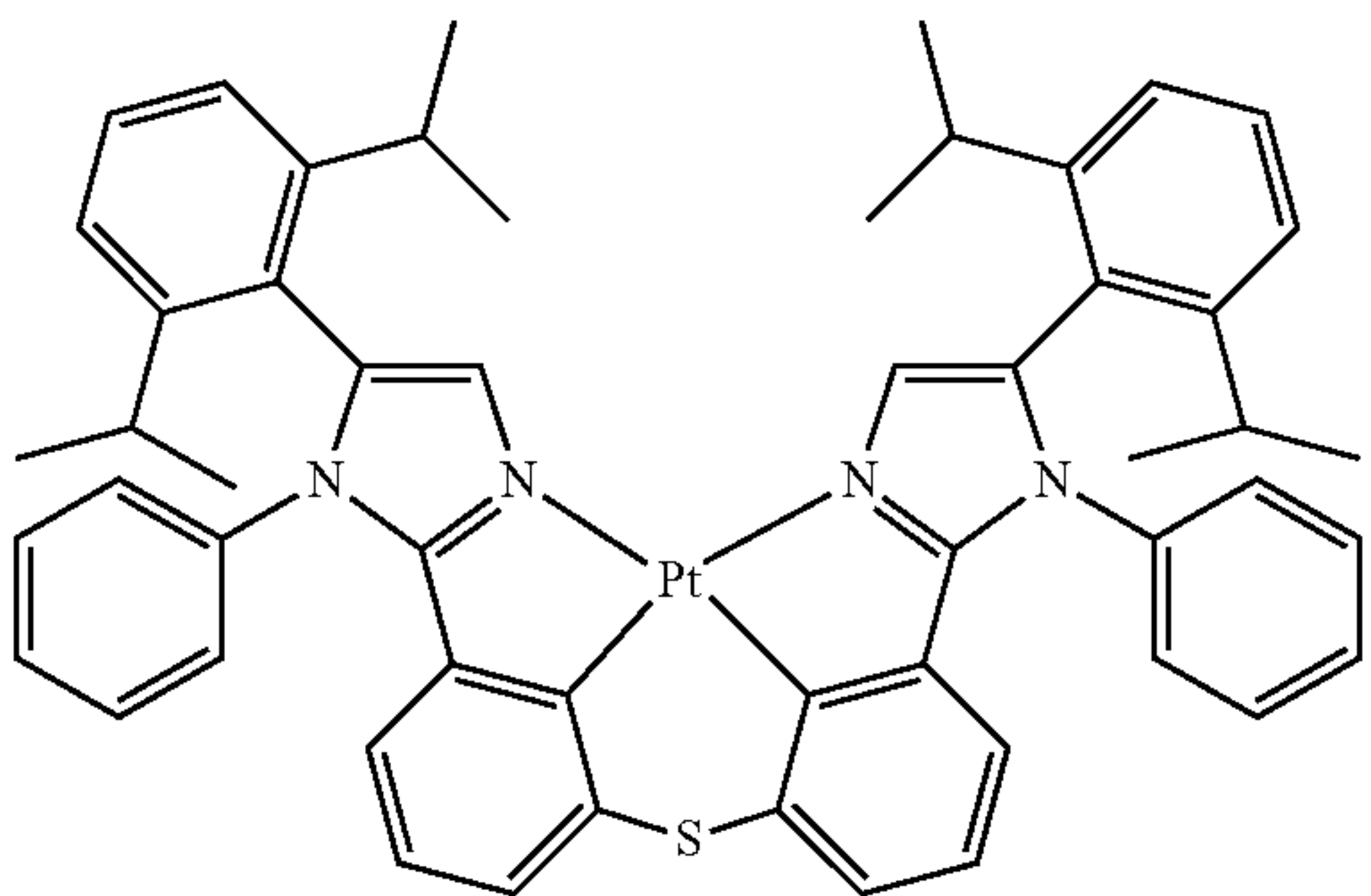
Compound 121
