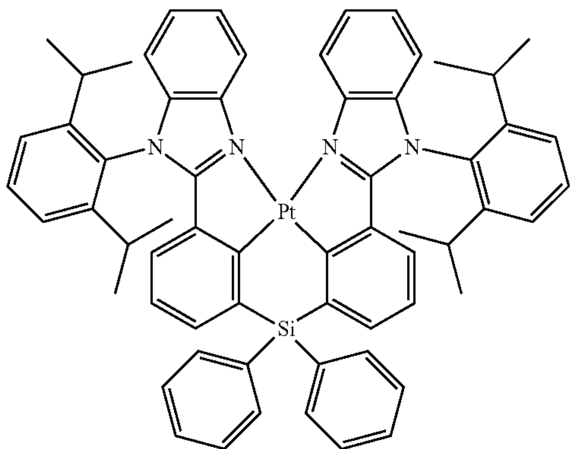
Compound 20
