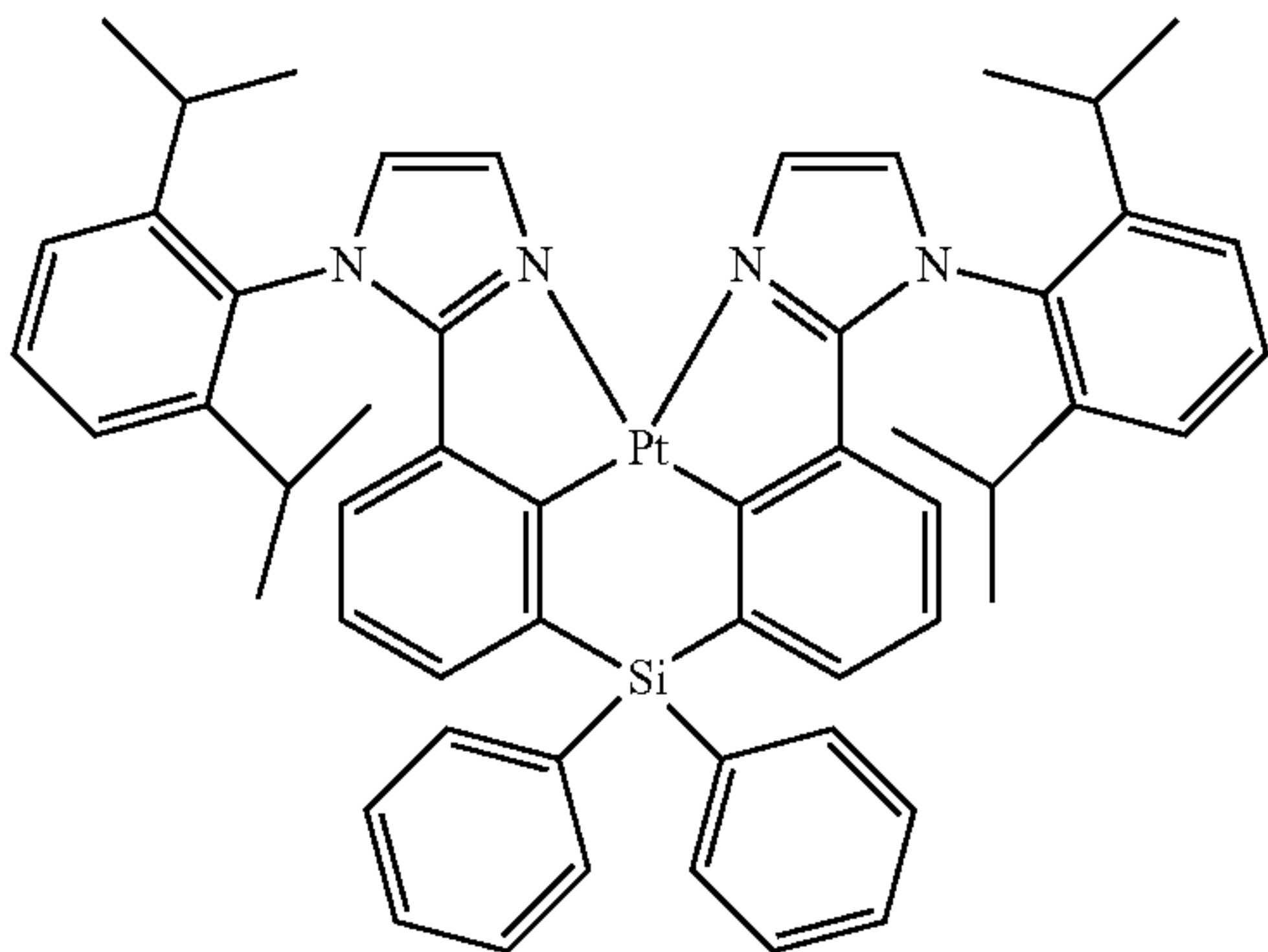
Compound 10
