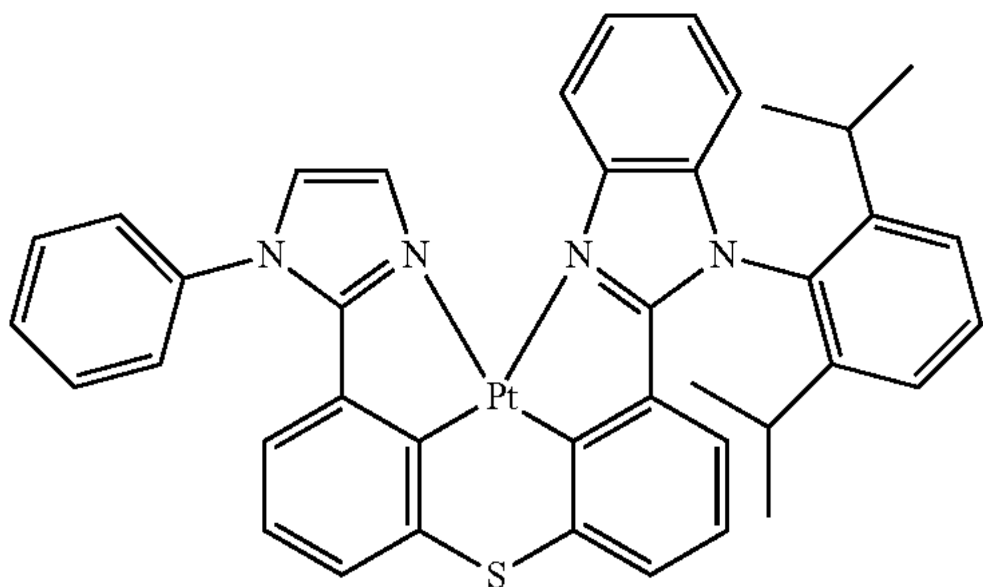
Compound 104
