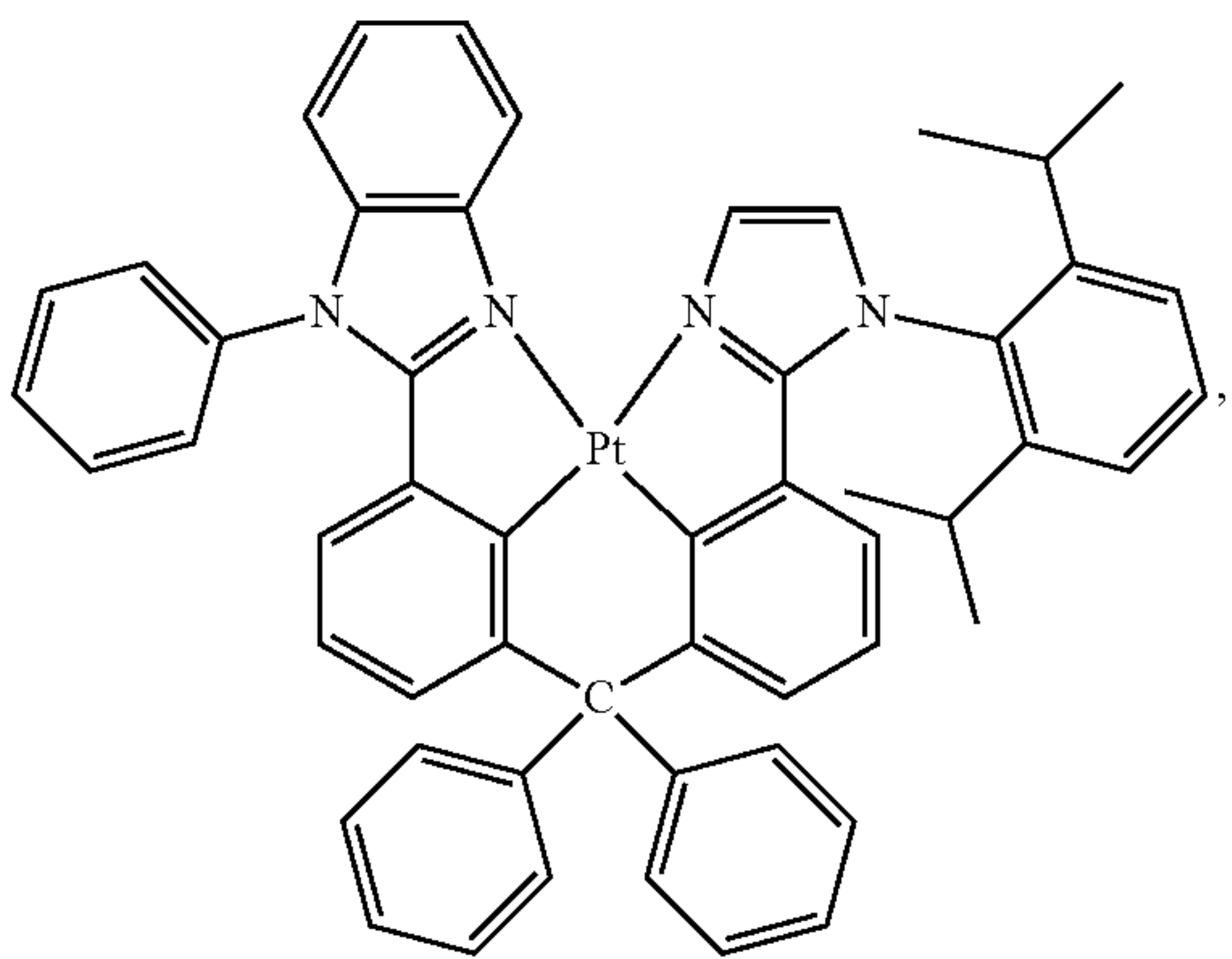
Compound 70
