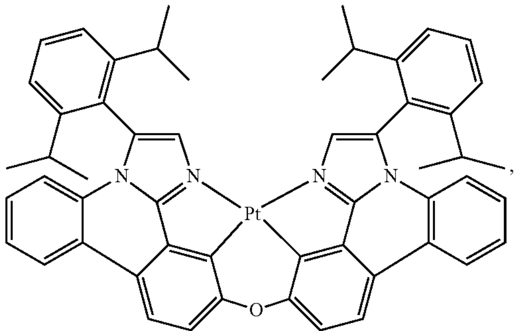
Compound 127
