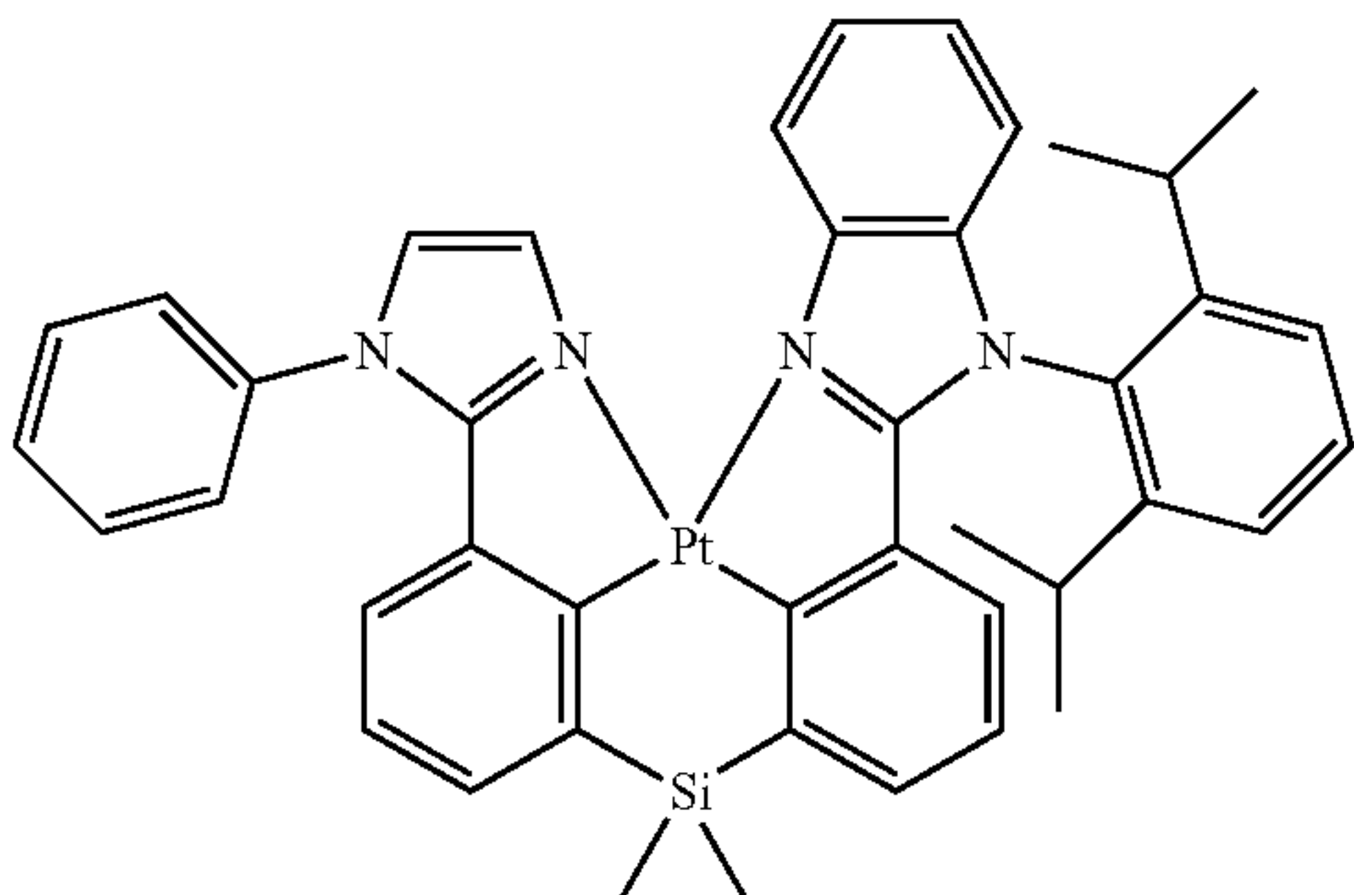
Compound 107
