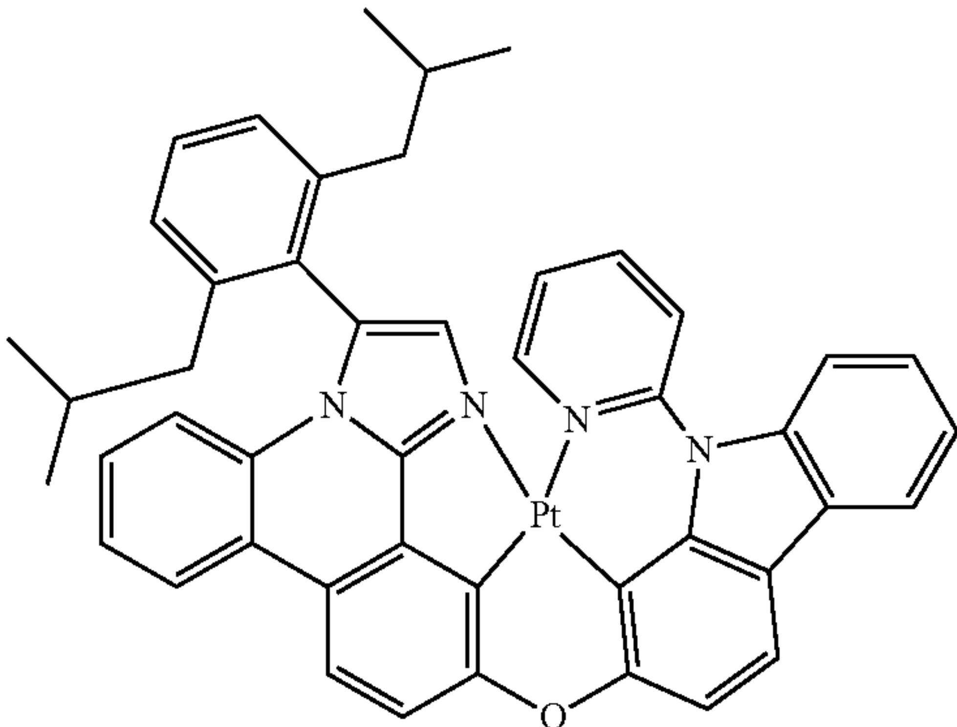
Compound 8'
