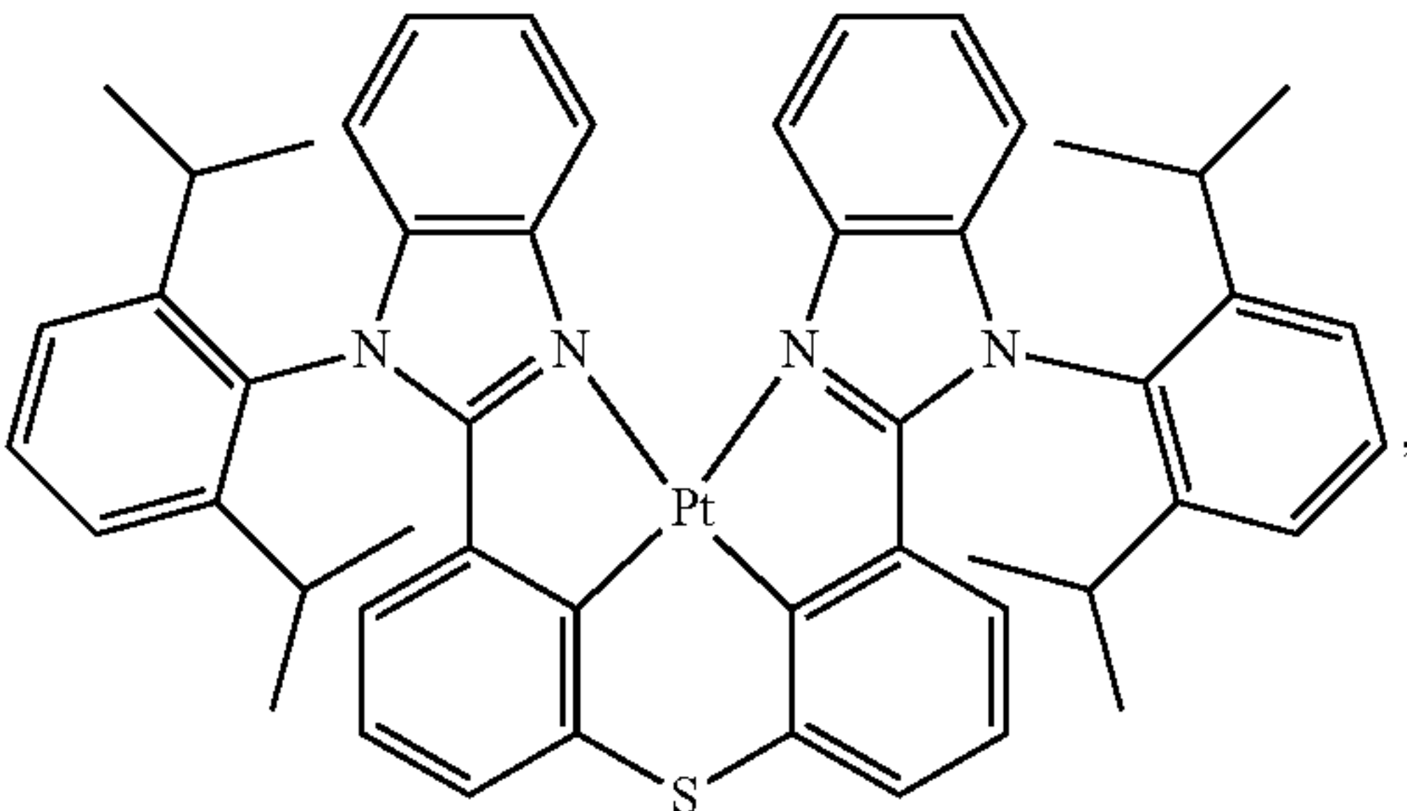
Compound 15
