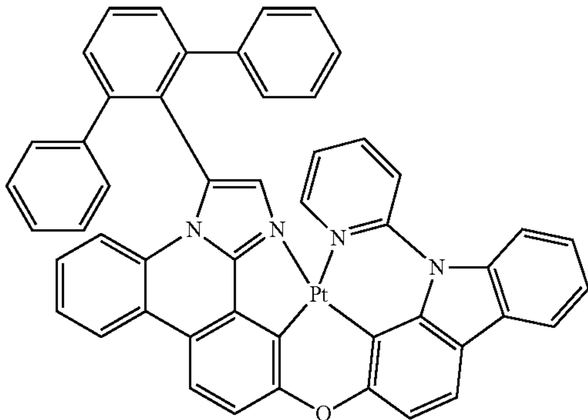
Compound 14'
