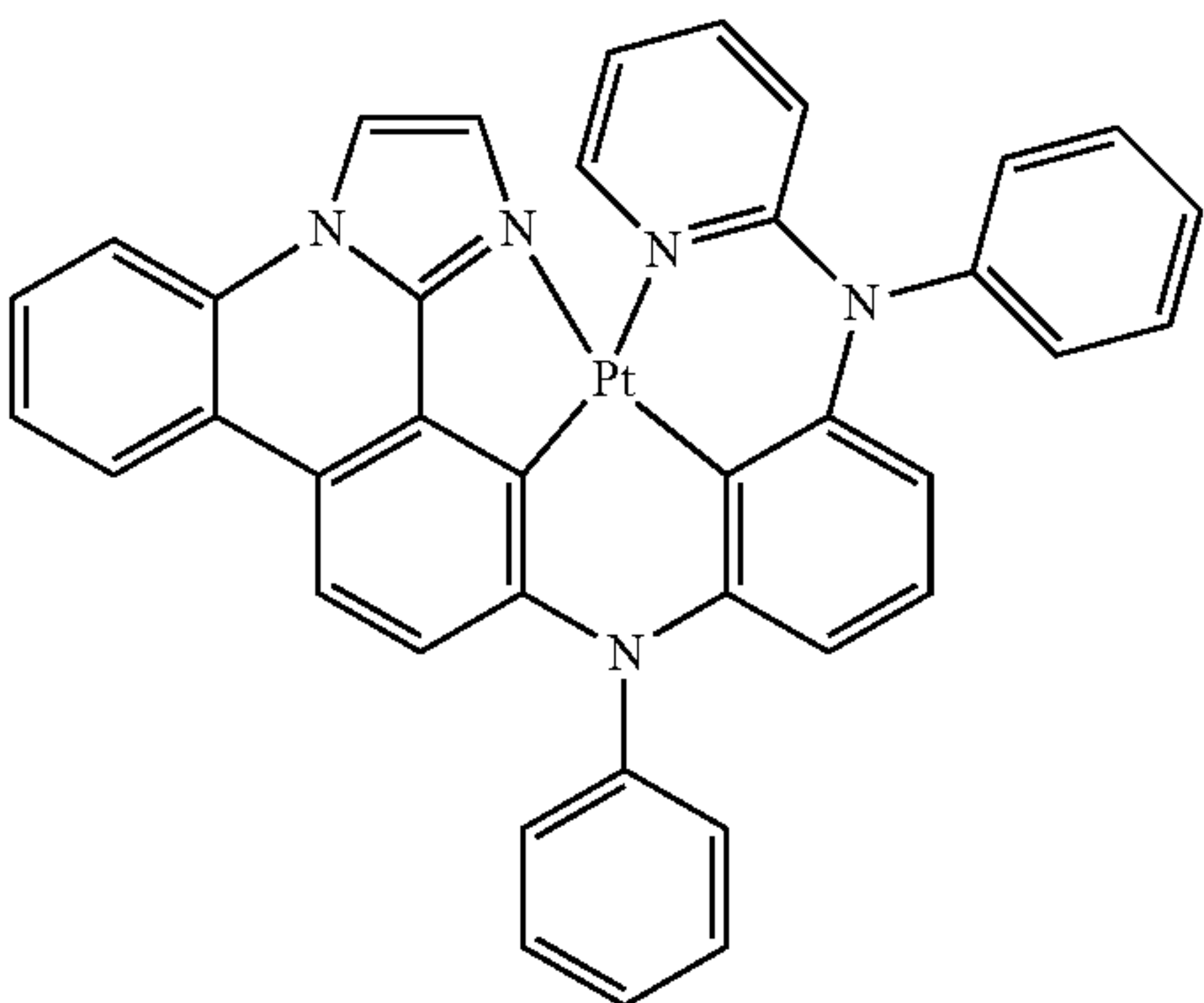
Compound 52'
