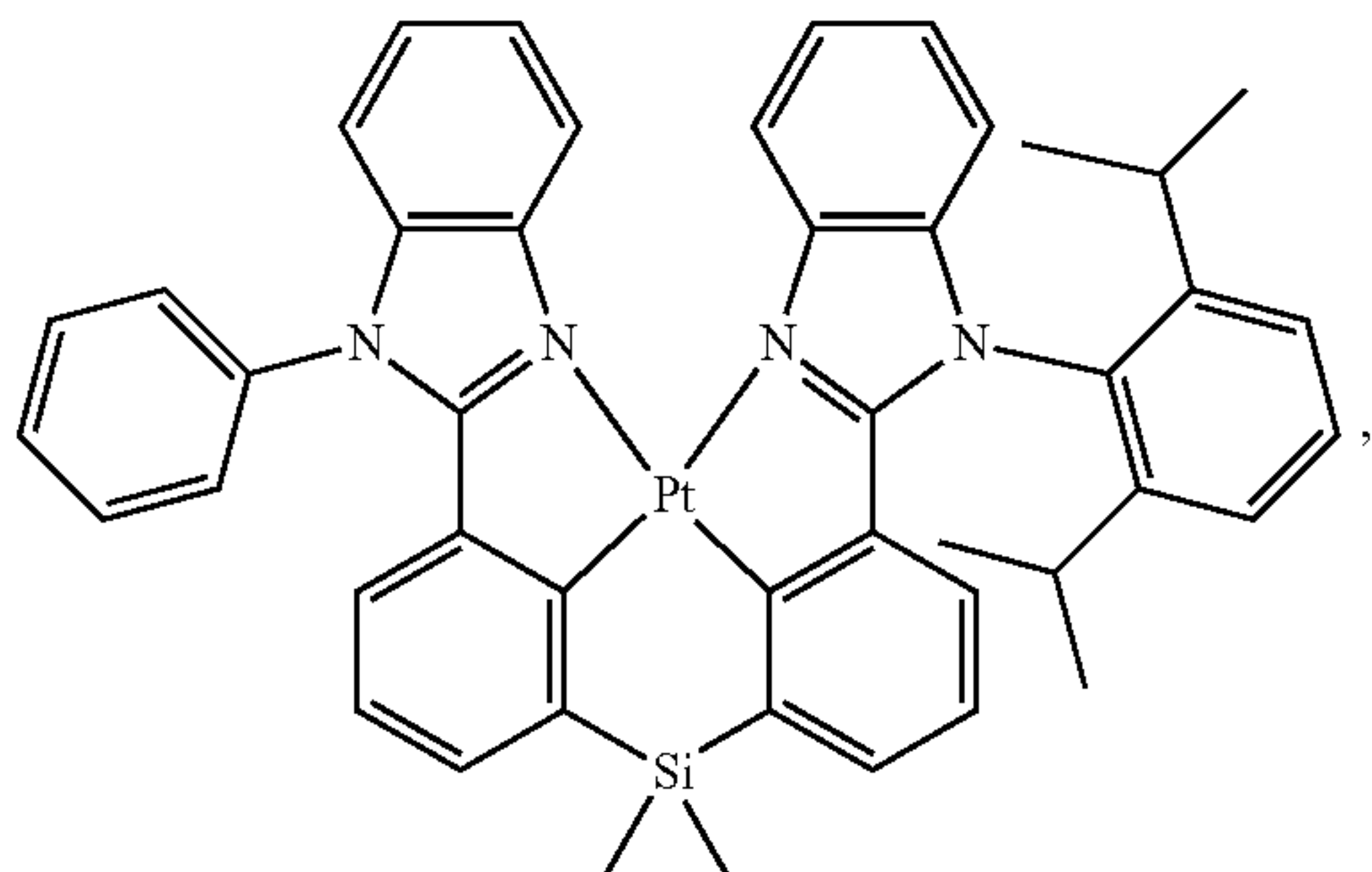
Compound 115
