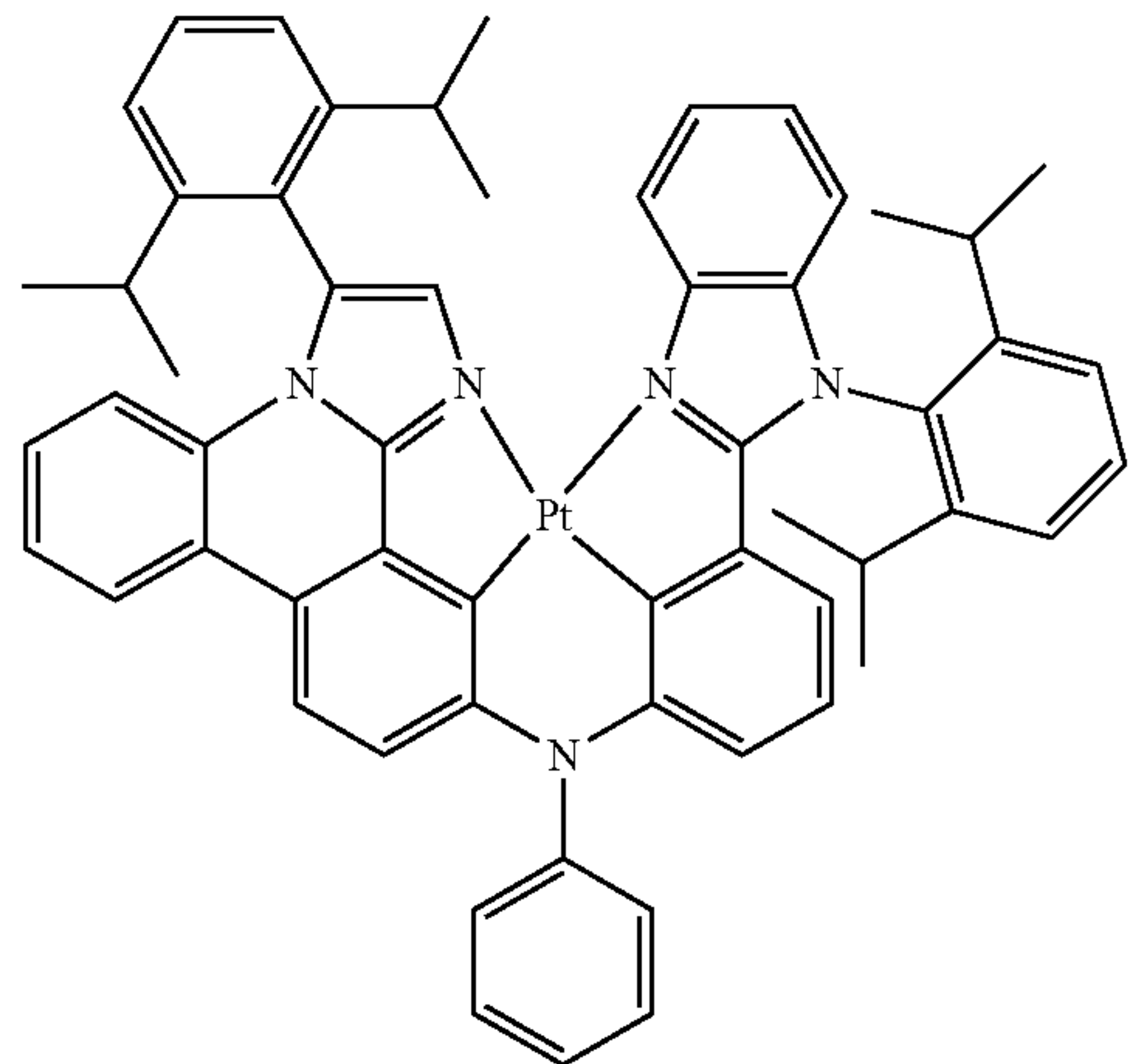
Compound 116'
