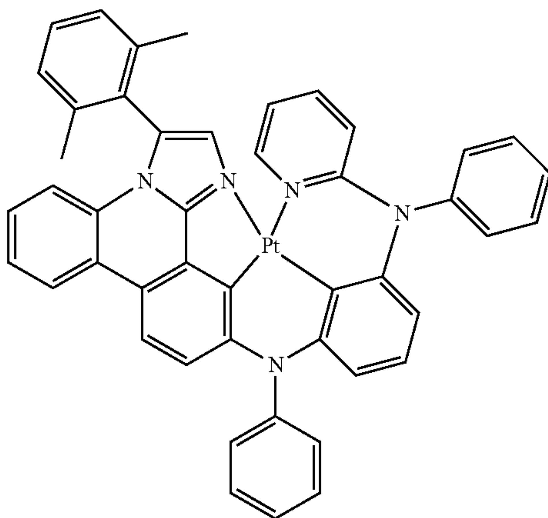
Compound 53'
