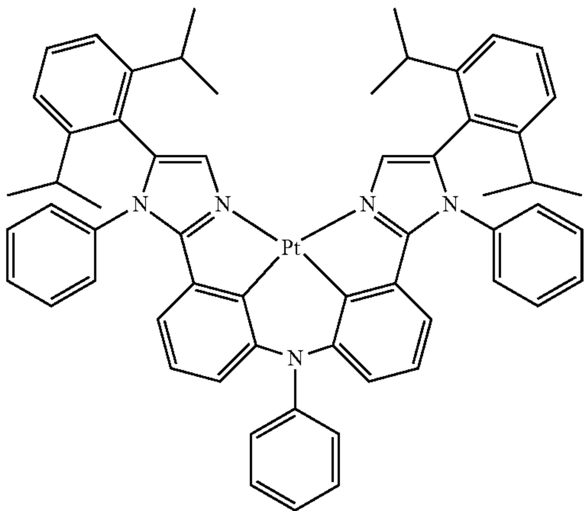
Compound 118
