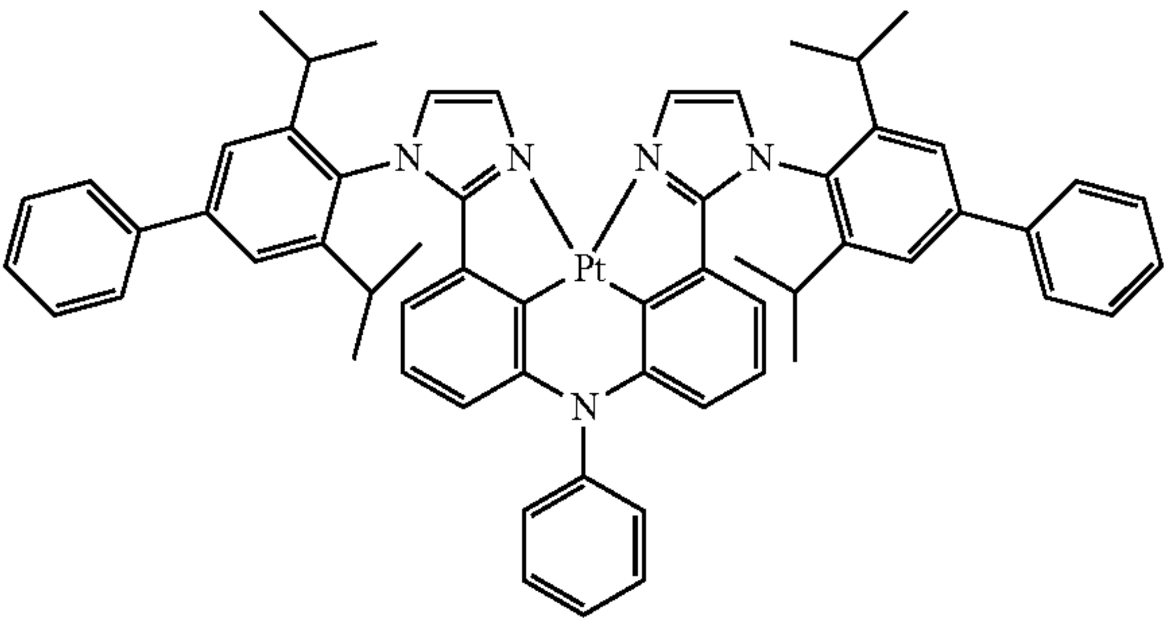
Compound 3
