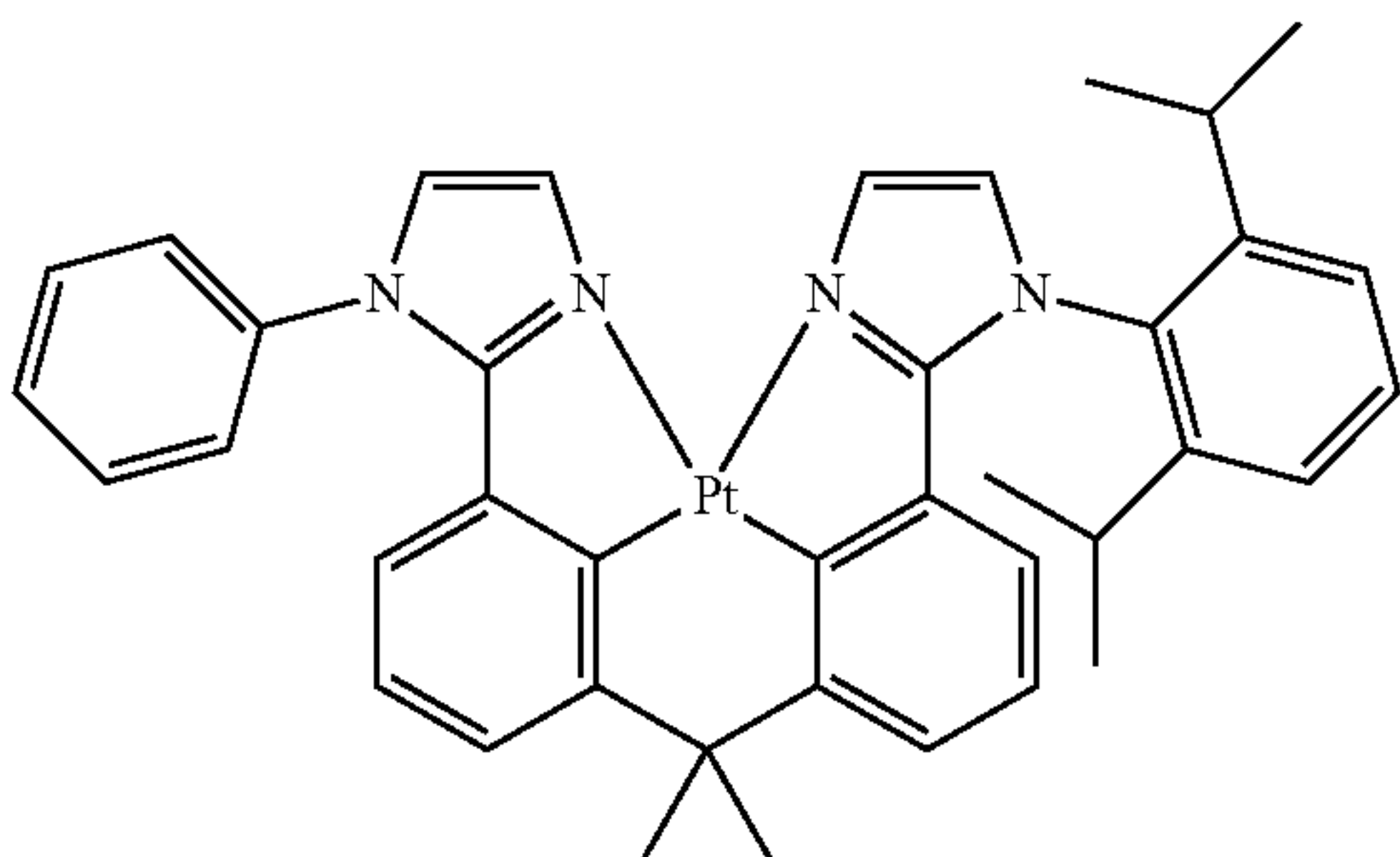
Compound 62
