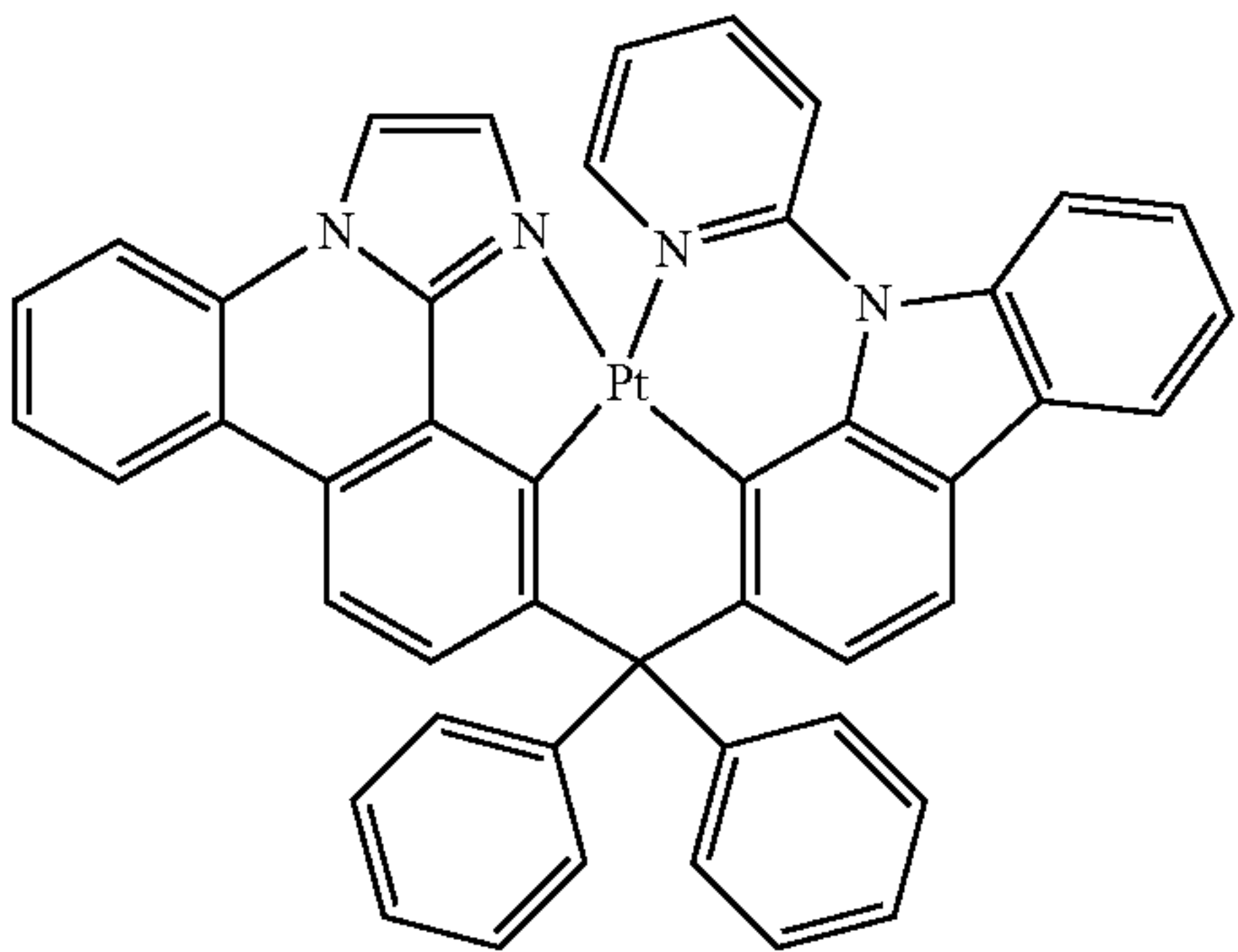
Compound 40'
