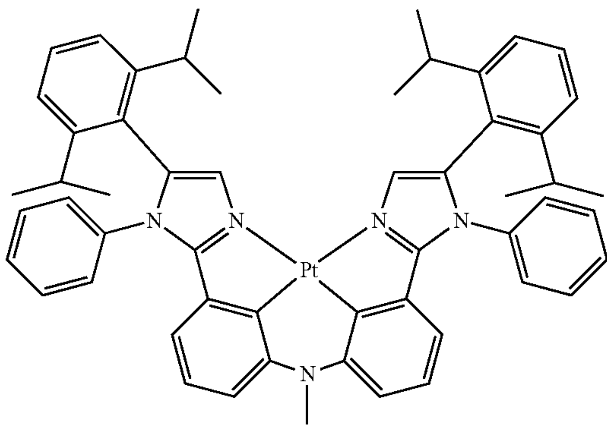
Compound 119
