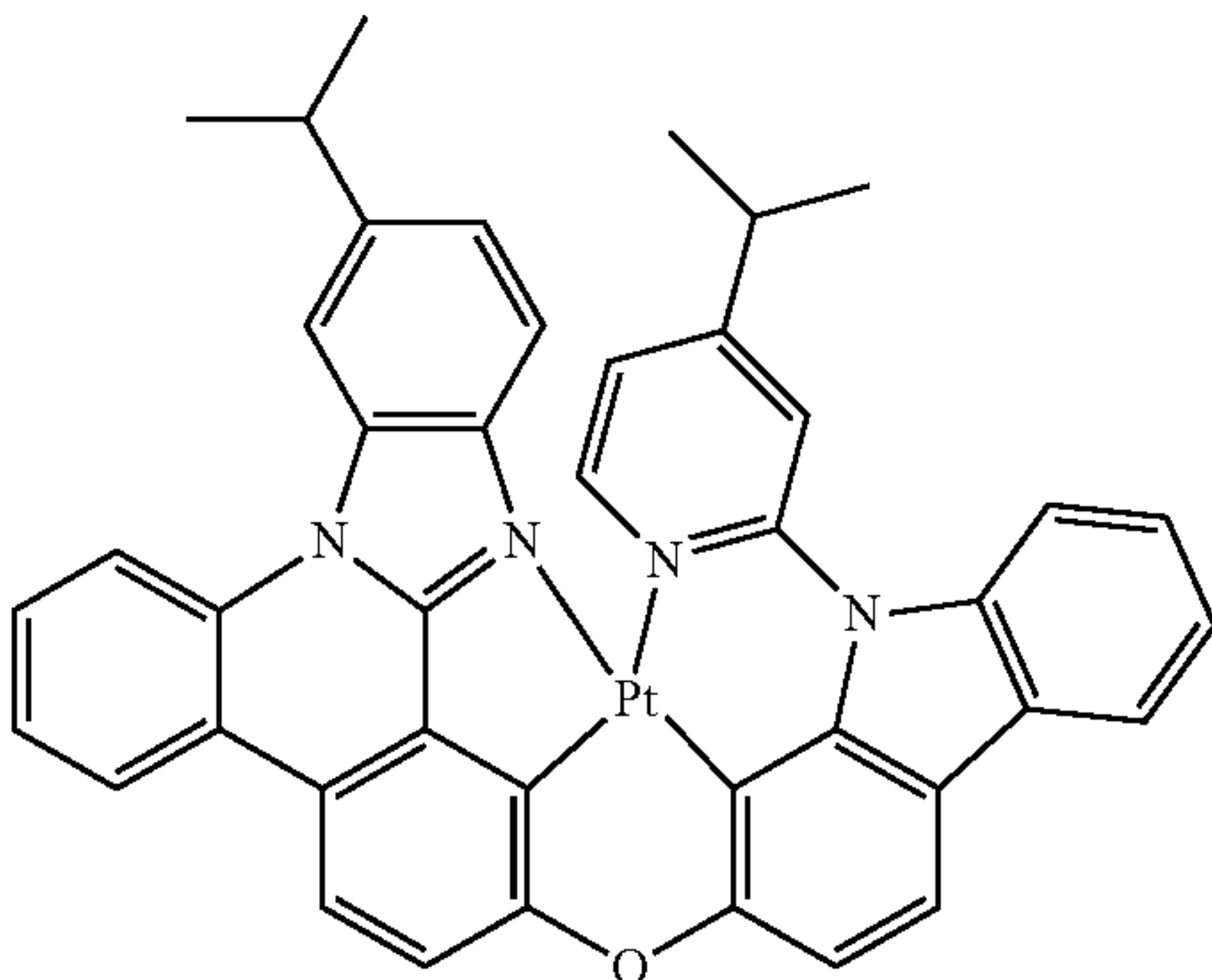
Compound 216'
