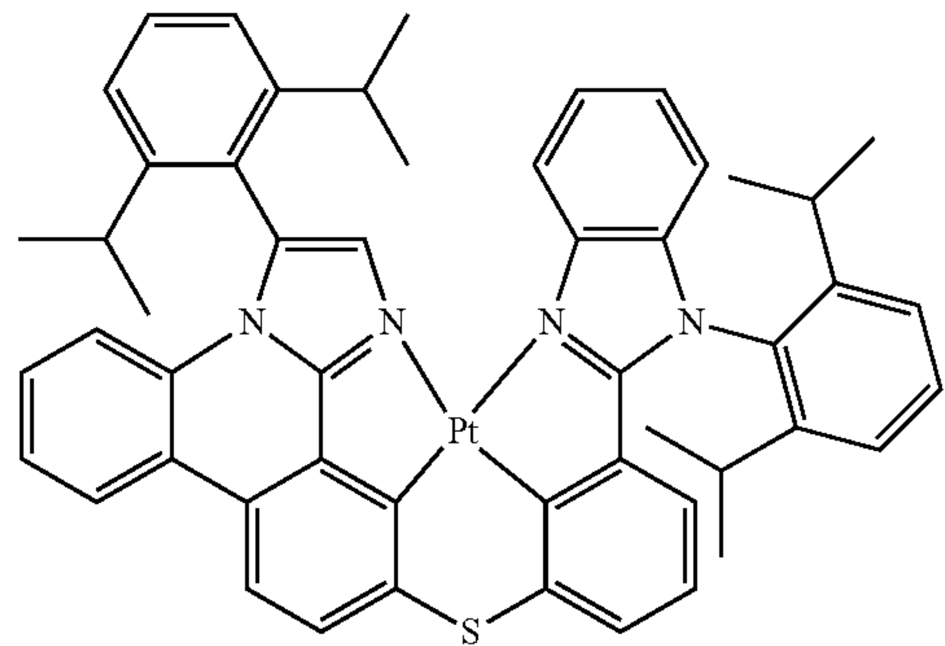
Compound 113'
