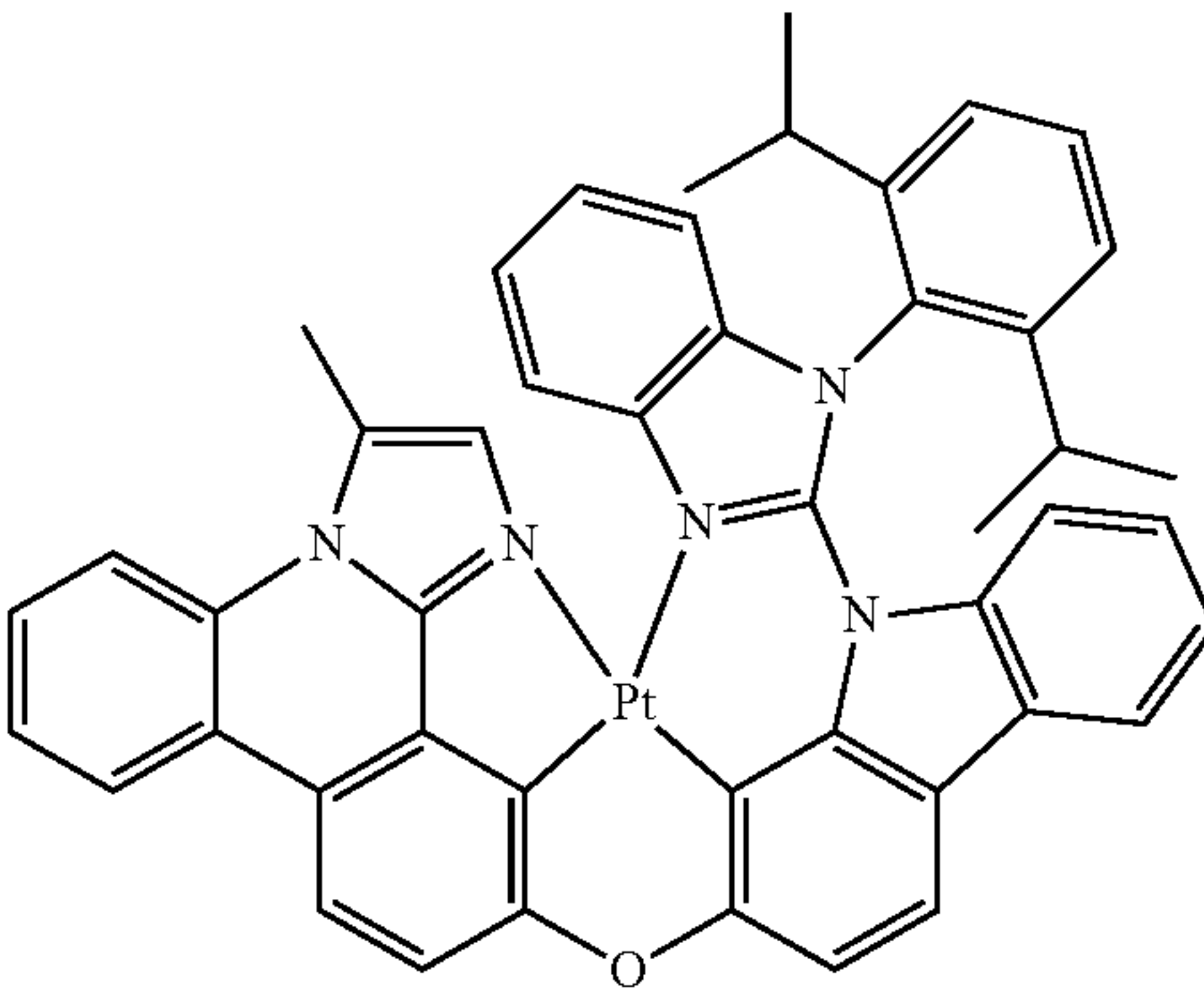
Compound 238'
