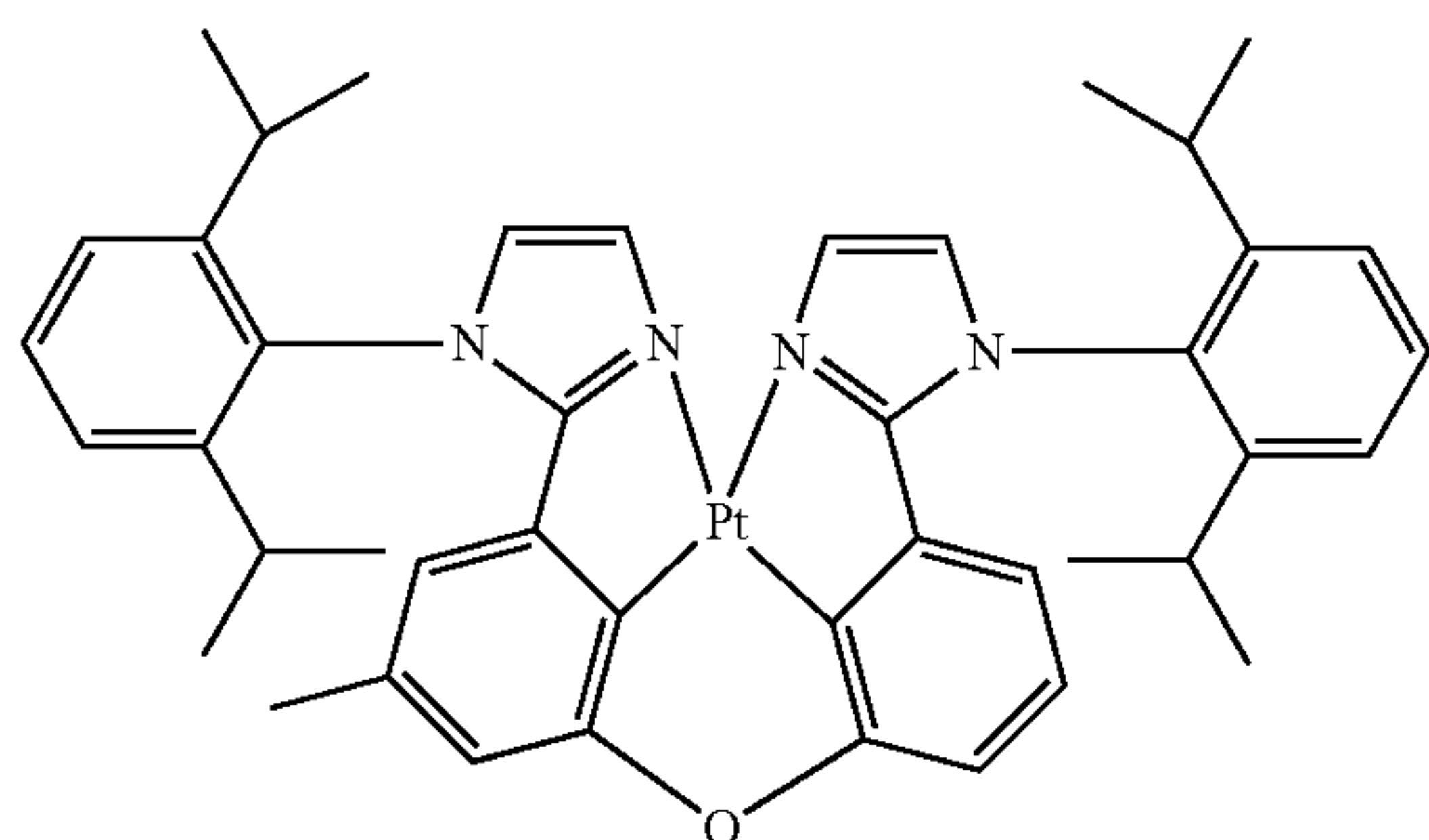
Compound 162
