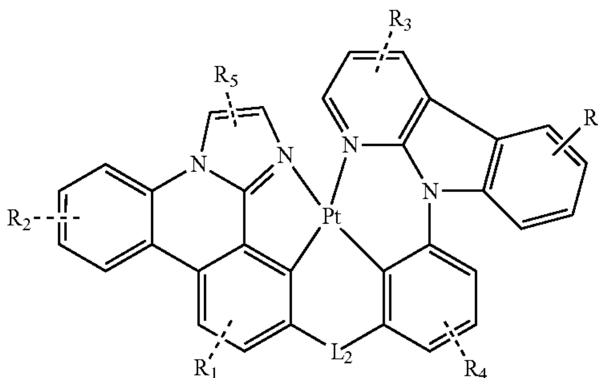
Formula VII'
