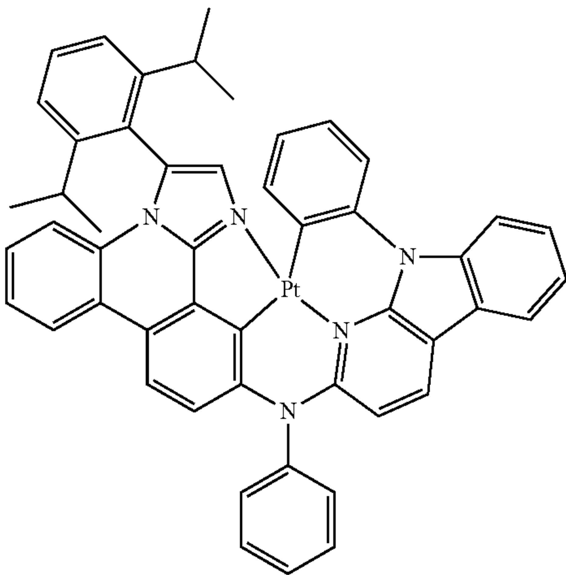
Compound 230'
