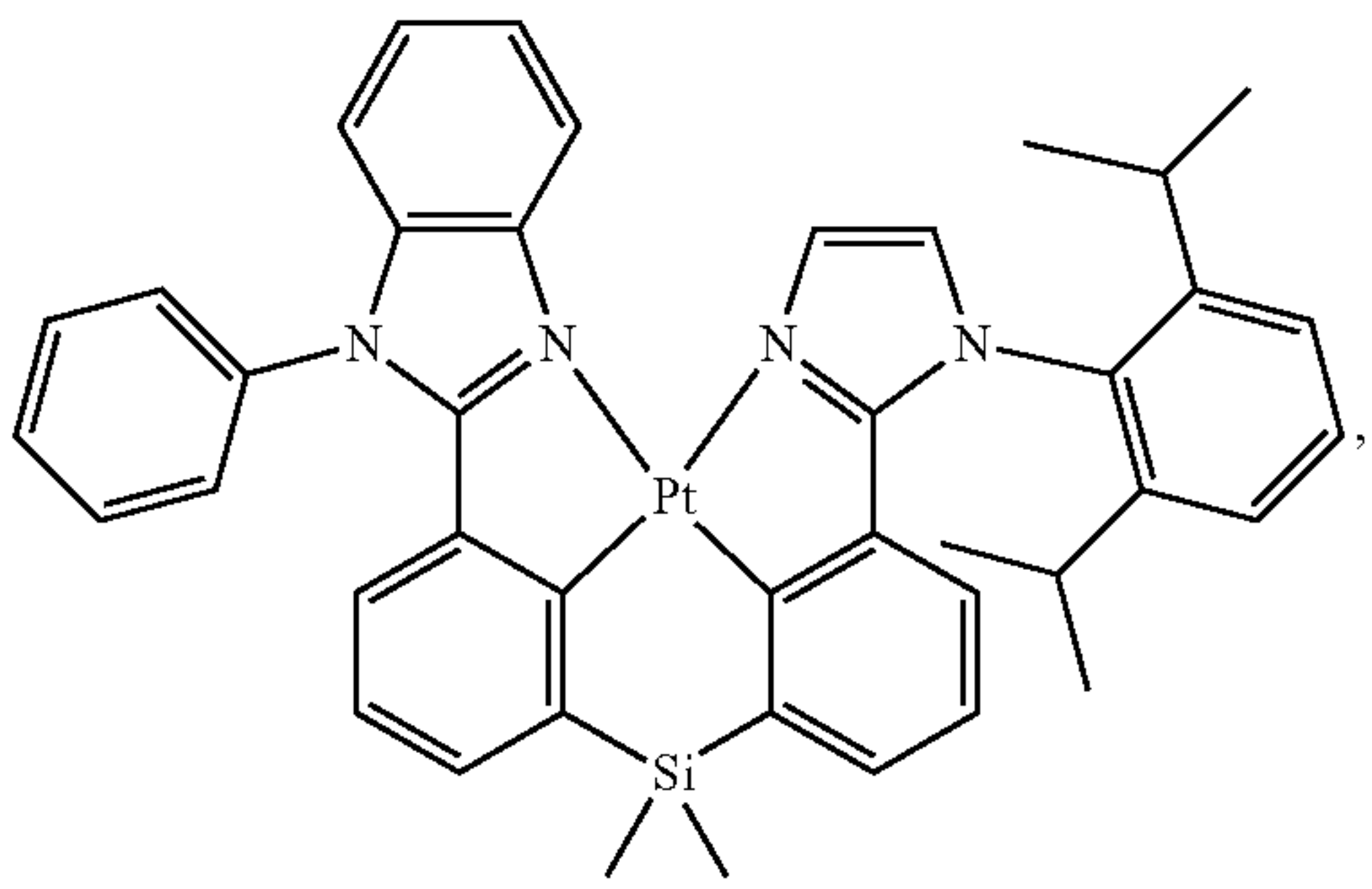
Compound 71
