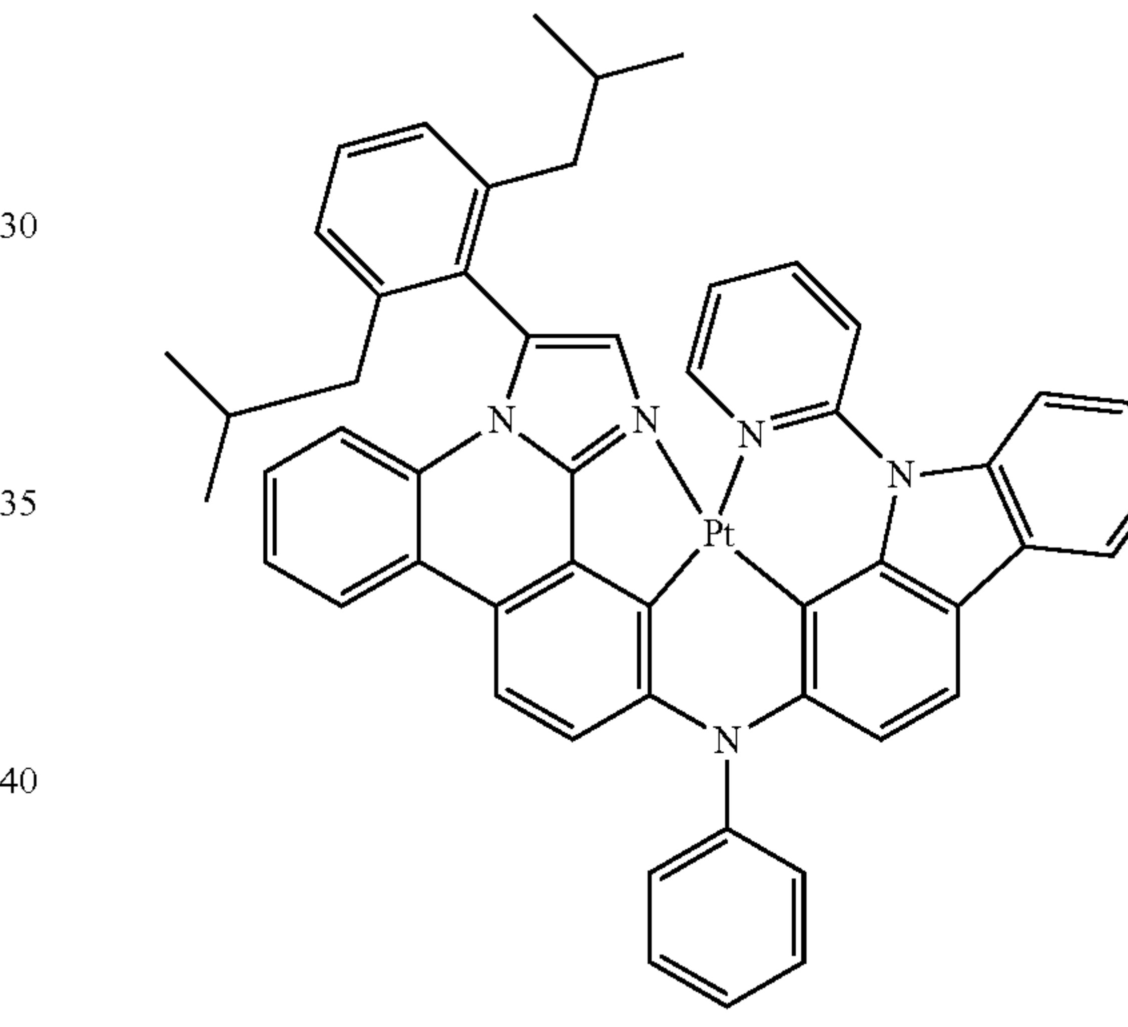
Compound 23'
