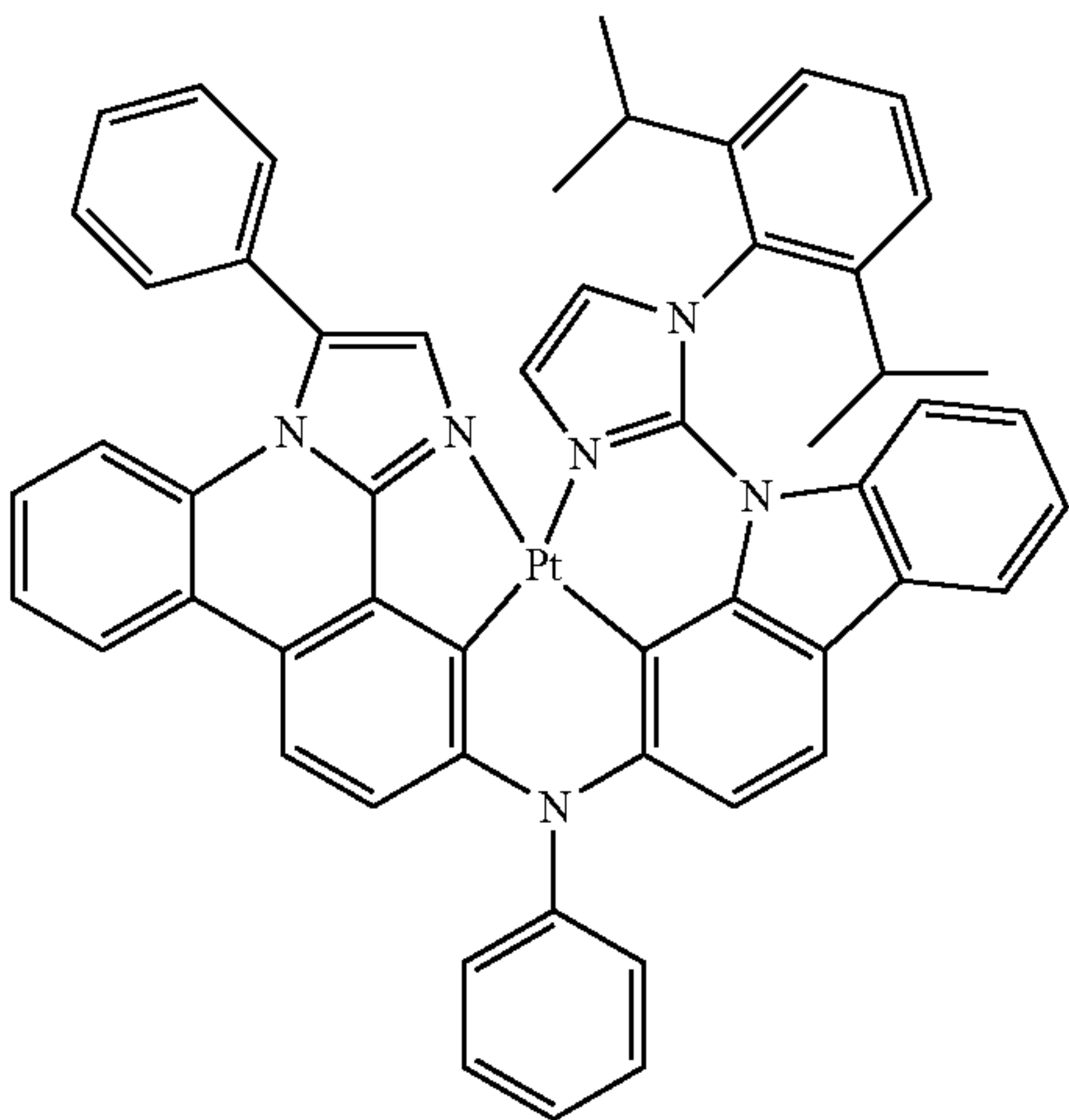
Compound 141'
