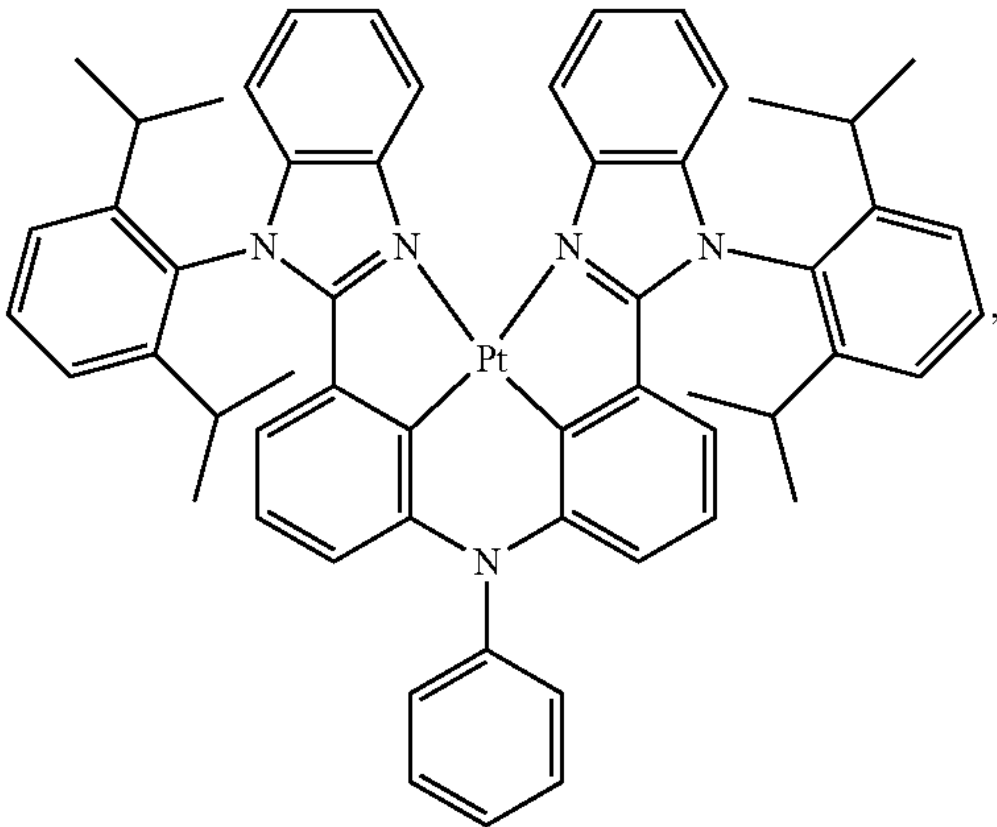
Compound 12
