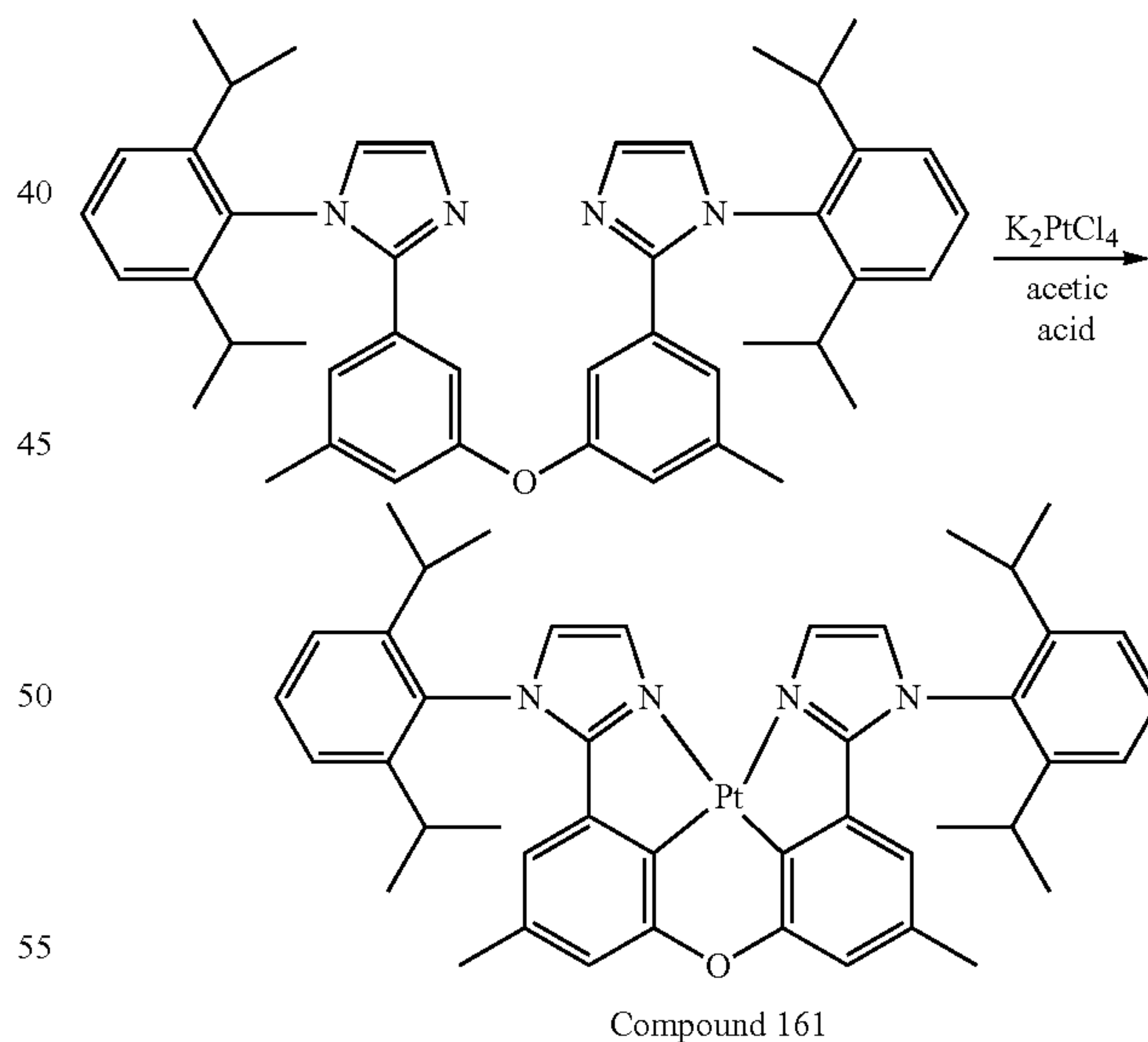
Synthesis of Compound 161
