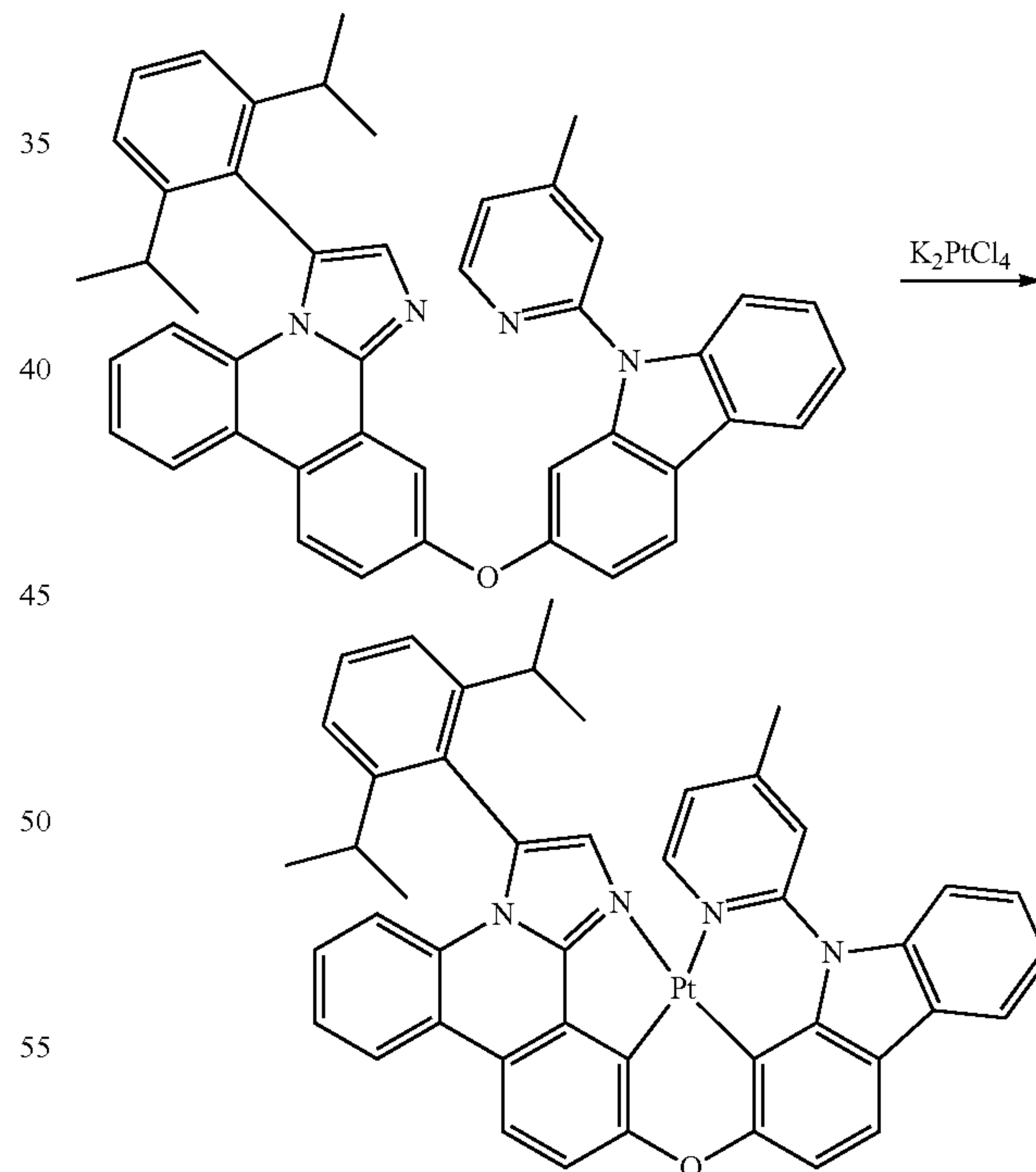
Synthesis of Compound 4'
