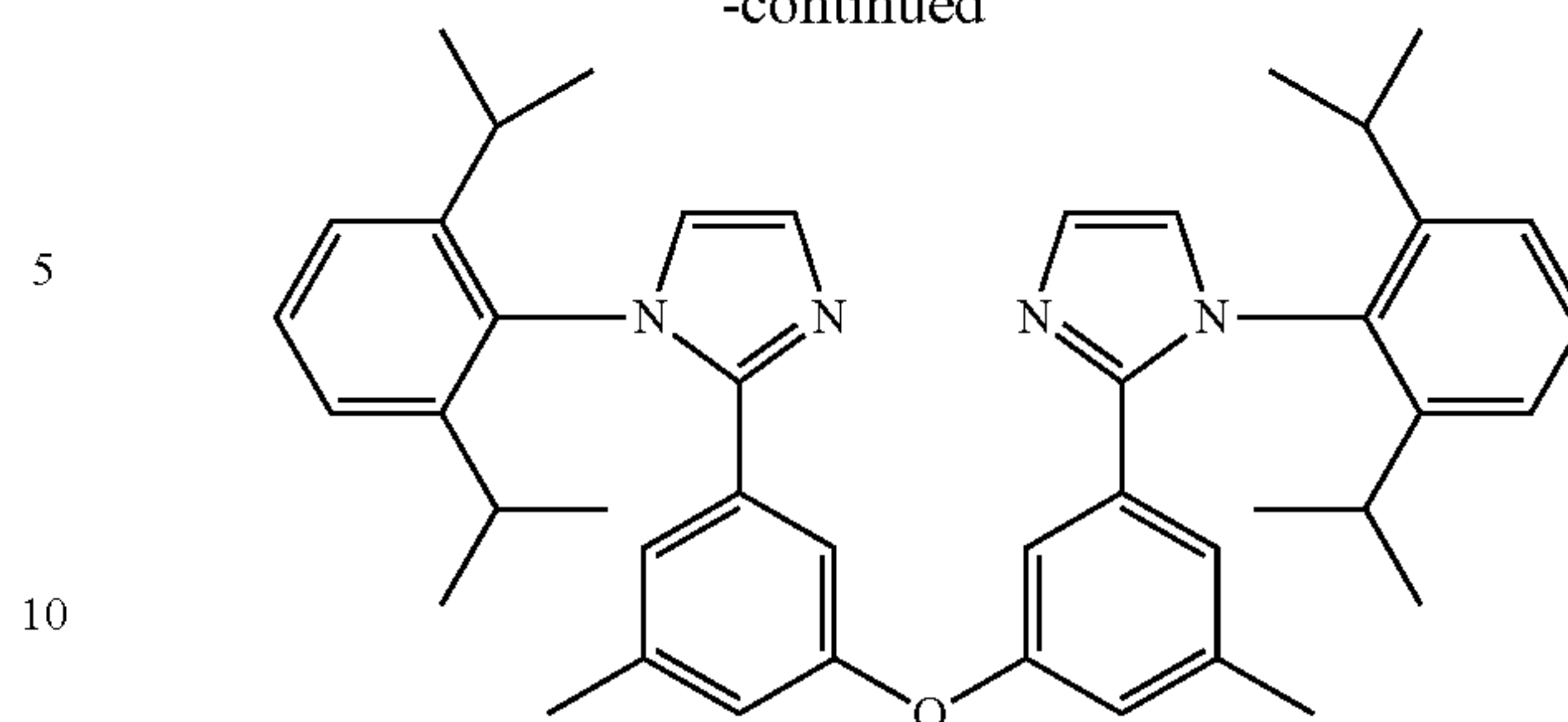
Synthesis of 2,2'-(oxybis(3-methyl-5,1-phenylene))bis(1-(2,6-diisopropylphenyl)-1H-imidazole
