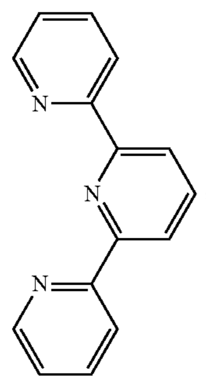
2,2':6',2''- terpyridine (tpy)
