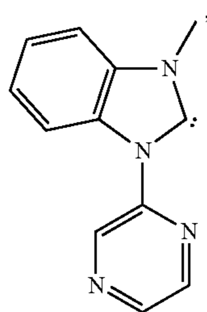
Mebim-pz
