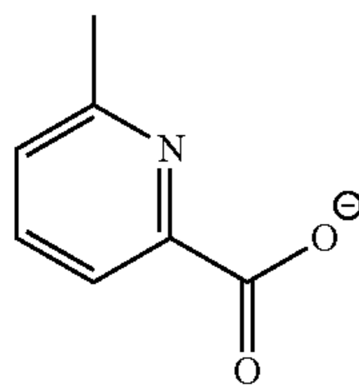
Me-pic
