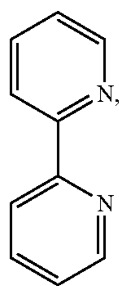
2,2'- bipyridine (bpy)
