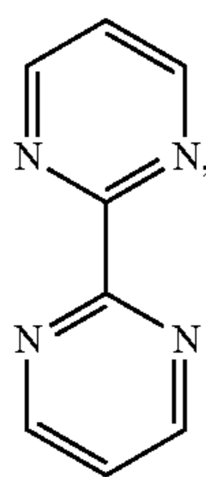
2,2'- bipyrimidine (bpm)
