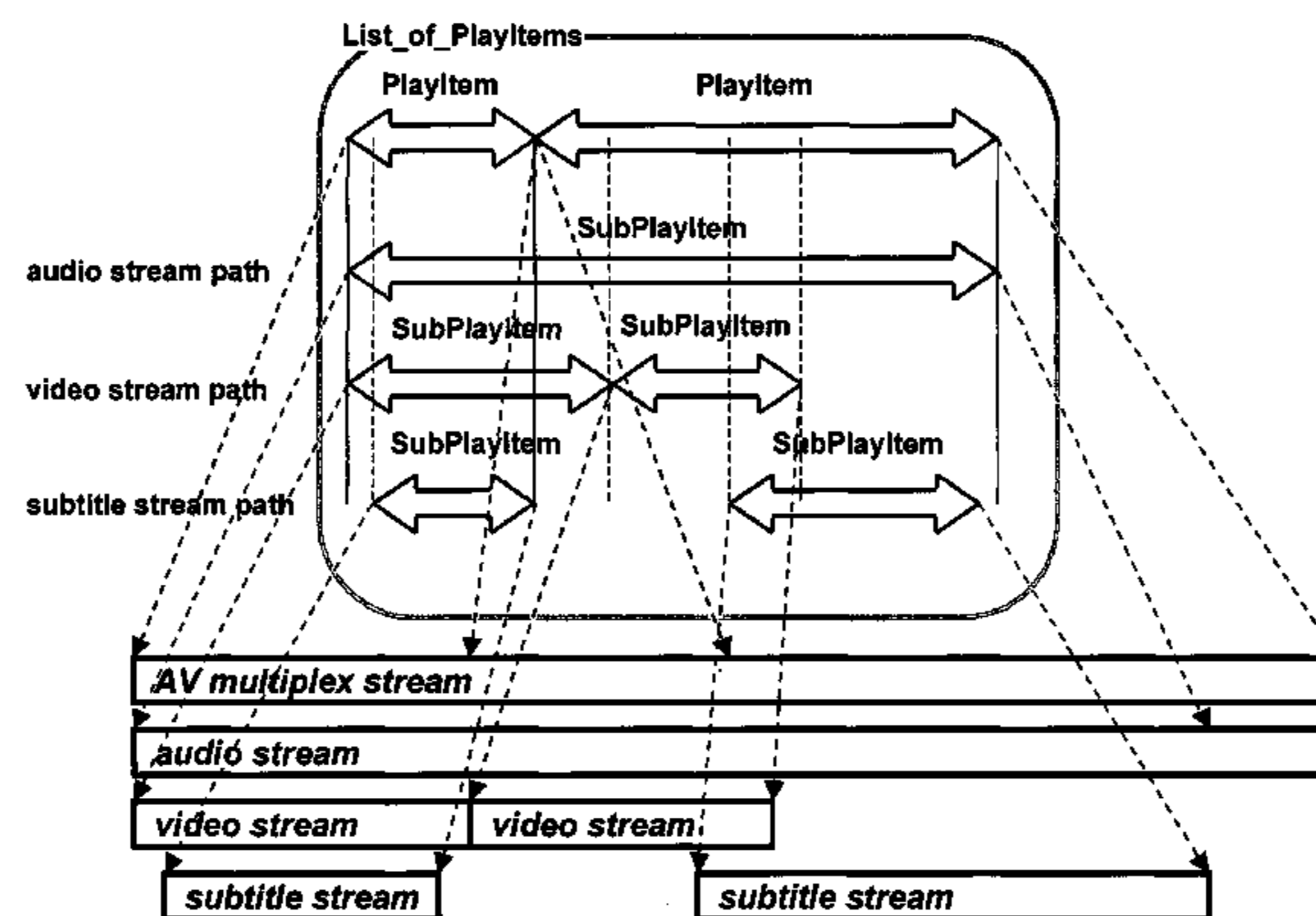
List_of_PlayItems Example
