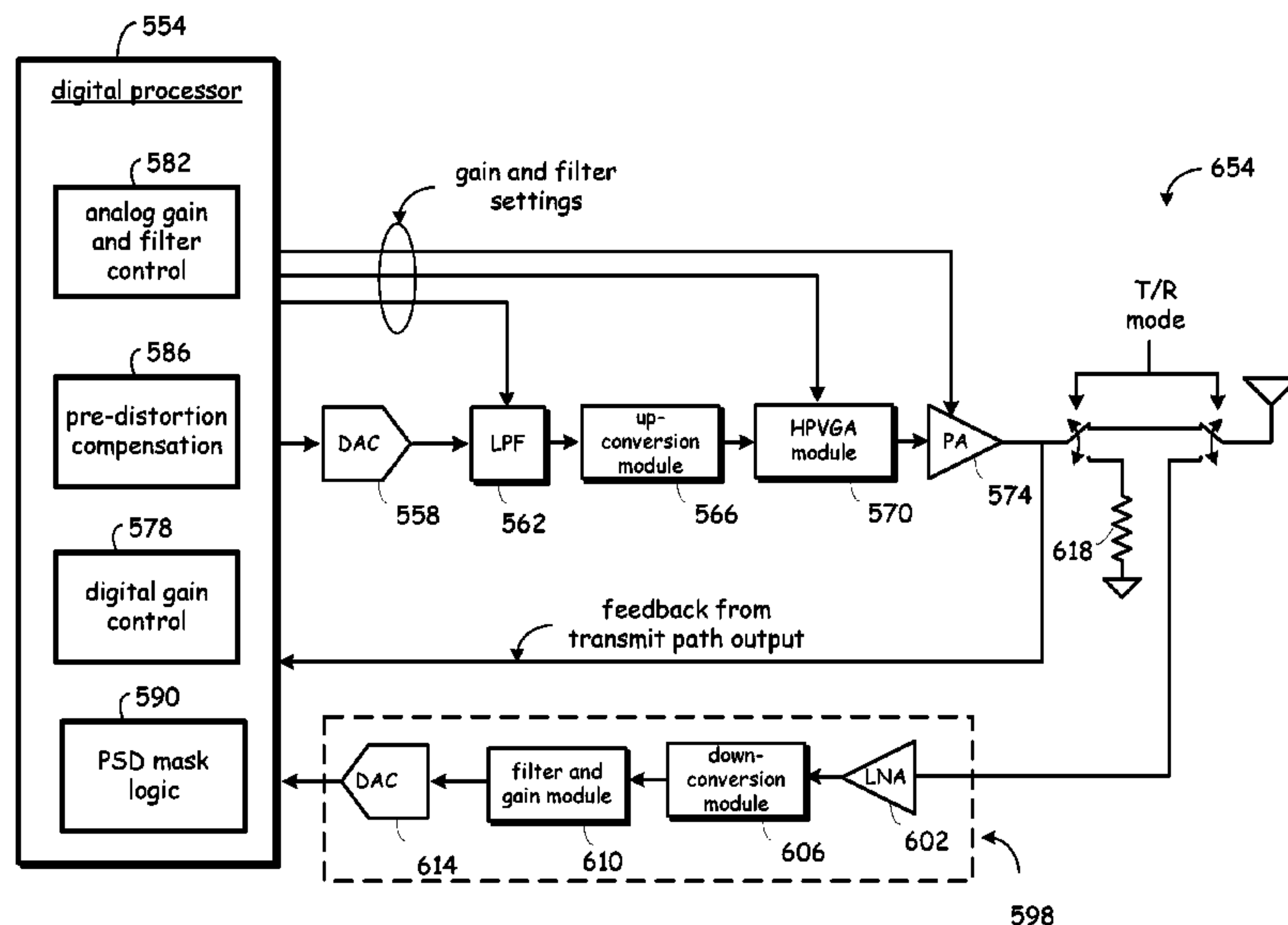
transceiver 650
