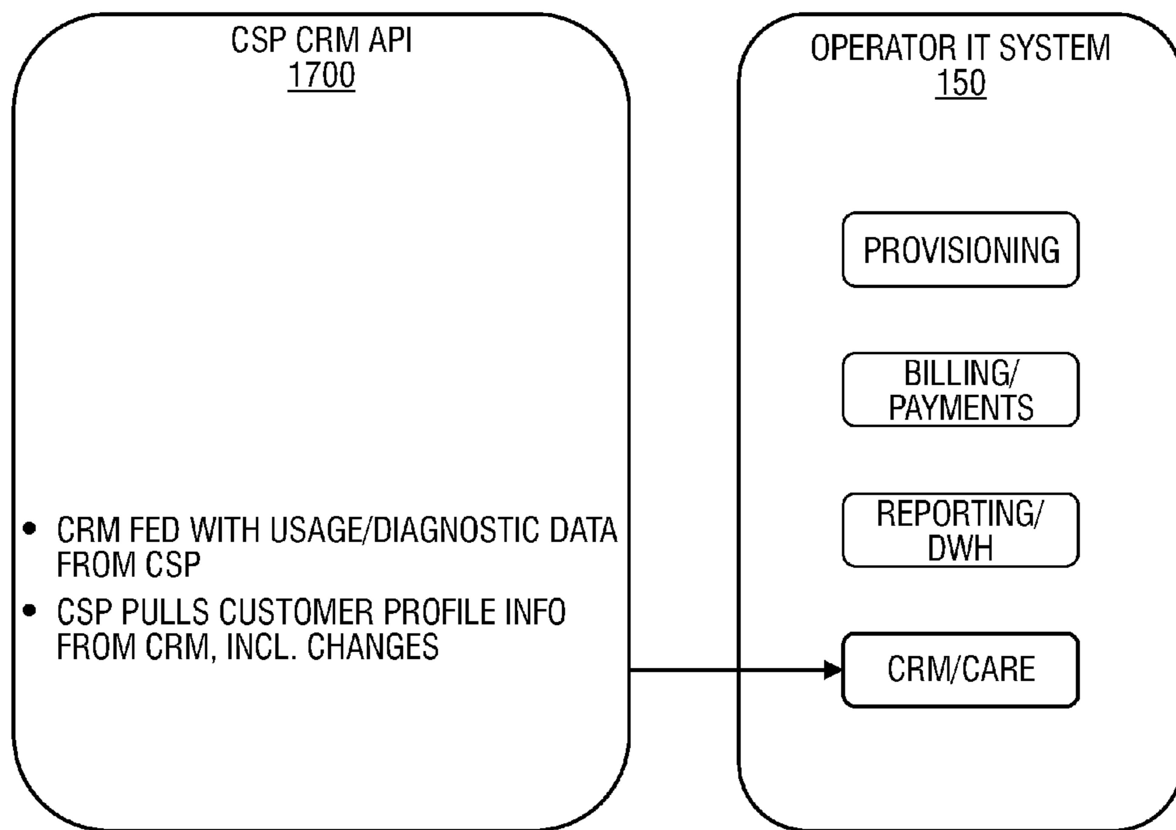
CRM INTEGRATION
