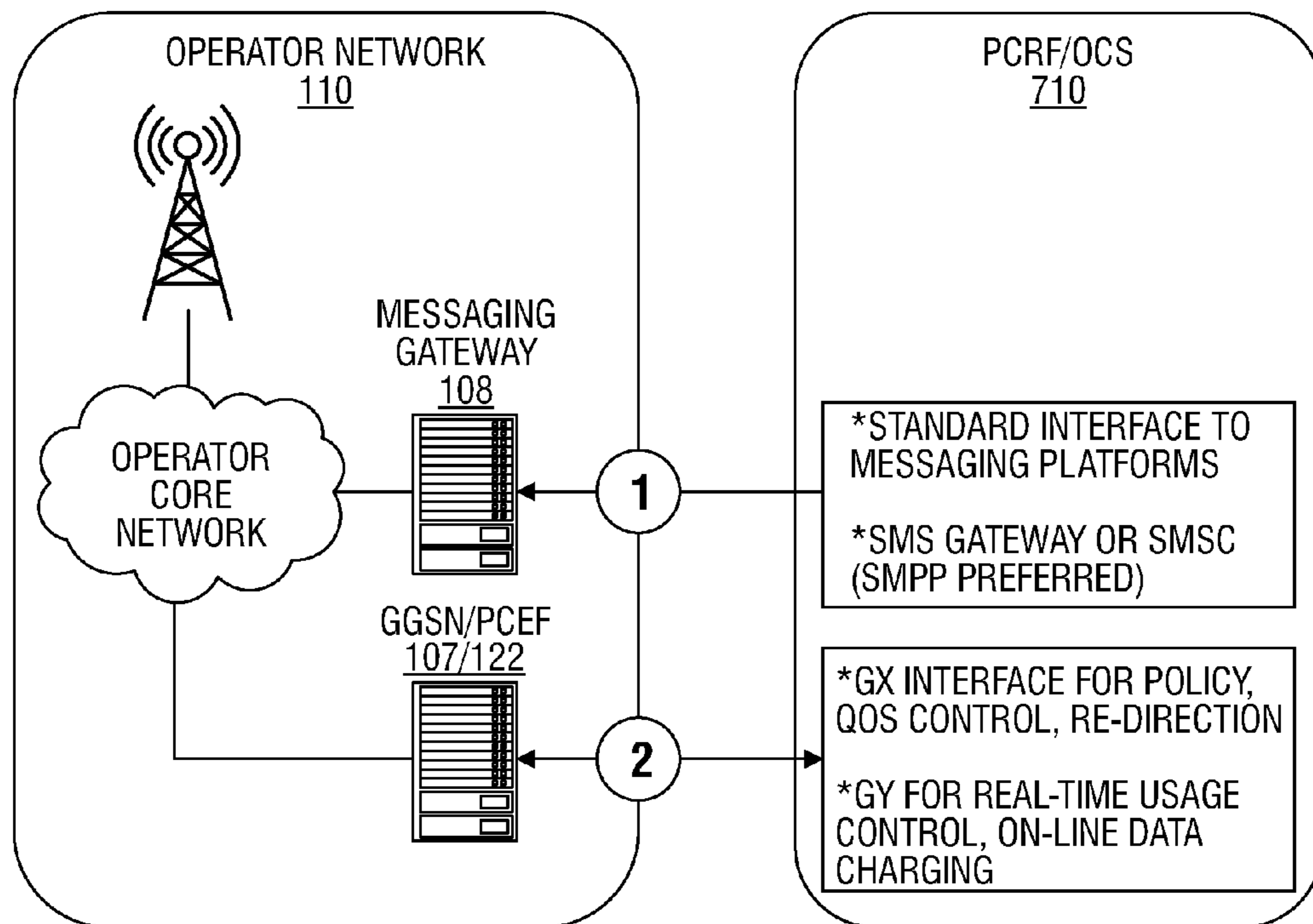
NETWORK INTEGRATION
