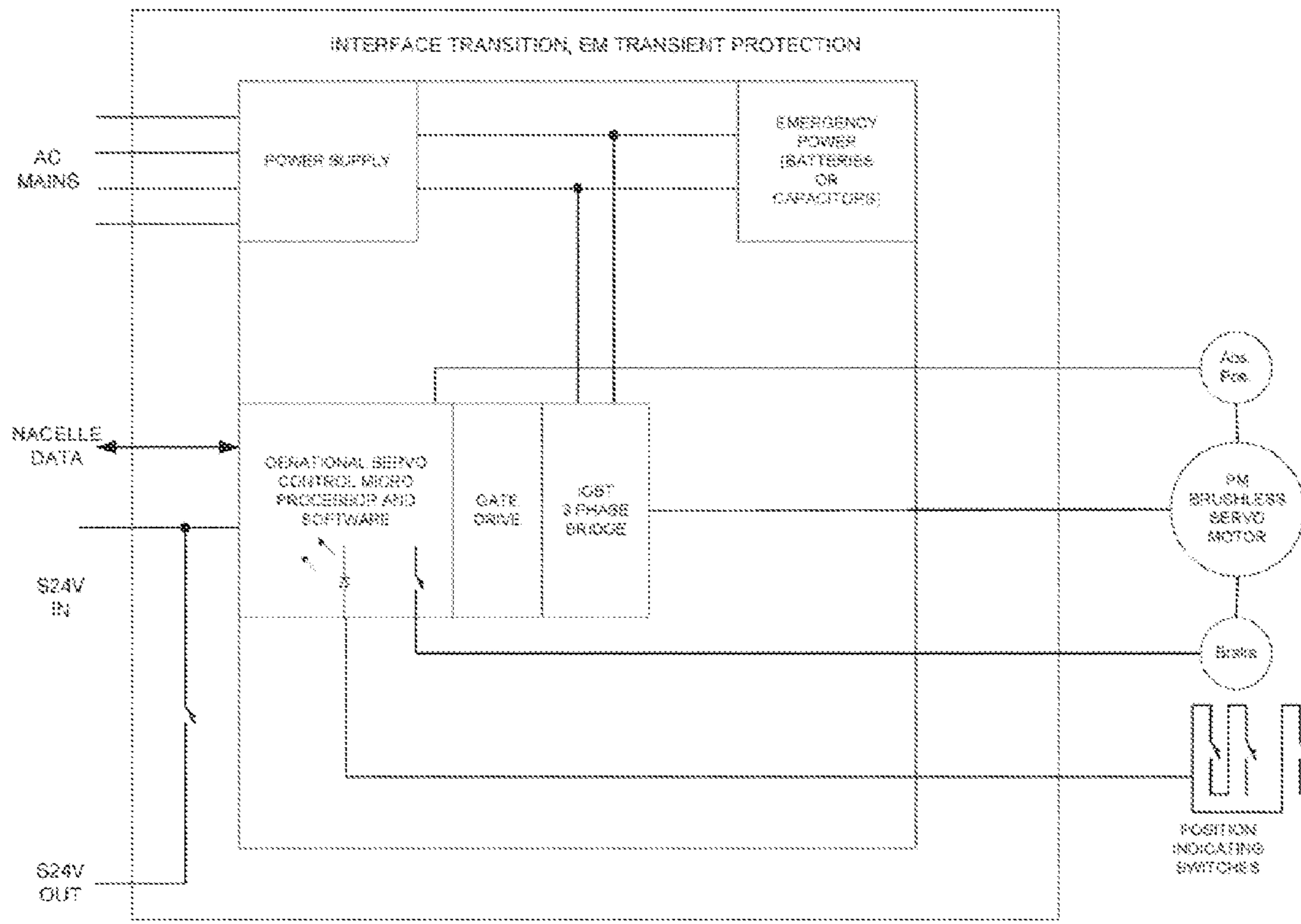
BRUSHLESS PITCH SYSTEM - CONVENTIONAL IMPLEMENTATION
