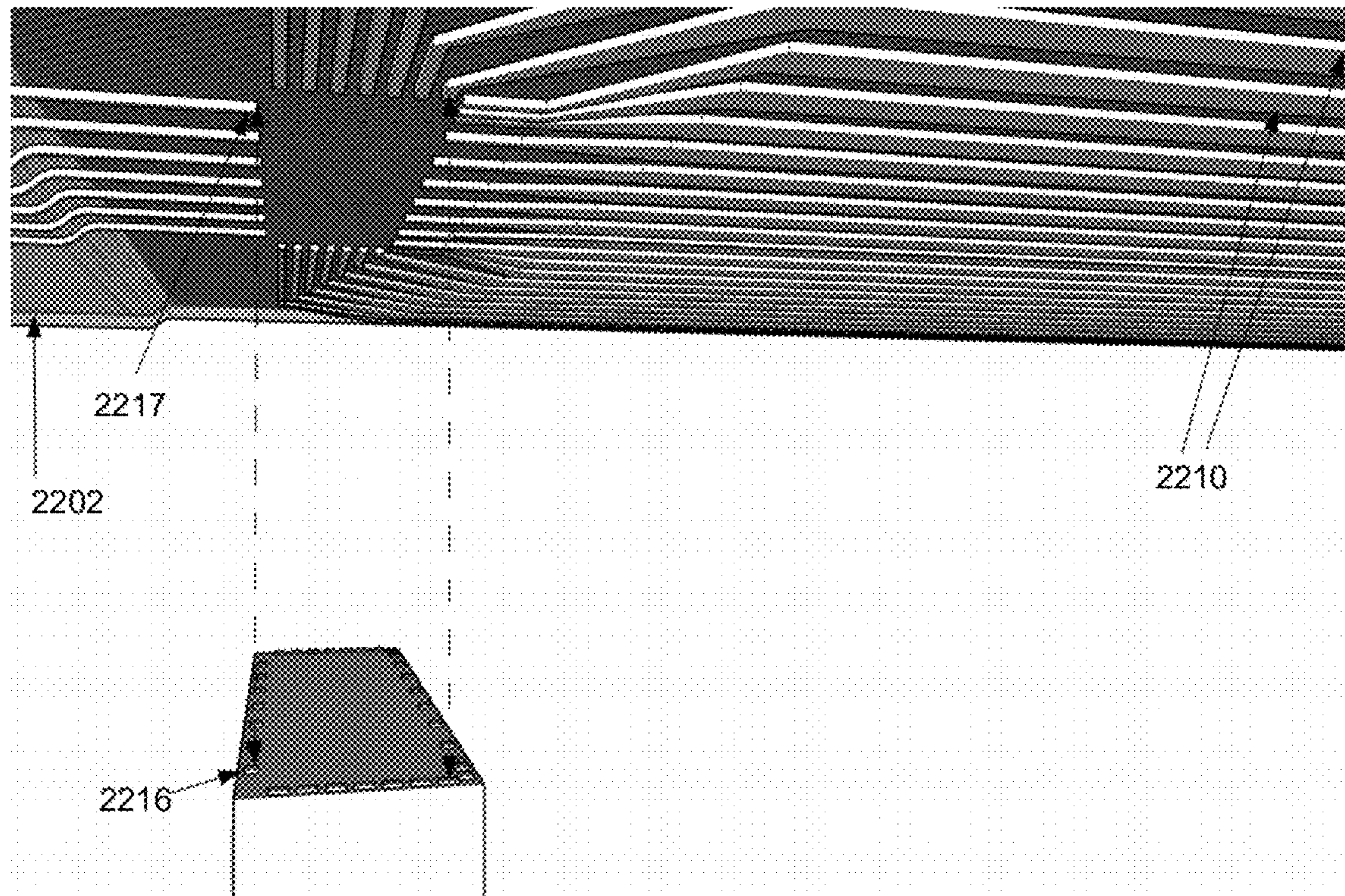
Fig 23e- IC COF attach
