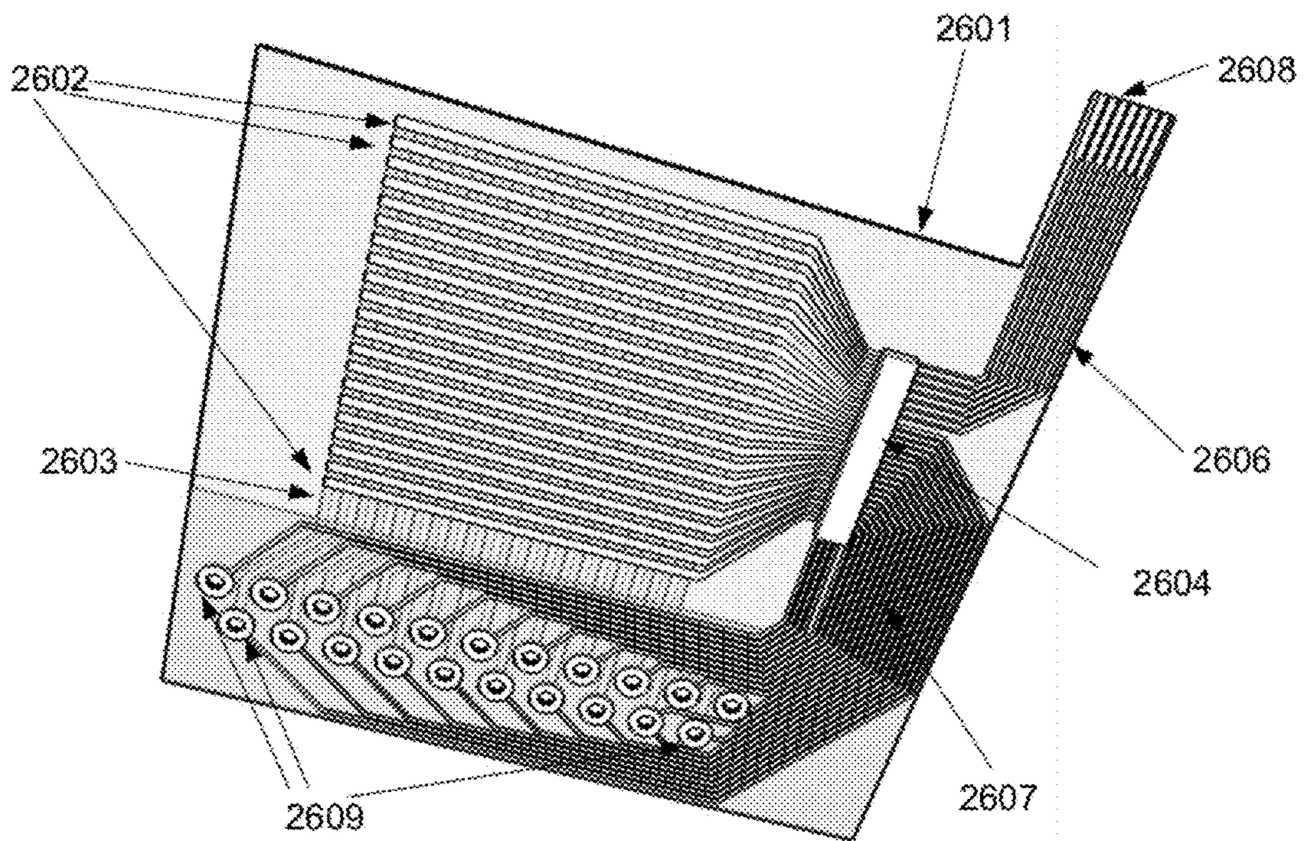
Figure 26b: Single Chip- Bottom View
