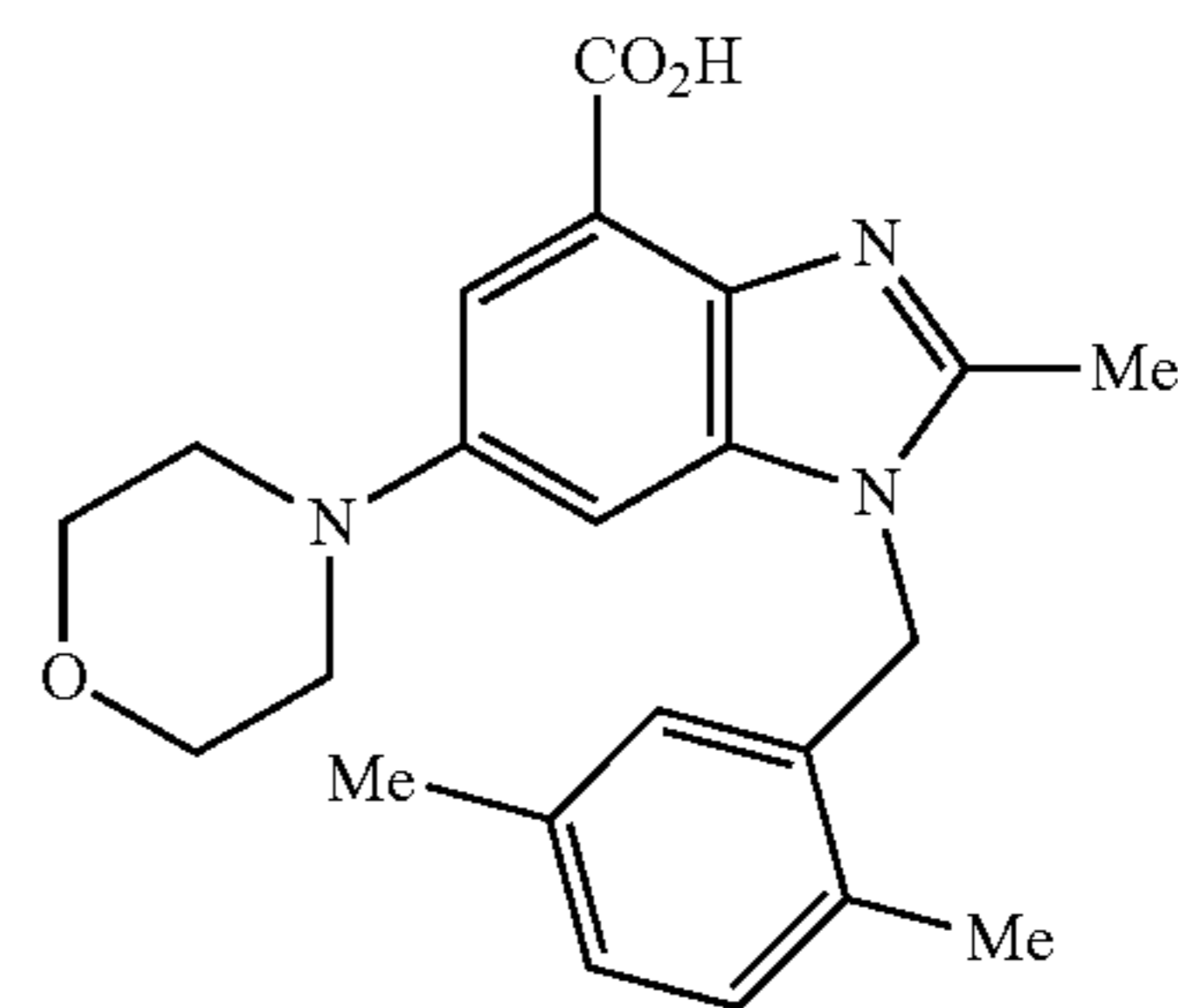
Preparation of 1-[(2,5-dimethylphenyl)methyl]-2-methyl-6-(4-morpholinyl)-1H-benzimidazole-4-carboxylic acid
