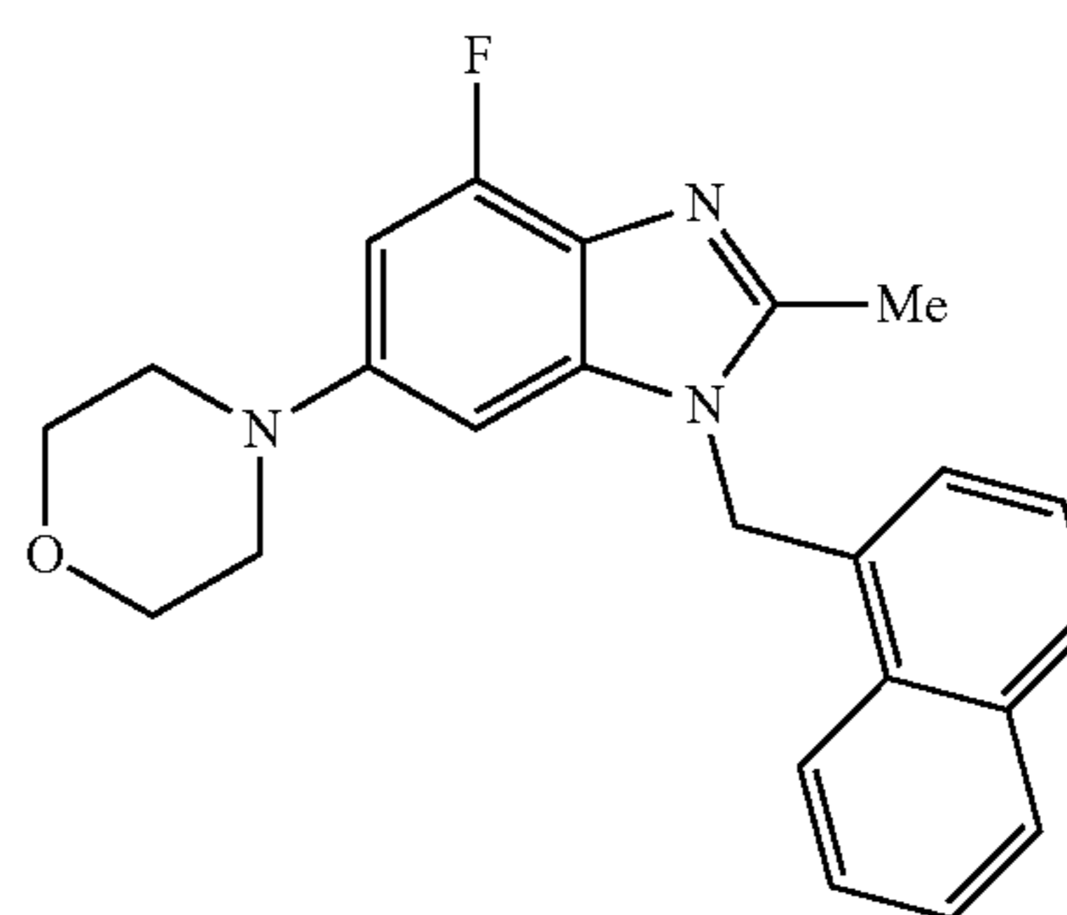
Preparation of 4-fluoro-2-methyl-6-(4-morpholinyl)-1-(1-naphthalenylmethyl)-1H-benzimidazol-4-ol
