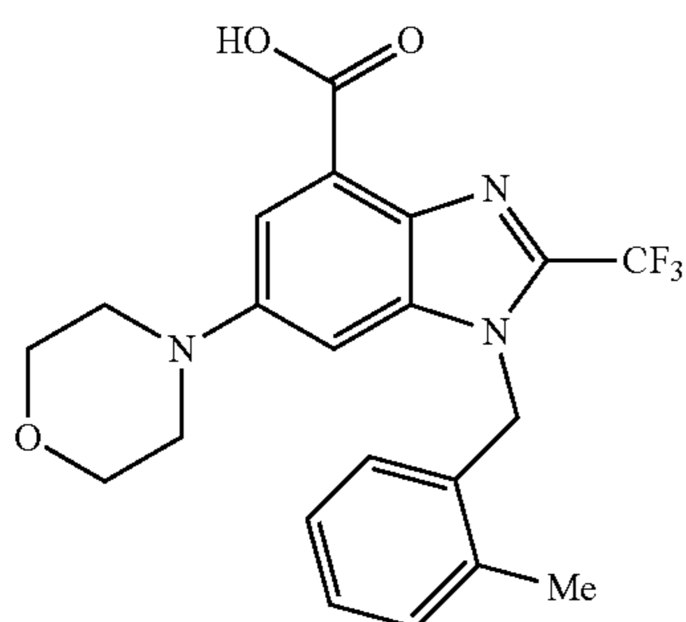
Preparation of 2-methyl-1-[(2-methylphenyl)methyl]-6-(4-morpholinyl)-1H-benzimidazole-4-carboxylic acid
