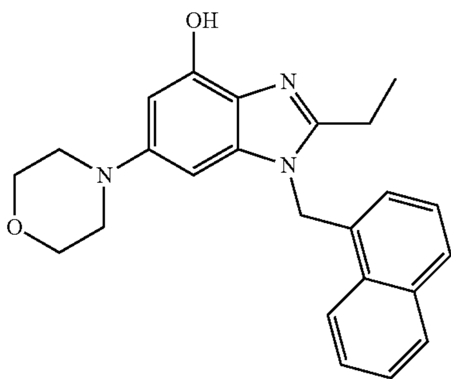
Preparation of 2-ethyl-6-(4-morpholinyl)-1-(1-naphthalenylmethyl)-1H-benzimidazol-4-ol
