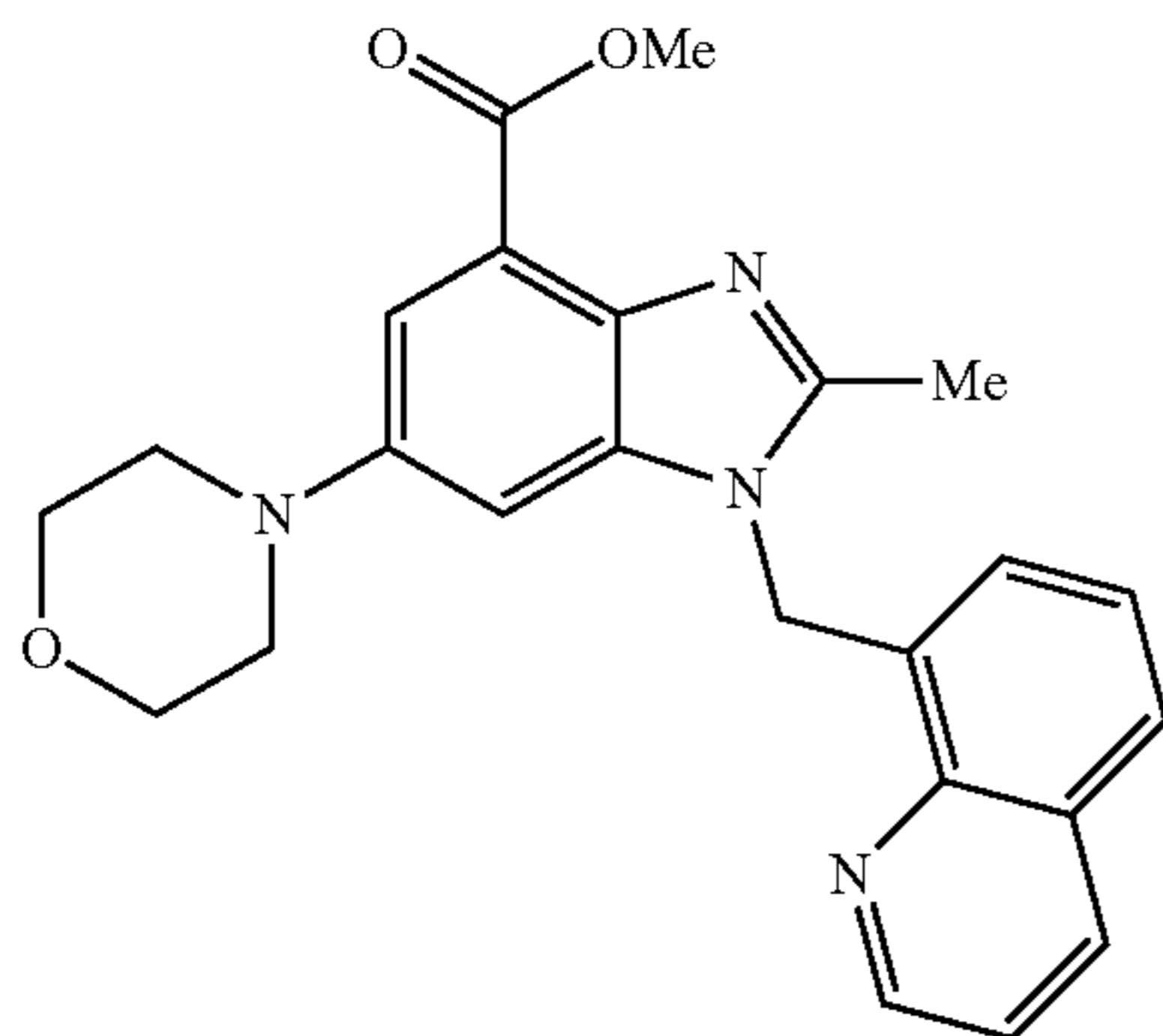
Preparation of methyl 2-methyl-6-(4-morpholinyl)-1-(8-quinolinylmethyl)-1H-benzimidazole-4-carboxylate
