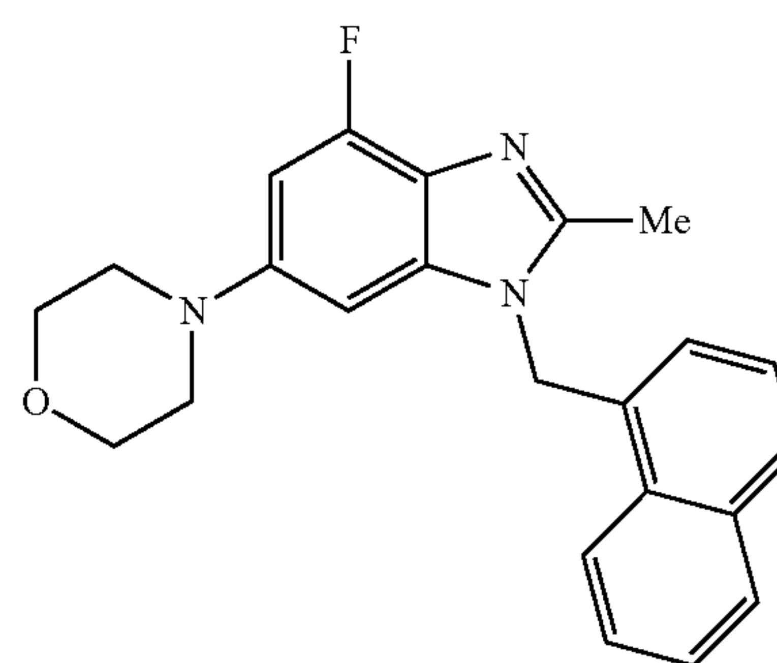
Preparation of 4-fluoro-2-methyl-6-(4-morpholinyl)-1-(1-naphthalenylmethyl)-1H-benzimidazole
