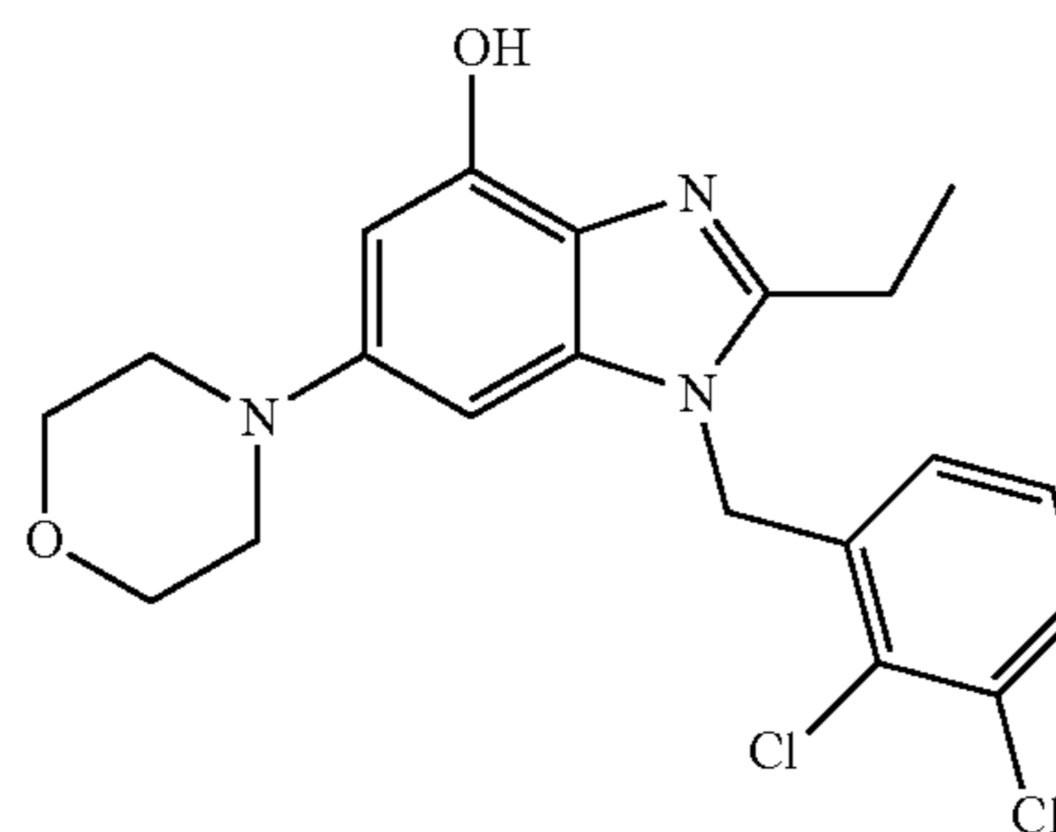
Preparation of 1-[(2,3-dichlorophenyl)methyl]-2-ethyl-6-(4-morpholinyl)-1H-benzimidazol-4-ol
