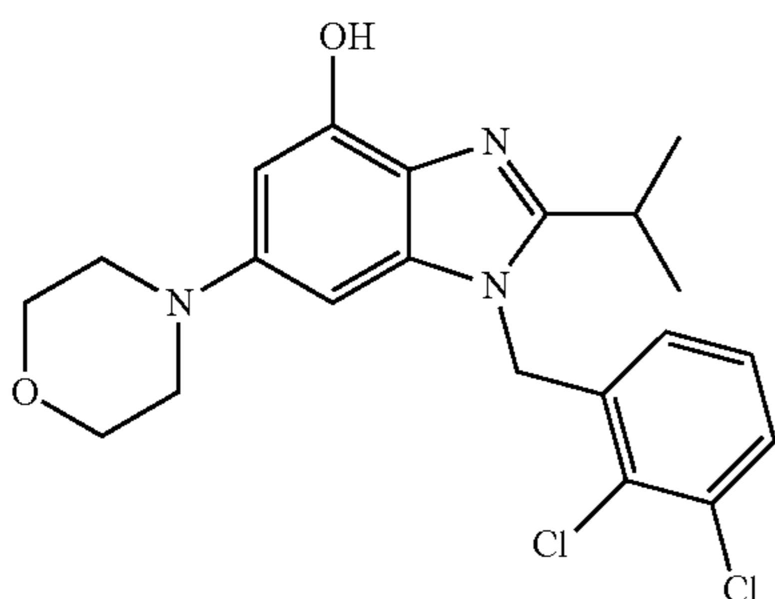
Preparation of 1-[(2,3-dichlorophenyl)methyl]-2-(1-methylethyl)-6-(4-morpholinyl)-1H-benzimidazol-4-ol
