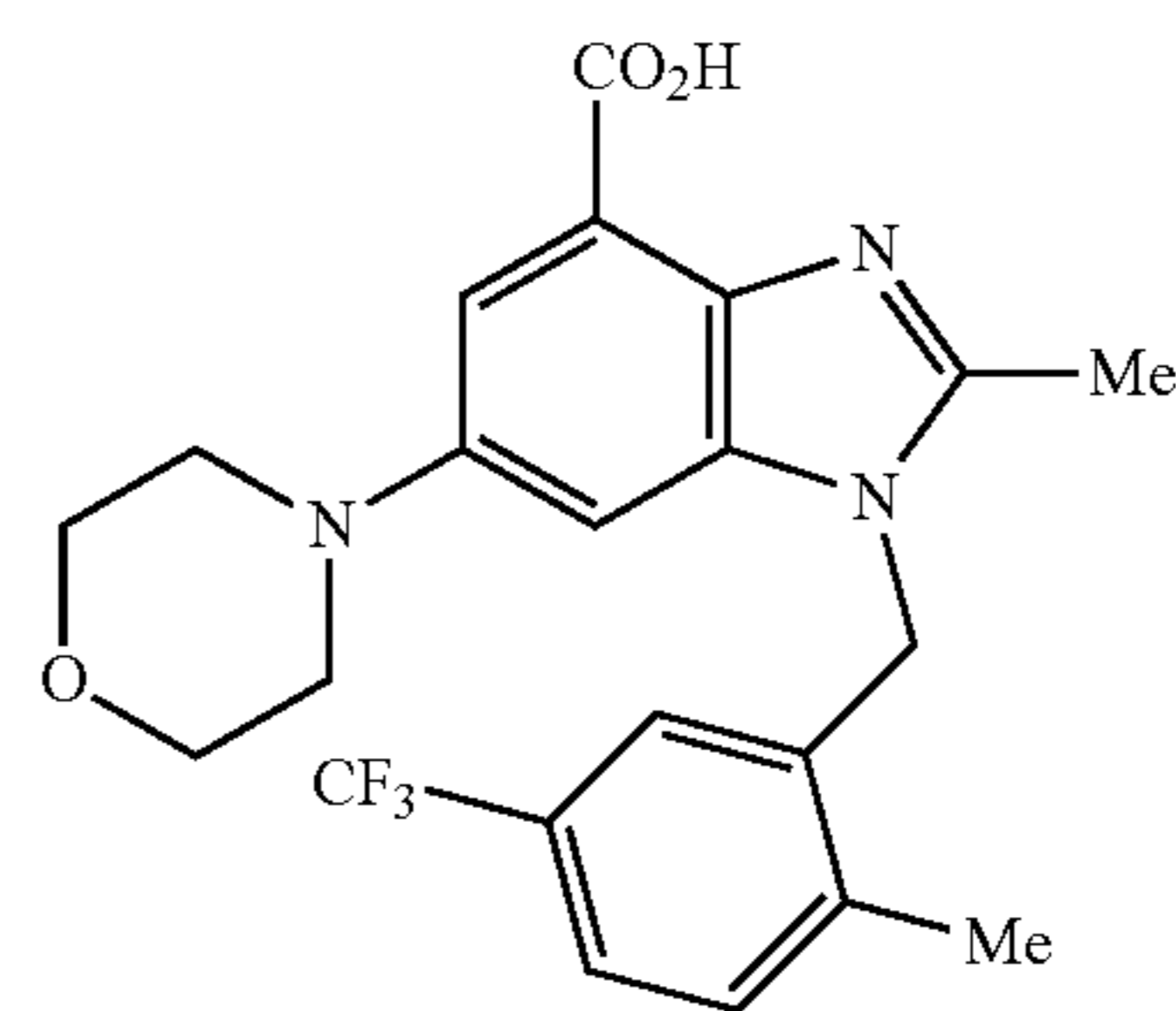
Preparation of 2-methyl-1-([2-methyl-5-(trifluoromethyl)phenyl]methyl)-6-(4-morpholinyl)-1H-benzimidazole-4-carboxylic acid
