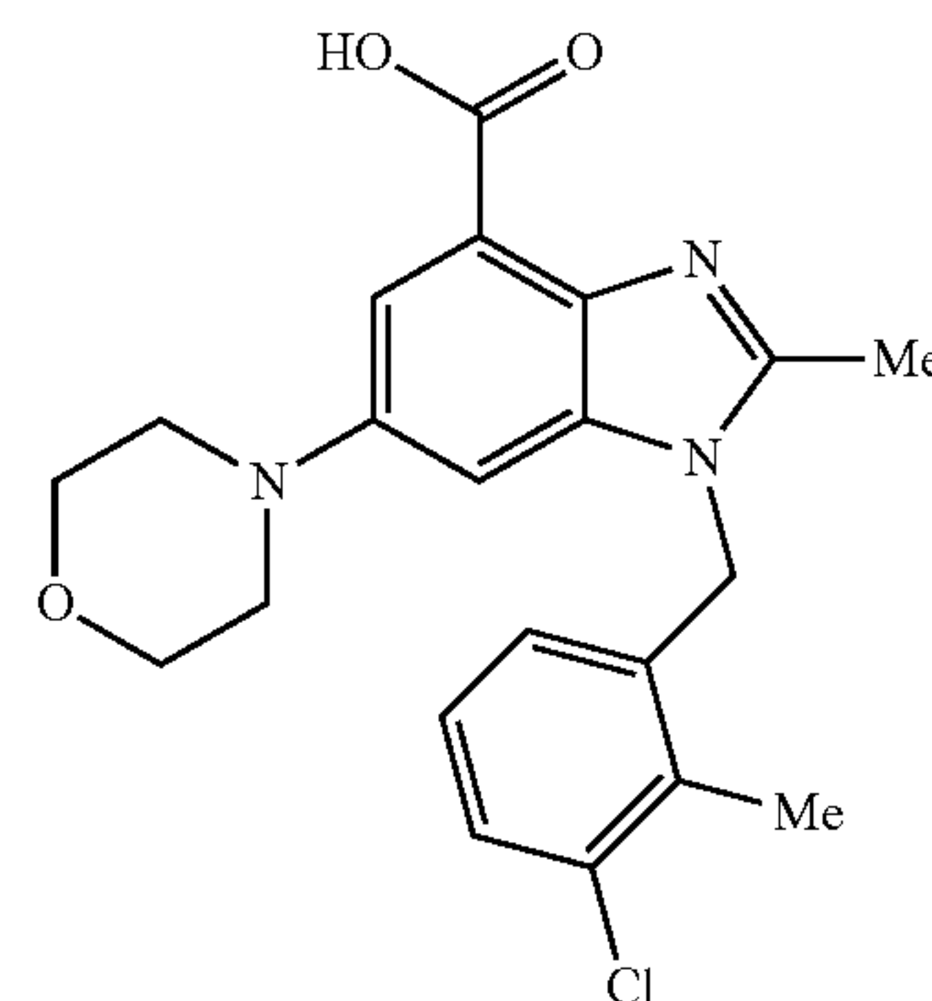
Preparation of 1-[(3-chloro-2-methylphenyl)methyl]-2-methyl-6-(4-morpholinyl)-1H-benzimidazole-4-carboxylic acid
