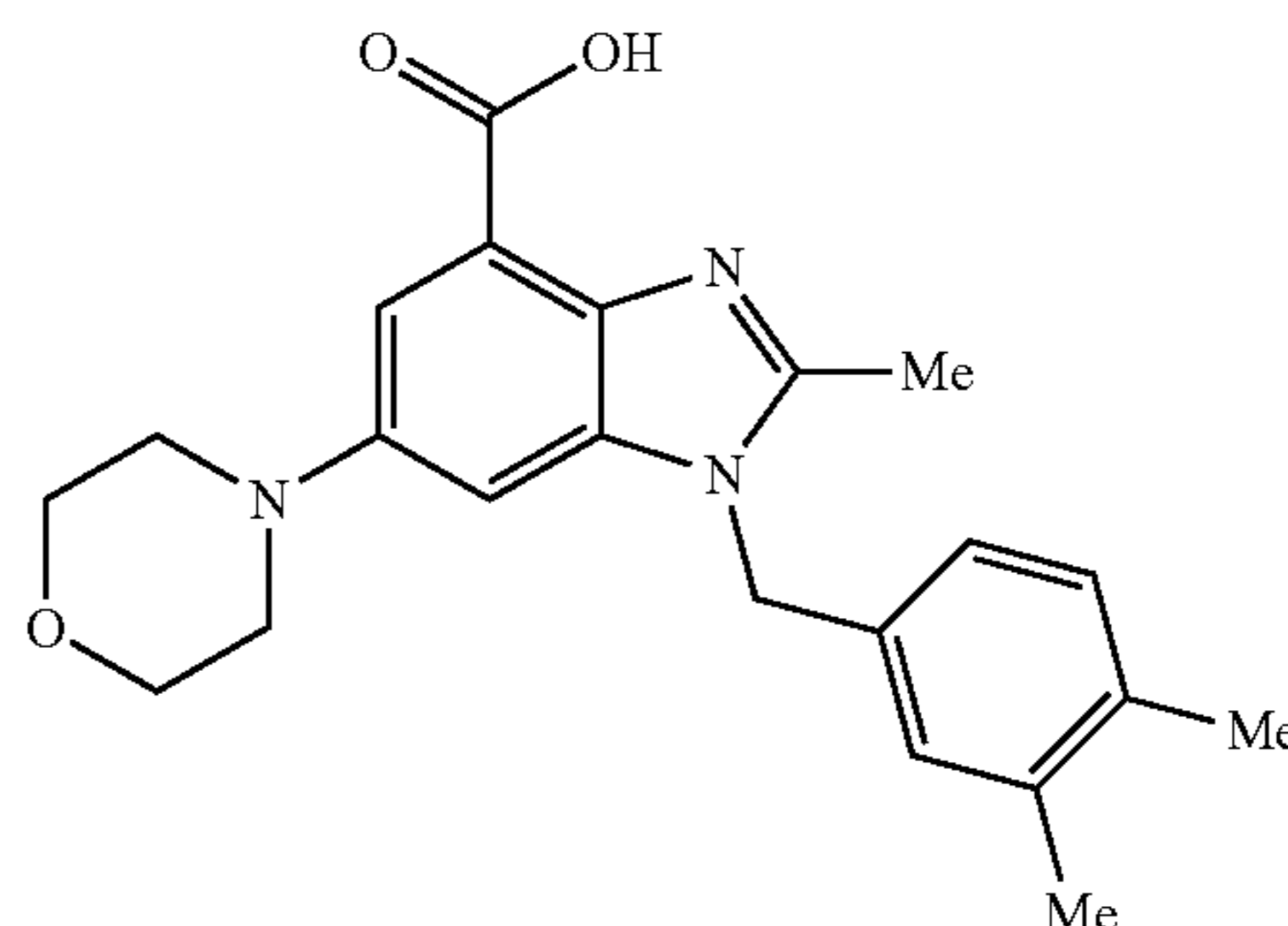
Preparation of 1-[(3,4-dimethylphenyl)methyl]-2-methyl-6-(4-morpholinyl)-1H-benzimidazole-4-carboxylic acid
