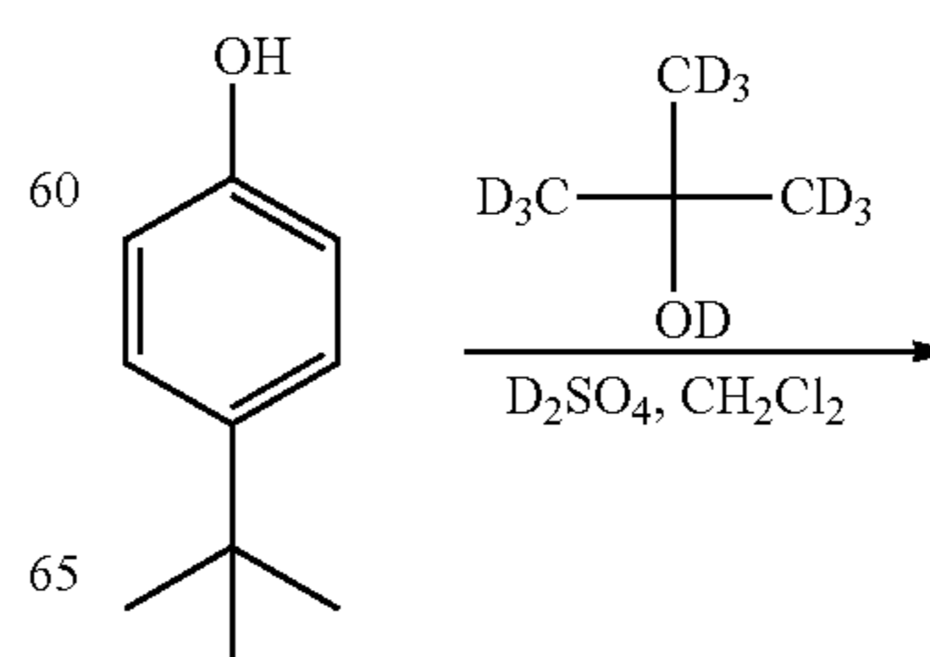
Scheme 6. Preparation of Compound 125
