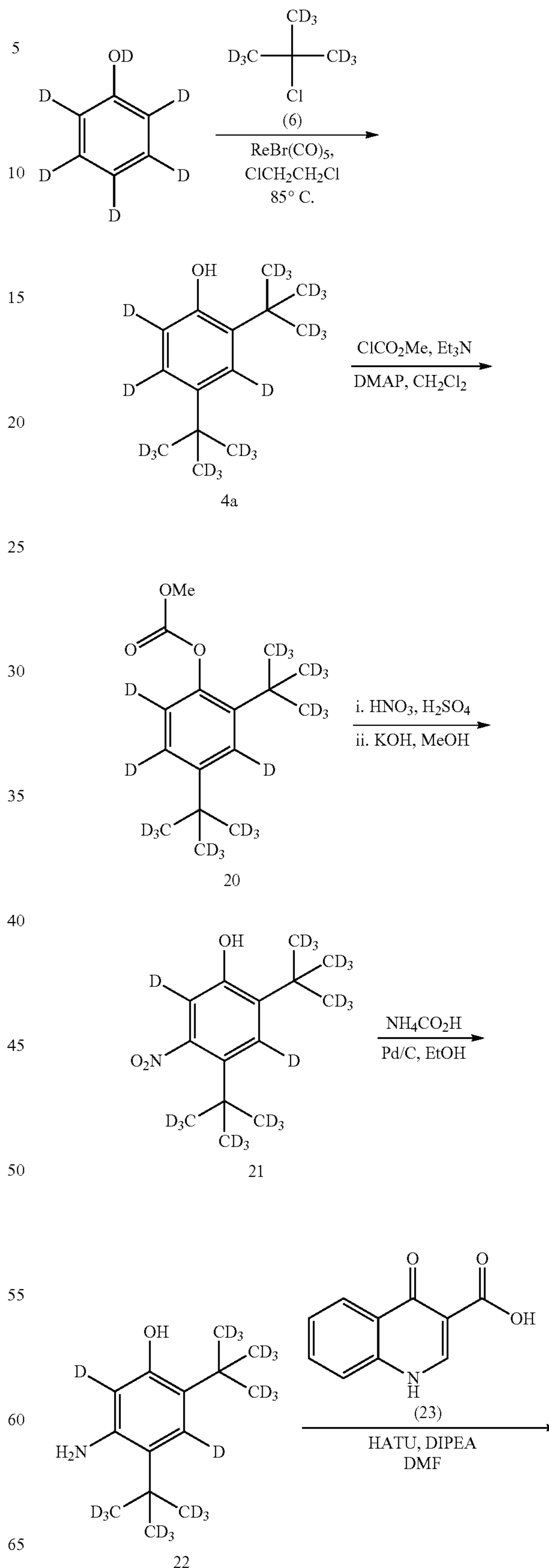
Scheme 5. Preparation of Compound 110
