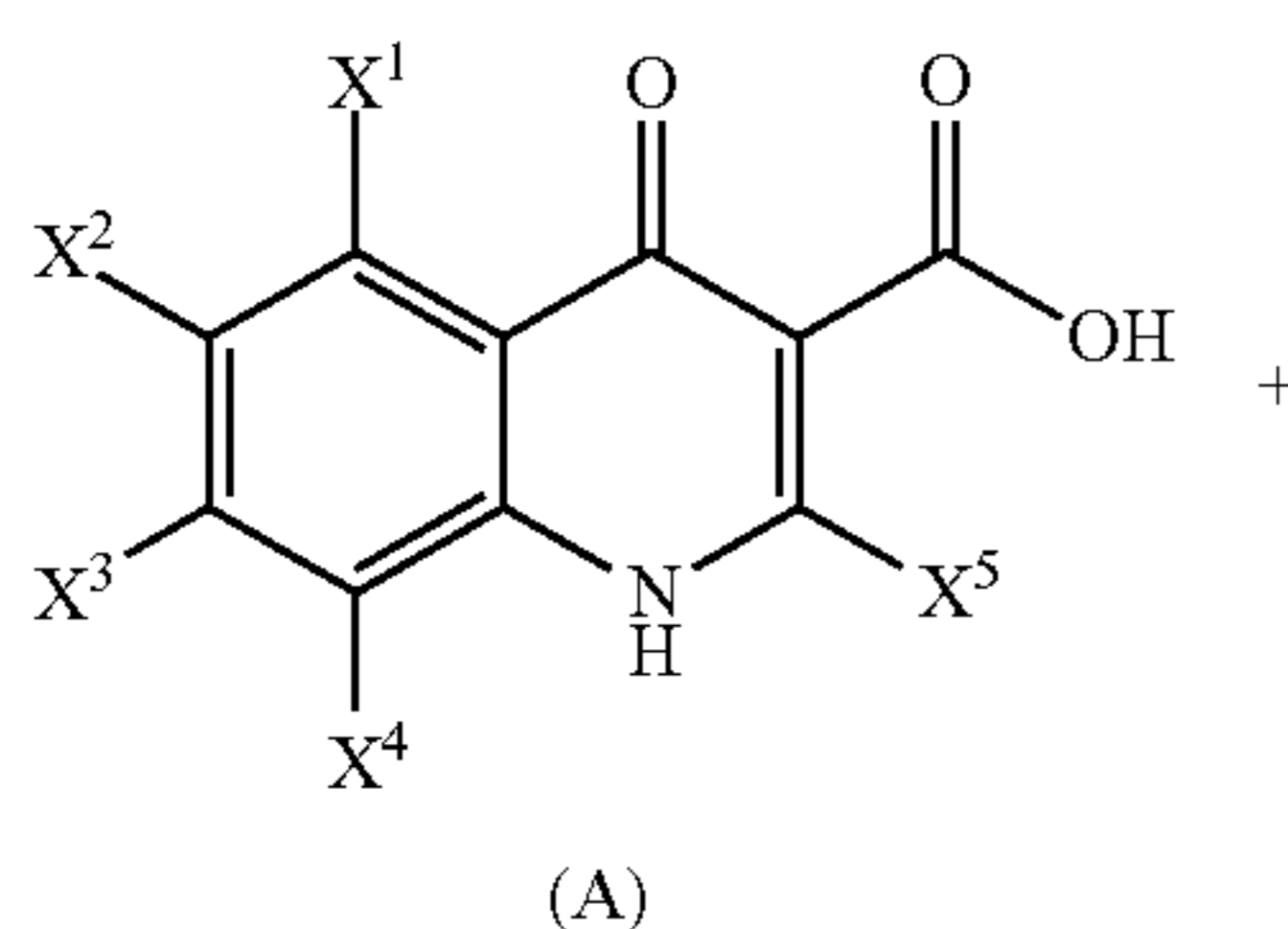
Scheme 1:
