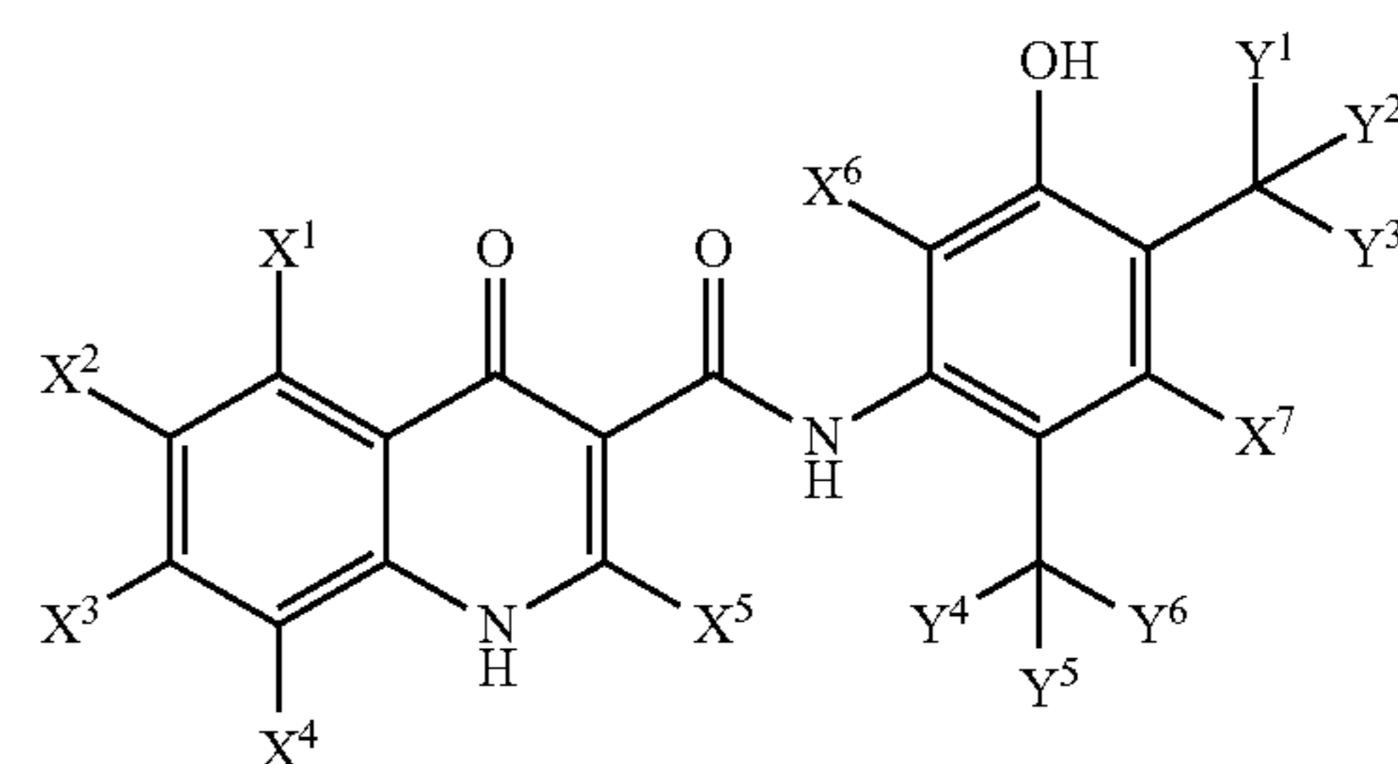
Formula I
