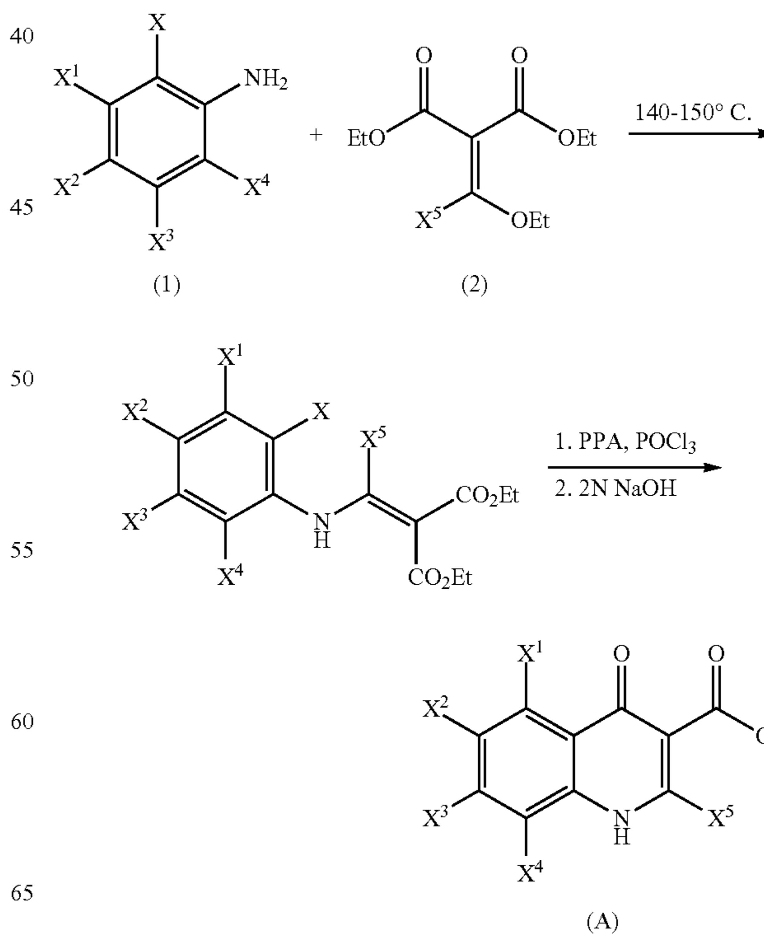
Scheme 2:
