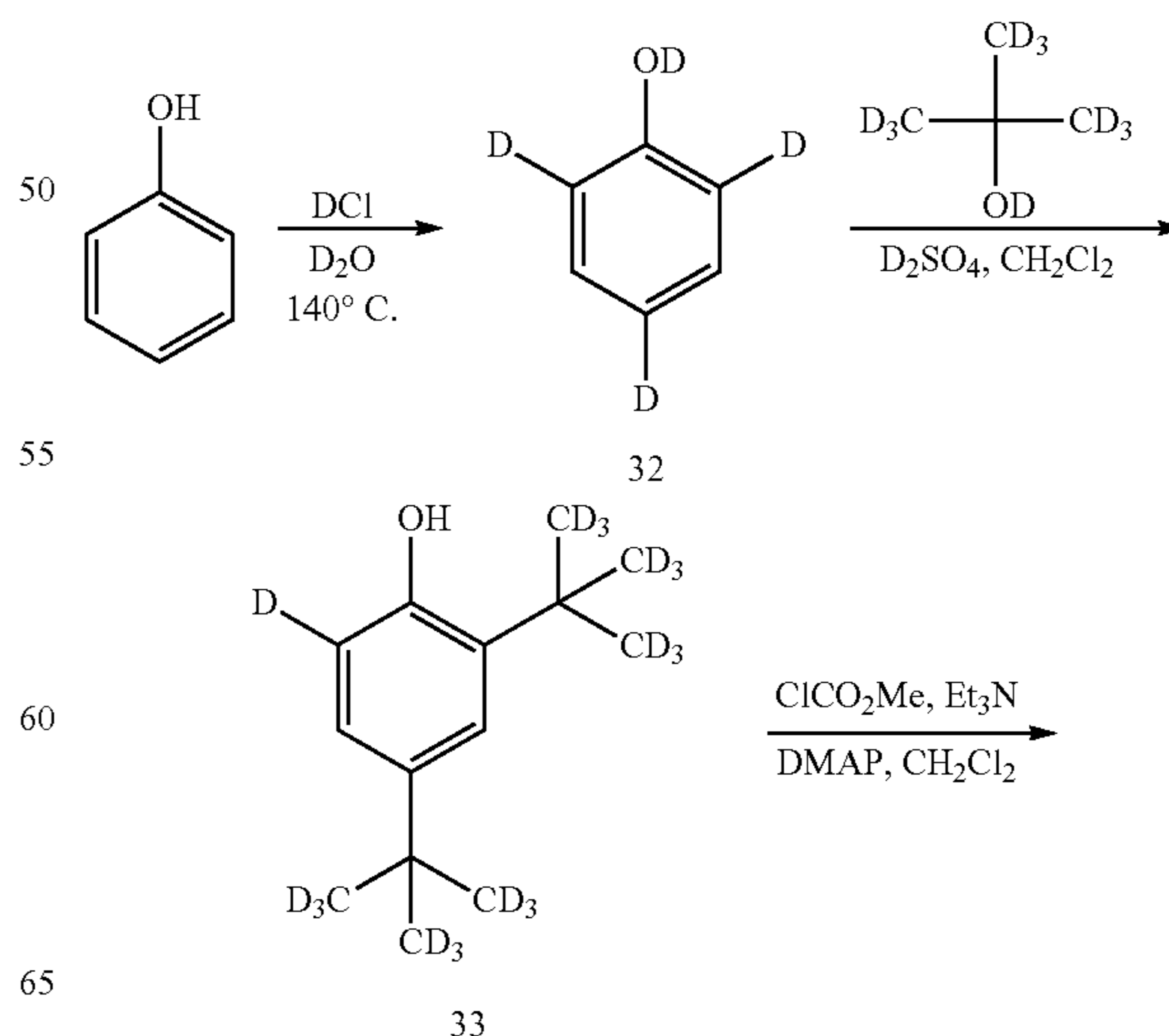
Scheme 8. Preparation of Compound 105
