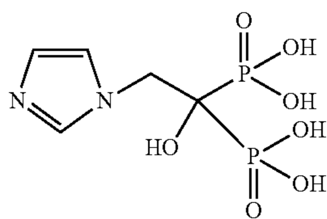
Zoledronic acid
