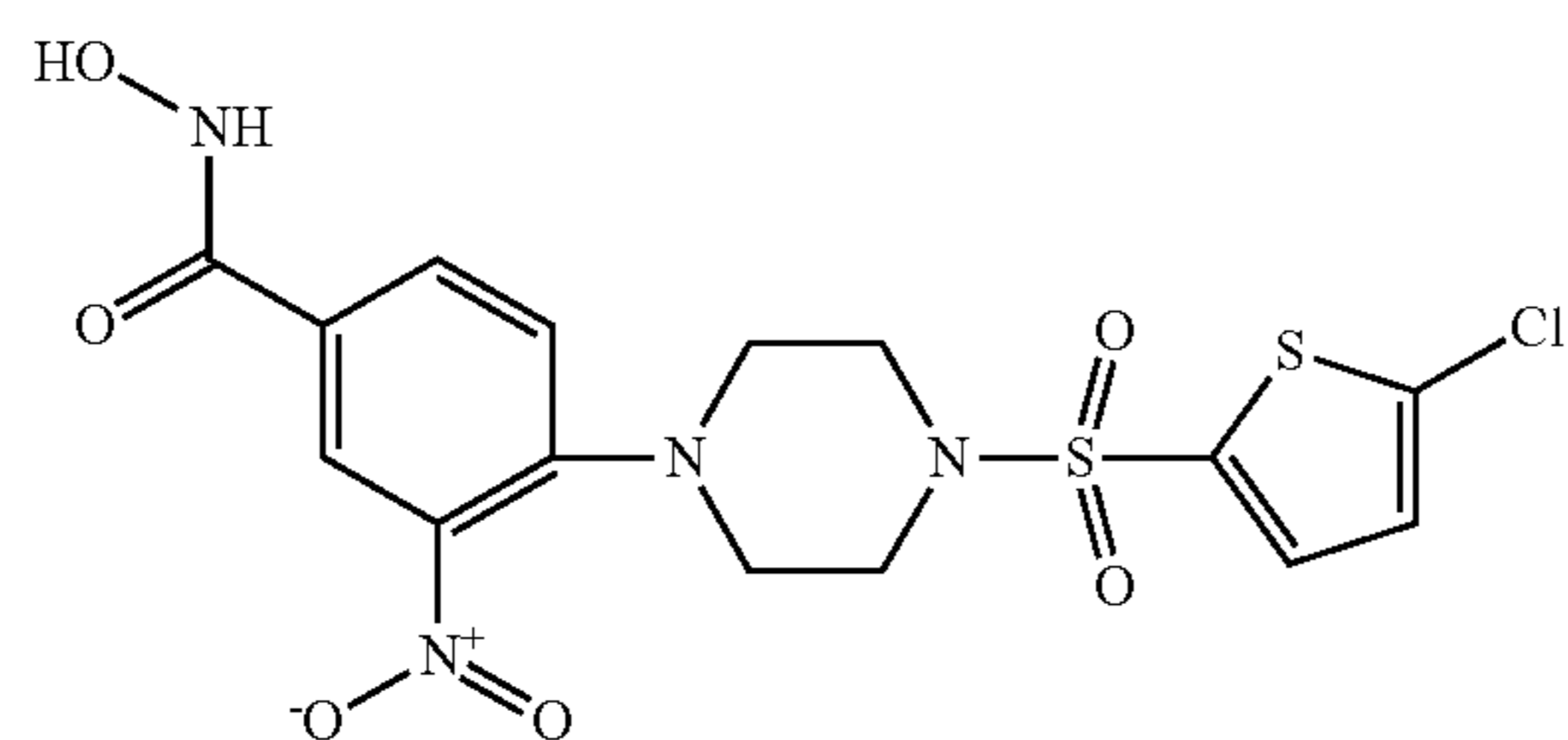
\bullet C_2HF_3O_2 (1:1), Co. No. 20; Ex. [B1]; ms. 447
