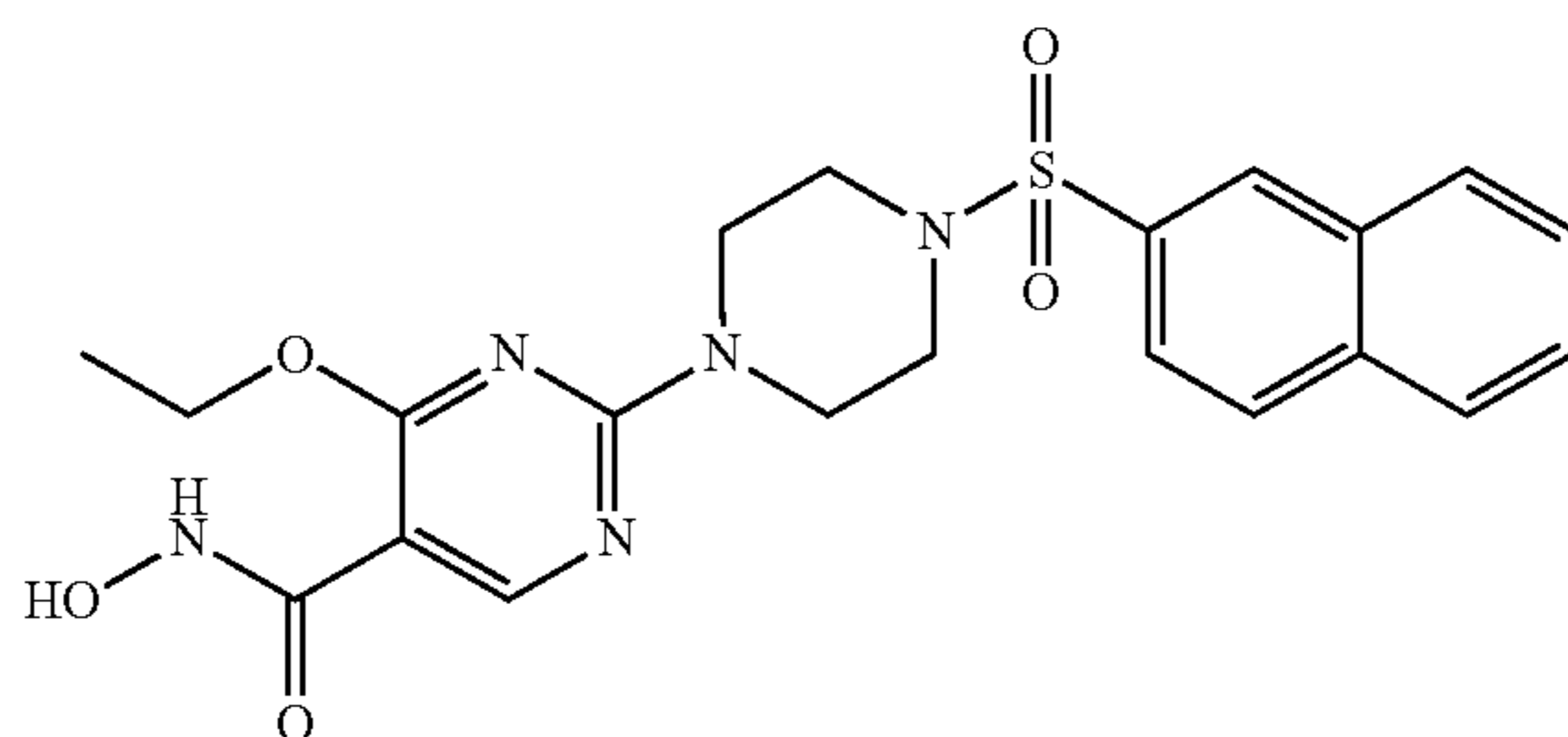
Co. No. 12; Ex. [B13]; mp. 197° C.
