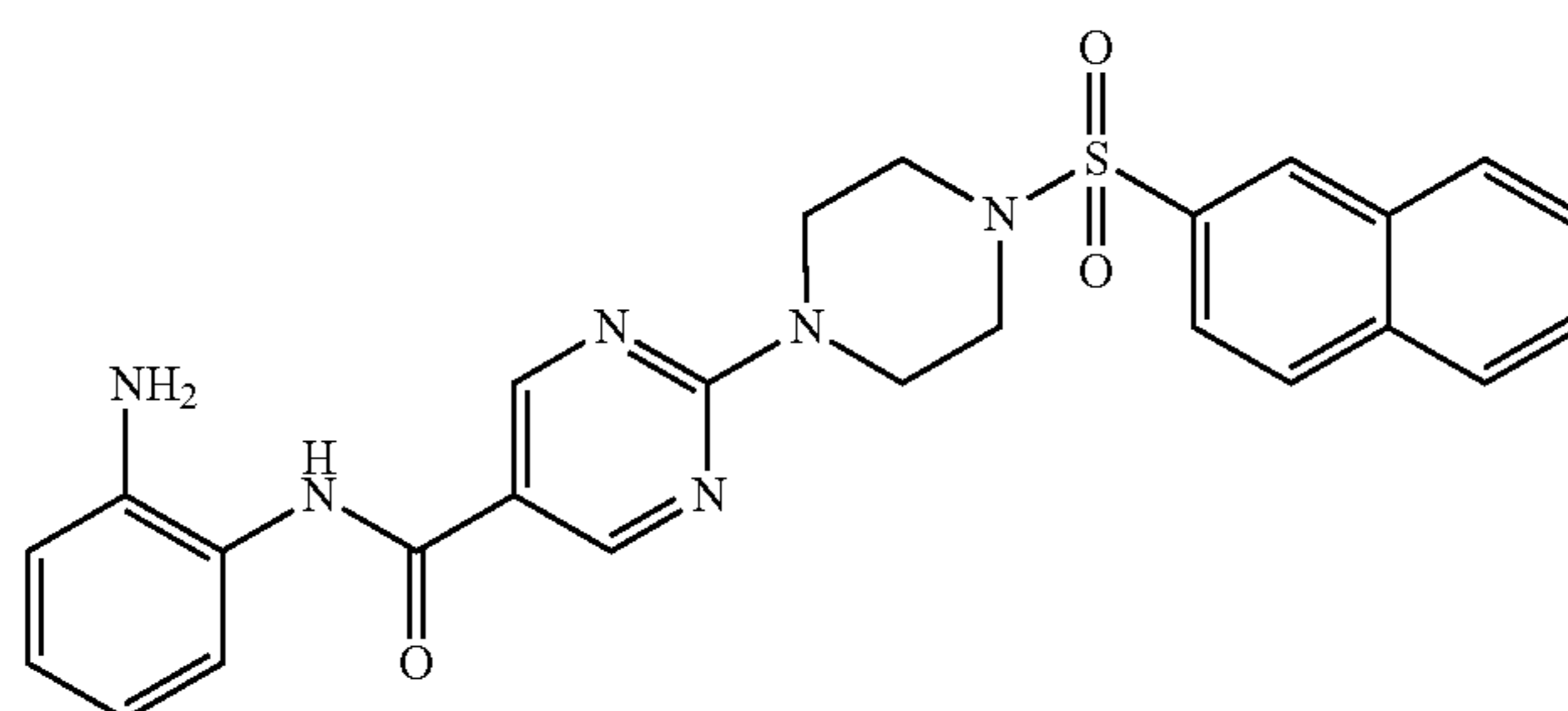
Co. No. 13; Ex. [B14]; mp. 238° C.
