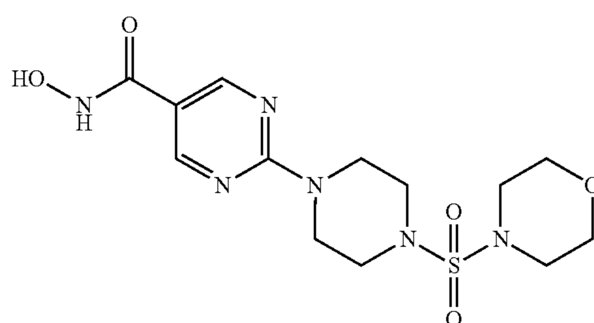
Co. No. 14; Ex. [B15]; MH + = 373
