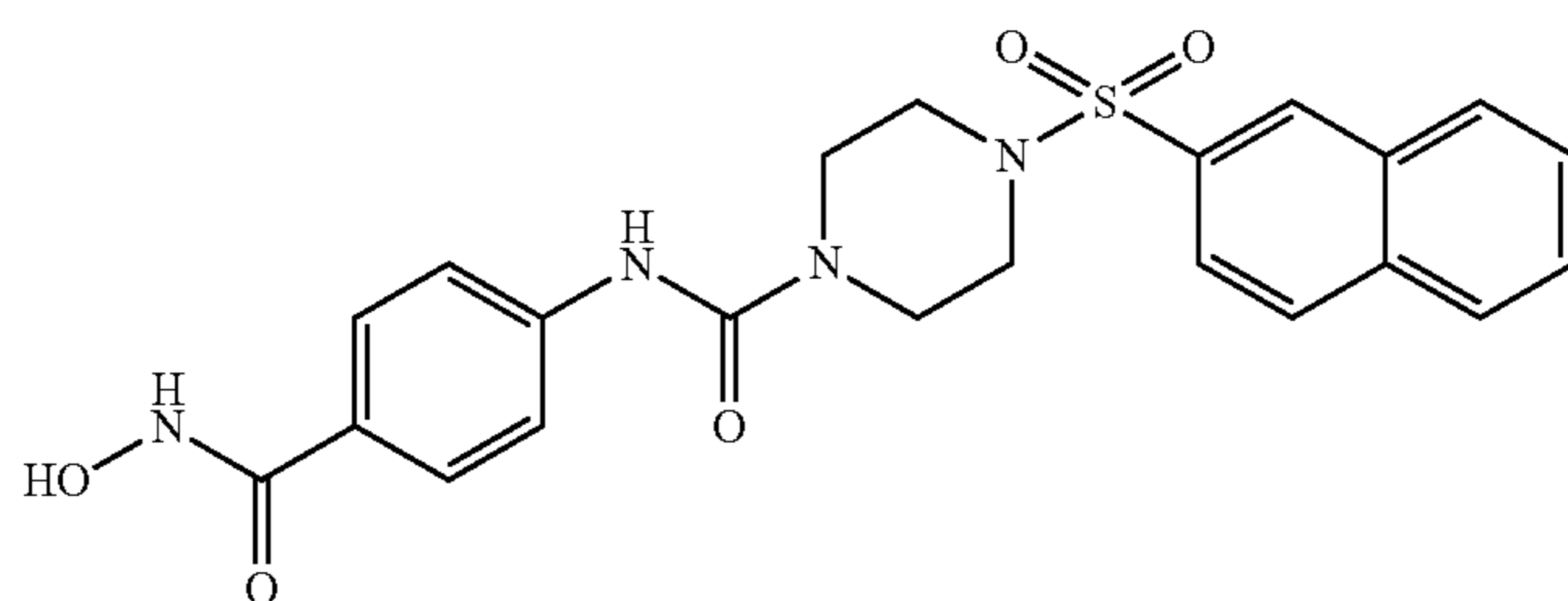
Co. No. 8; Ex. [B9]
