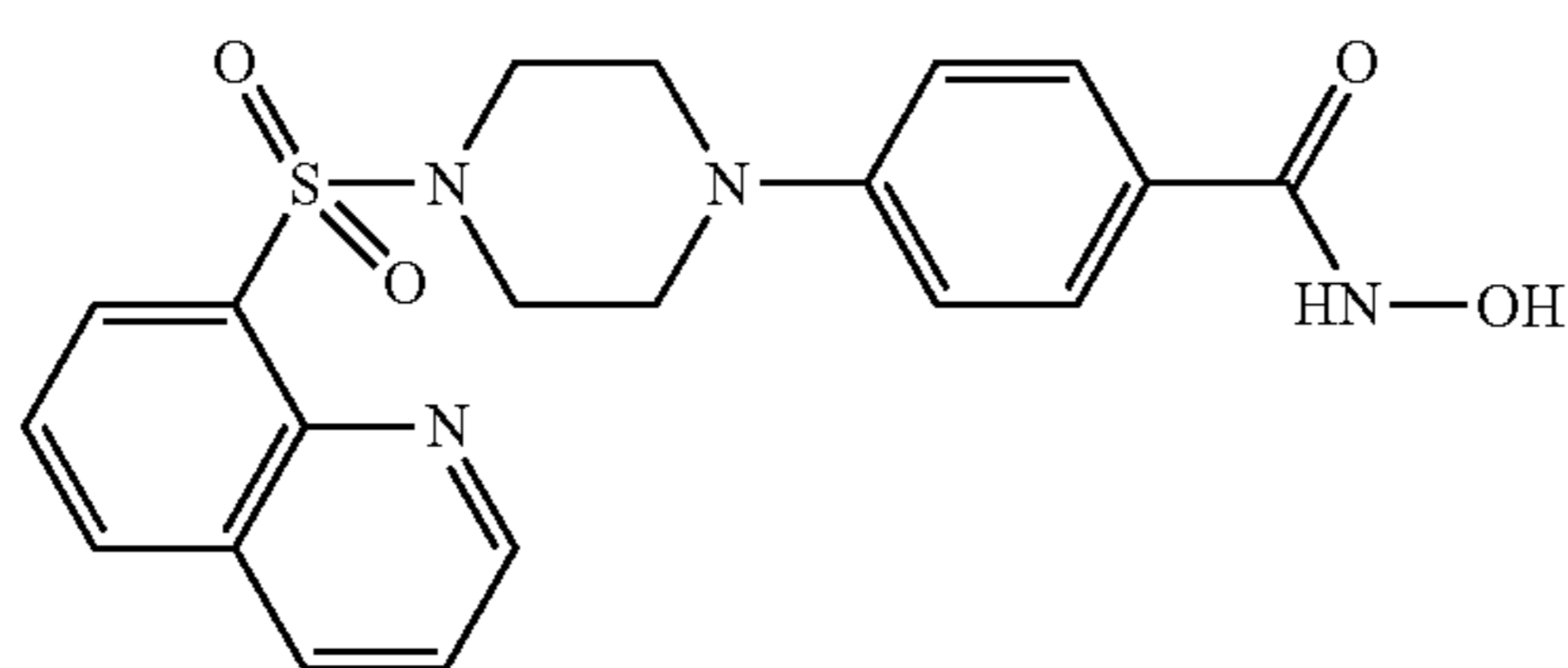
Co. No. 71; Ex. [B1]
