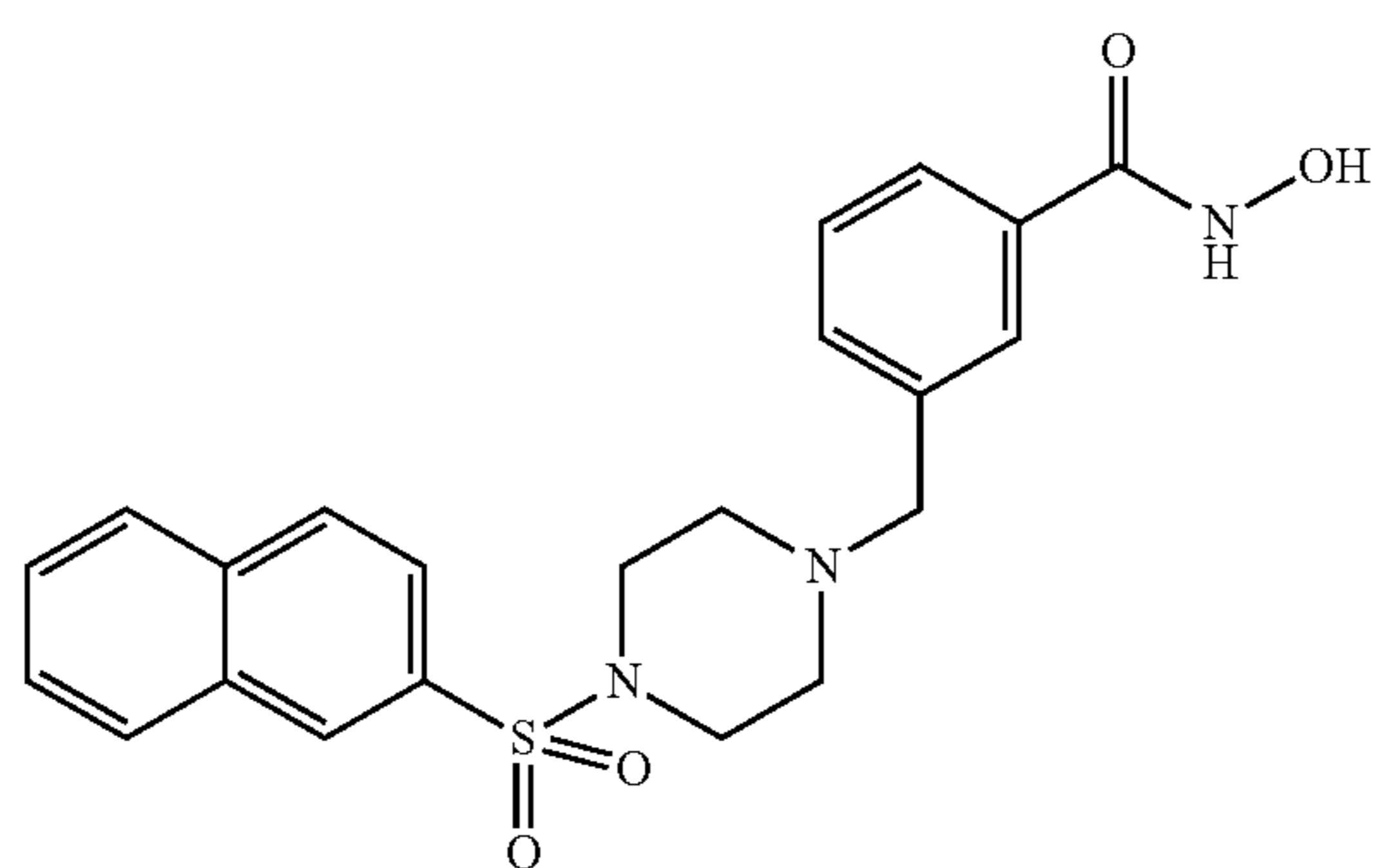
Co. No. 7; Ex. [B8]
