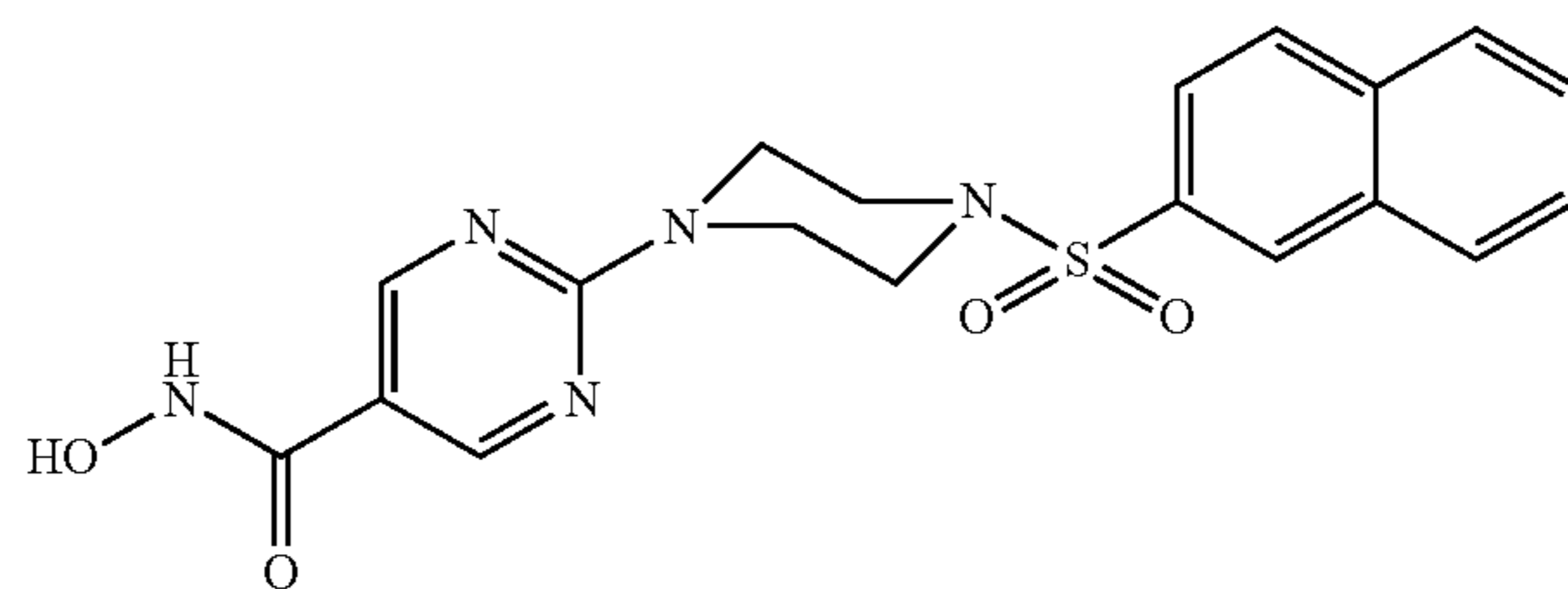
Co. No. 6; Ex. [B7]; mp. 265° C.
