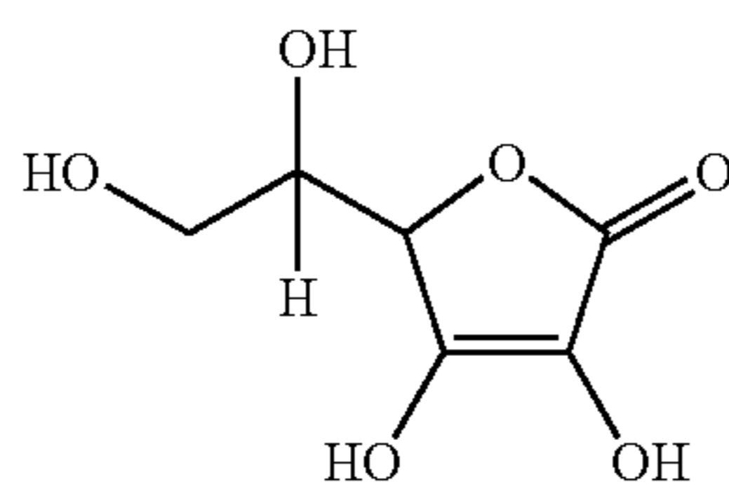
Ascorbic Acid
