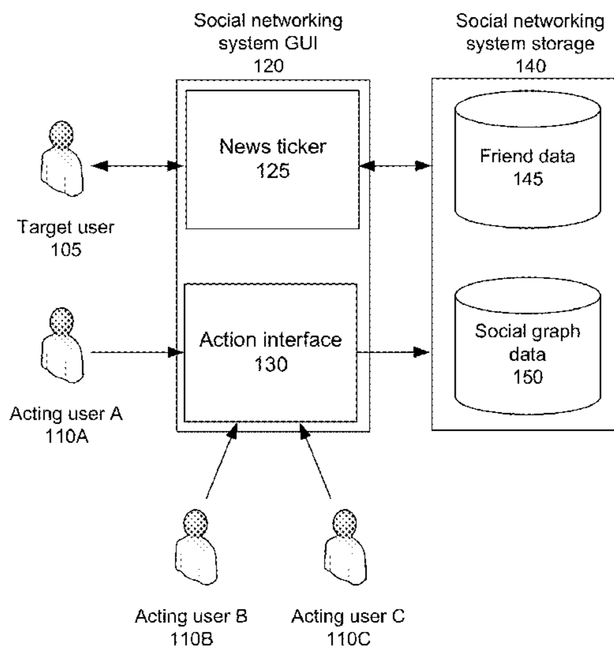
Social Networking System 100
