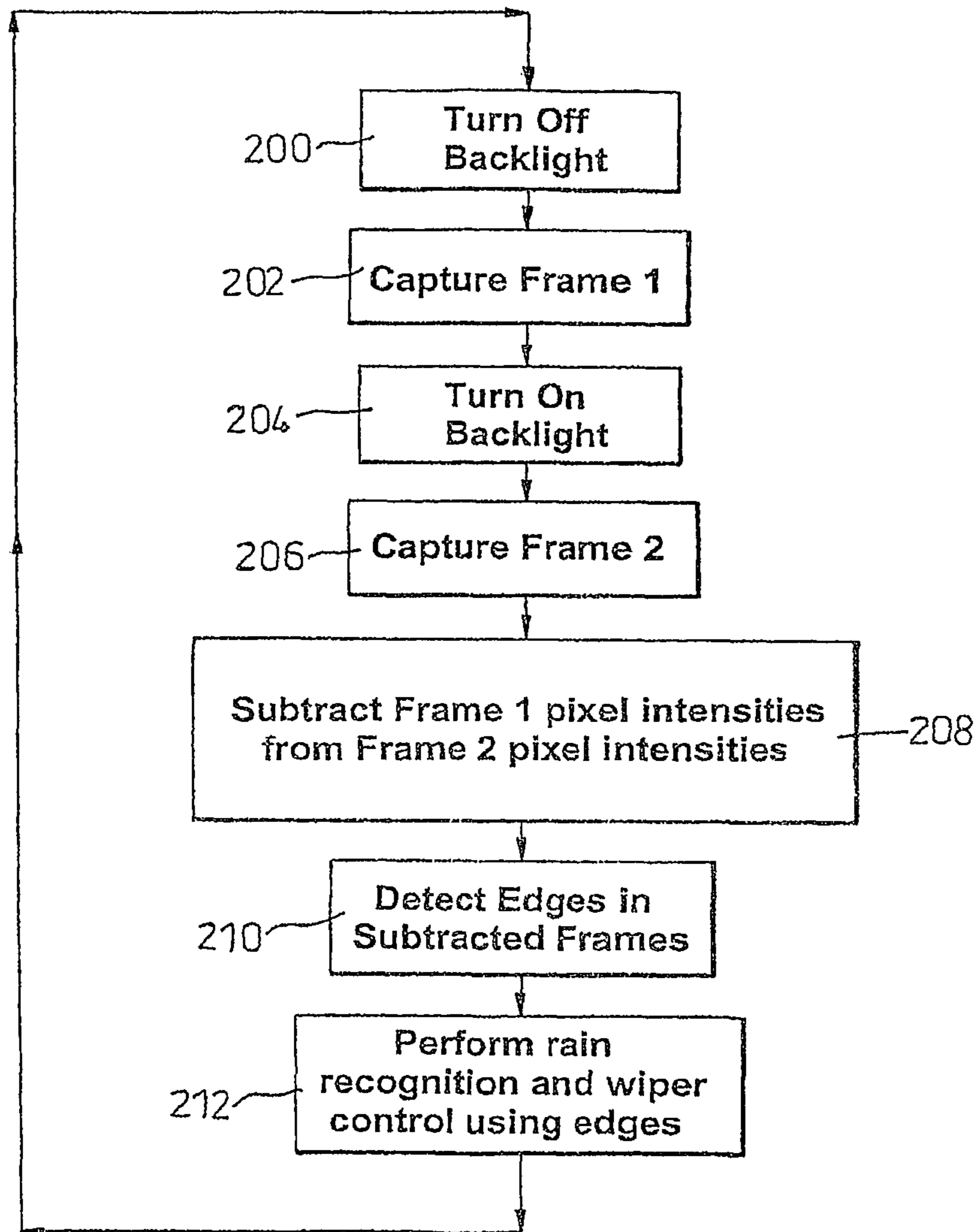
Frame Subtraction Control Diagram
