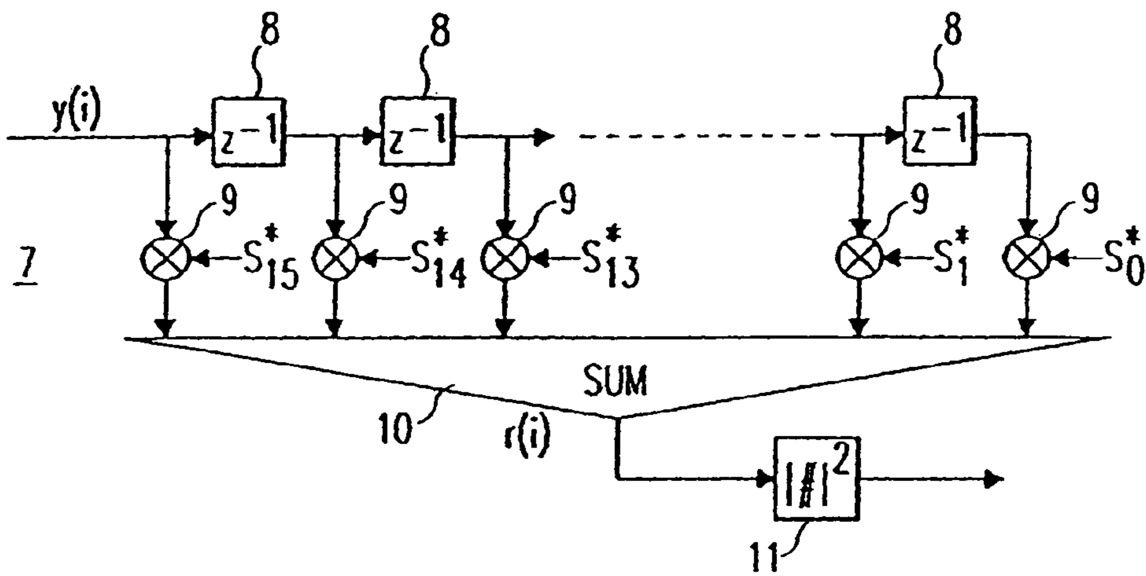
Fig. 2 (PRIOR ART)
