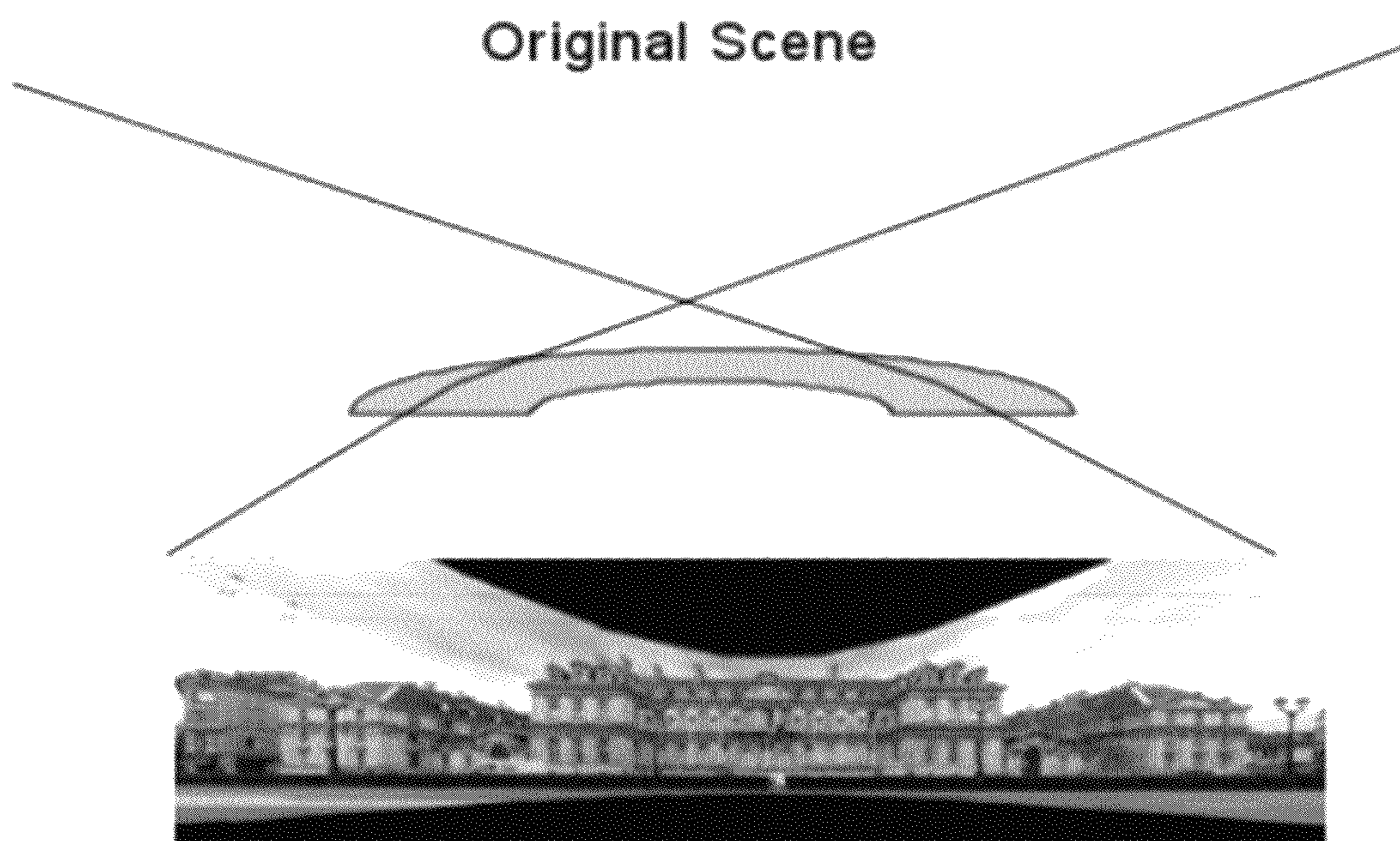
Scene Mapped onto Image Sensor
