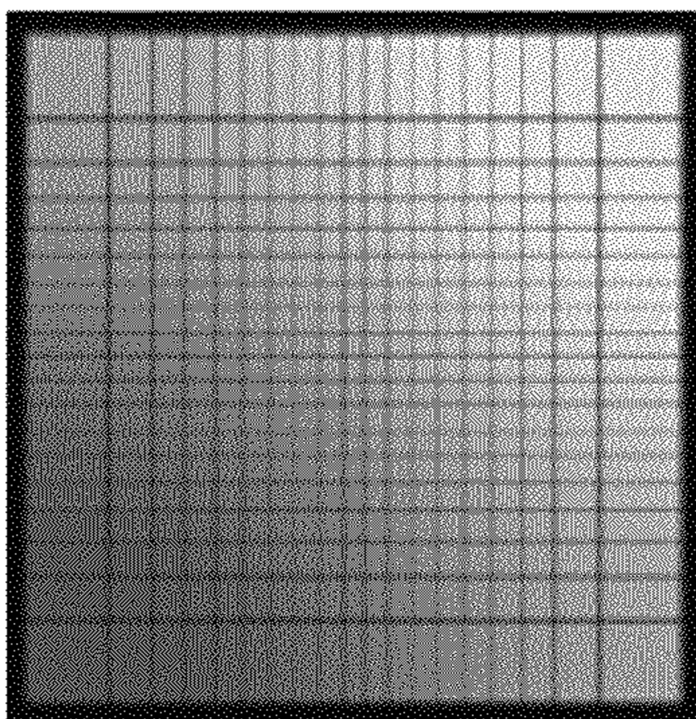
f(x) Applied to Cartesians Axes
