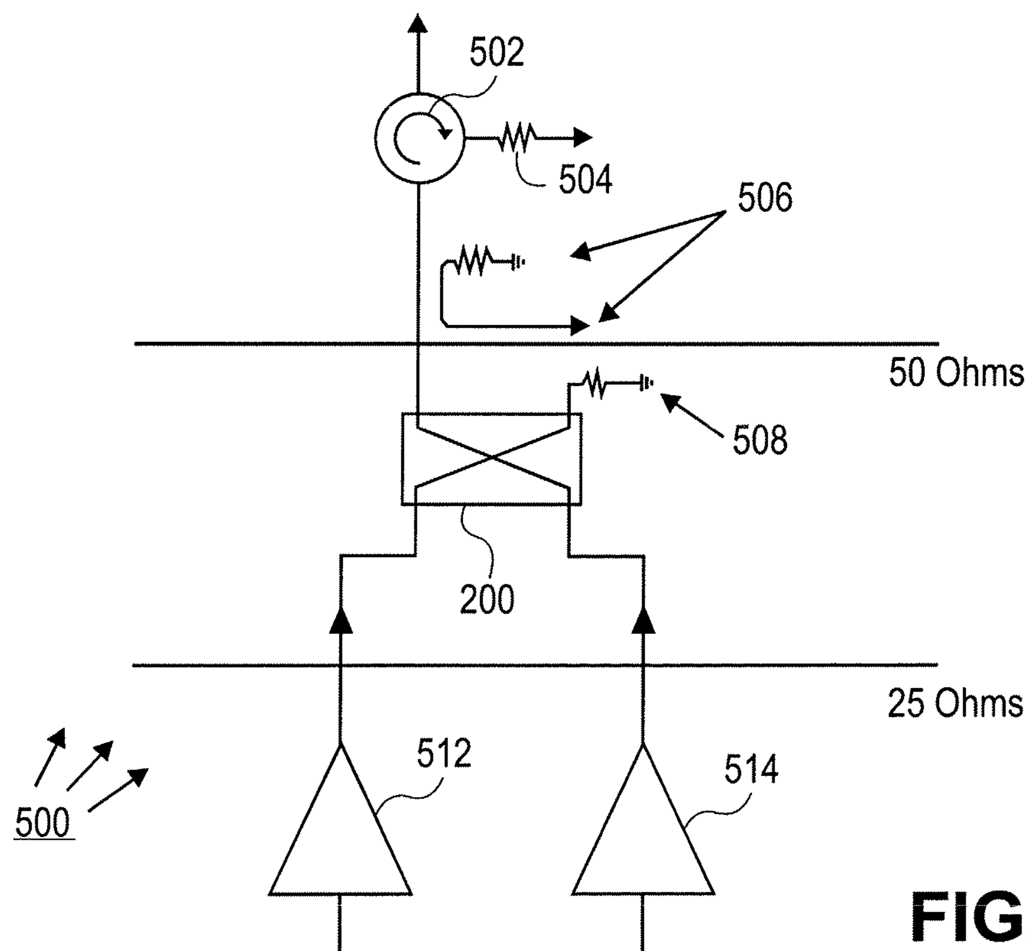
FIG. 6 (PRIOR ART)
