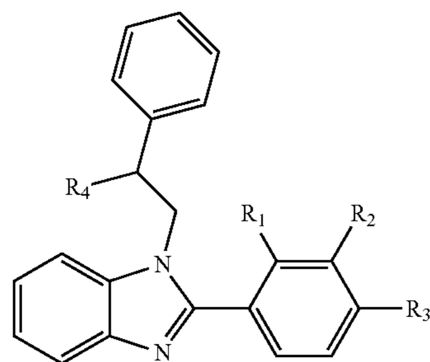
Scheme 1
