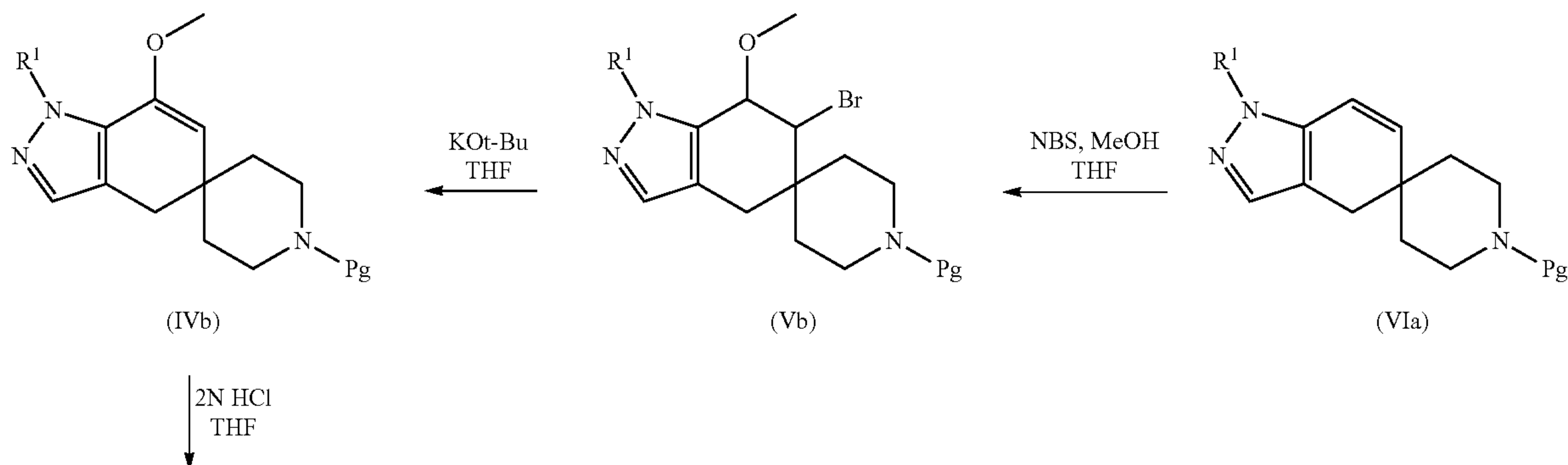
Reaction Scheme II
