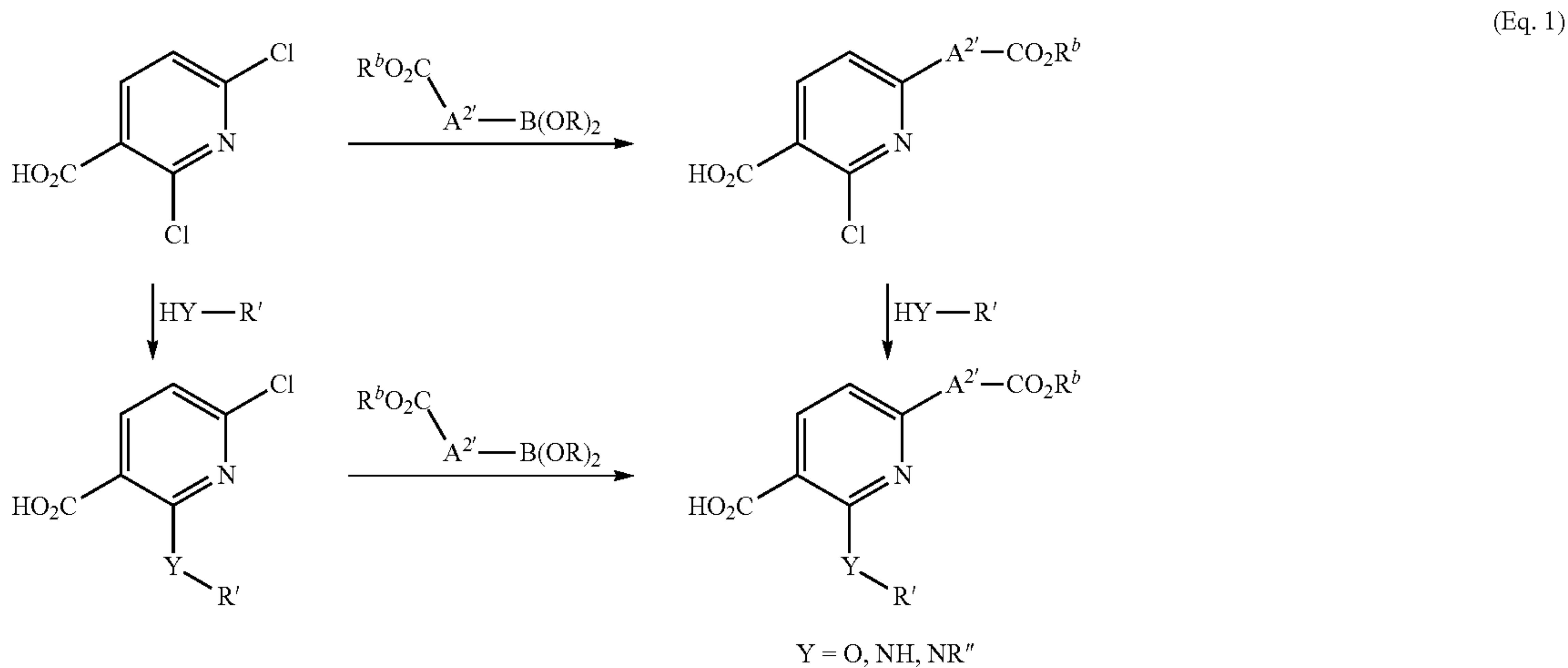
Reaction Scheme IX
