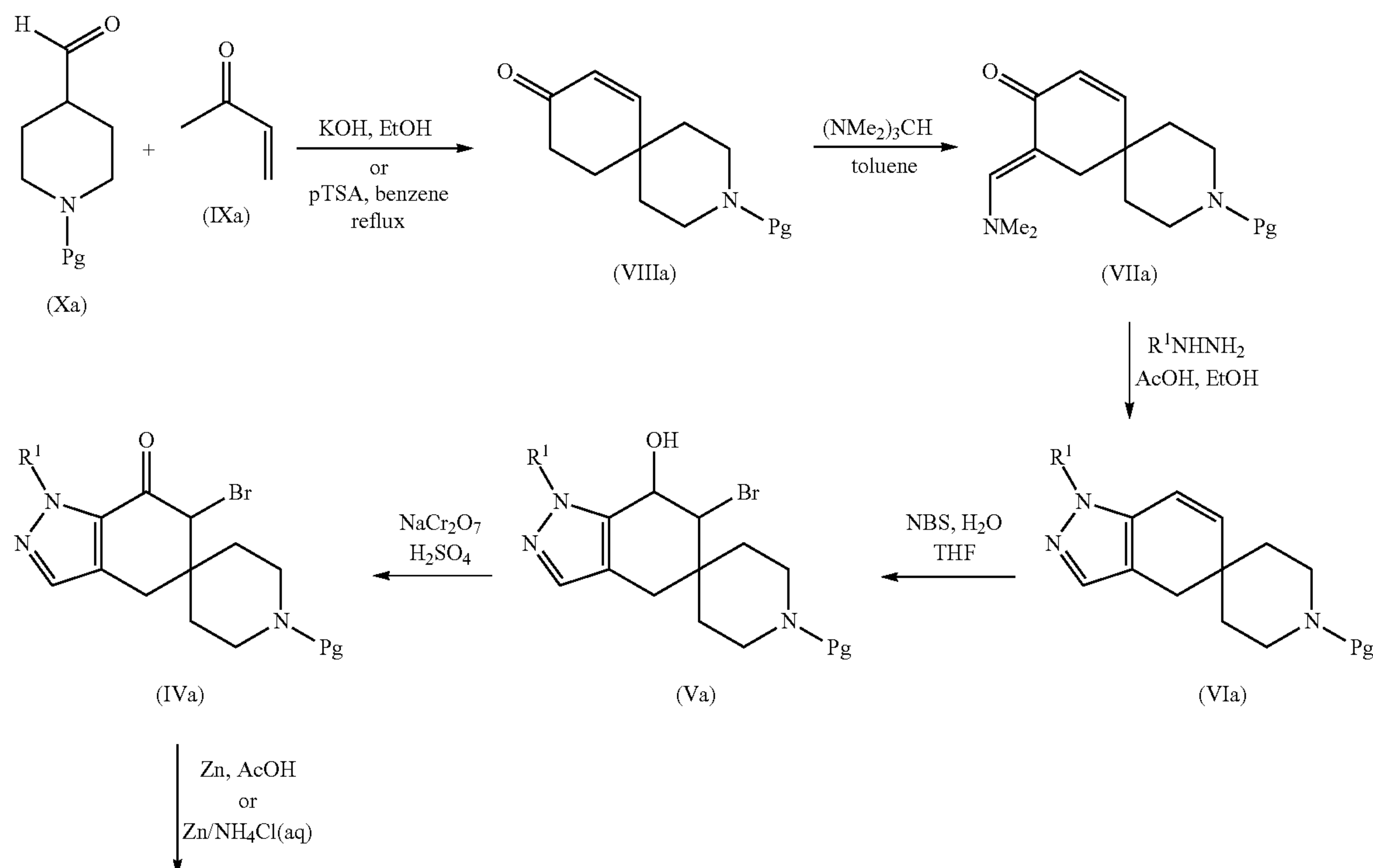
Reaction Scheme IA
