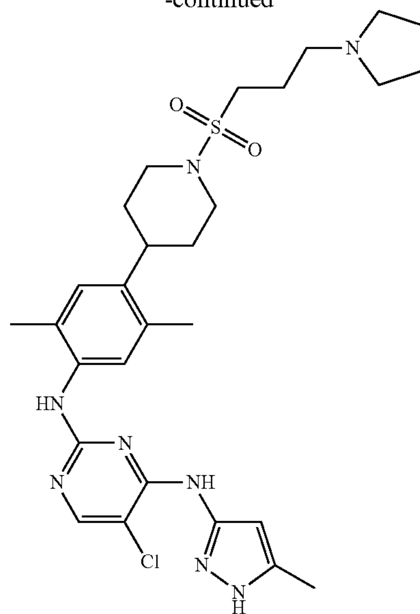
5-chloro-N2-(2,5-dimethyl-4-(1-(3-(pyrrolidin-1-yl)propylsulfonyl)piperidin-4-yl)phenyl)-N4-(5-methyl-1H-pyrazol-3-yl)pyrimidine-2,4-diamine
