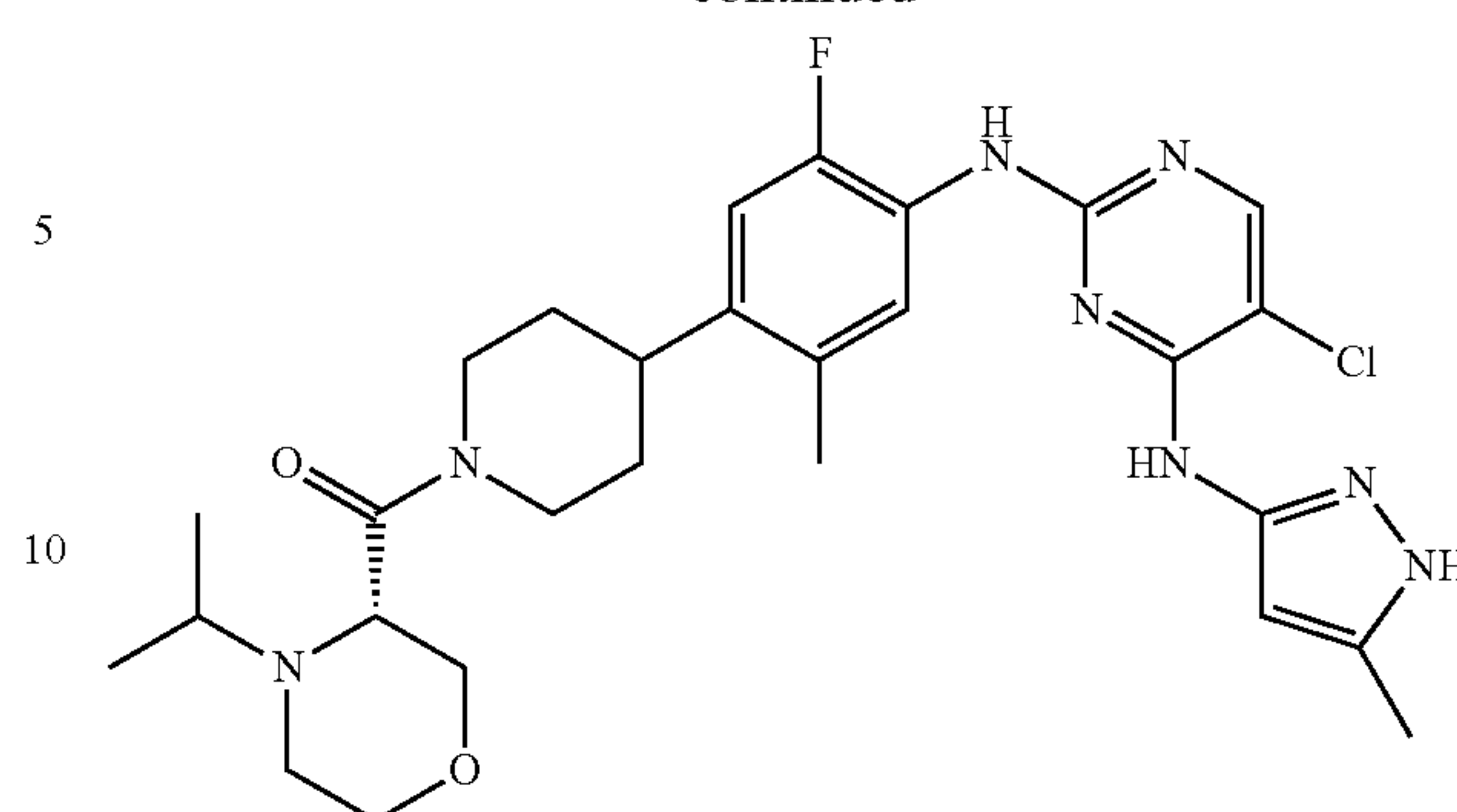
(S)-(4-(4-(5-chloro-4-(5-methyl-1H-pyrazol-3-ylamino)pyrimidin-2-ylamino)-5-fluoro-2-methylphenyl)piperidin-1-yl)(4-isopropylmorpholin-3-yl)methanone
