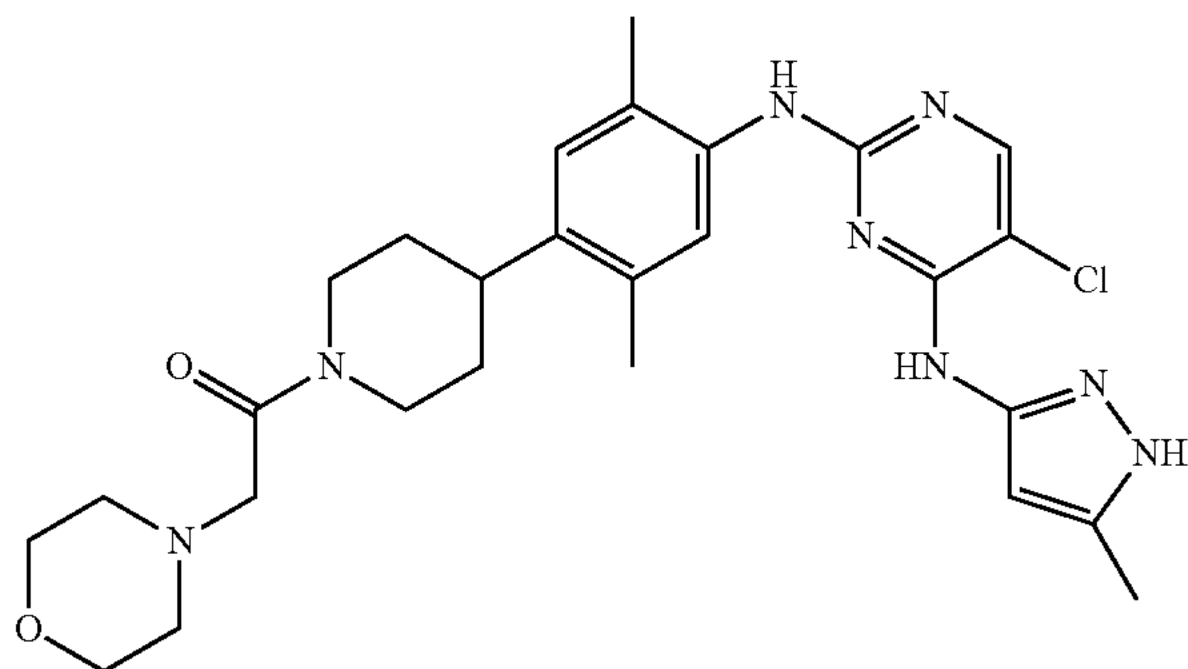
1-(4-(4-(5-chloro-4-(5-methyl-1H-pyrazol-3-ylamino)pyrimidin-2-ylamino)-2,5-dimethylphenyl)piperidin-1-yl)-2-morpholinoethanone
