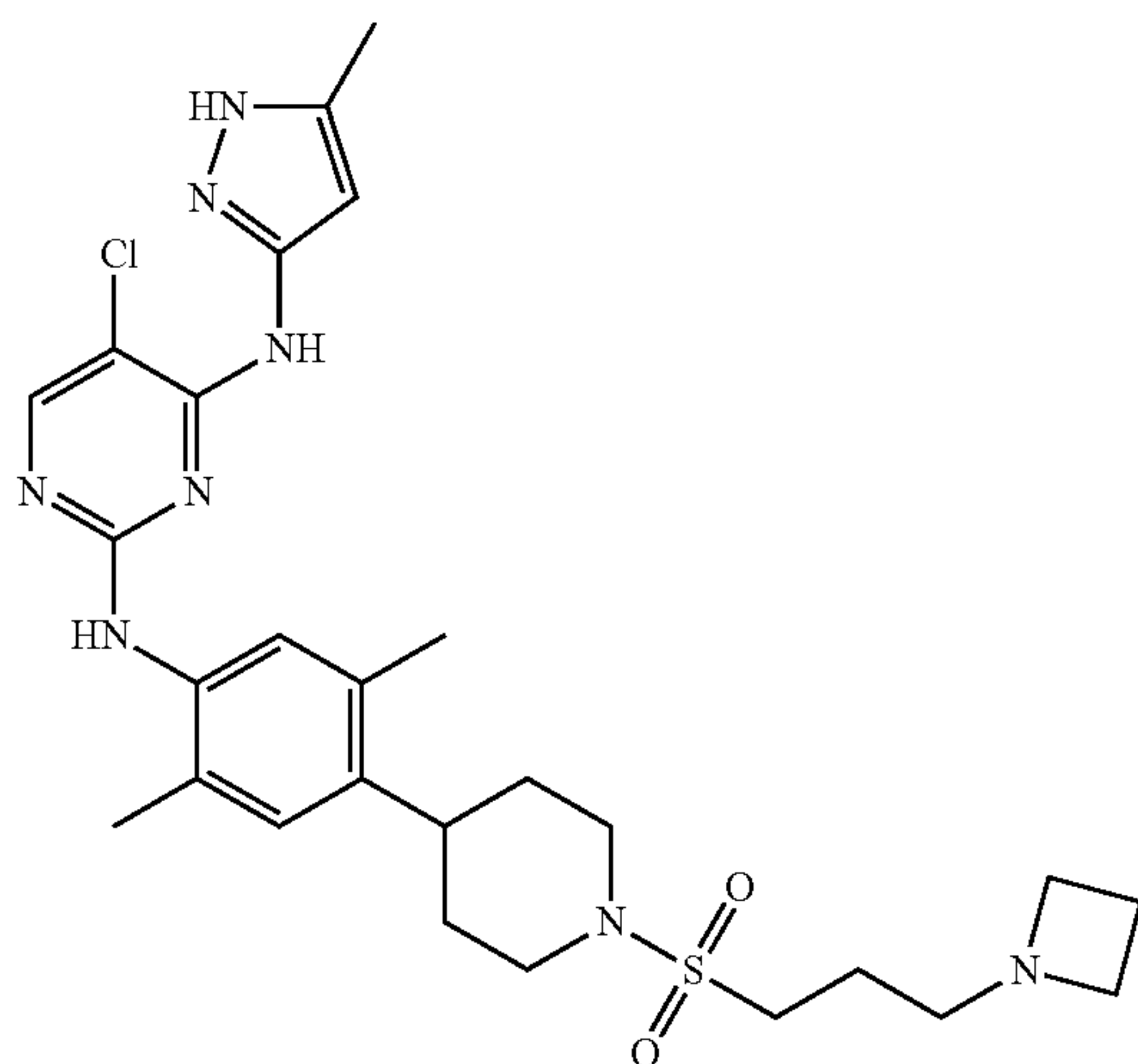
N2-(4-(1-(3-(azetidin-1-yl)propylsulfonyl)piperidin-4-yl)-2,5-dimethylphenyl)-5-chloro-N4-(5-methyl-1H-pyrazol-3-yl)pyrimidine-2,4-diamine
