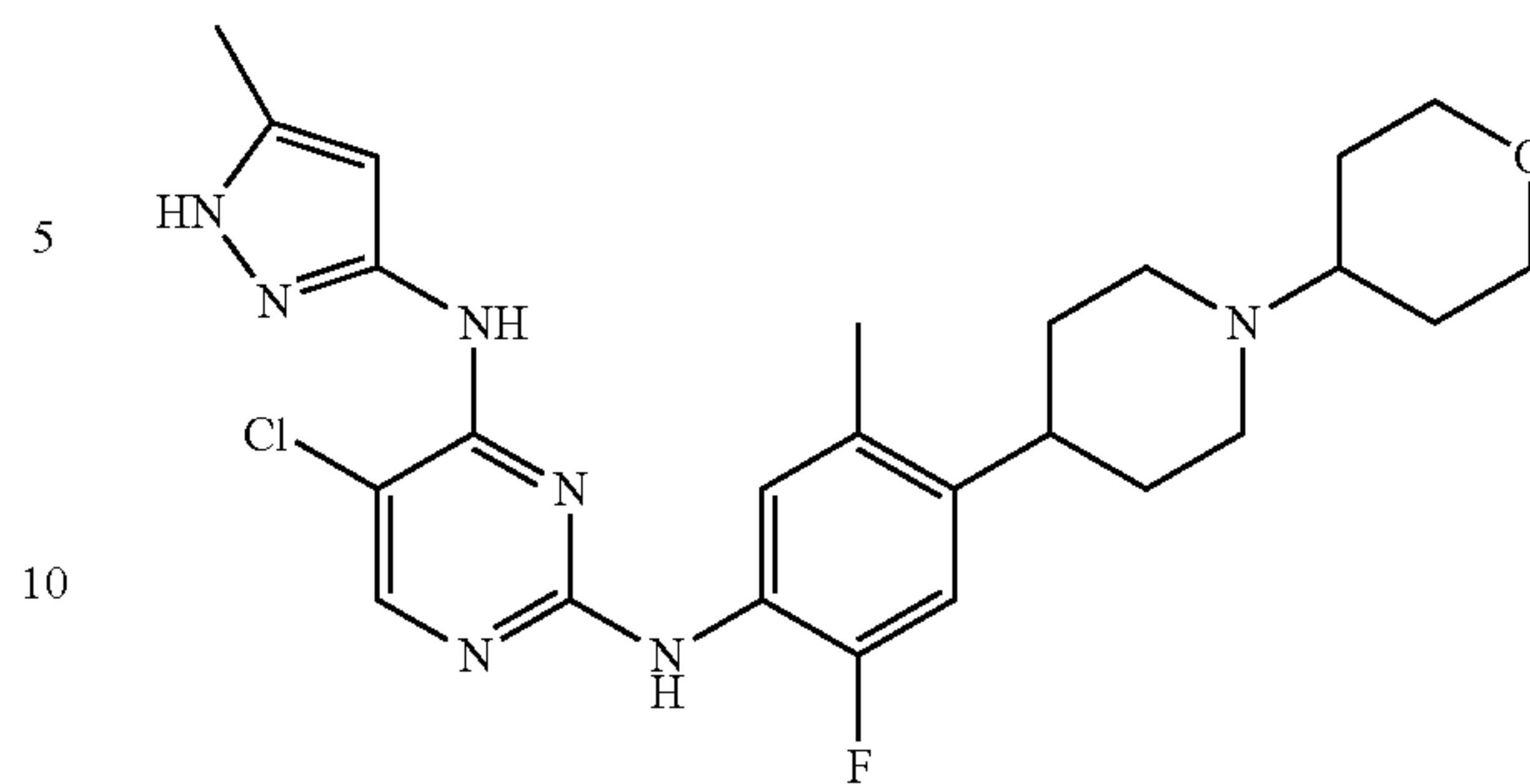
5-chloro-N2-(2-fluoro-5-methyl-4-(1-(tetrahydro-2H-pyran-4-yl)piperidin-4-yl)phenyl)-N4-(5-methyl-1H-pyrazol-3-yl)pyrimidine-2,4-diamine
