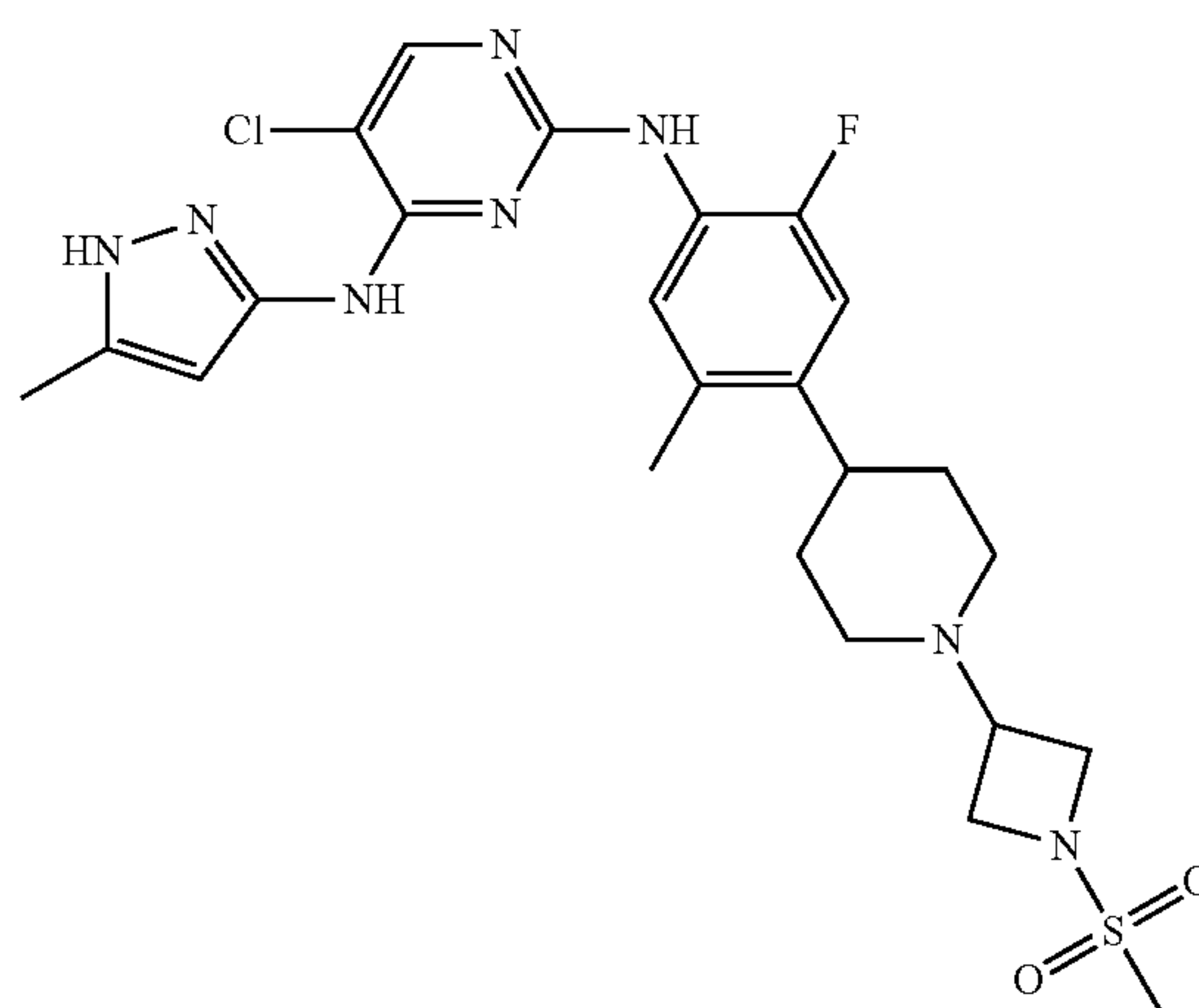
5-chloro-N2-(2-fluoro-5-methyl-4-(1-(1-(methylsulfonyl)azetidin-3-yl)piperidin-4-yl)phenyl)-N4-(5-methyl-1H-pyrazol-3-yl)pyrimidine-2,4-diamine
