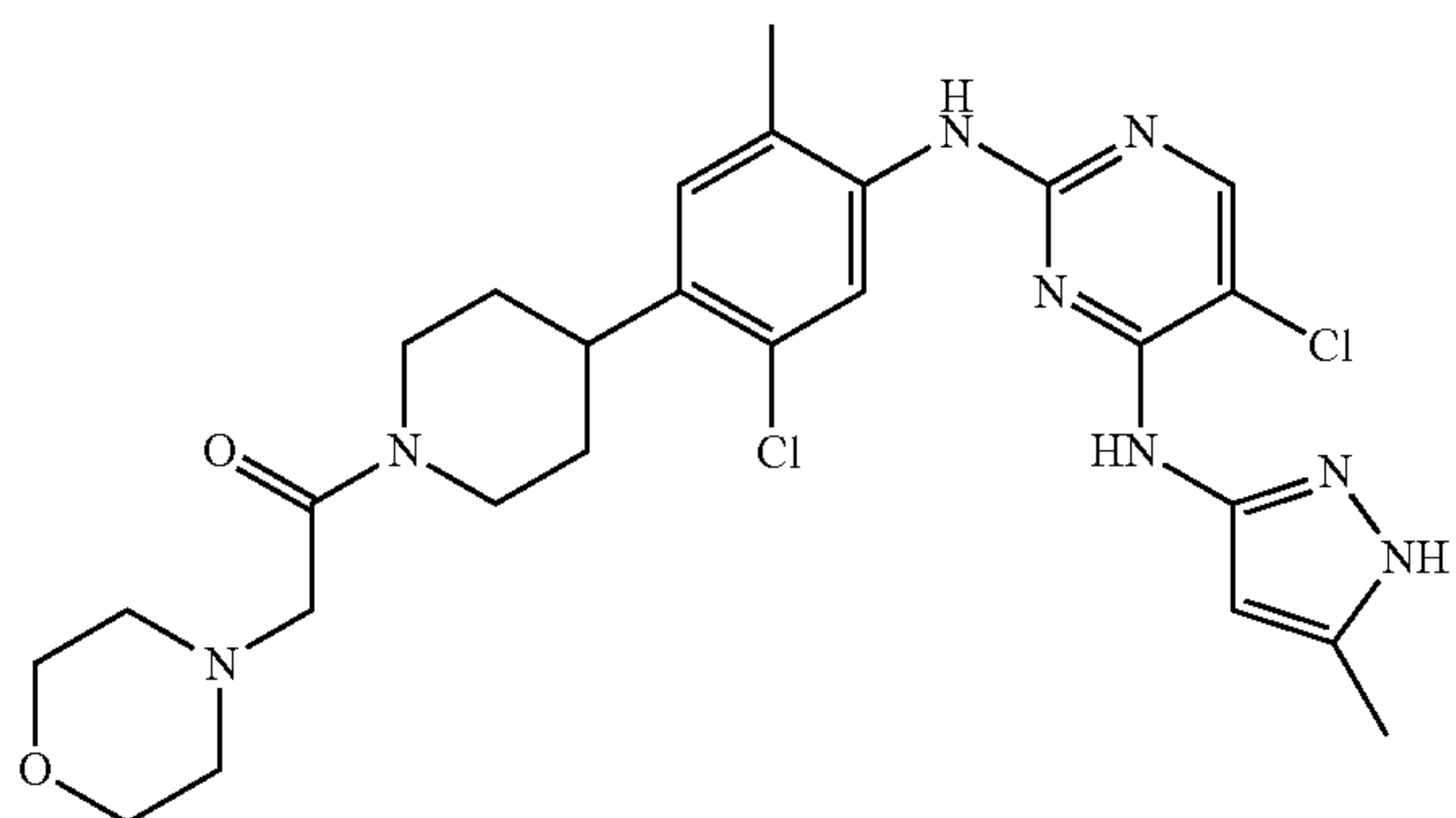
1-(4-(2-chloro-4-(5-chloro-4-(5-methyl-1H-pyrazol-3-ylamino)pyrimidin-2-ylamino)-5-methylphenyl)piperidin-1-yl)-2-morpholinoethanone
