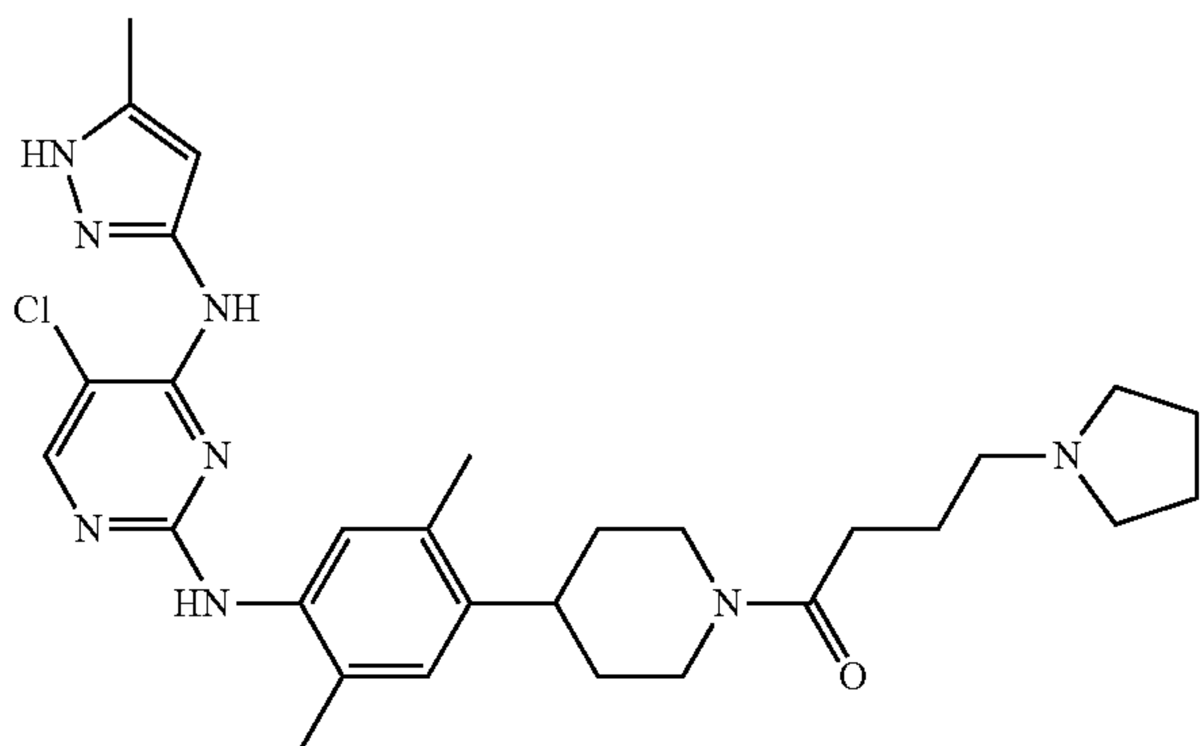
1-(4-(4-(5-chloro-4-(5-methyl-1H-pyrazol-3-ylamino)pyrimidin-2-ylamino)-2,5-dimethylphenyl)piperidin-1-yl)-4-(pyrrolidin-1-yl)butane-1-one
