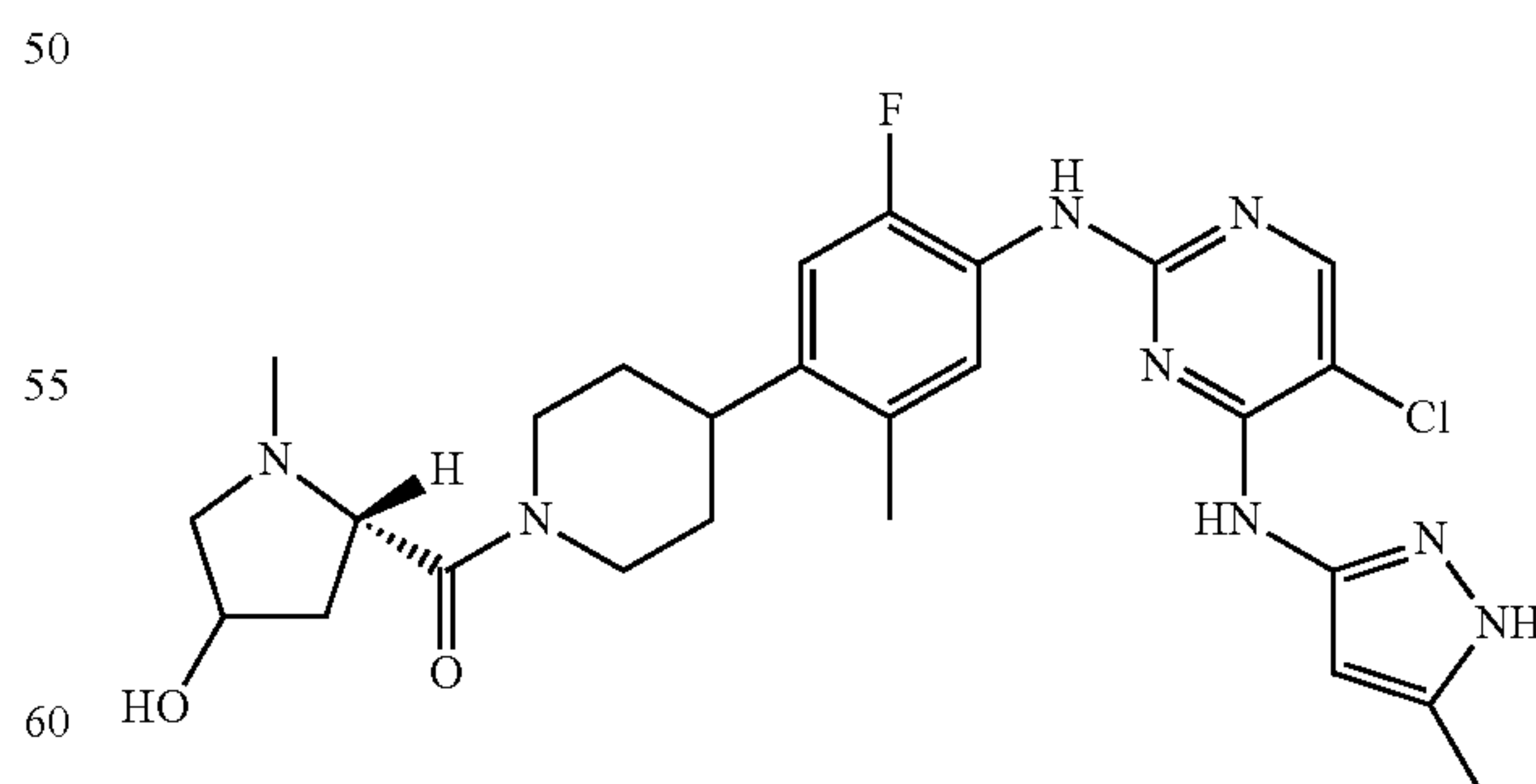
(4-(4-(5-chloro-4-(5-methyl-1H-pyrazol-3-ylamino)pyrimidin-2-ylamino)-5-fluoro-2-methylphenyl)piperidin-1-yl)((2S)-4-hydroxy-1-methylpyrrolidin-2-yl)methanone
