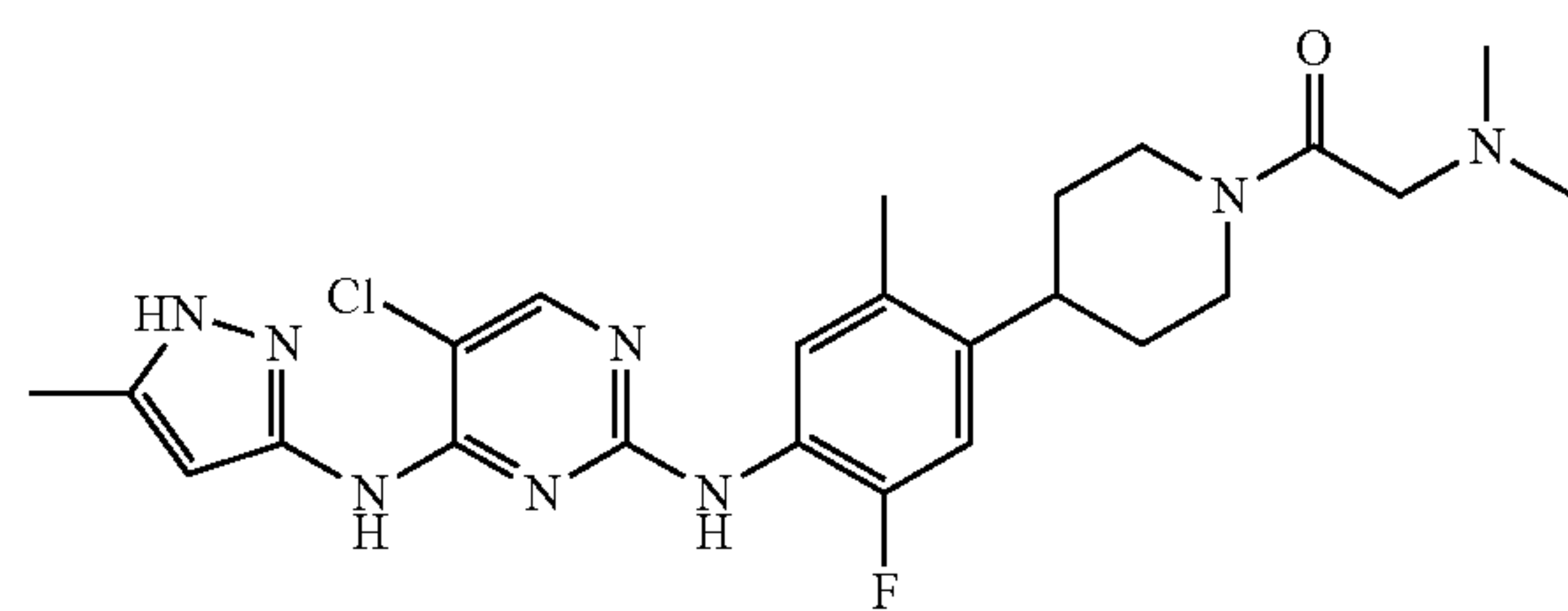
1-(4-(4-(5-chloro-4-(5-methyl-1H-pyrazol-3-ylamino)pyrimidin-2-ylamino)-5-fluoro-2-methylphenyl)piperidin-1-yl)-2-(dimethylamino)ethanone
