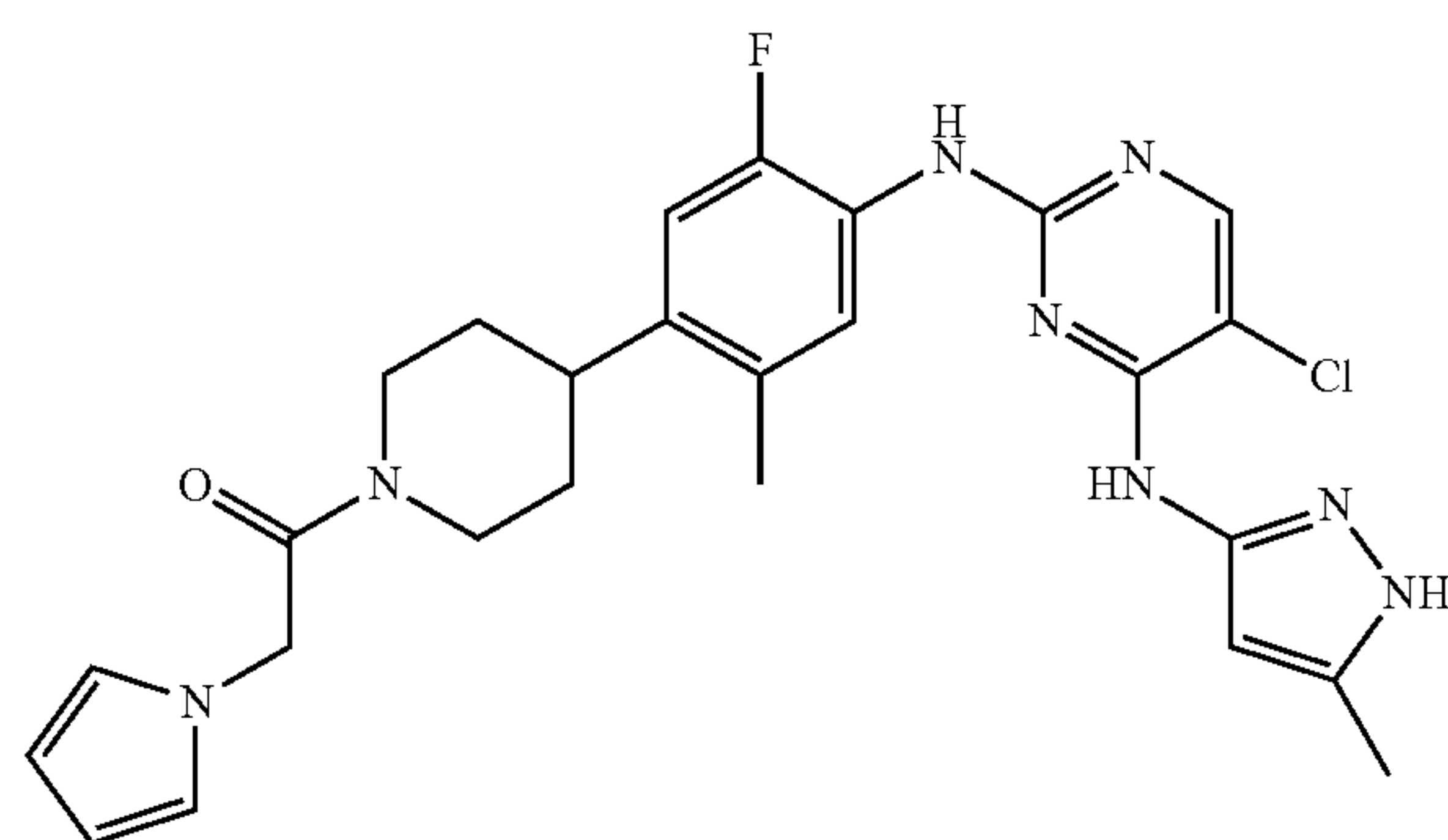
1-(4-(4-(5-chloro-4-(5-methyl-1H-pyrazol-3-ylamino)pyrimidin-2-ylamino)-5-fluoro-2-methylphenyl)piperidin-1-yl)-2-(1H-pyrrol-1-yl)ethanone
