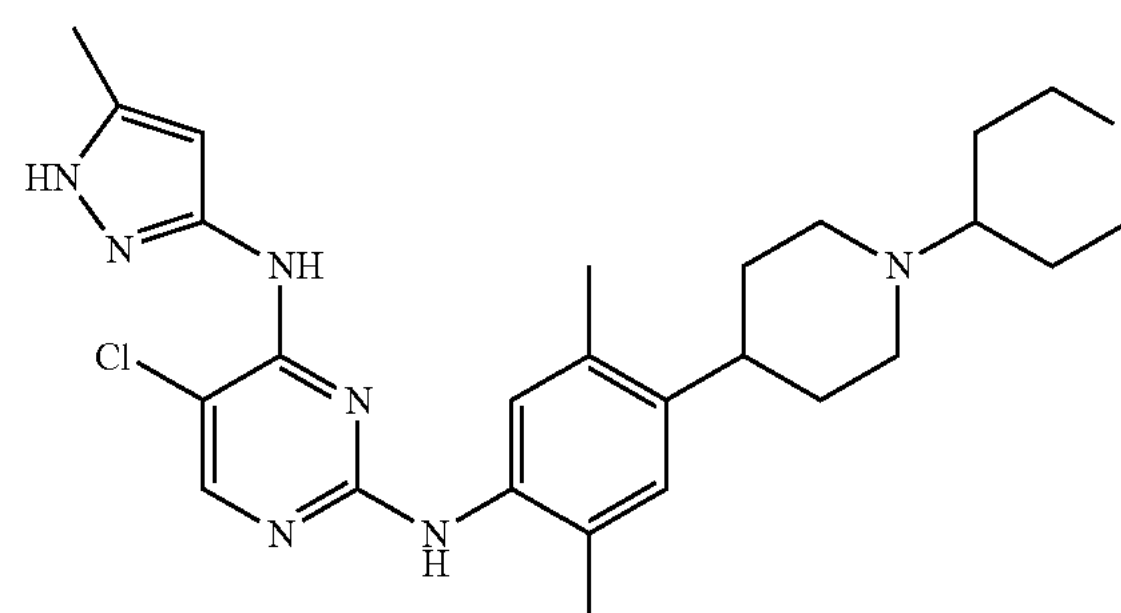
5-chloro-N2-(2,5-dimethyl-4-(1-(tetrahydro-2H-thiopyran-4-yl)piperidin-4-yl)phenyl)-N4-(5-methyl-1H-pyrazol-3-yl)pyrimidine-2,4-diamine
