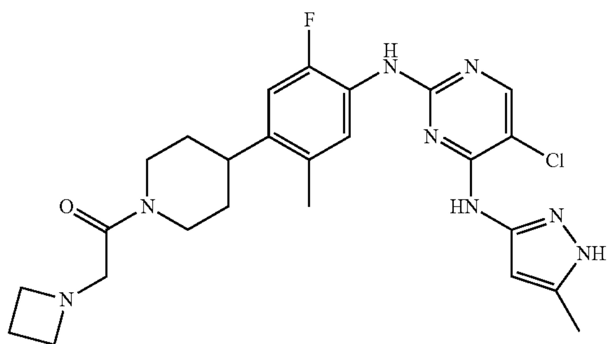
2-(azetidin-1-yl)-1-(4-(4-(5-chloro-4-(5-methyl-1H-pyrazol-3-ylamino)pyrimidin-2-ylamino)-5-fluoro-2-methylphenyl)piperidin-1-yl)ethanone
