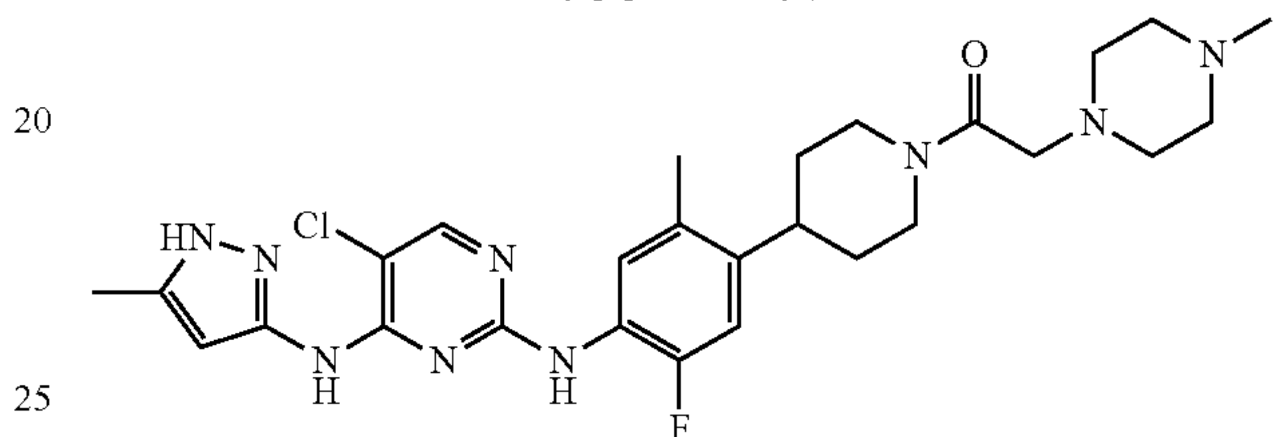
1-(4-(4-(5-chloro-4-(5-methyl-1H-pyrazol-3-ylamino)pyrimidin-2-ylamino)-5-fluoro-2-methylphenyl)piperidin-1-yl)-2-(4-methylpiperidin-1-yl)ethanone
