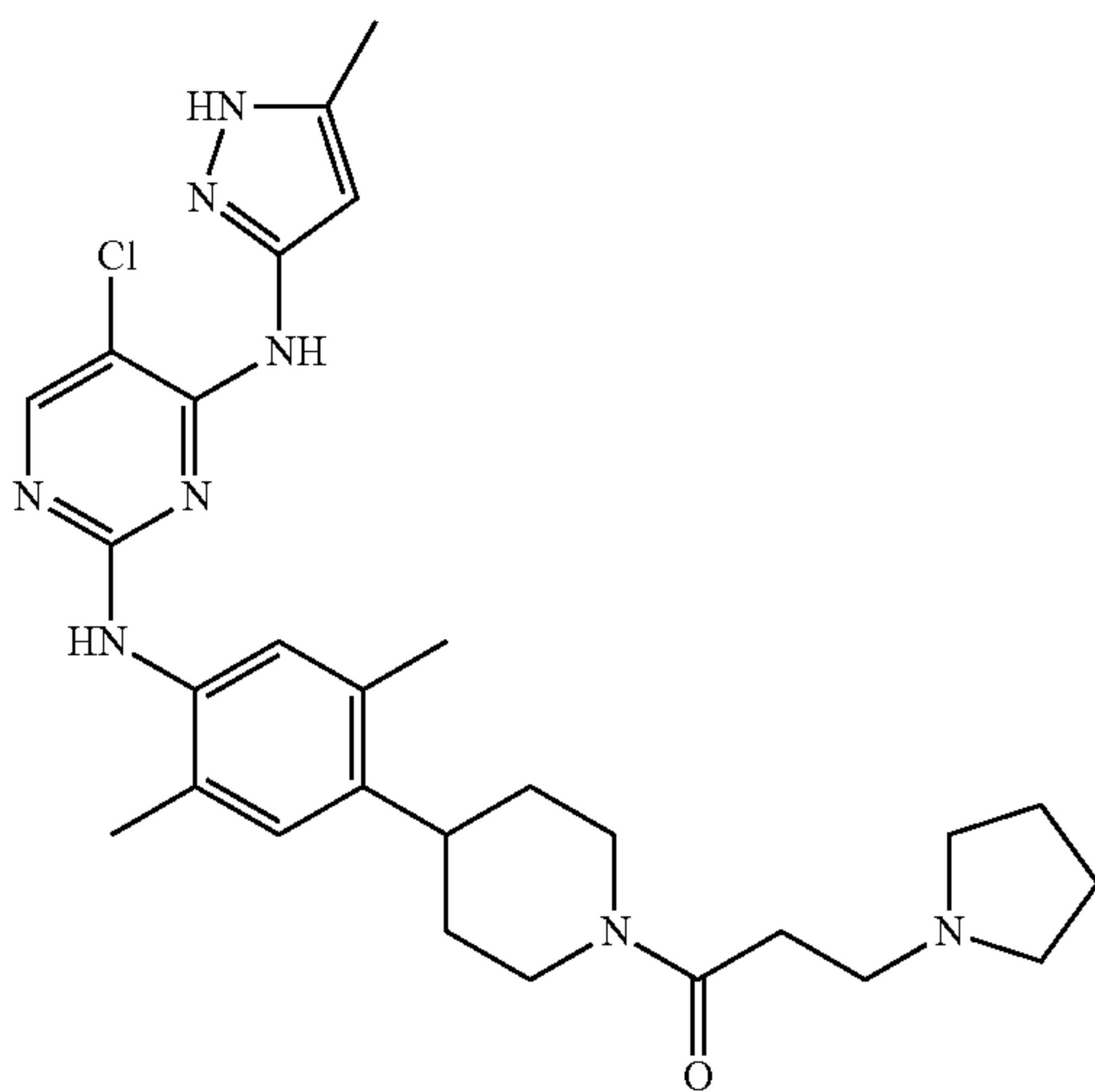
1-(4-(4-(5-chloro-4-(5-methyl-1H-pyrazol-3-ylamino)pyrimidin-2-ylamino)-2,5-dimethylphenyl)piperidin-1-yl)-3-(pyrrolidin-1-yl)propan-1-one
