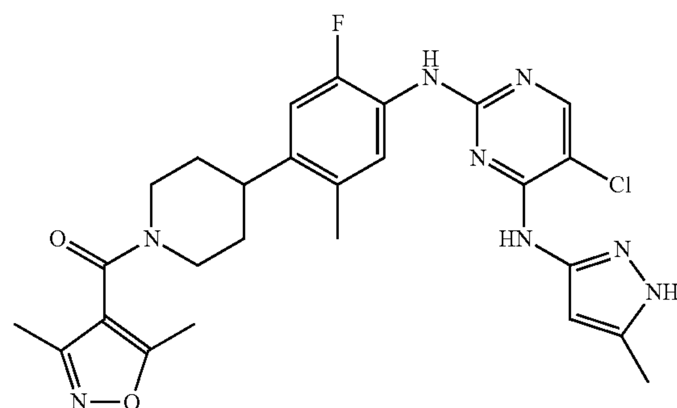
(4-(4-(5-chloro-4-(5-methyl-1H-pyrazol-3-ylamino)pyrimidin-2-ylamino)-5-fluoro-2-methylphenyl)piperidin-1-yl)(3,5-dimethylisoxazol-4-yl)methanone
