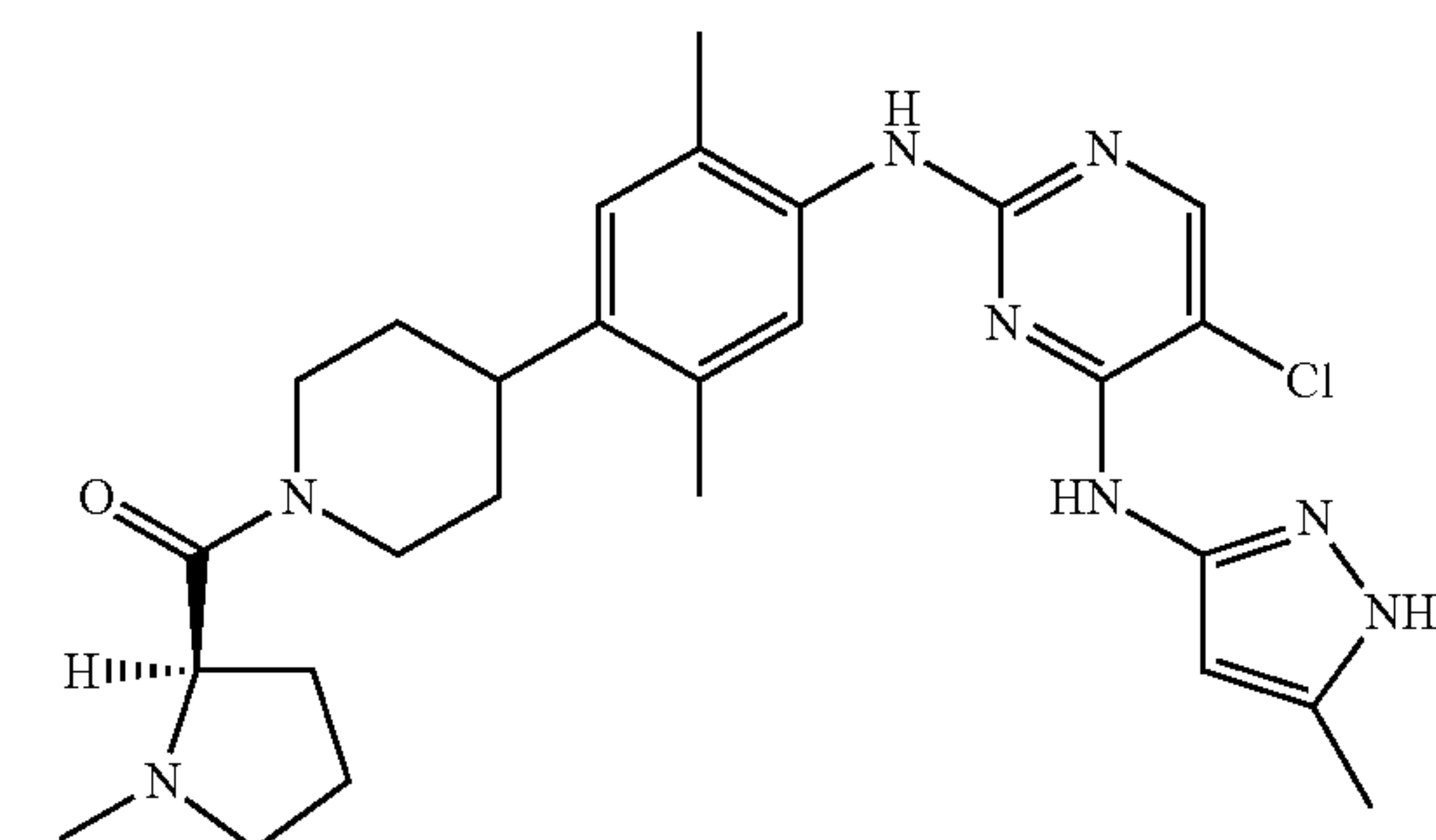
(R)-(4-(4-(5-chloro-4-(5-methyl-1H-pyrazol-3-ylamino)pyrimidin-2-ylamino)-2,5-dimethylphenyl)piperidin-1-yl)-1-methylpyrrolidin-2-yl)methanone
