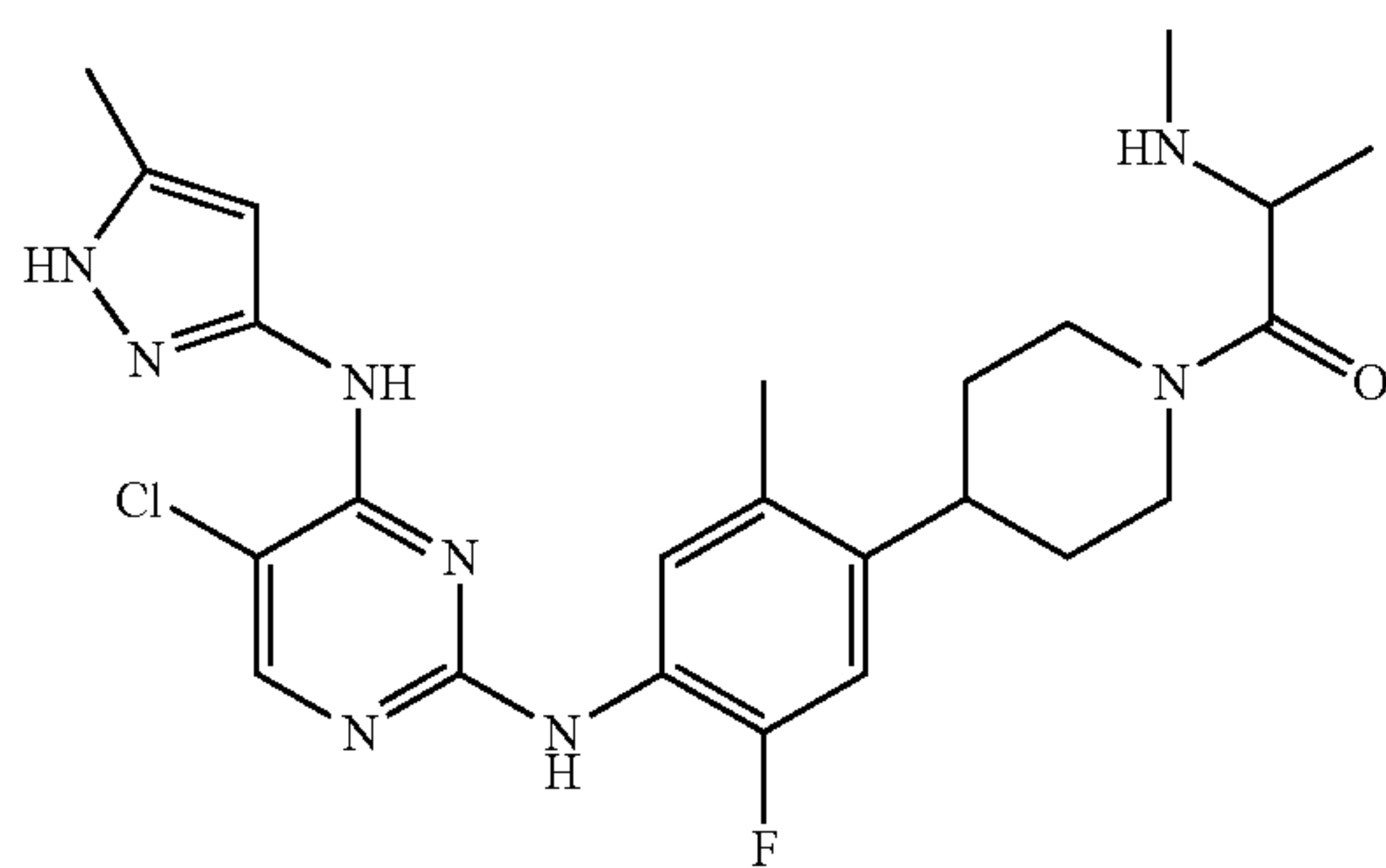
1-(4-(4-(5-chloro-4-(5-methyl-1H-pyrazol-3-ylamino)pyrimidin-2-ylamino)-5-fluoro-2-methylphenyl)piperidin-1-yl)-2-(methylamino)propan-1-one
