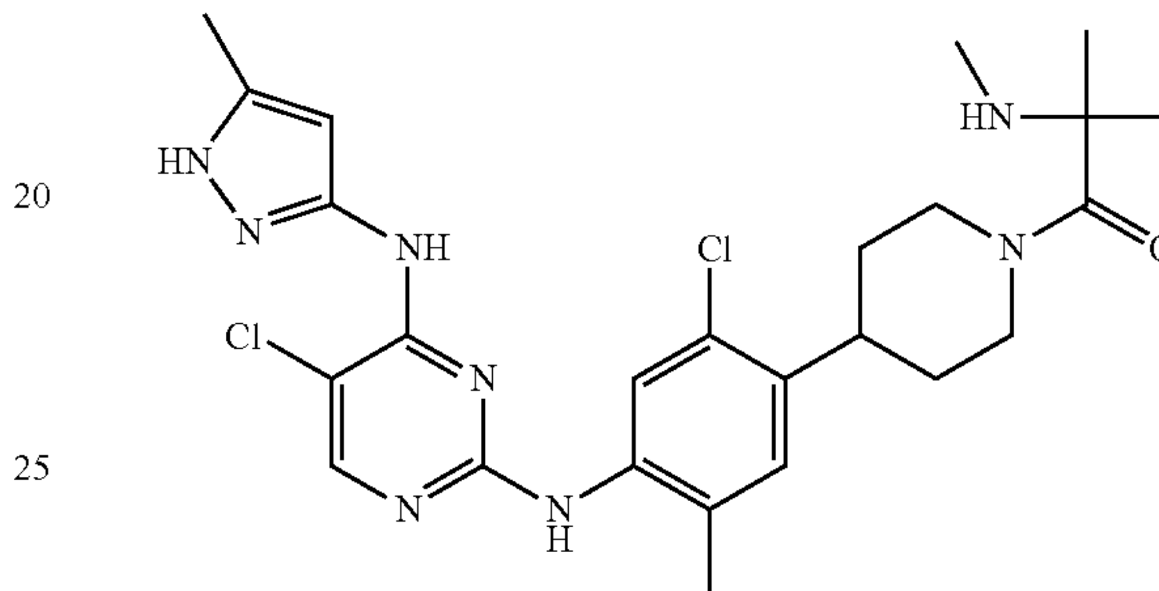
1-(4-(2-chloro-4-(5-chloro-4-(5-methyl-1H-pyrazol-3-ylamino)pyrimidin-2-ylamino)-5-methylphenyl)piperidin-1-yl)-2-methyl-2-(methylamino)propan-1-one
