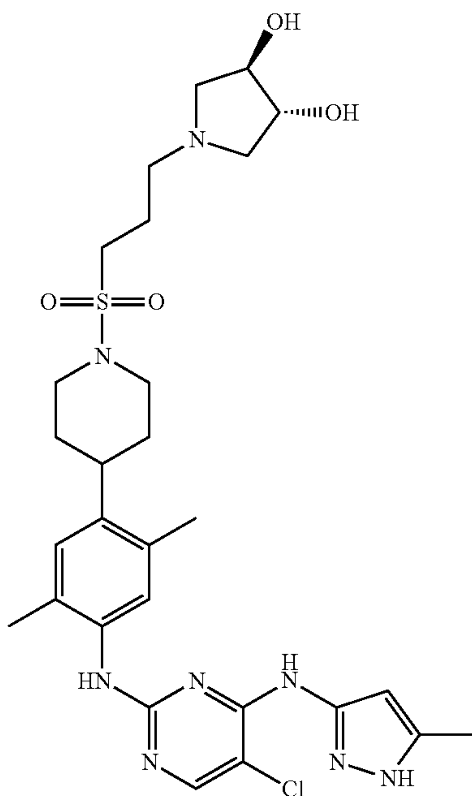
(3R,4R)-1-(3-(4-(4-(5-chloro-4-(5-methyl-1H-pyrazol-3-ylamino)pyrimidin-2-ylamino)-2,5-dimethylphenyl)piperidin-1-yl)sulfonyl)propyl)pyrrolidine-3,4-diol
