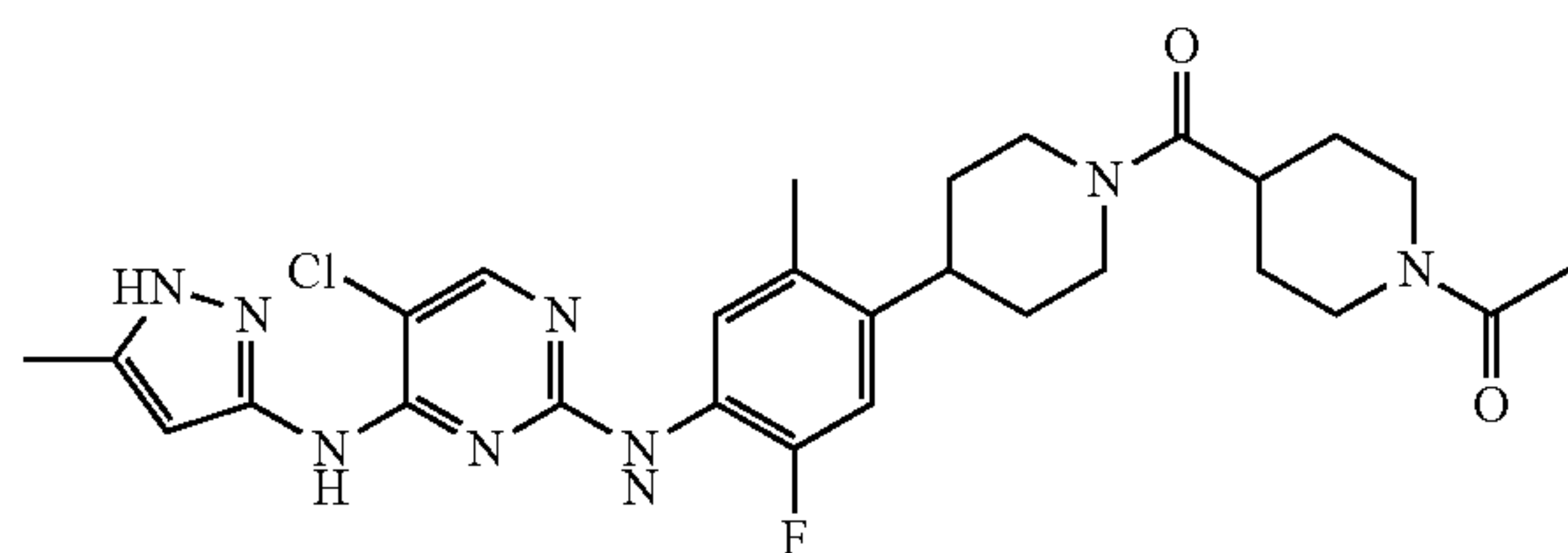
1-(4-(4-(5-chloro-4-(5-methyl-1H-pyrazol-3-ylamino)pyrimidin-2-ylamino)-2,5-dimethylphenyl)piperidin-1-yl)-2-methoxyethanone
