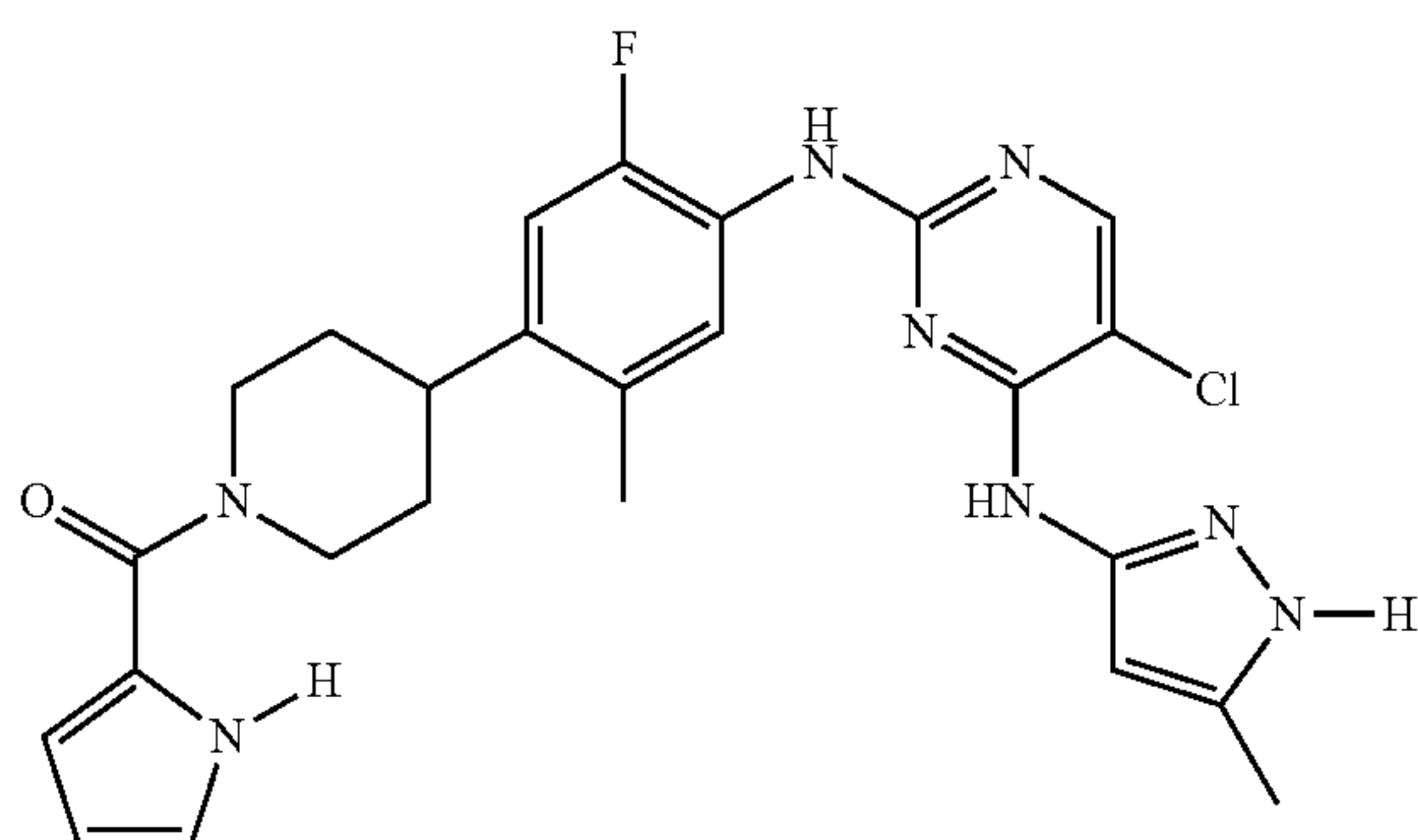
(4-(4-(5-chloro-4-(5-methyl-1H-pyrazol-3-ylamino)pyrimidin-2-ylamino)-5-fluoro-2-methylphenyl)piperidin-1-yl)(1H-pyrrol-2-yl)methanone
