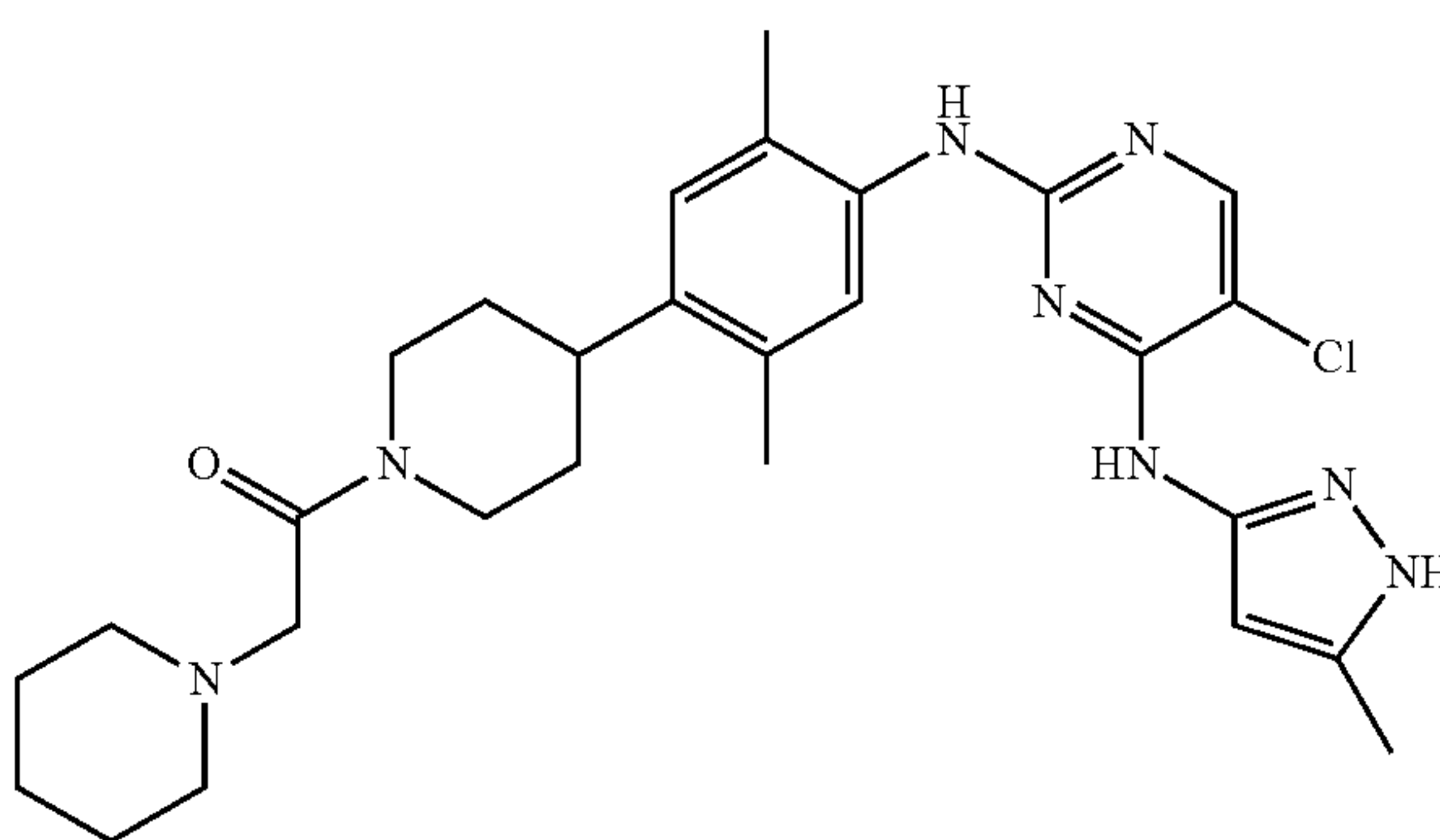
1-(4-(4-(5-chloro-4-(5-methyl-1H-pyrazol-3-ylamino)pyrimidin-2-ylamino)-2,5-dimethylphenyl)piperidin-1-yl)-2-(piperidin-1-yl)ethanone
