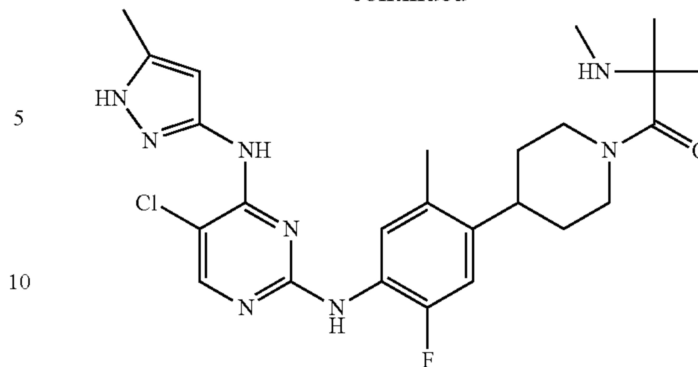
1-(4-(4-(5-chloro-4-(5-methyl-1H-pyrazol-3-ylamino)pyrimidin-2-ylamino)-5-fluoro-2-methylphenyl)piperidin-1-yl)-2-methyl-2-(methylamino)propan-1-one
