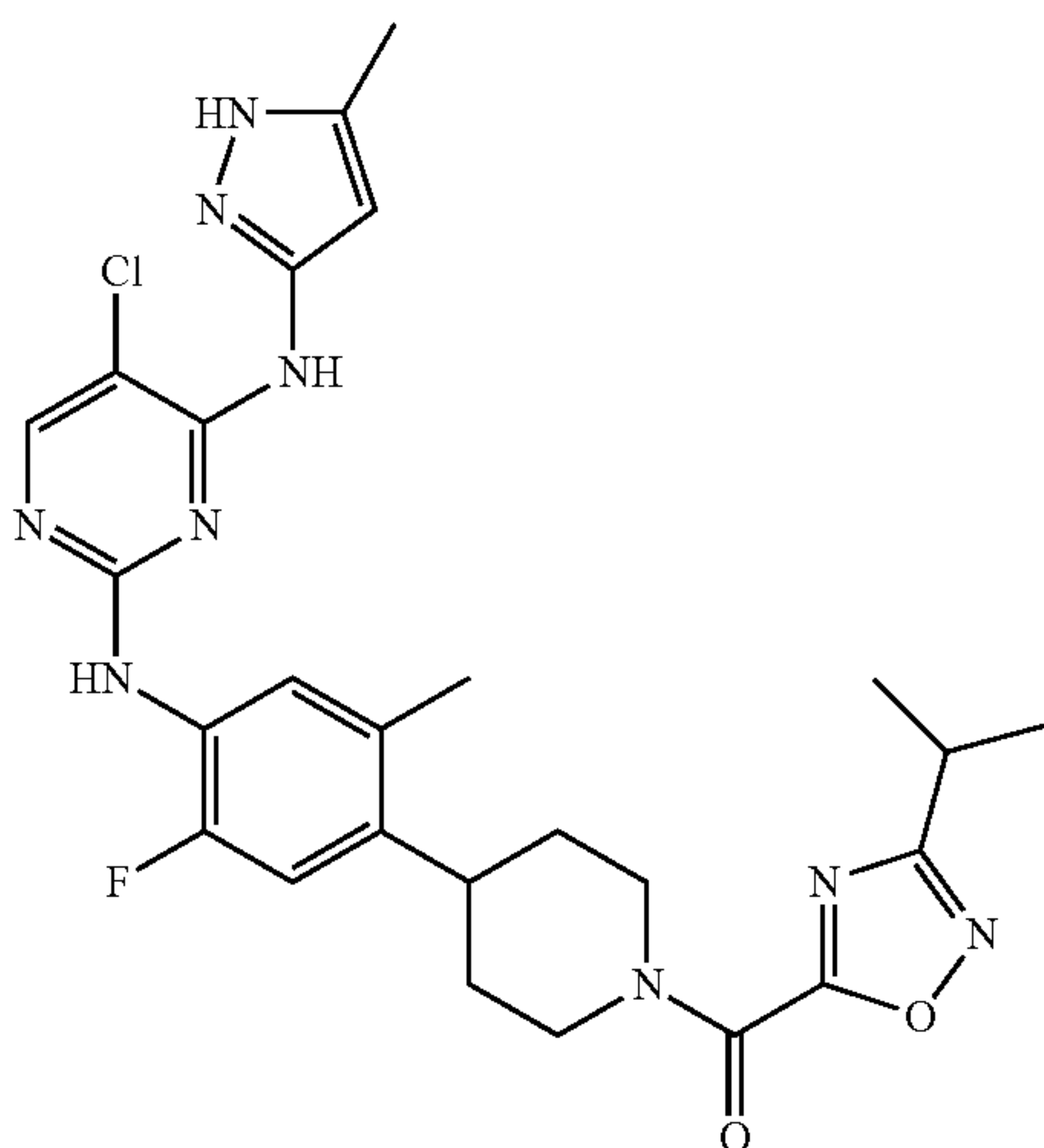
(4-(4-(5-chloro-4-(5-methyl-1H-pyrazol-3-ylamino)pyrimidin-2-ylamino)-5-fluoro-2-methylphenyl)piperidin-1-yl)-(3-isopropyl-1,2,4-oxadiazol-5-yl)methanone
