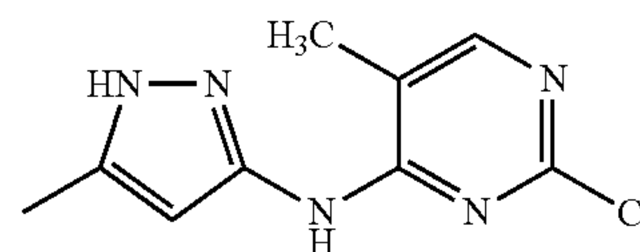
2-chloro-5-methyl-N-(5-methyl-1H-pyrazol-3-yl)pyrimidin-4-amine
