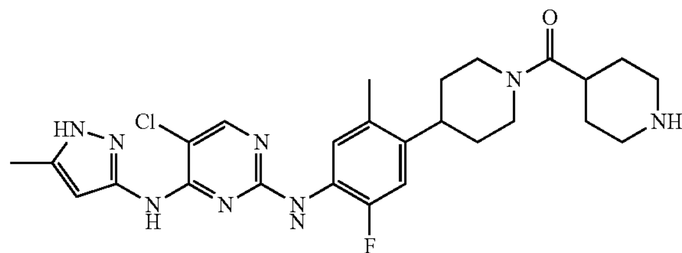
(4-(4-(5-chloro-4-(5-methyl-1H-pyrazol-3-ylamino)pyrimidin-2-ylamino)-5-fluoro-2-methylphenyl)piperidin-1-yl)(piperidin-4-yl)methanone
