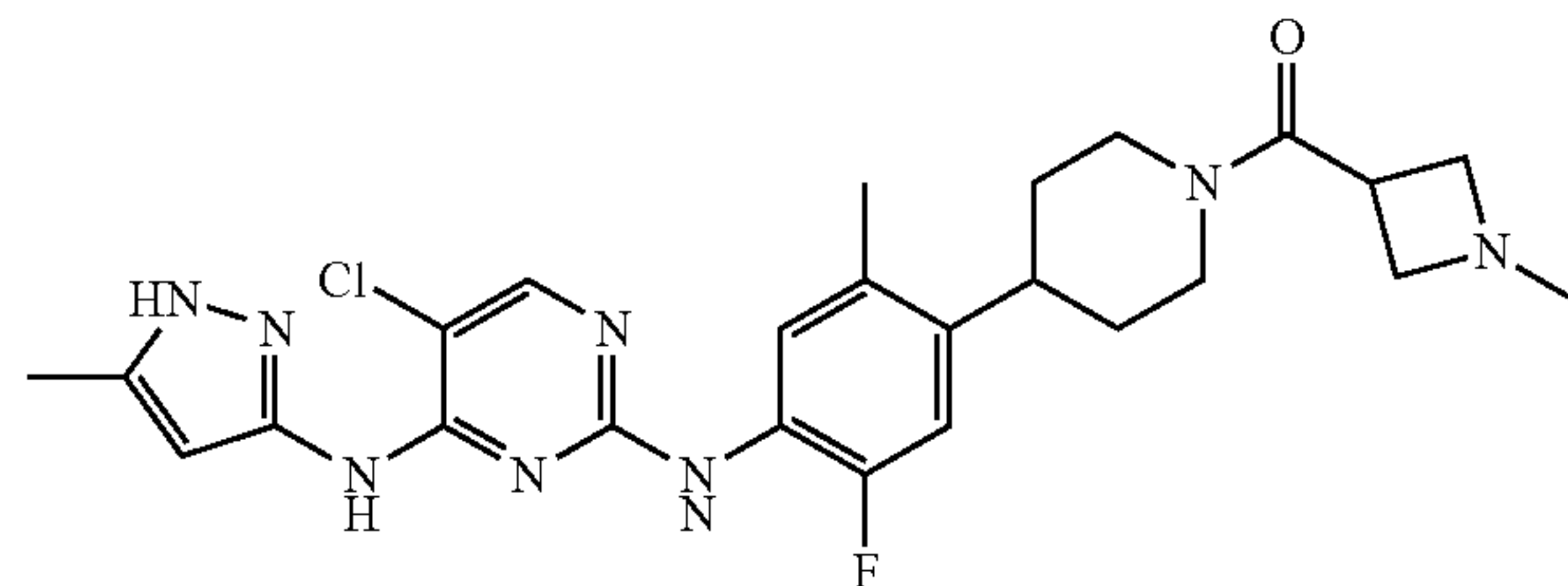
(4-(4-(5-chloro-4-(5-methyl-1H-pyrazol-3-ylamino)pyrimidin-2-ylamino)-5-fluoro-2-methylphenyl)piperidin-1-yl)(1-methylazetidin-3-yl)methanone
