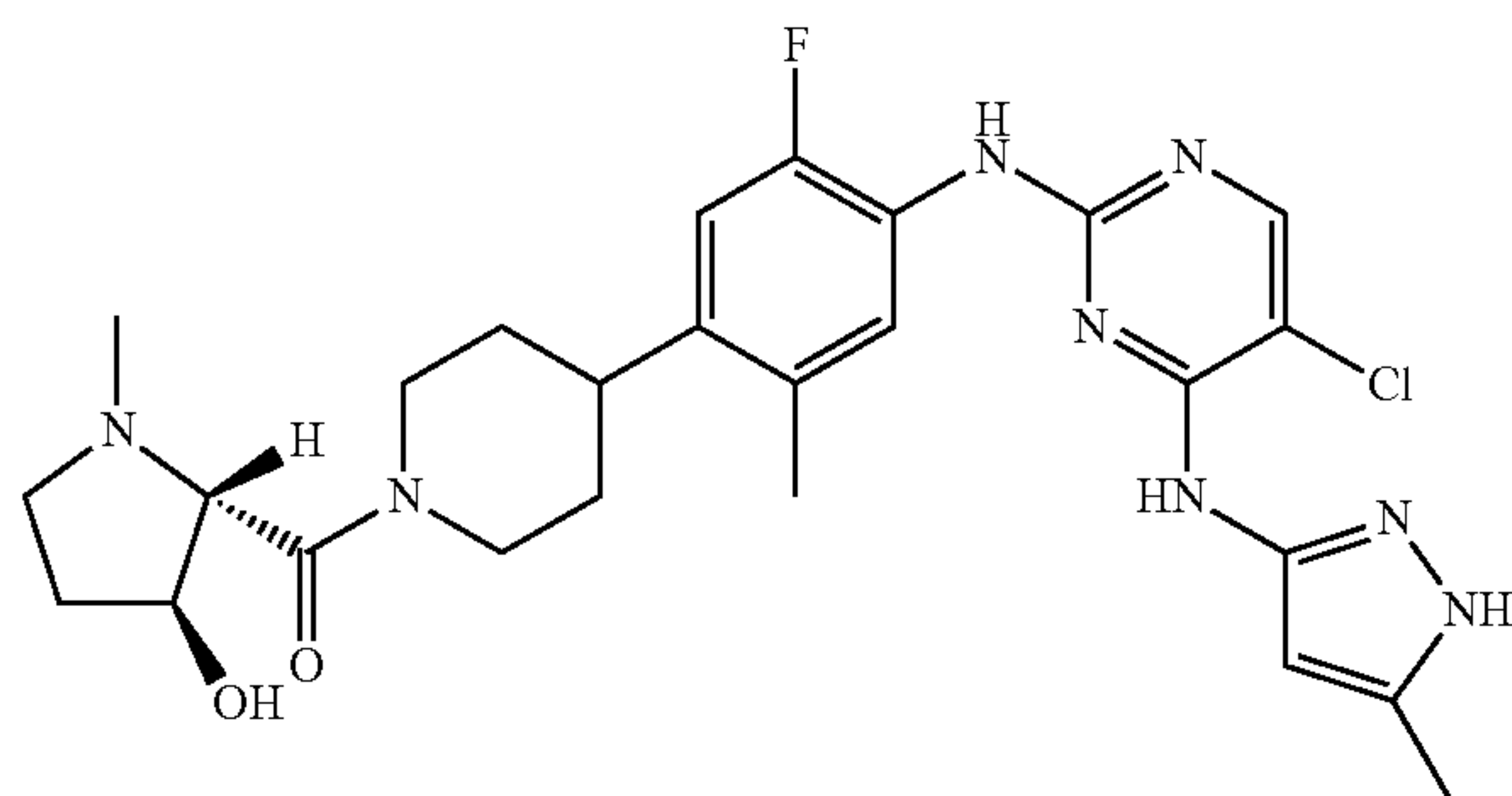
(4-(4-(5-chloro-4-(5-methyl-1H-pyrazol-3-ylamino)pyrimidin-2-ylamino)-5-fluoro-2-methylphenyl)piperidin-1-yl)((2S,3R)-3-hydroxy-1-methylpyrrolidin-2-yl)methanone
