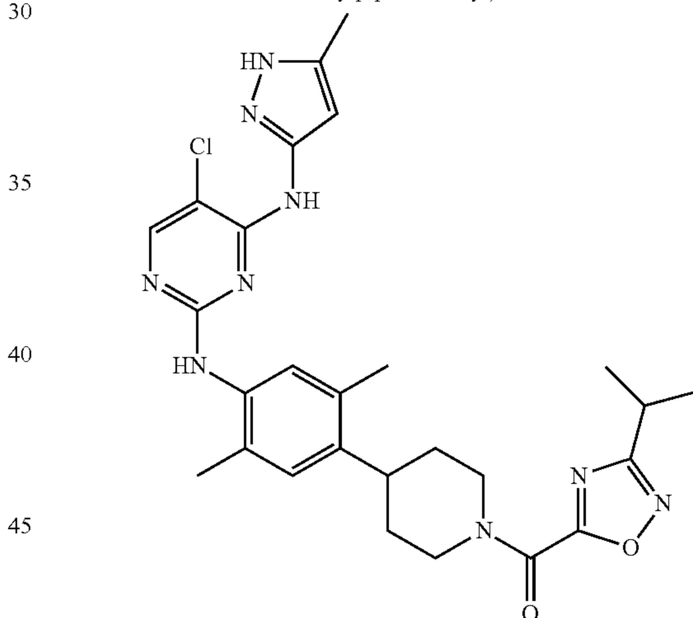
(4-(4-(5-chloro-4-(5-methyl-1H-pyrazol-3-ylamino)pyrimidin-2-ylamino)-2,5-dimethylphenyl)piperidin-1-yl)-(3-isopropyl-1,2,4-oxadiazol-5-yl)methanone
