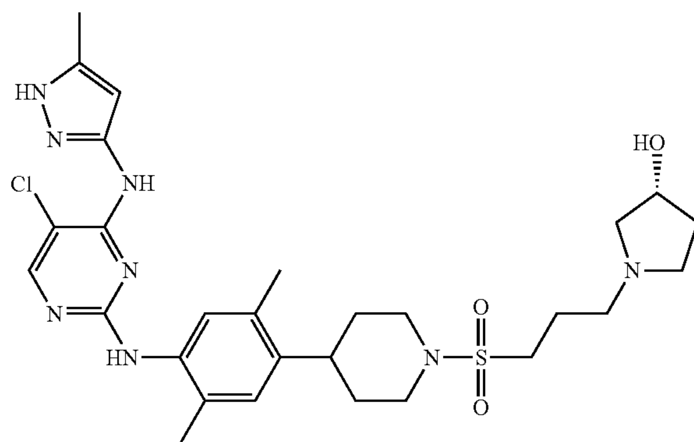
(R)-1-(3-(4-(4-(5-chloro-4-(5-methyl-1H-pyrazol-3-ylamino)pyrimidin-2-ylamino)-2,5-dimethylphenyl)piperidin-1-ylsulfonyl)propyl)pyrrolidin-3-ol
