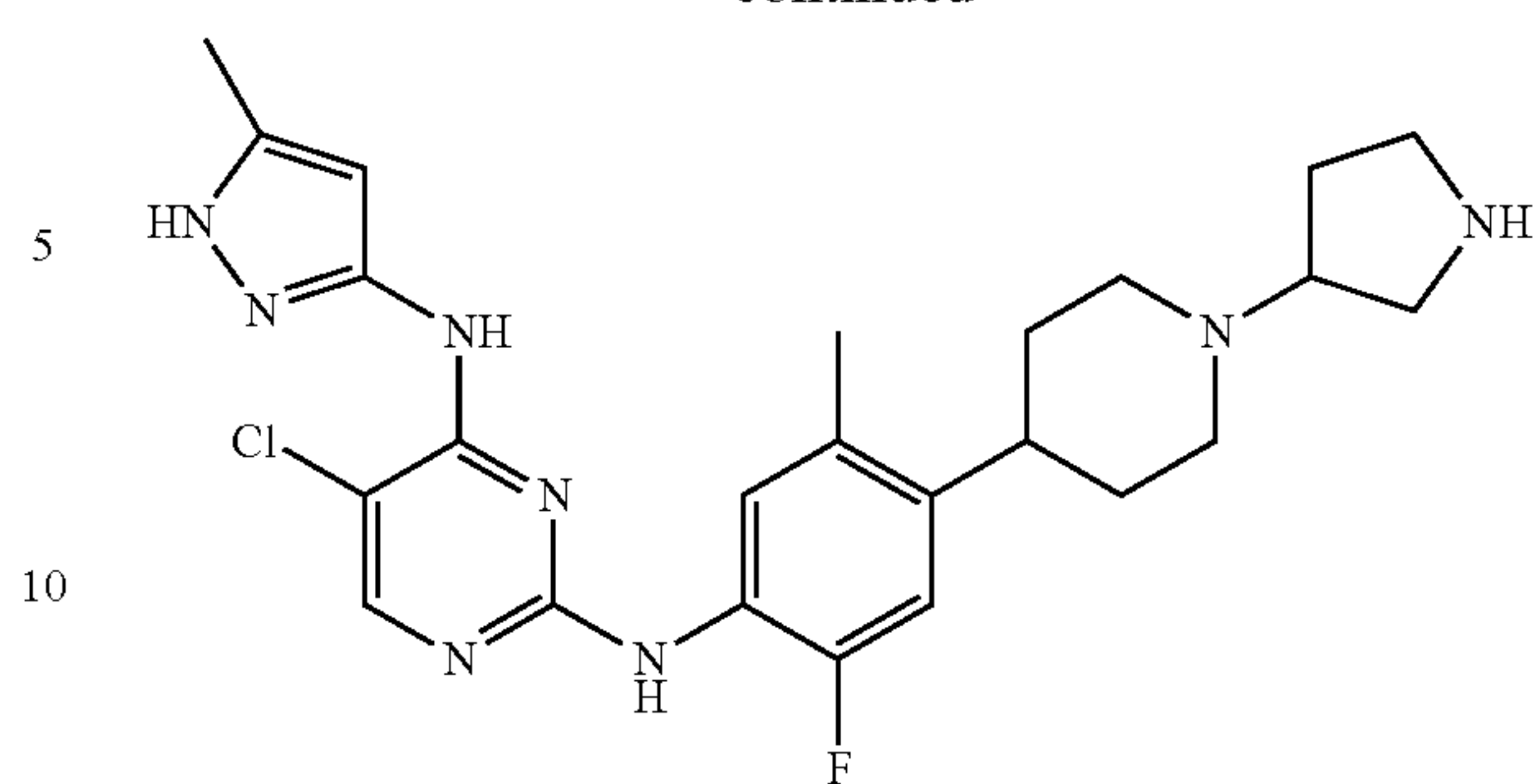
5-chloro-N2-(2-fluoro-5-methyl-4-(1-(pyrrolidin-3-yl)piperidin-4-yl)phenyl)-N4-(5-methyl-1H-pyrazol-3-yl)pyrimidine-2,4-diamine
