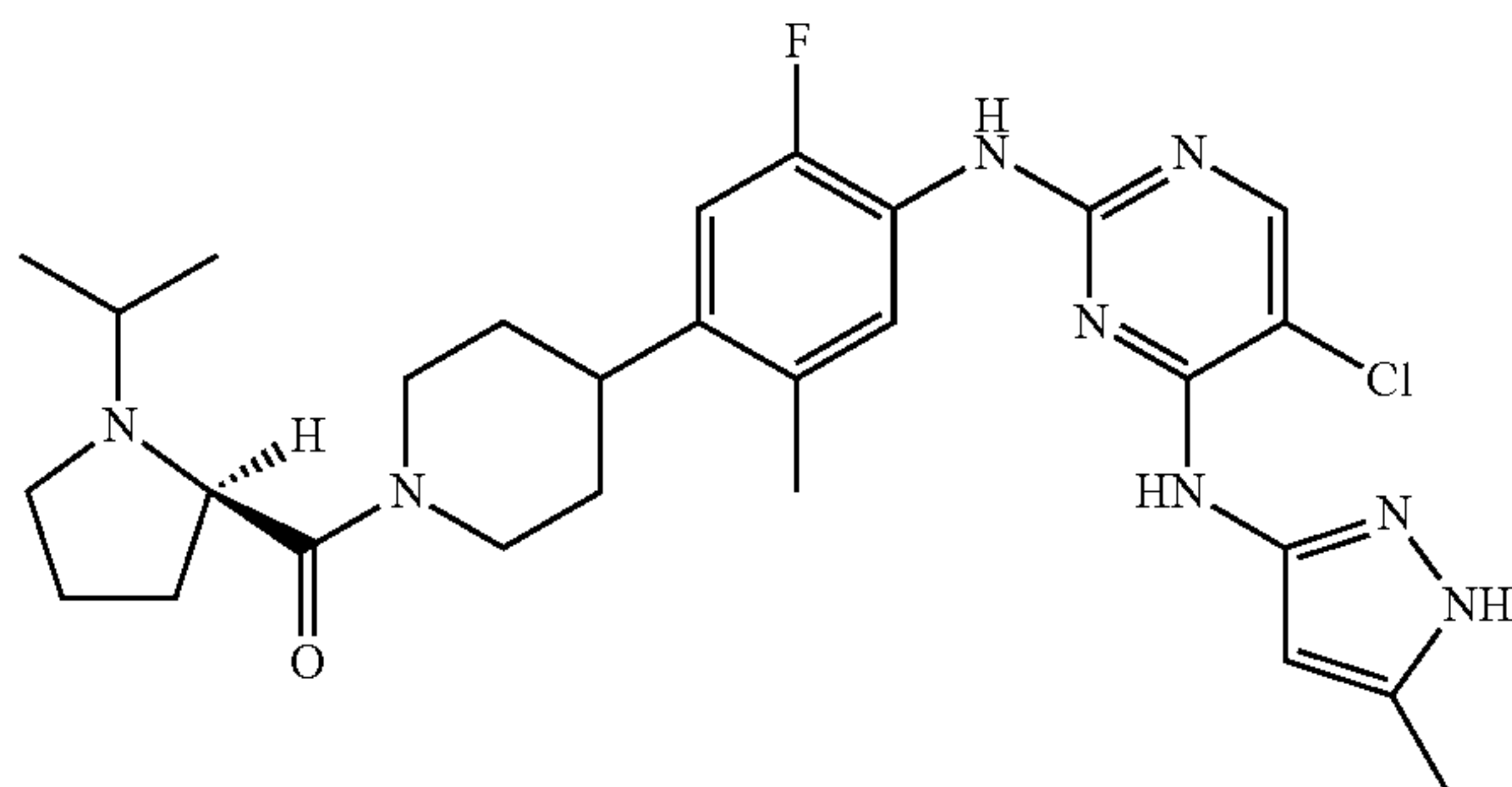
(R)-(4-(4-(5-chloro-4-(5-methyl-1H-pyrazol-3-ylamino)pyrimidin-2-ylamino)-5-fluoro-2-methylphenyl)piperidin-1-yl)(1-isopropylpyrrolidin-2-yl)methanone
