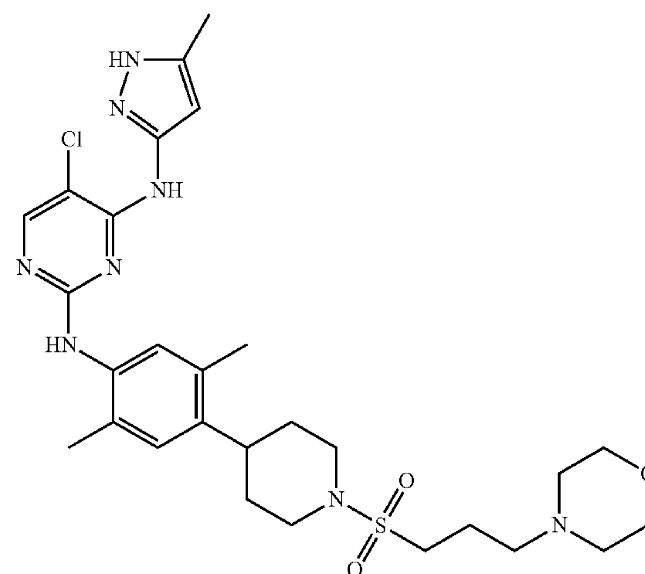
5-chloro-N2-(2,5-dimethyl-4-(1-(3-morpholinopropylsulfonyl)piperidin-4-yl)phenyl)-N4-(5-methyl-1H-pyrazol-3-yl)pyrimidine-2,4-diamine
