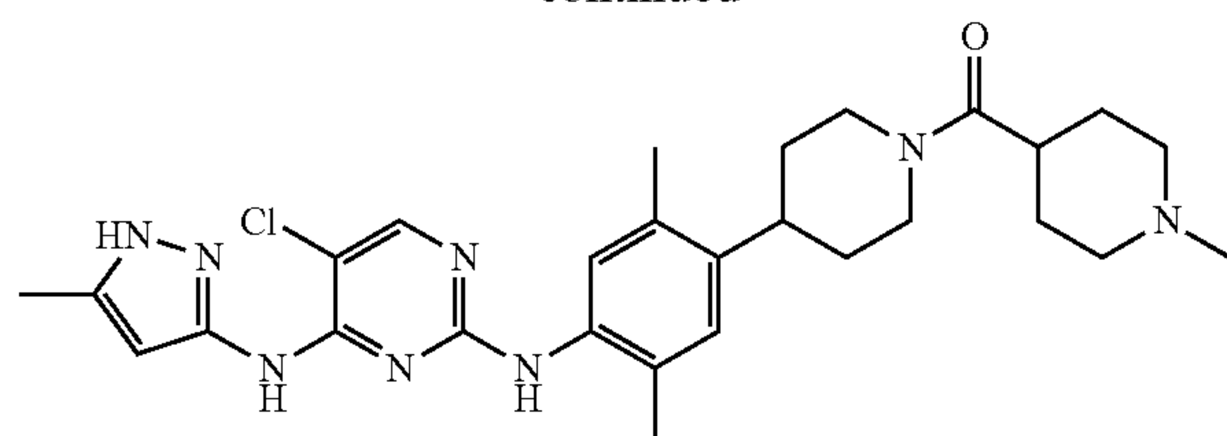
(4-(4-(5-chloro-4-(5-methyl-1H-pyrazol-3-ylamino)pyrimidin-2-ylamino)-2,5-dimethylphenyl)piperidin-1-yl)(1-methylpiperidin-4-yl)methanone
