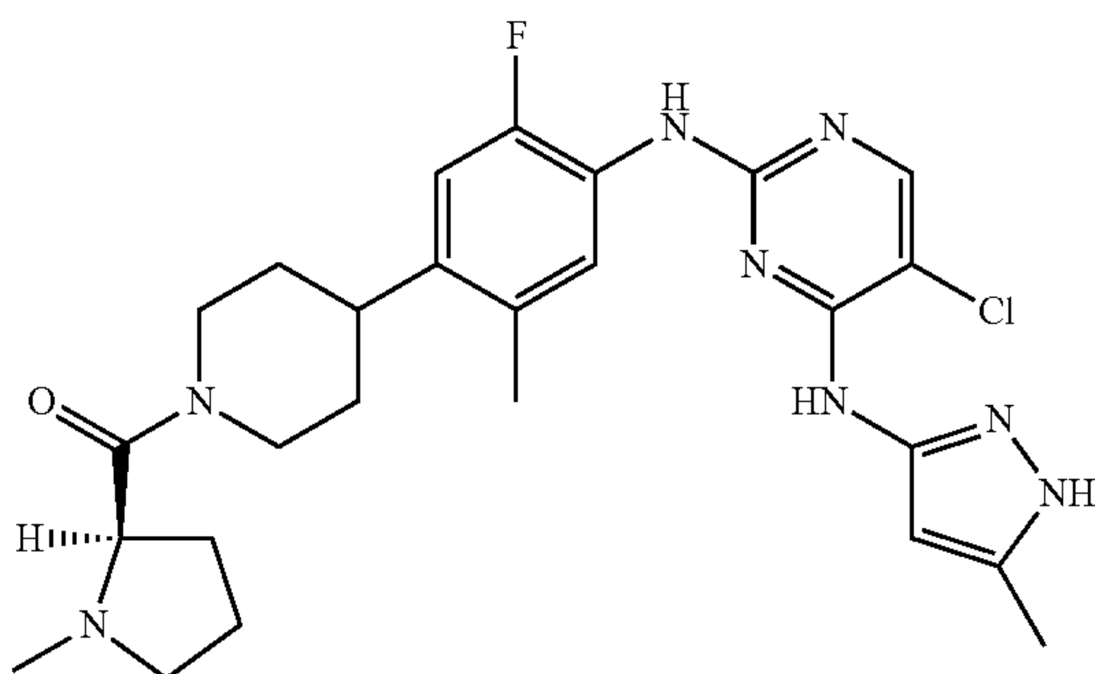
(R)-(4-(4-(5-chloro-4-(5-methyl-1H-pyrazol-3-ylamino)pyrimidin-2-ylamino)-5-fluoro-2-methylphenyl)piperidin-1-yl)1-methylpyrrolidin-2-yl)methanone
