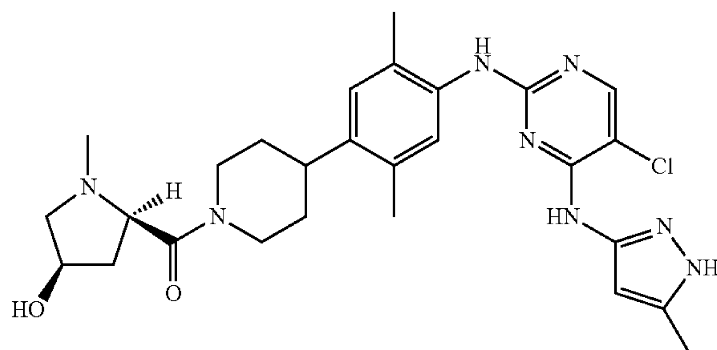
(4-(4-(5-chloro-4-(5-methyl-1H-pyrazol-3-ylamino)pyrimidin-2-ylamino)-2,5-dimethylphenyl)piperidin-1-yl)((2R,4R)-4-hydroxy-1-methylpyrrolidin-2-yl)methanone
