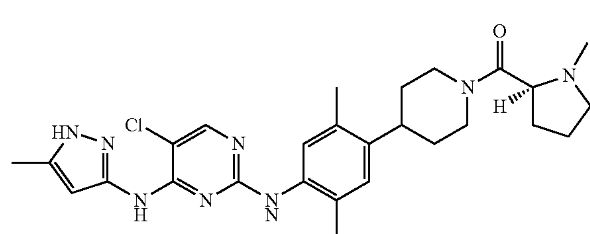
(S)-(4-(4-(5-chloro-4-(5-methyl-1H-pyrazol-3-ylamino)pyrimidin-2-ylamino)-2,5-dimethylphenyl)piperidin-1-yl)(1-methylpyrrolidin-2-yl)methanone
