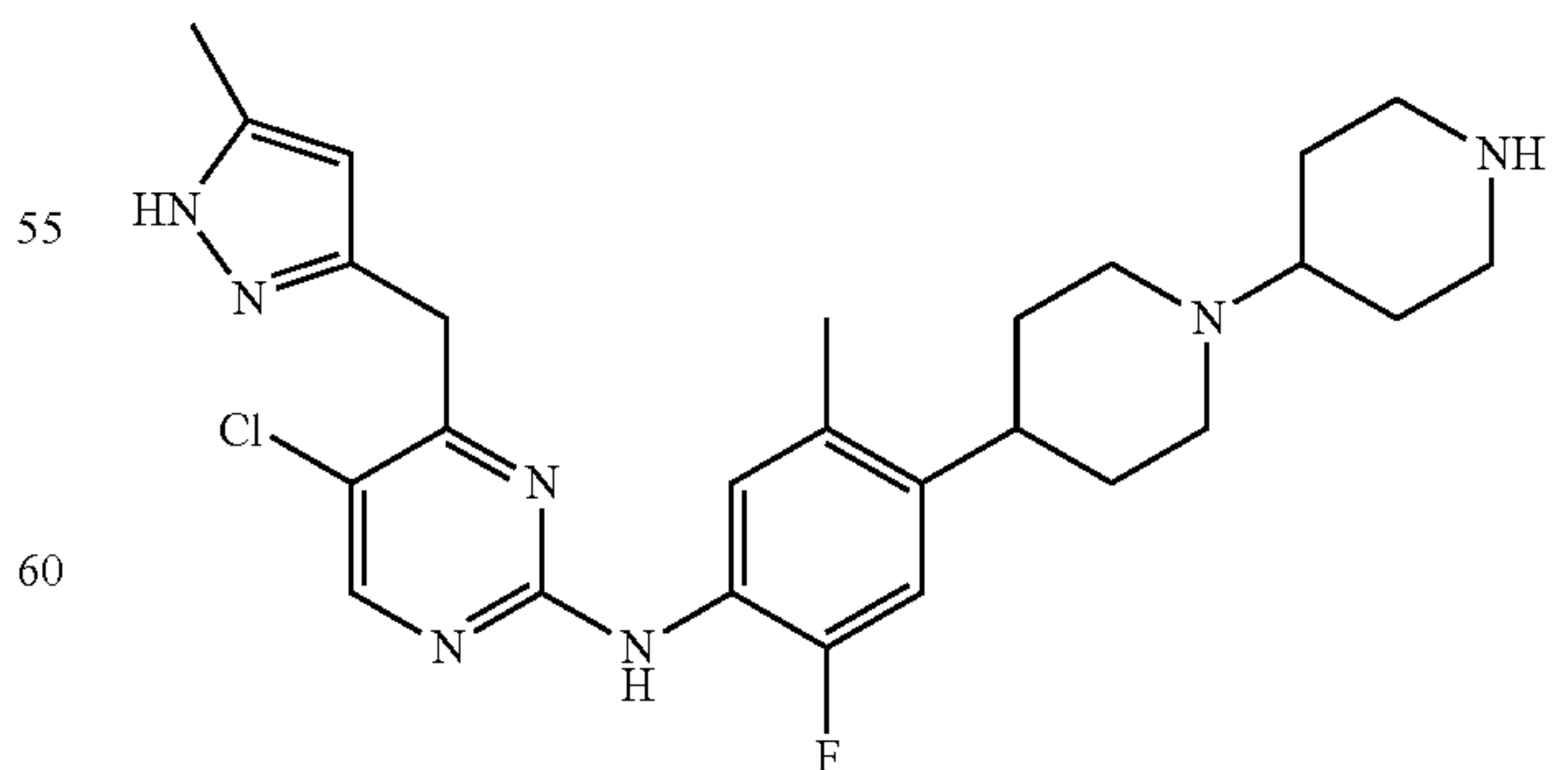
N2-(4-(1,4'-bipiperidin-4-yl)-2-fluoro-5-methylphenyl)-5-chloro-N4-(5-methyl-1H-pyrazol-3-yl)pyrimidine-2,4-diamine
