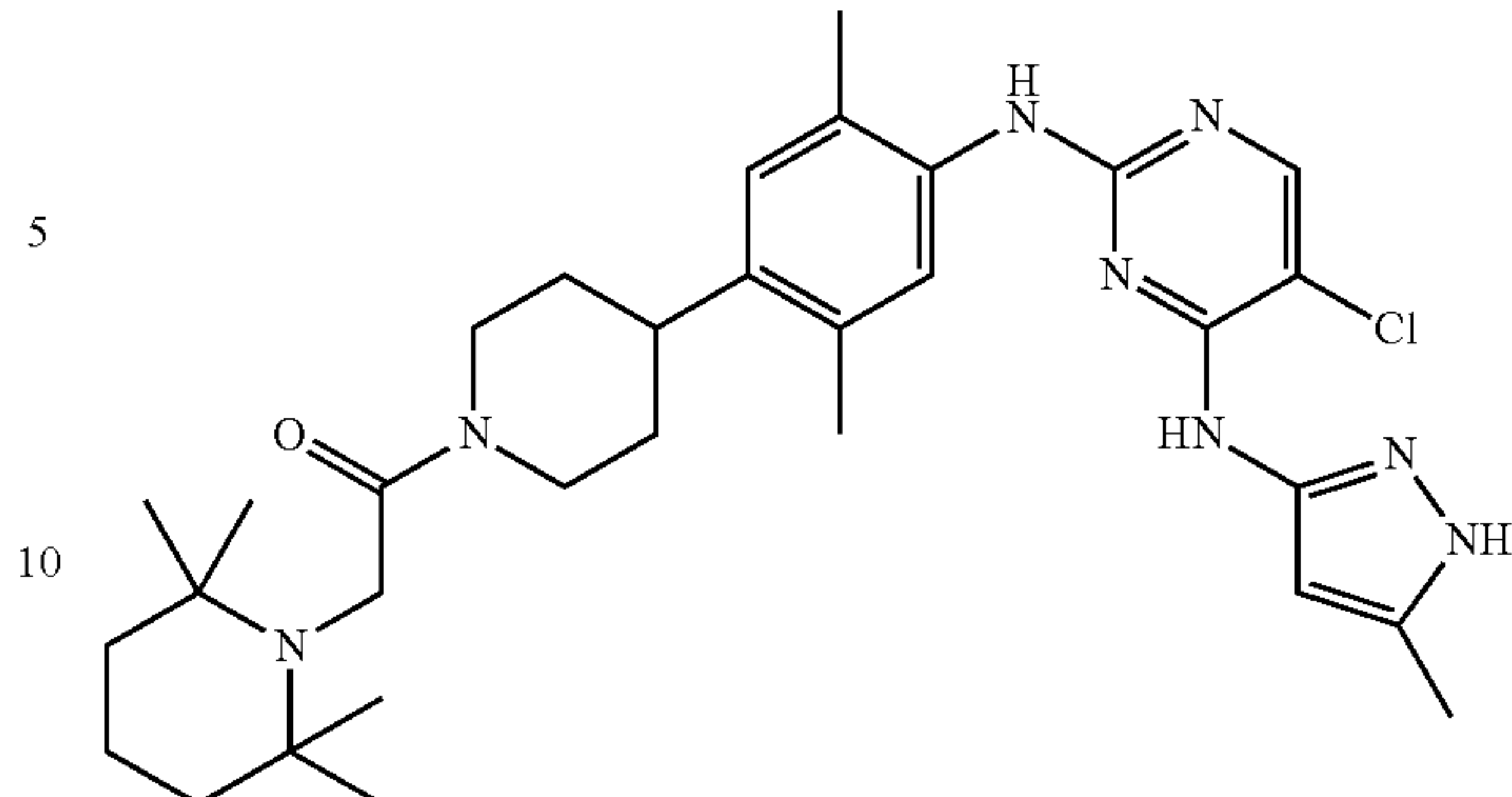
1-(4-(4-(5-chloro-4-(5-methyl-1H-pyrazol-3-ylamino)pyrimidin-2-ylamino)-2,5-dimethylphenyl)piperidin-1-yl)-2-(2,2,6,6-tetramethylpiperidin-1-yl)ethanone
