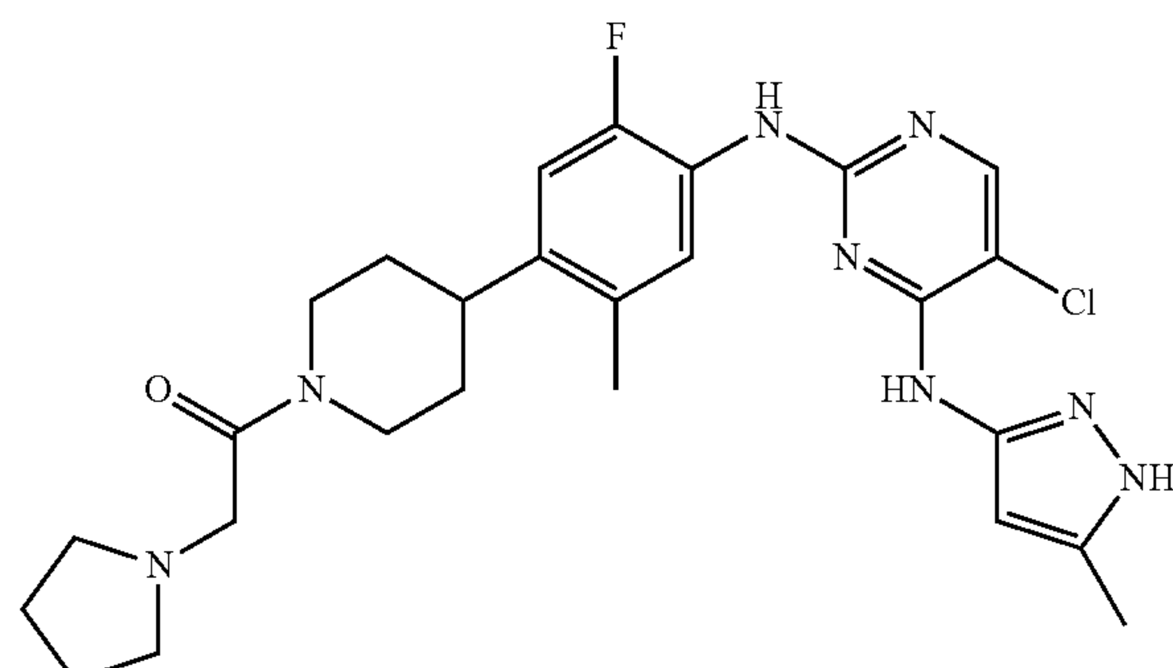
1-(4-(4-(5-chloro-4-(5-methyl-1H-pyrazol-3-ylamino)pyrimidin-2-ylamino)-5-fluoro-2-methylphenyl)piperidin-1-yl)-2-(pyrrolidin-1-yl)ethanone
