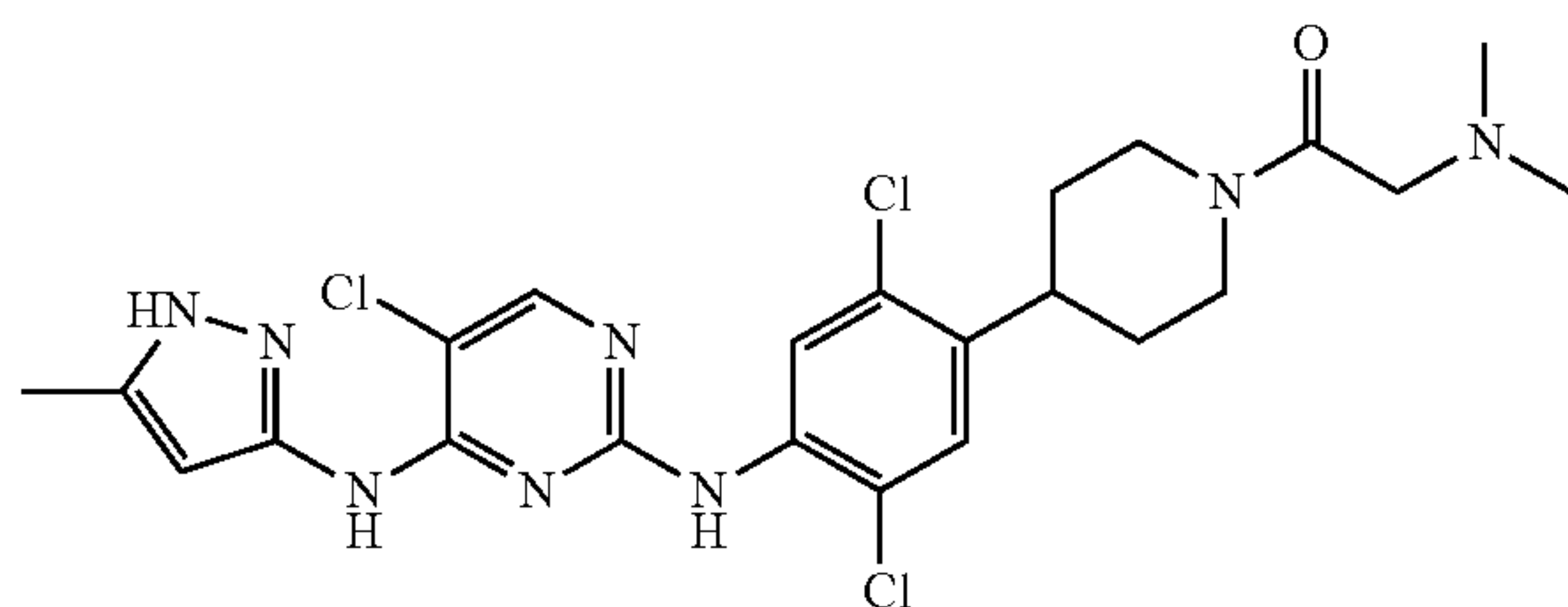
1-(4-(2,5-dichloro-4-(5-chloro-4-(5-methyl-1H-pyrazol-3-ylamino)pyrimidin-2-ylamino)phenyl)piperidin-1-yl)-2-(dimethylamino)ethanone
