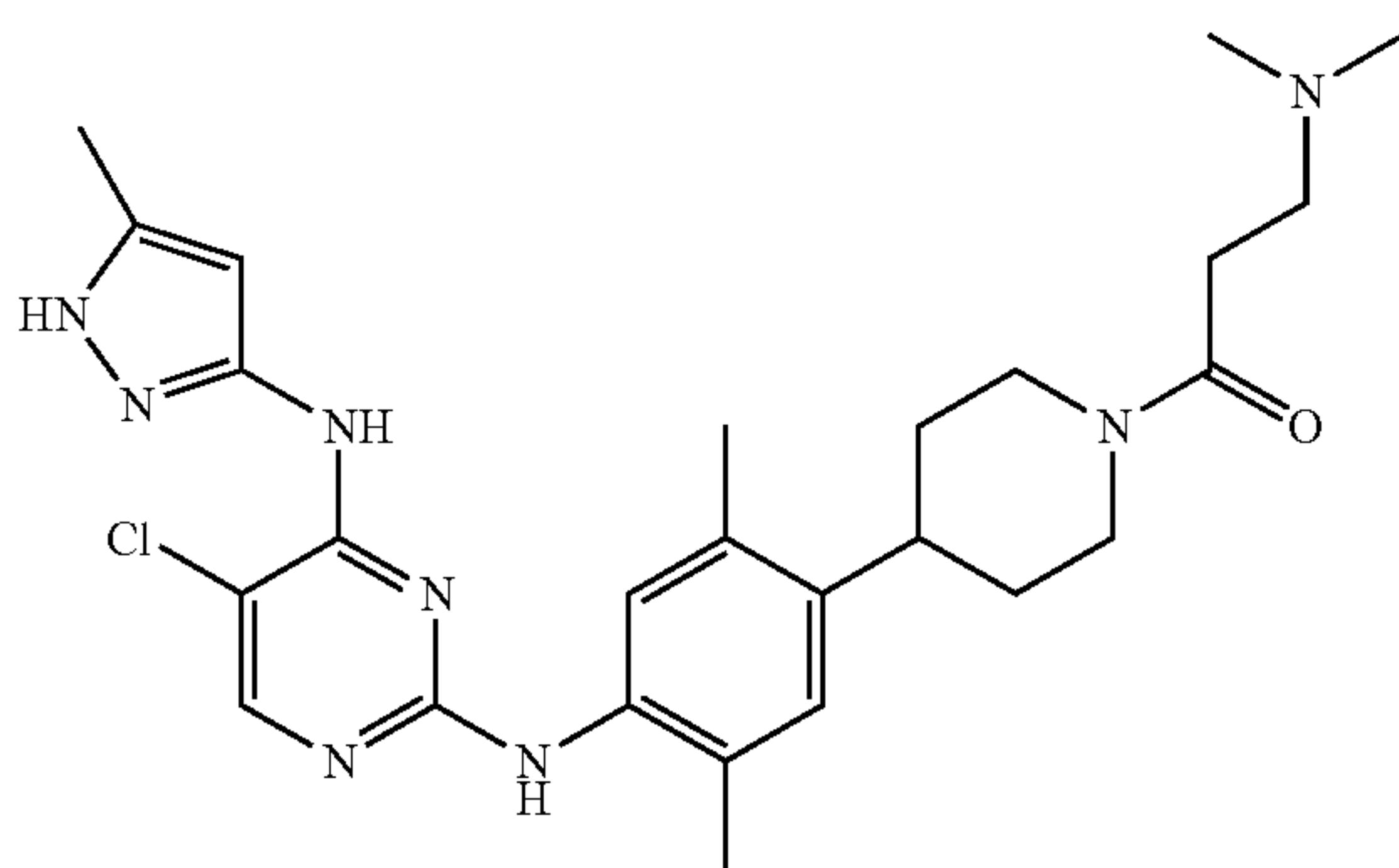
1-(4-(4-(5-chloro-4-(5-methyl-1H-pyrazol-3-ylamino)pyrimidin-2-ylamino)-2,5-dimethylphenyl)piperidin-1-yl)-3-(dimethylamino)propan-1-one
