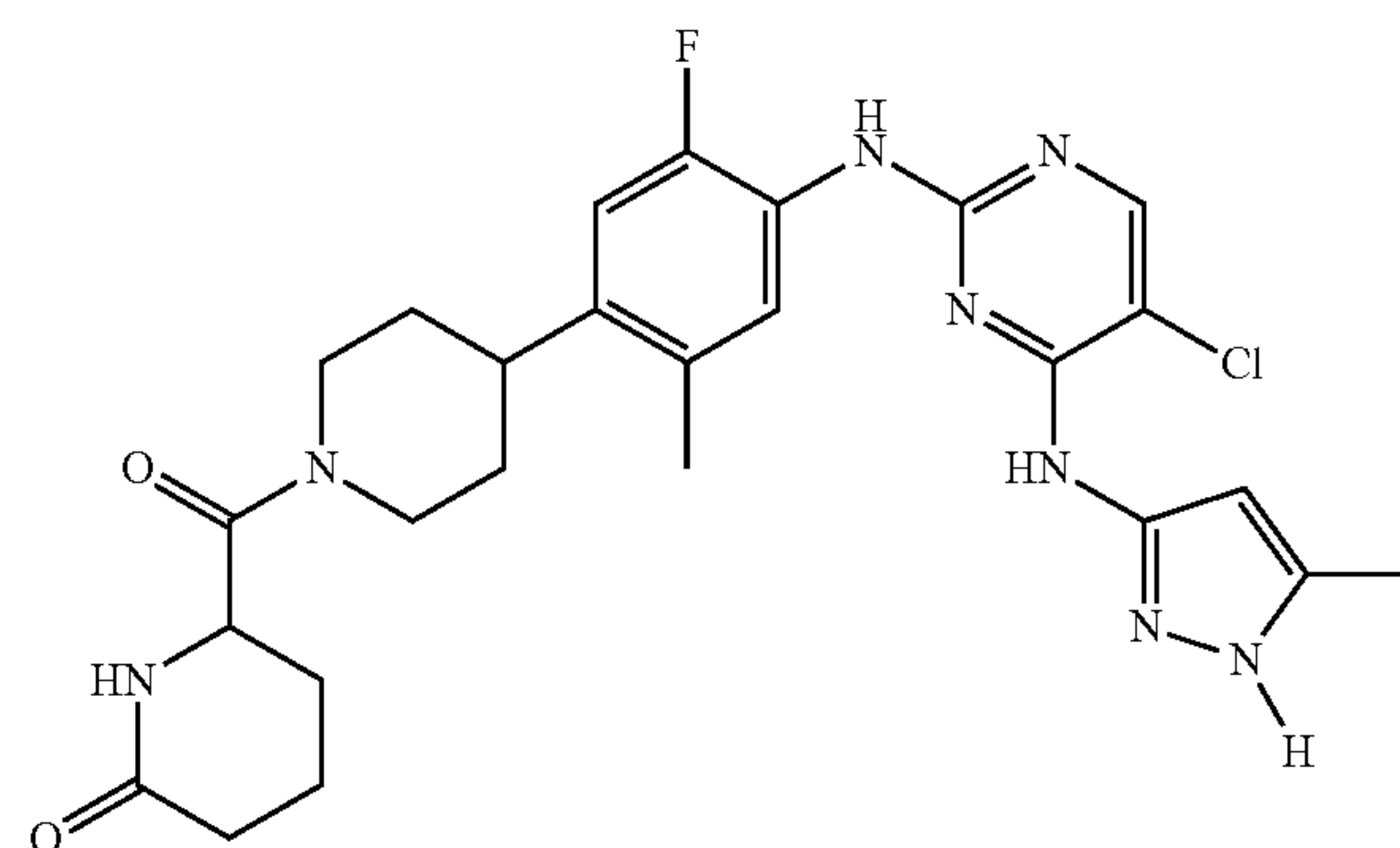
6-(4-(4-(5-chloro-4-(5-methyl-1H-pyrazol-3-ylamino)pyrimidin-2-ylamino)-5-fluoro-2-methylphenyl)piperidin-1-carbonyl)piperidin-2-one
