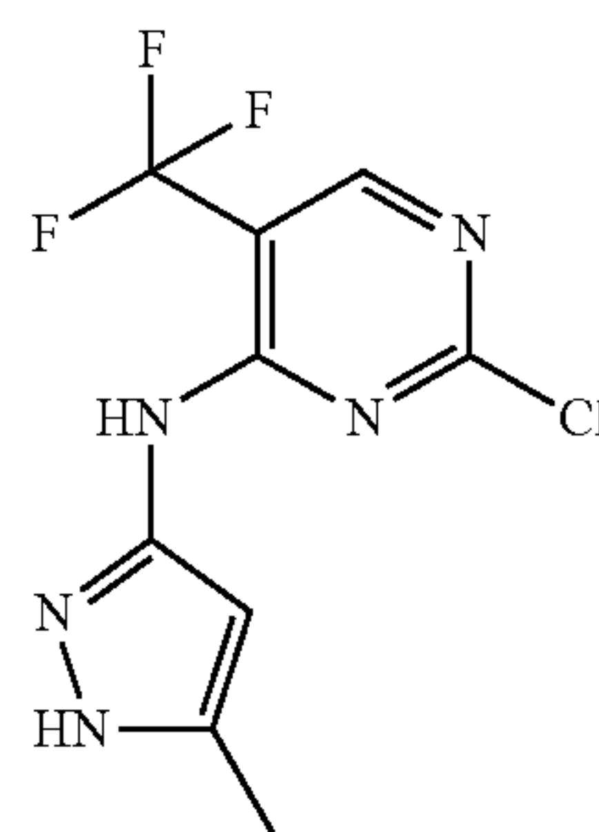
2-chloro-N-(5-methyl-1H-pyrazol-3-yl)-5-(trifluoromethyl)pyrimidin-4-amine
