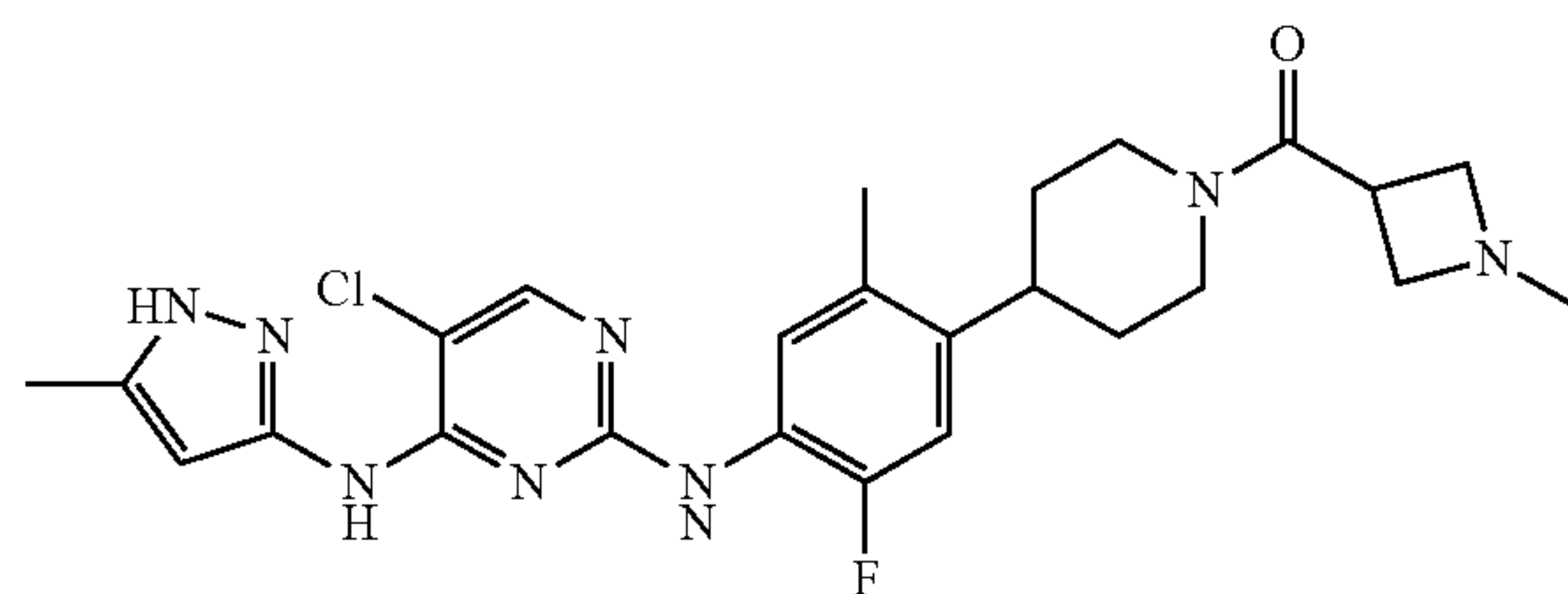
3-(4-(4-(5-chloro-4-(5-methyl-1H-pyrazol-3-ylamino)pyrimidin-2-ylamino)-5-fluoro-2-methylphenyl)piperidin-1-carbonyl)azetidin-2-one
