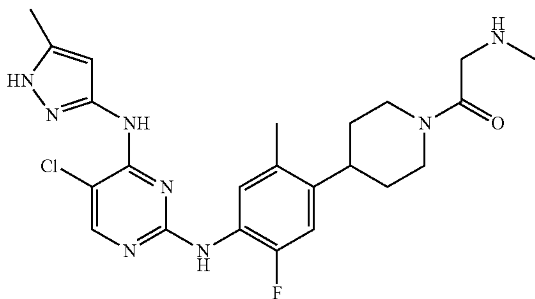
1-(4-(4-(5-chloro-4-(5-methyl-1H-pyrazol-3-ylamino)pyrimidin-2-ylamino)-5-fluoro-2-methylphenyl)piperidin-1-yl)-2-(methylamino)ethanone
