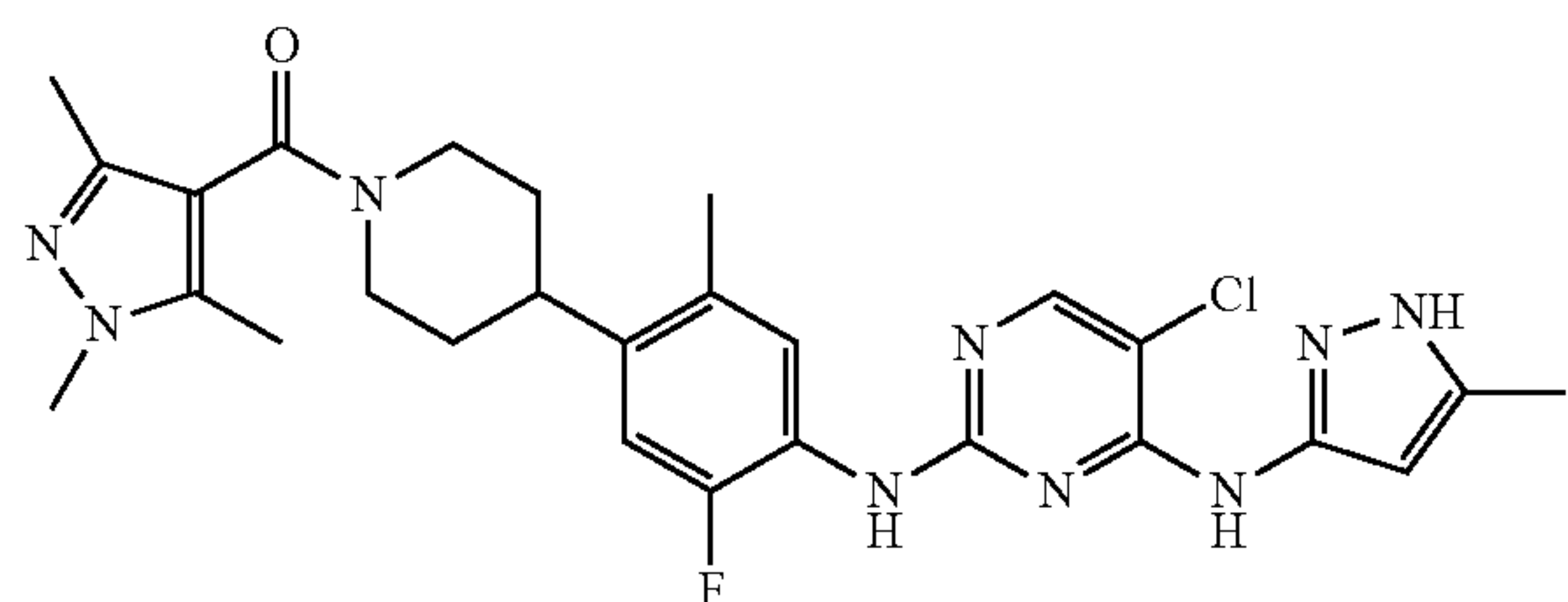
(4-(4-(5-chloro-4-(5-methyl-1H-pyrazol-3-ylamino)pyrimidin-2-ylamino)-5-fluoro-2-methylphenyl)piperidin-1-yl)(1,3,5-trimethyl-1H-pyrazol-4-yl)methanone
