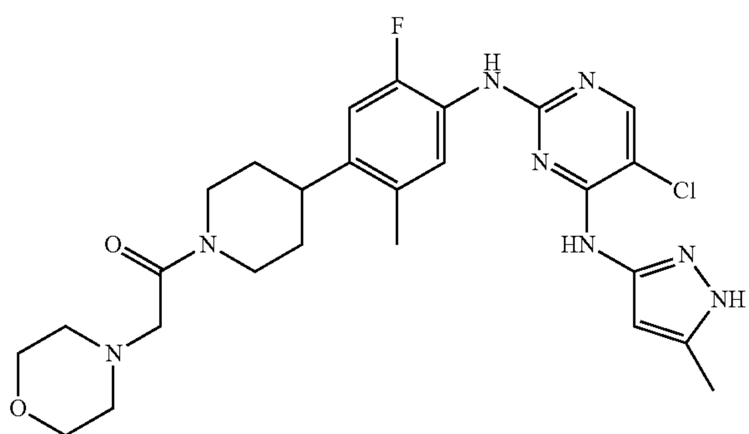
1-(4-(4-(5-chloro-4-(5-methyl-1H-pyrazol-3-ylamino)pyrimidin-2-ylamino)-5-fluoro-2-methylphenyl)piperidin-1-yl)-2-morpholinoethanone
