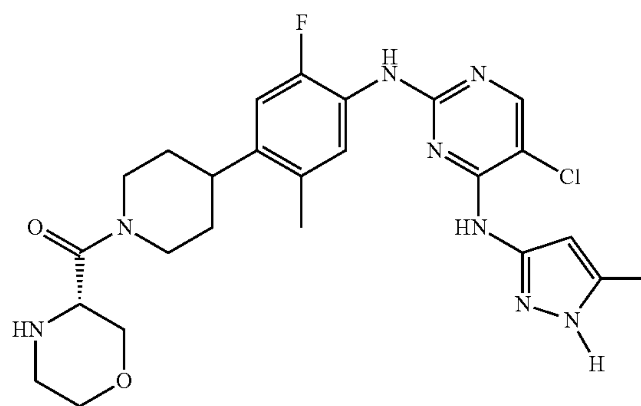
(S)-(4-(4-(5-chloro-4-(5-methyl-1H-pyrazol-3-ylamino)pyrimidin-2-ylamino)-5-fluoro-2-methylphenyl)piperidin-1-yl)(morpholin-3-yl)methanone
