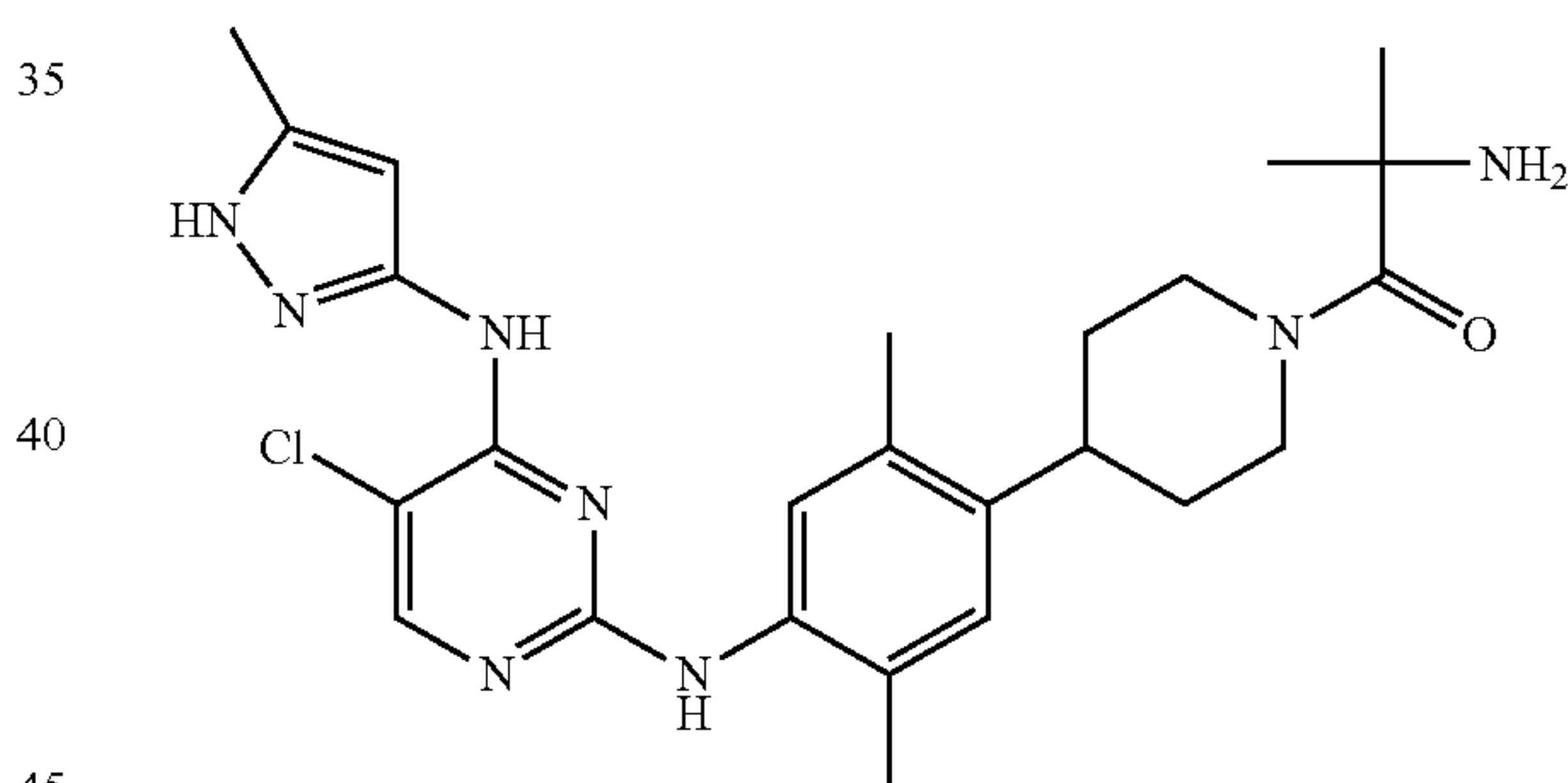
2-amino-1-(4-(4-(5-chloro-4-(5-methyl-1H-pyrazol-3-ylamino)pyrimidin-2-ylamino)-2,5-dimethylphenyl)piperidin-1-yl)-2-methylpropan-1-one
