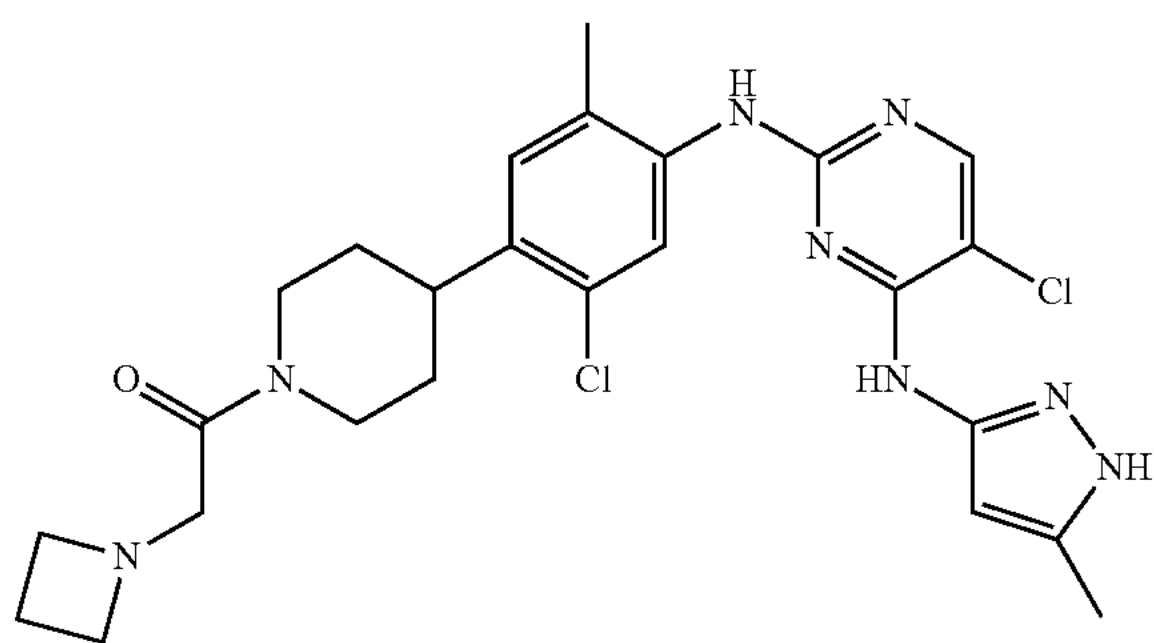
2-(azetidin-1-yl)-1-(4-(2-chloro-4-(5-chloro-4-(5-methyl-1H-pyrazol-3-ylamino)pyrimidin-2-ylamino)-5-methylphenyl)piperidin-1-yl)ethanone
