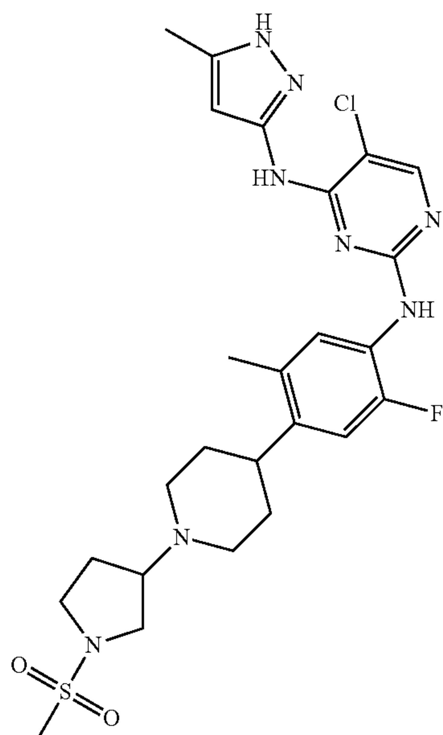
5-chloro-N2-(2-fluoro-5-methyl-4-(1-(1-(methylsulfonyl)pyrrolidin-3-yl)piperidin-4-yl)phenyl)-N4-(5-methyl-1H-pyrazol-3-yl)pyrimidine-2,4-diamine
