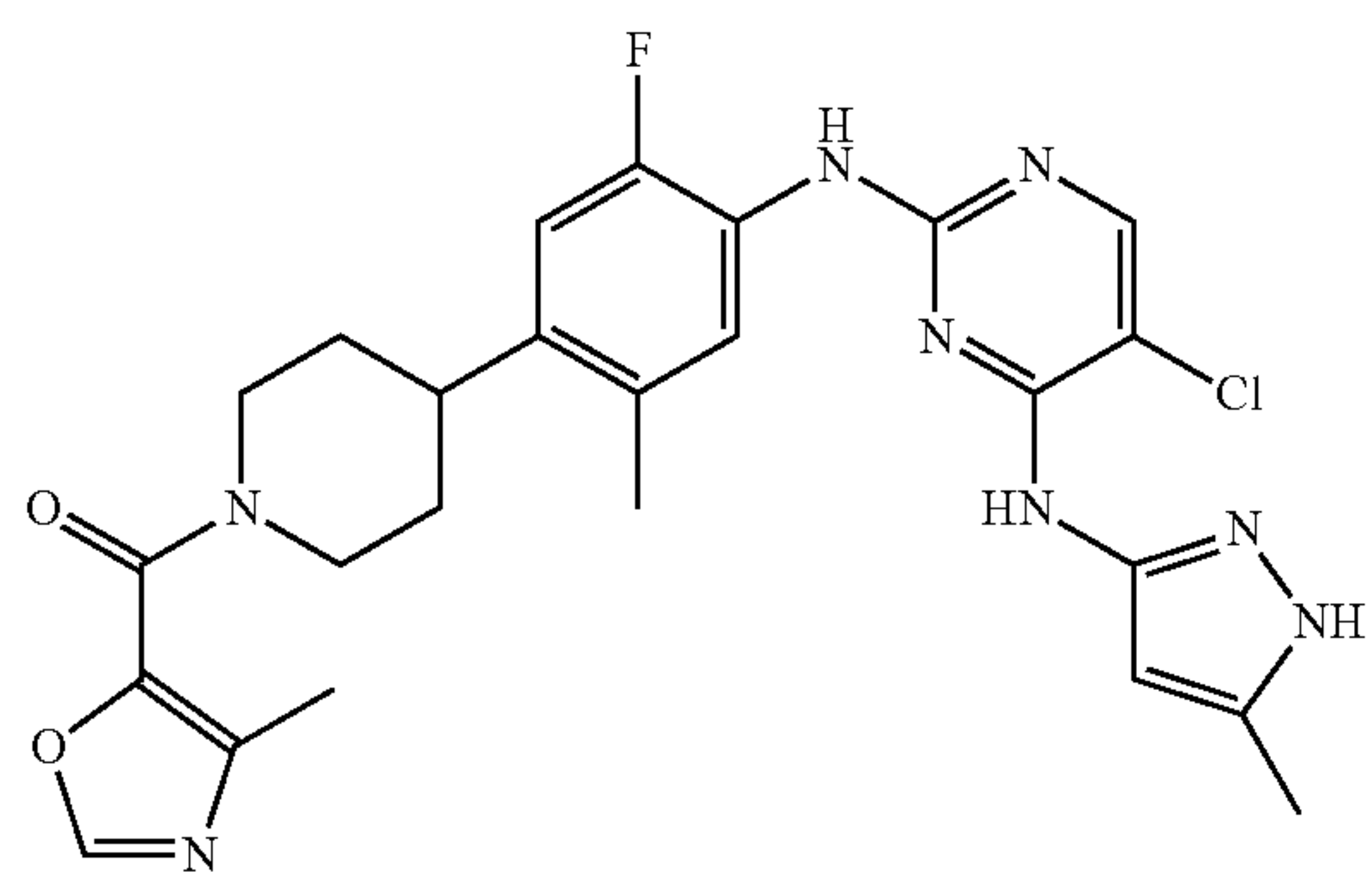
(4-(4-(5-chloro-4-(5-methyl-1H-pyrazol-3-ylamino)pyrimidin-2-ylamino)-5-fluoro-2-methylphenyl)piperidin-1-yl)(1-methyloxazol-5-yl)methanone
