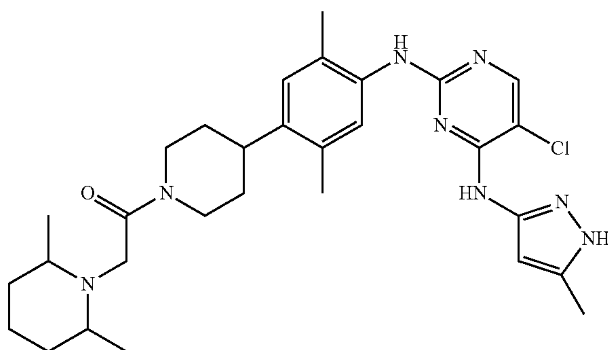
1-(4-(4-(5-chloro-4-(5-methyl-1H-pyrazol-3-ylamino)pyrimidin-2-ylamino)-2,5-dimethylphenyl)piperidin-1-yl)-2-(2,6-dimethylpiperidin-1-yl)ethanone
