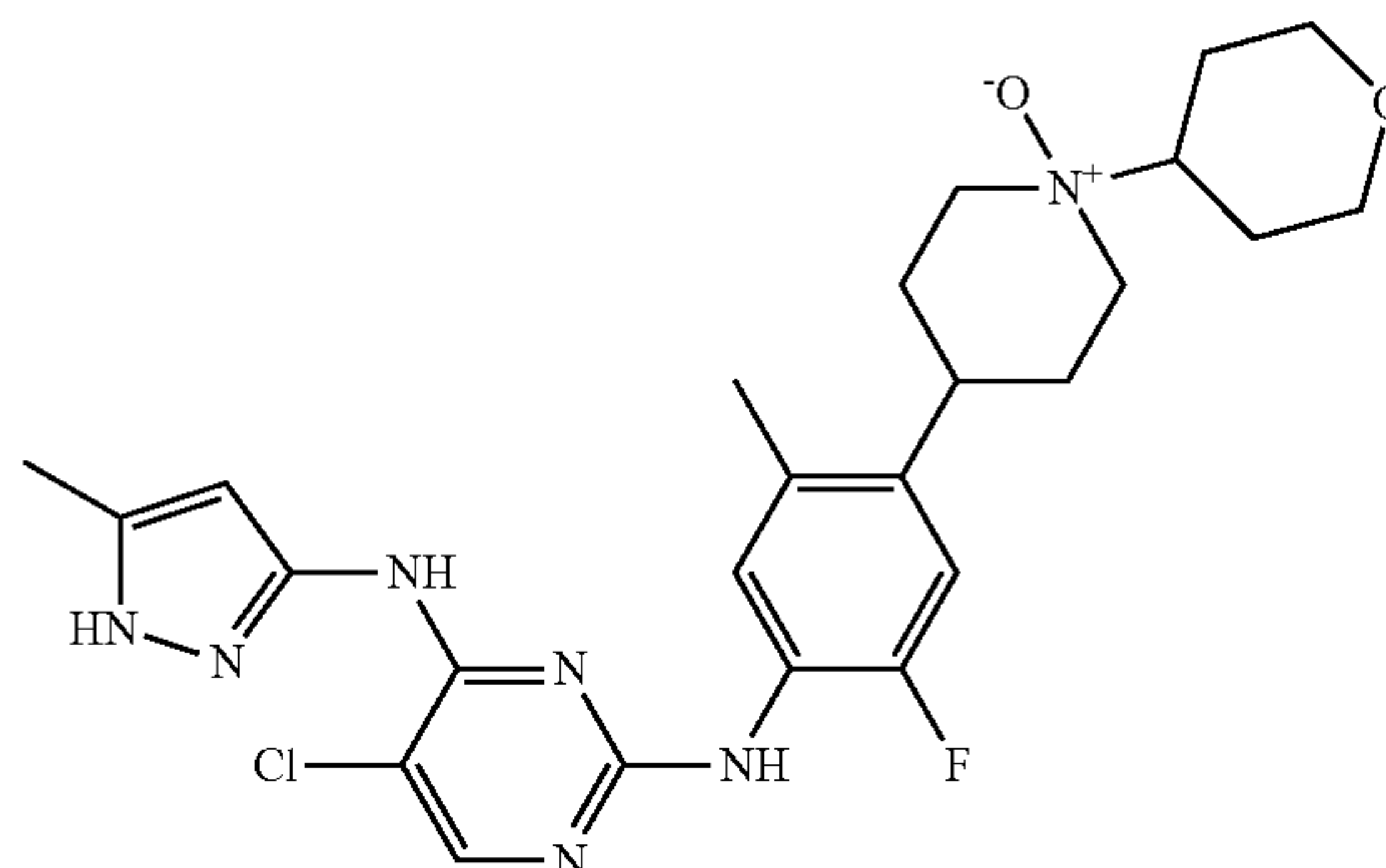
4-(4-(5-chloro-4-(5-methyl-1H-pyrazol-3-ylamino)pyrimidin-2-ylamino)-5-fluoro-2-methylphenyl)-1-(tetrahydro-2H-pyran-4-yl)piperidin 1-oxide
