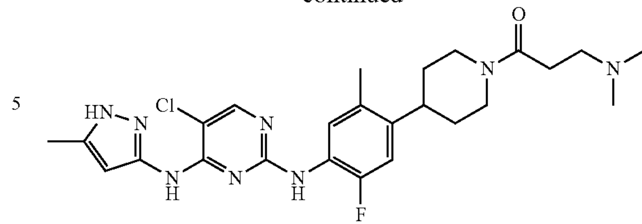
1-(4-(4-(5-chloro-4-(5-methyl-1H-pyrazol-3-ylamino)pyrimidin-2-ylamino)-5-fluoro-2-methylphenyl)piperidin-1-yl)-3-(dimethylamino)propan-1-one
