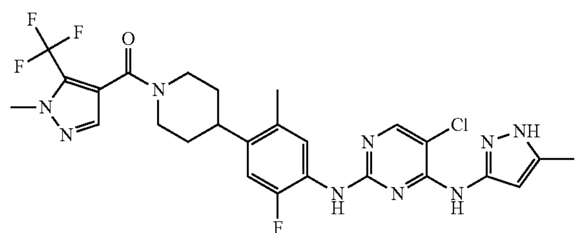
(4-(4-(5-chloro-4-(5-methyl-1H-pyrazol-3-ylamino)pyrimidin-2-ylamino)-5-fluoro-2-methylphenyl)piperidin-1-yl)(1-methyl-5-(trifluoromethyl)-1H-pyrazol-4-yl)methanone
