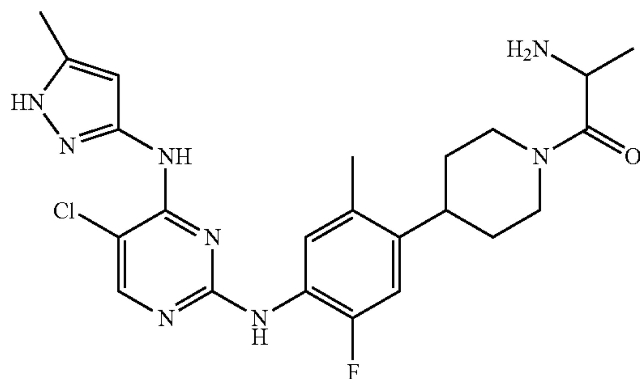
2-amino-1-(4-(4-(5-chloro-4-(5-methyl-1H-pyrazol-3-ylamino)pyrimidin-2-ylamino)-5-fluoro-2-methylphenyl)piperidin-1-yl)propan-1-one
