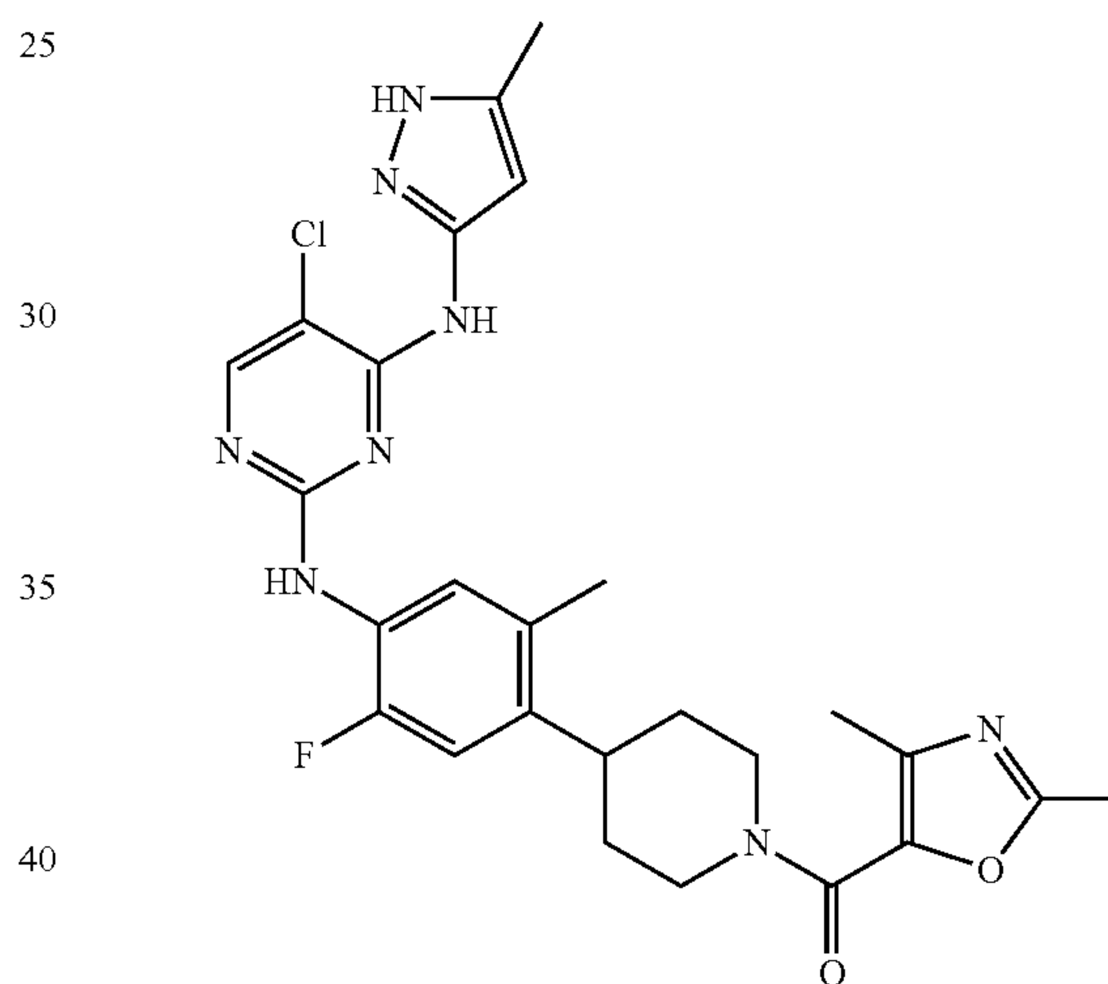
(4-(4-(5-chloro-4-(5-methyl-1H-pyrazol-3-ylamino)pyrimidin-2-ylamino)-5-fluoro-2-methylphenyl)piperidin-1-yl)(2,4-dimethyloxazol-5-yl)methanone
