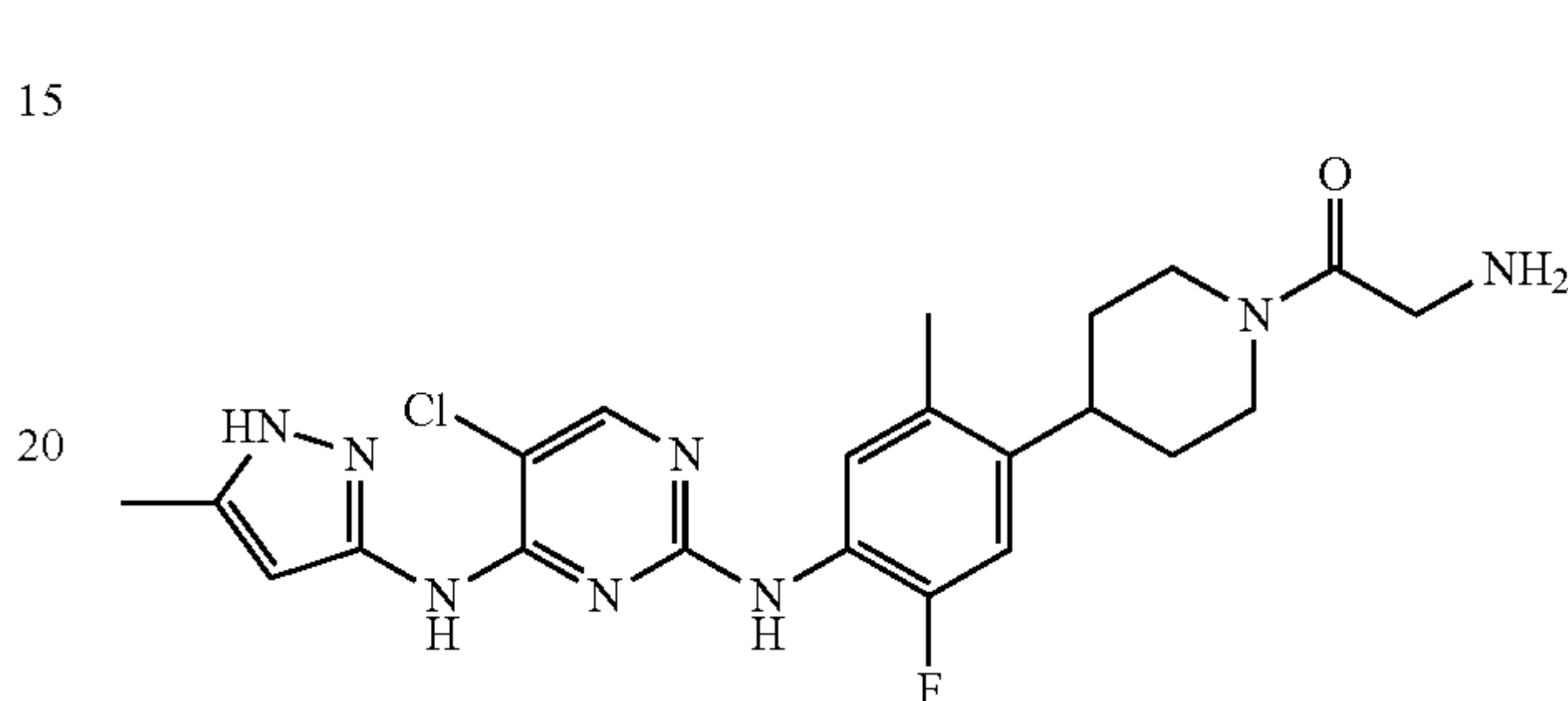
1-(4-(4-(5-chloro-4-(5-methyl-1H-pyrazol-3-ylamino)pyrimidin-2-ylamino)-5-fluoro-2-methylphenyl)piperidin-1-yl)-3-(dimethylamino)propan-1-one
