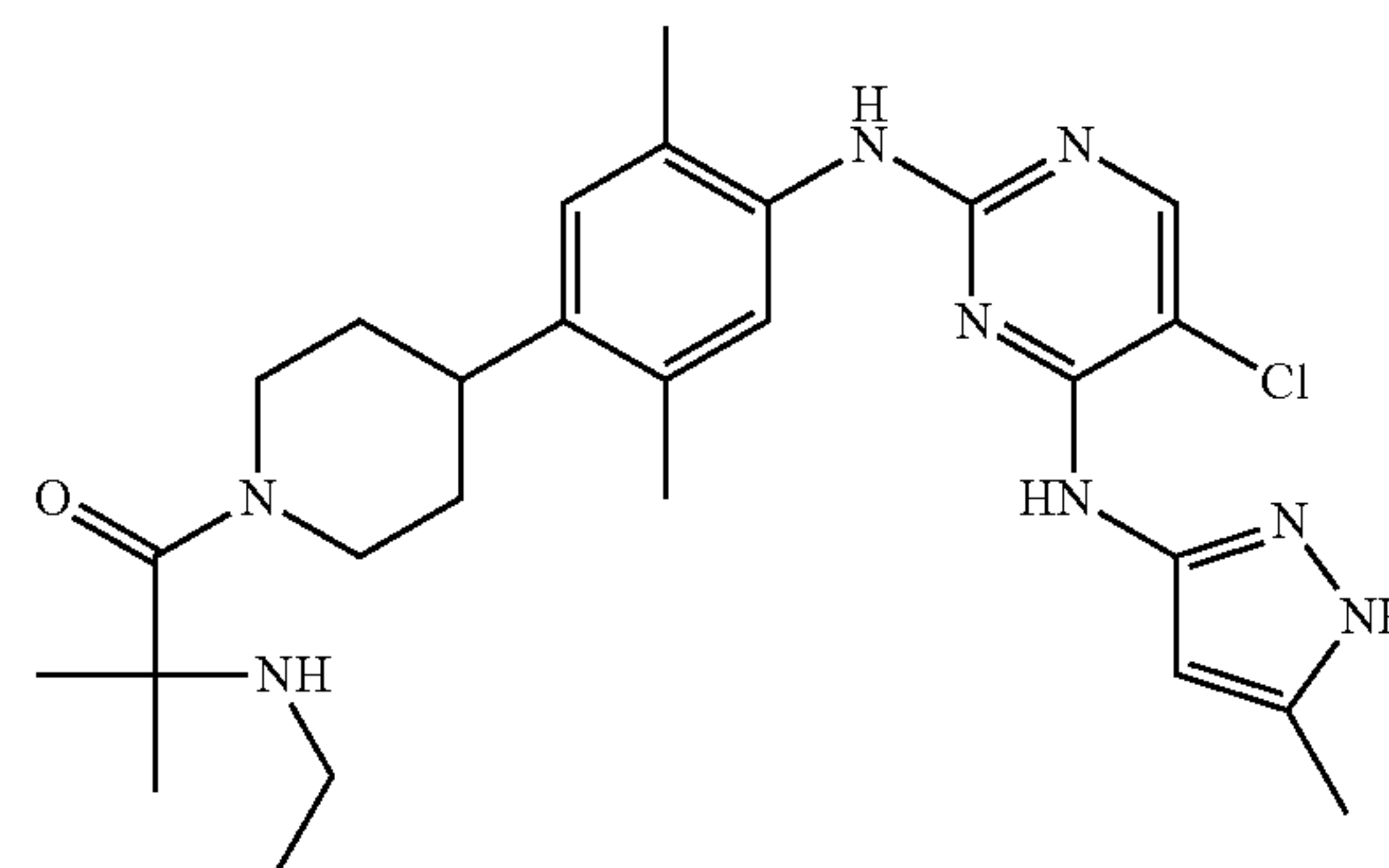
5-chloro-N2-(2,5-dimethyl-4-(1-(tetrahydro-2H-thiopyran-4-yl)piperidin-4-yl)phenyl)-N4-(5-methyl-1H-pyrazol-3-yl)pyrimidine-2,4-diamine
