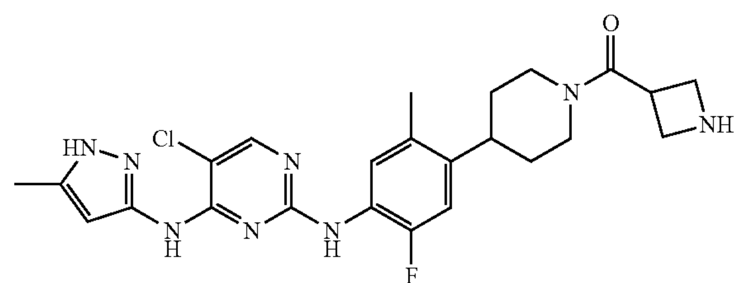
azetidin-3-yl(4-(4-(5-chloro-4-(5-methyl-1H-pyrazol-3-ylamino)pyrimidin-2-ylamino)-5-fluoro-2-methylphenyl)piperidin-1-yl)methanone
