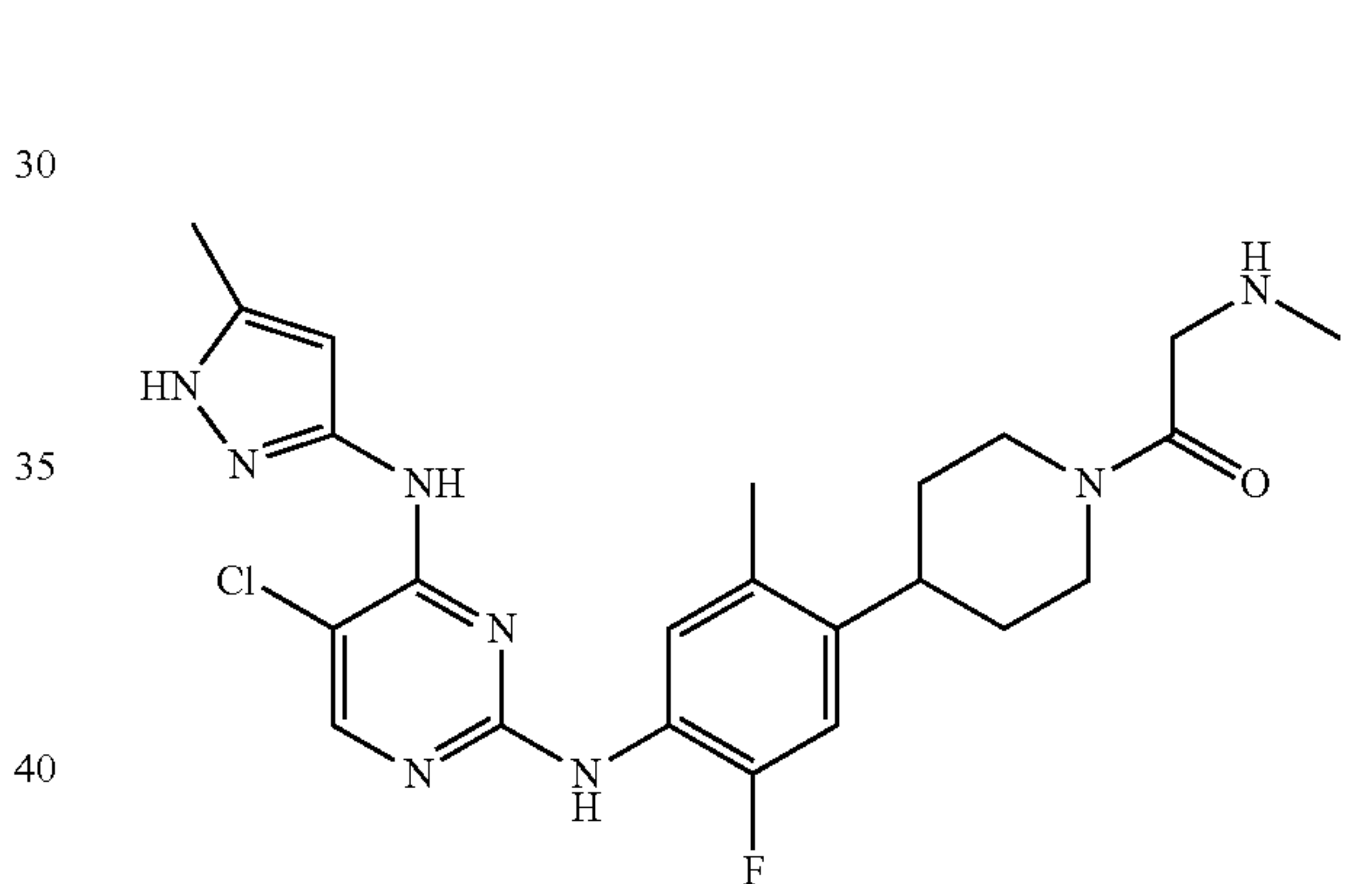
1-(4-(4-(5-chloro-4-(5-methyl-1H-pyrazol-3-ylamino)pyrimidin-2-ylamino)-5-fluoro-2-methylphenyl)piperidin-1-yl)-2-(methylamino)ethanone
