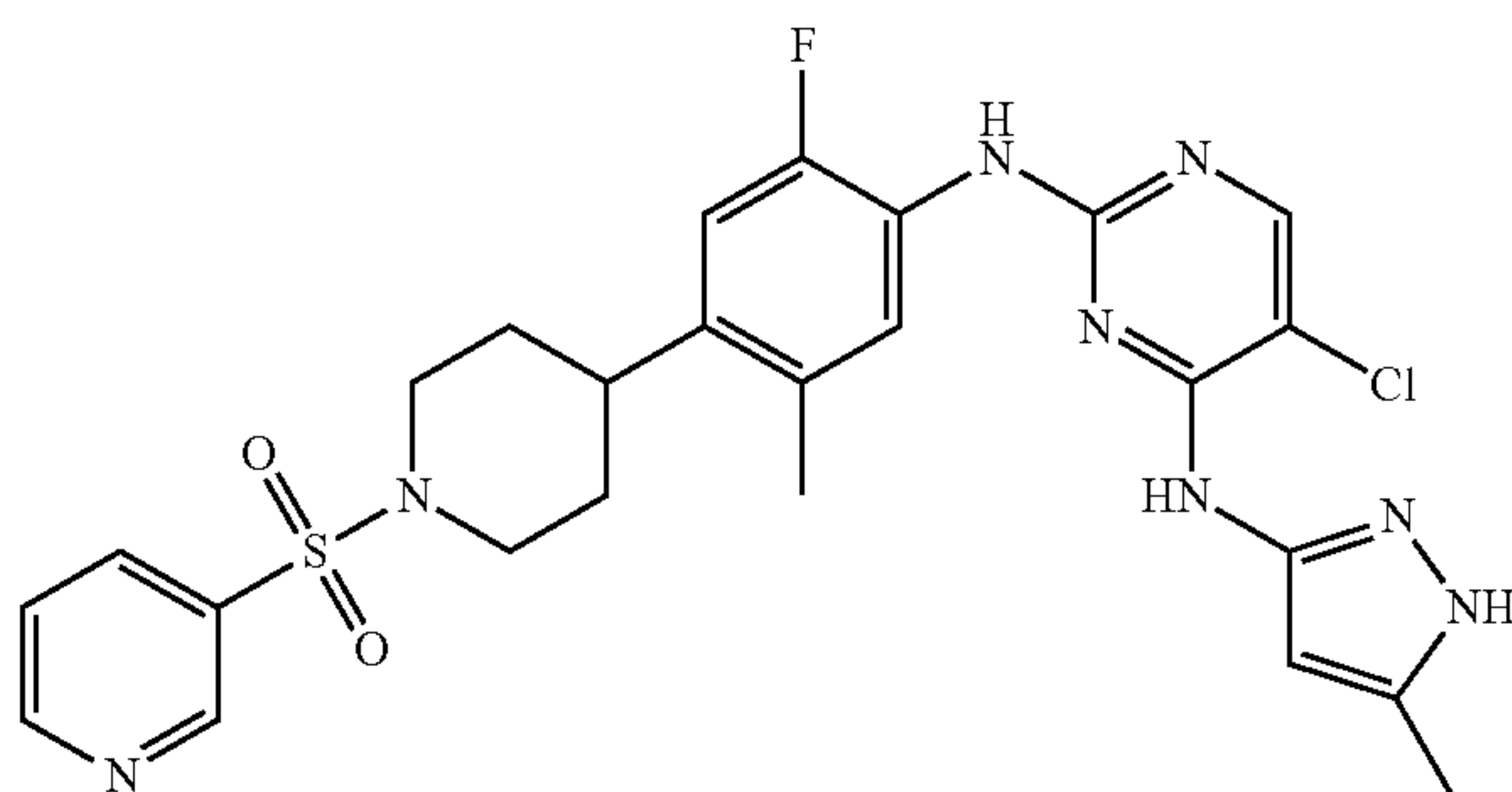
5-chloro-N2-(2-fluoro-5-methyl-4-(1-(pyridin-3-ylsulfonyl)piperidin-4-yl)phenyl)-N4-(5-methyl-1H-pyrazol-3-yl)pyrimidine-2,4-diamine
