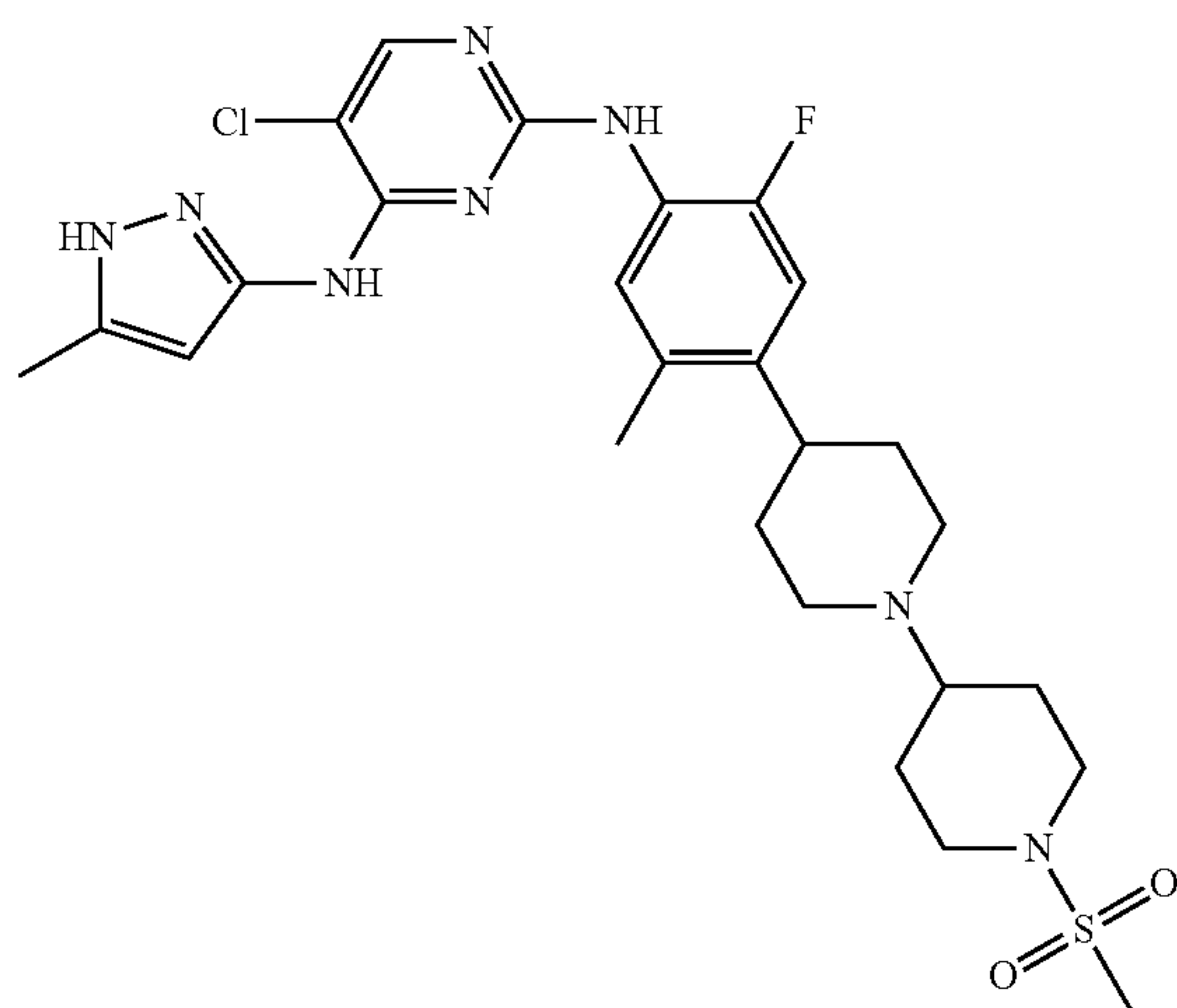
5-chloro-N2-(2-fluoro-5-methyl-4-(1'-(methylsulfonyl)-1,4'-bipiperidin-4-yl)phenyl)-N4-(5-methyl-1H-pyrazol-3-yl)pyrimidine-2,4-diamine
