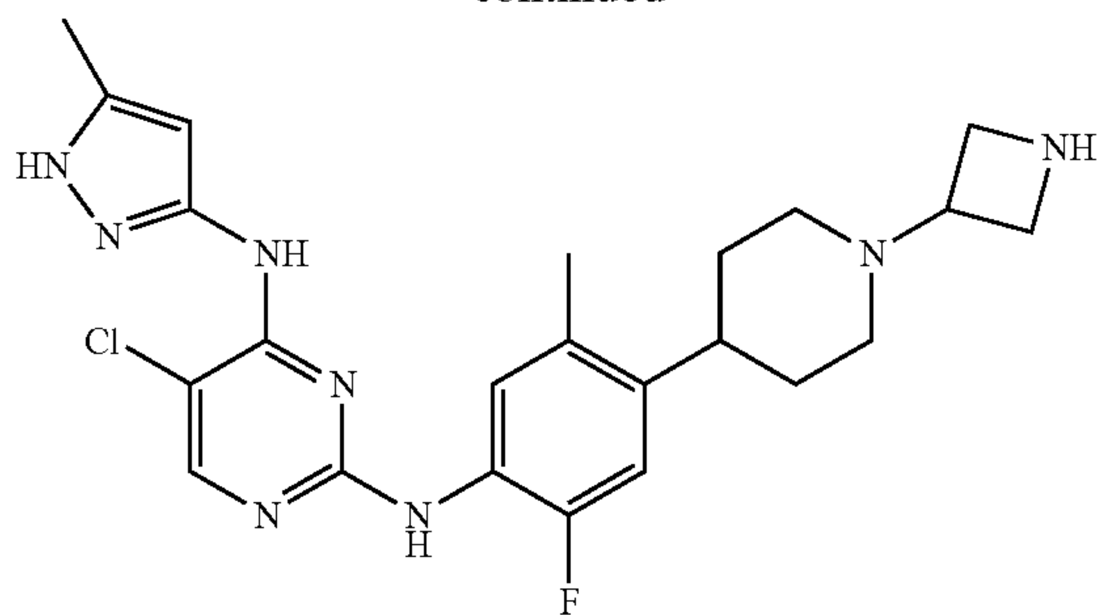
N2-(4-(1-(azetidin-3-yl)piperidin-4-yl)-2-fluoro-5-methylphenyl)-5-chloro-N4-(5-methyl-1H-pyrazol-3-yl)pyrimidine-2,4-diamine
