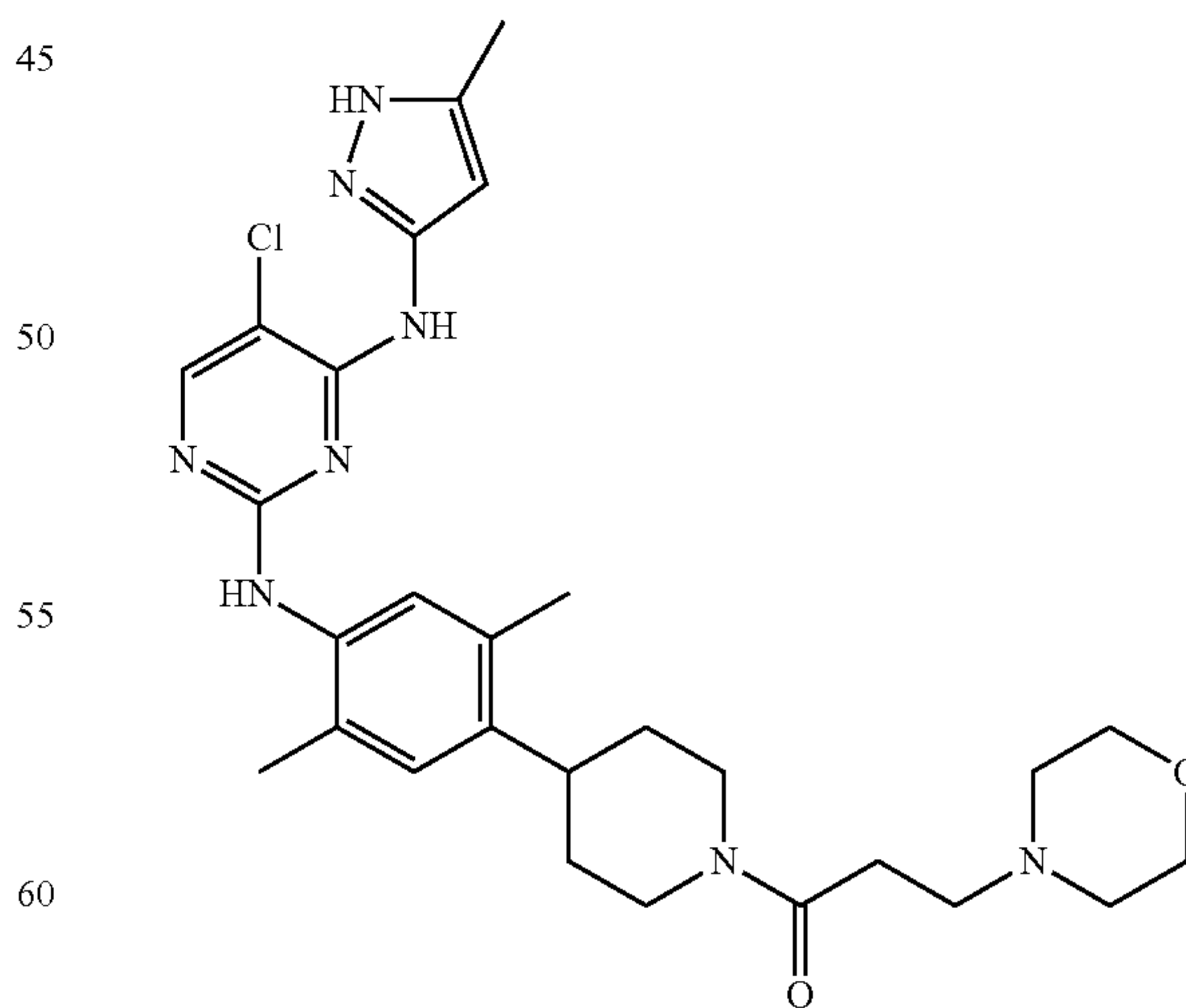
1-(4-(4-(5-chloro-4-(5-methyl-1H-pyrazol-3-ylamino)pyrimidin-2-ylamino)-2,5-dimethylphenyl)piperidin-1-yl)-3-morpholinopropan-1-one
