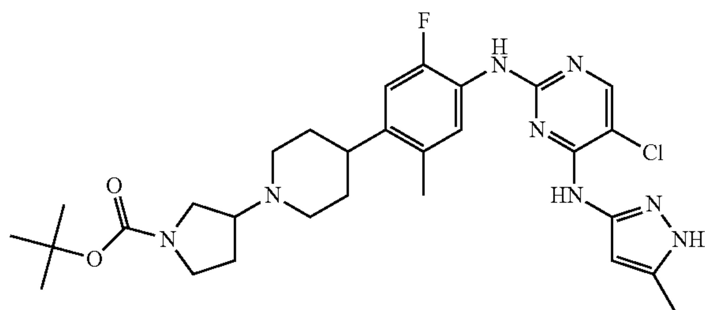
tert-butyl 3-(4-(4-(5-chloro-4-(5-methyl-1H-pyrazol-3-ylamino)pyrimidin-2-ylamino)-5-fluoro-2-methylphenyl)piperidin-1-yl)pyrrolidine-1-carboxylate
