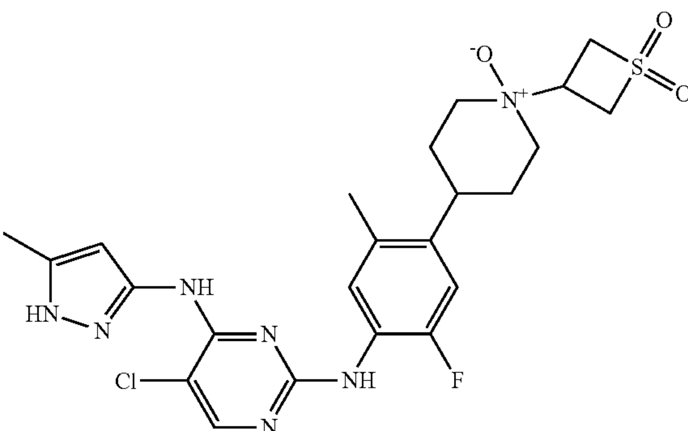
5-Chloro-N2-{4-[1-(1,1-dioxo-1λ6-thietan-3-yl)-1-oxide-piperidin-4-yl]-2-fluoro-5-methyl-phenyl}-N4-(5-ethyl-1H-pyrazol-3-yl)-pyrimidine-2,4-diamine
