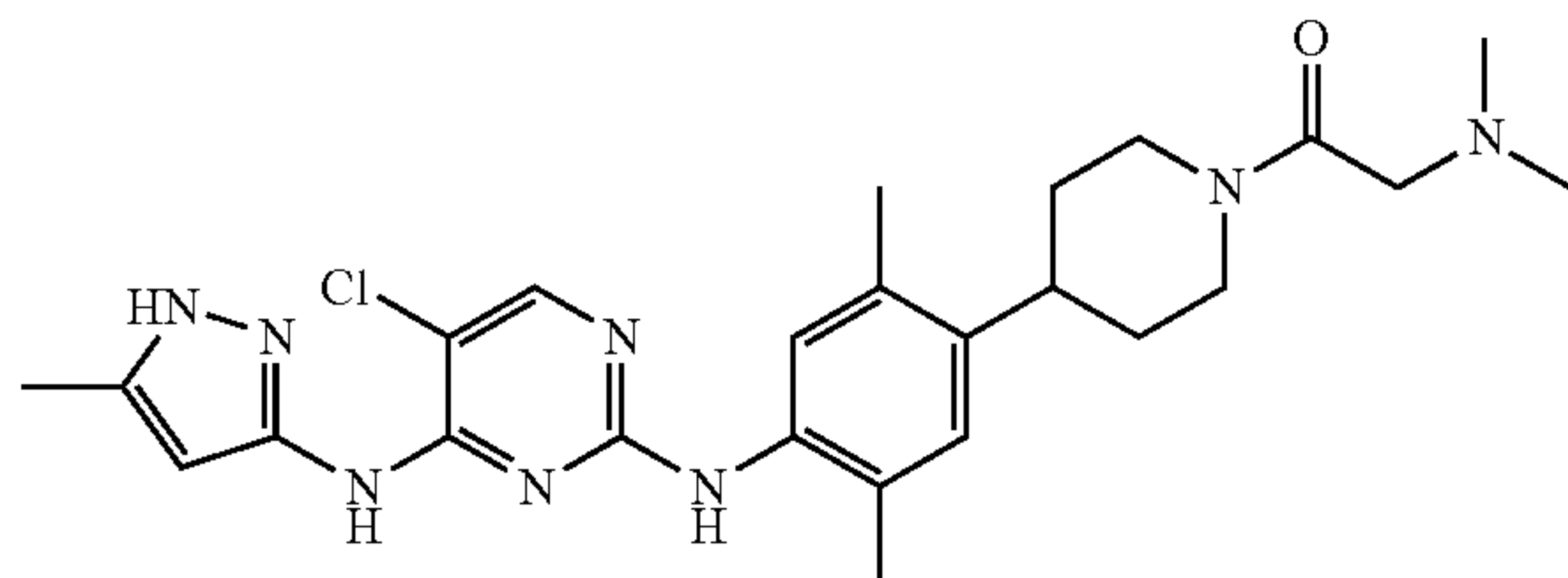
1-(4-(4-(5-chloro-4-(5-methyl-1H-pyrazol-3-ylamino)pyrimidin-2-ylamino)-2,5-dimethylphenyl)piperidin-1-yl)-2-(dimethylamino)ethanone
