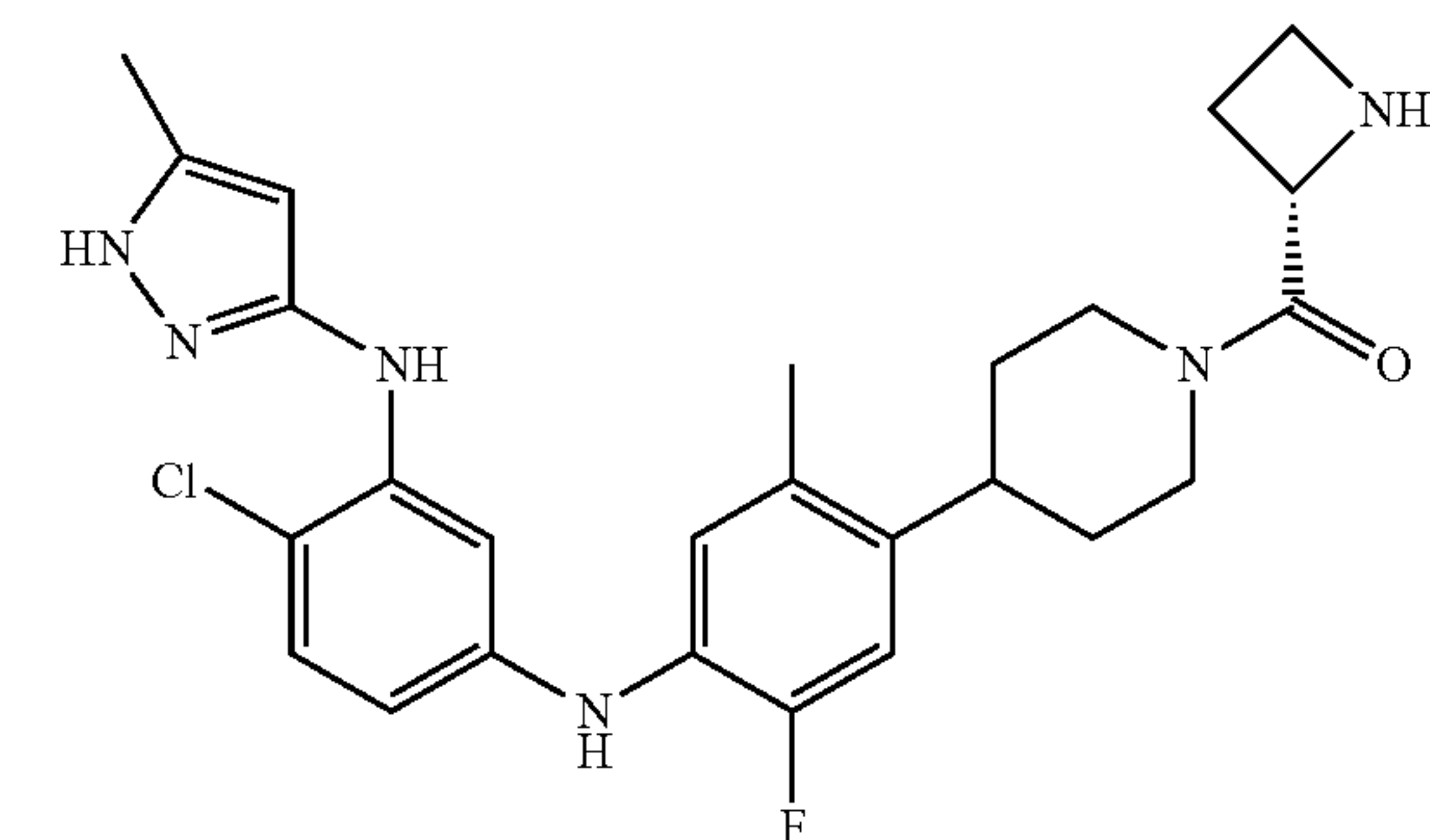
(S)-azetidin-2-yl(4-(4-(5-chloro-4-(5-methyl-1H-pyrazol-3-ylamino)pyrimidin-2-ylamino)-5-fluoro-2-methylphenyl)piperidin-1-yl)methanone
