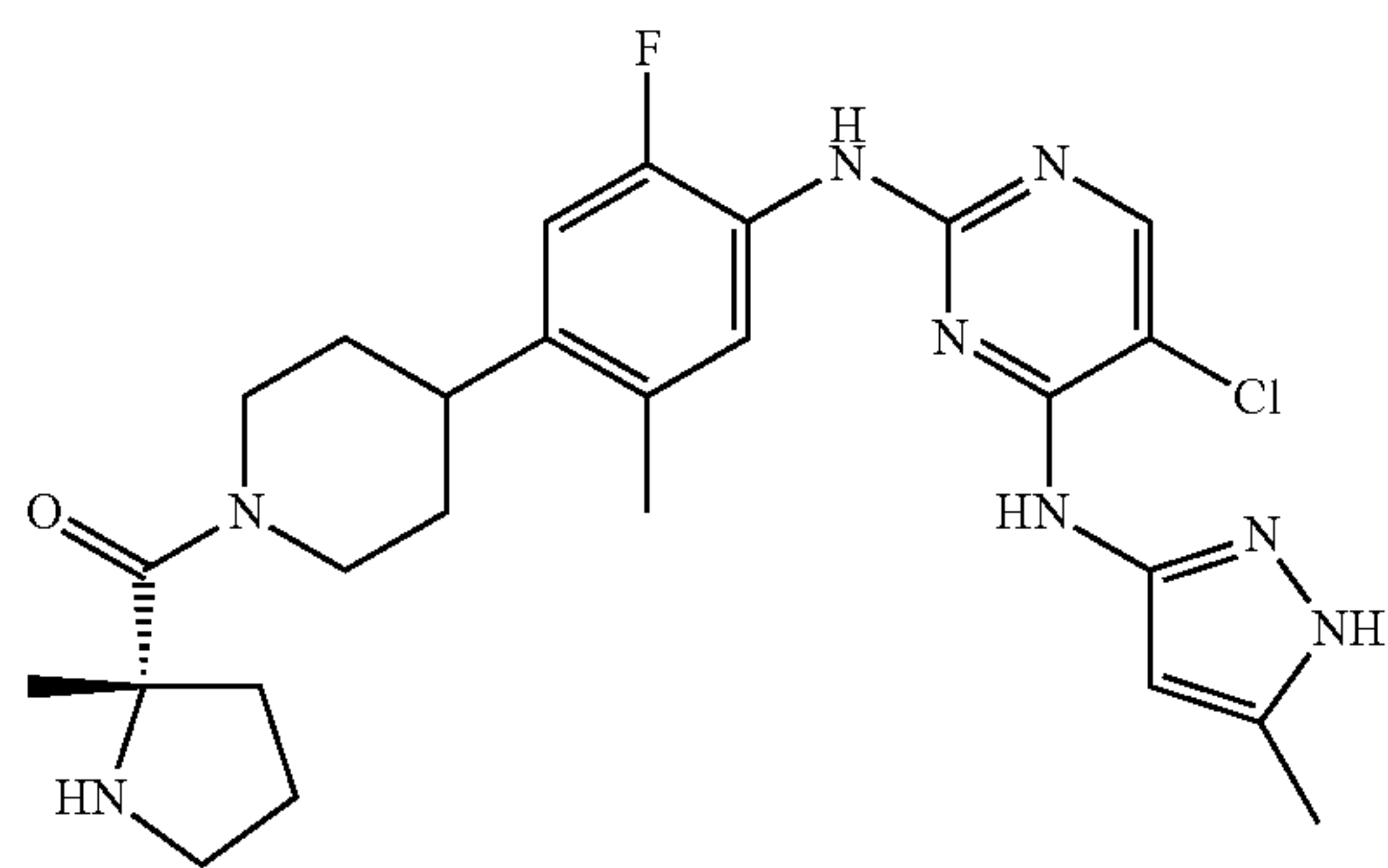
(S)-(4-(4-(5-chloro-4-(5-methyl-1H-pyrazol-3-ylamino)pyrimidin-2-ylamino)-5-fluoro-2-methylphenyl)piperidin-1-yl)(2-methylpyrrolidin-2-yl)methanone
