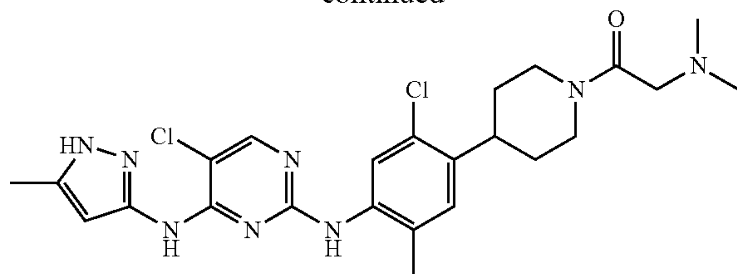
1-(4-(2-chloro-4-(5-chloro-4-(5-methyl-1H-pyrazol-3-ylamino)pyrimidin-2-ylamino)-5-methylphenyl)piperidin-1-yl)-2-(dimethylamino)ethanone
