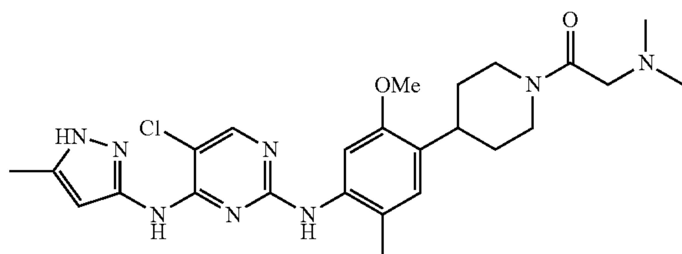
1-(4-(4-(5-chloro-4-(5-methyl-1H-pyrazol-3-ylamino)pyrimidin-2-ylamino)-2-methoxy-5-methylphenyl)piperidin-1-yl)-2-(dimethylamino)ethanone
