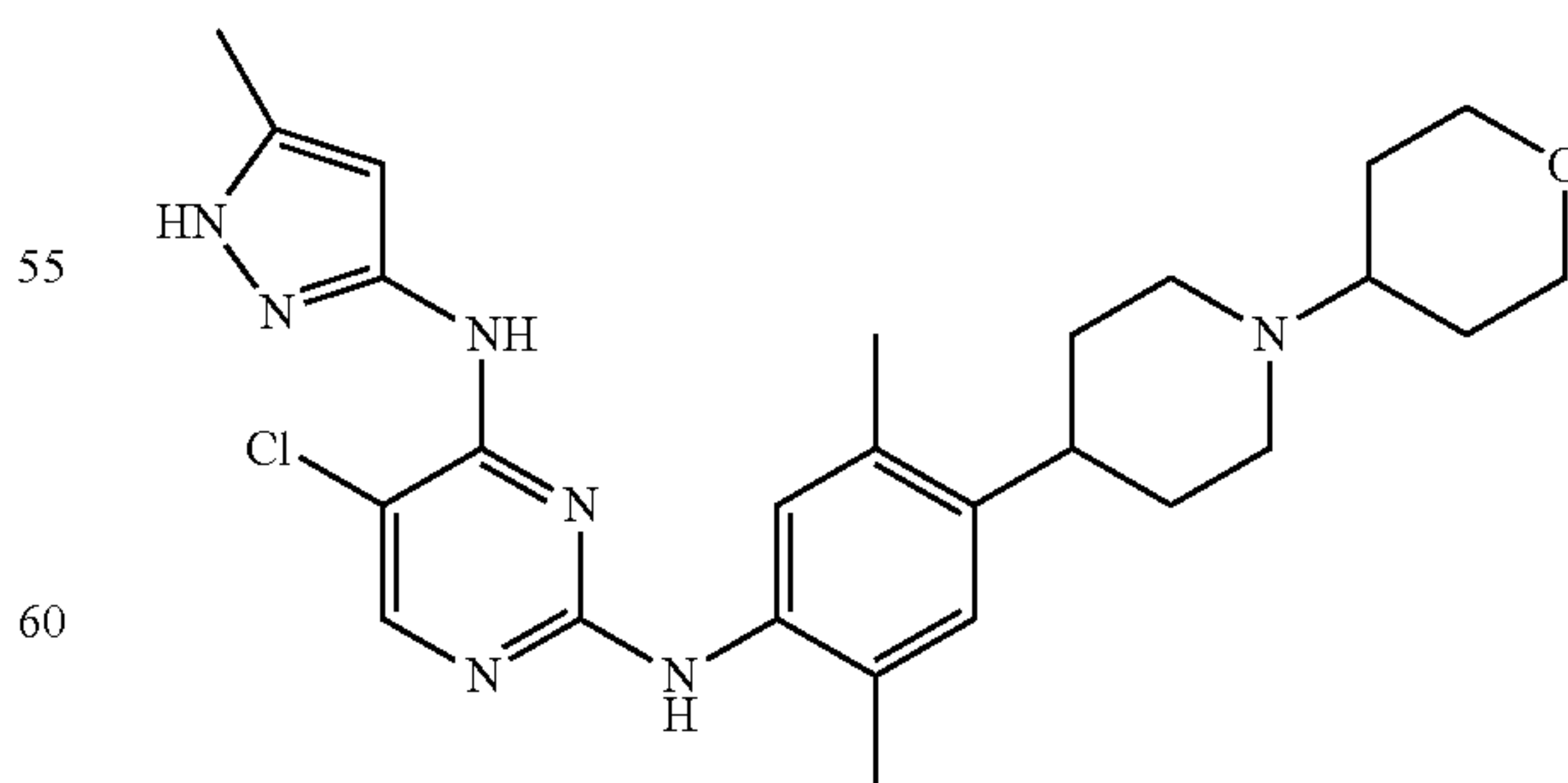
5-chloro-N2-(2,5-dimethyl-4-(1-(tetrahydro-2H-pyran-4-yl)piperidin-4-yl)phenyl)-N4-(5-methyl-1H-pyrazol-3-yl)pyrimidine-2,4-diamine
