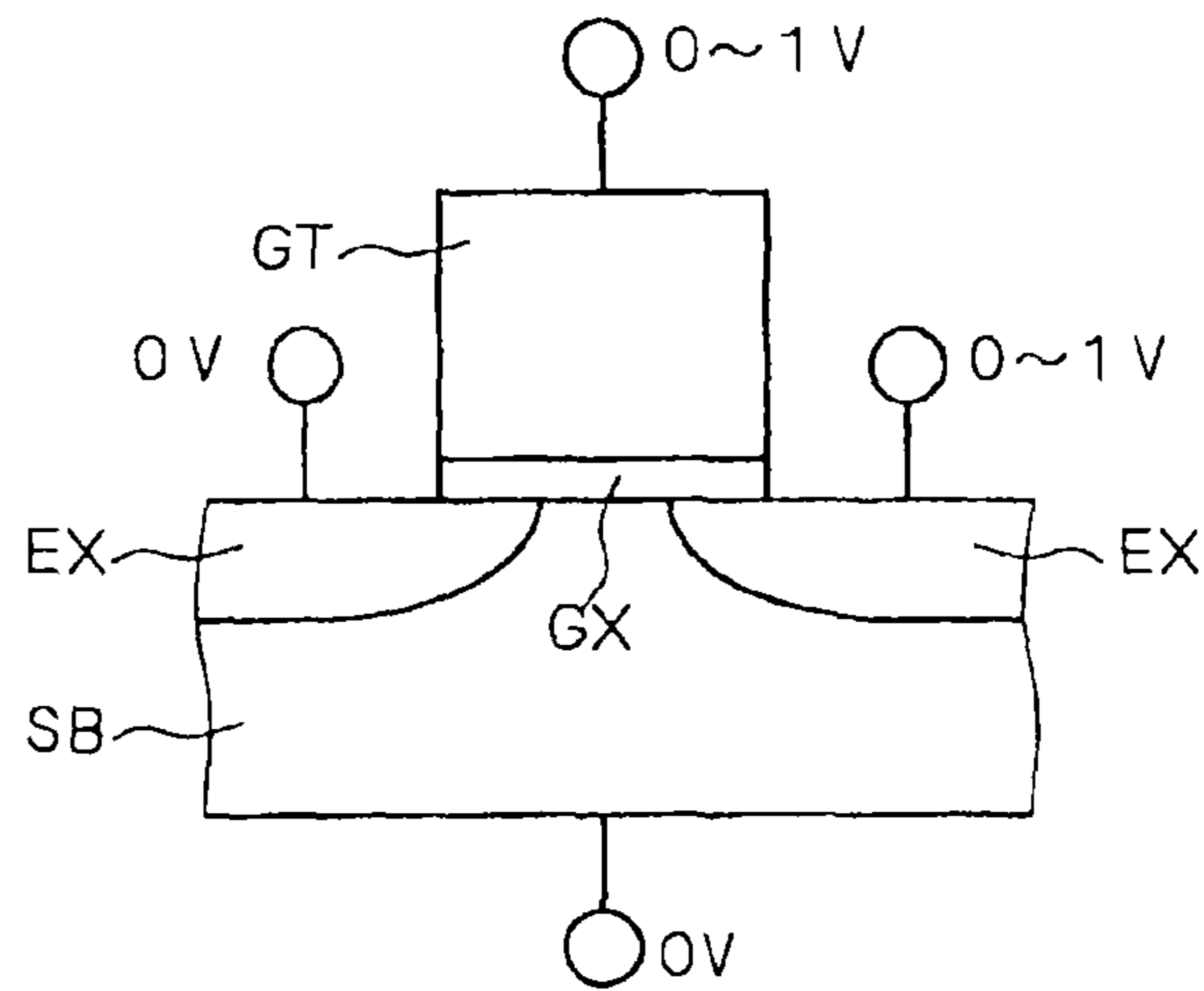
FIG. 37 (BACKGROUND ART)
