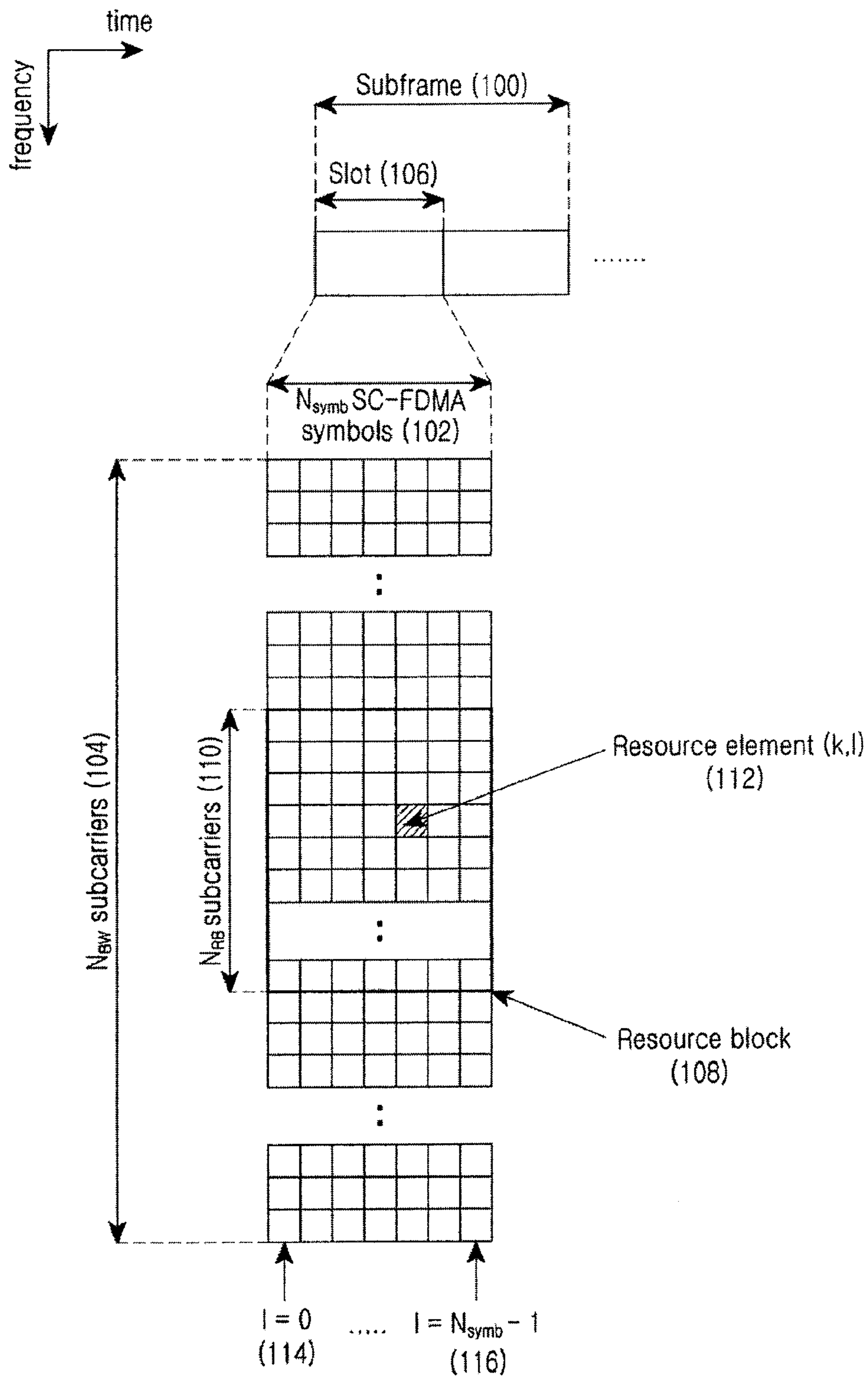
FIG. 1 (CONVENTIONAL ART)
