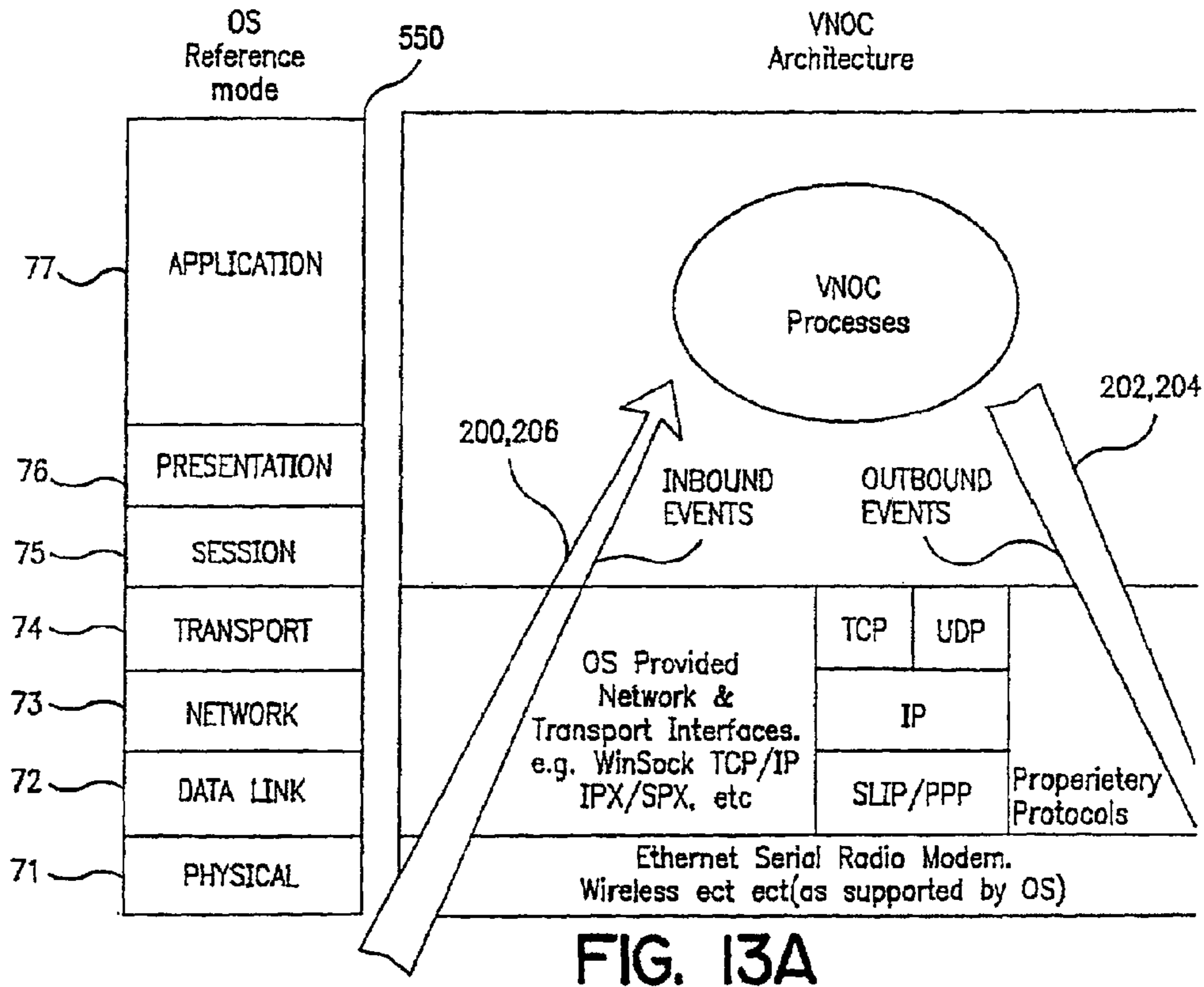
FIG. 13A Network architecture based on the OSI model
