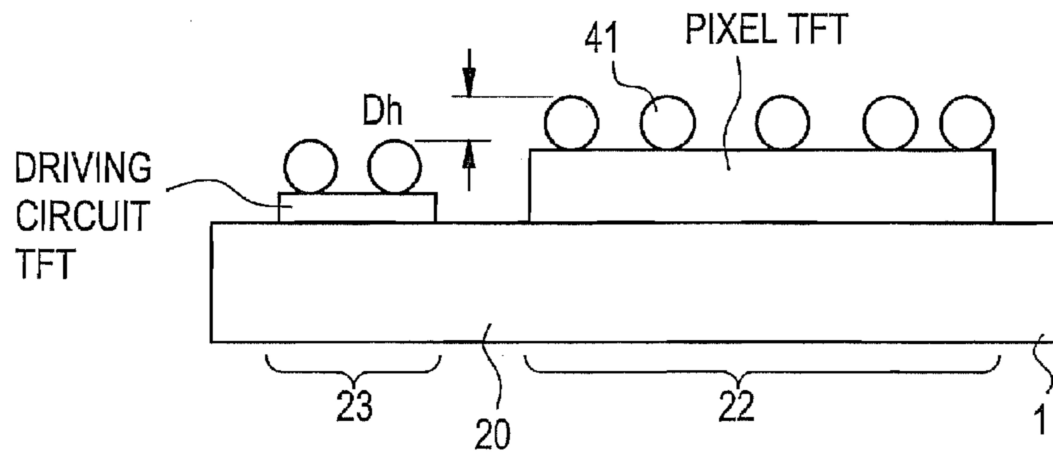
FIG. 36 PRIOR ART
