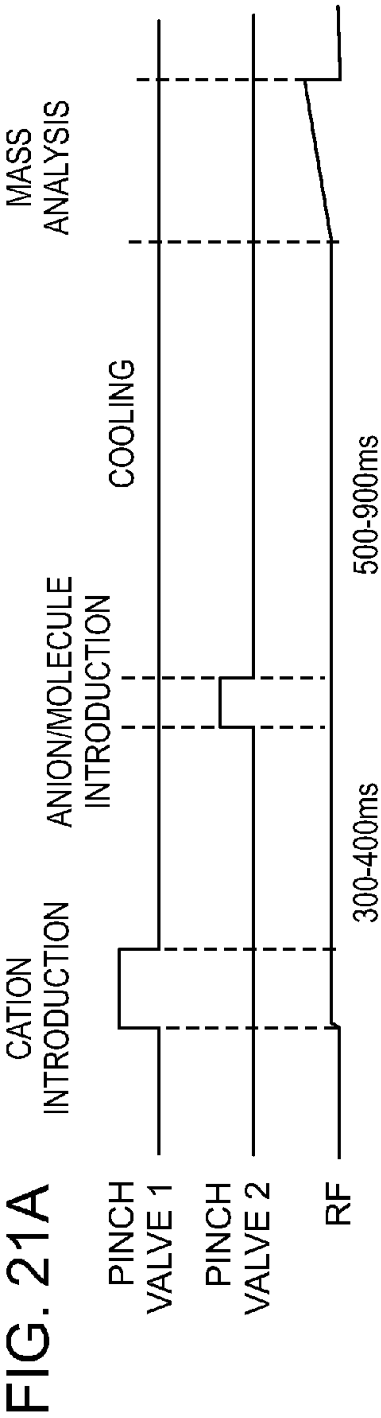
Angiotensin 1 cation with azobenzene molecule
