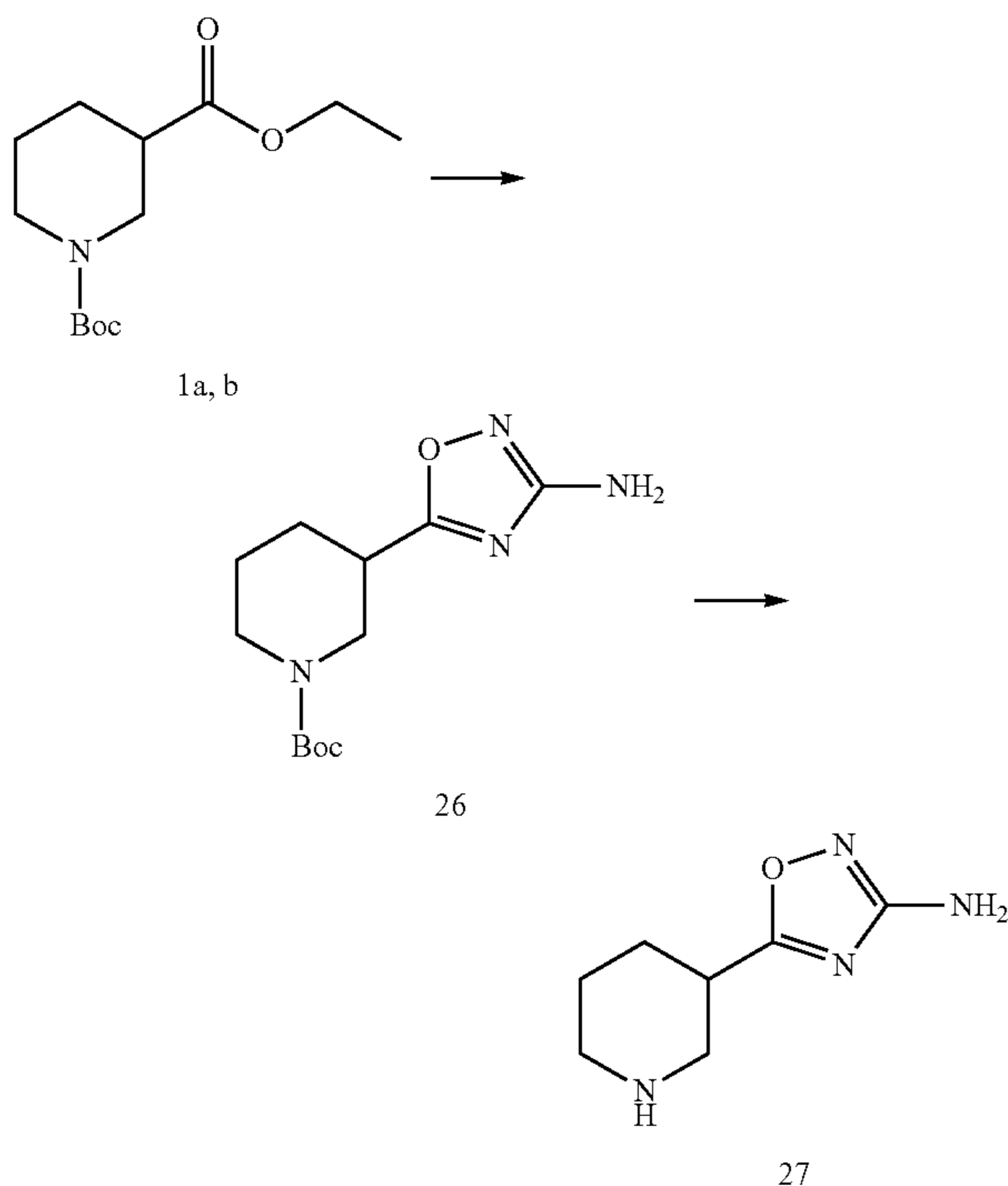
tert-Butyl 3-(3-amino-1,2,4-oxadiazol-5-yl)piperidine-1-carboxylate (26)
