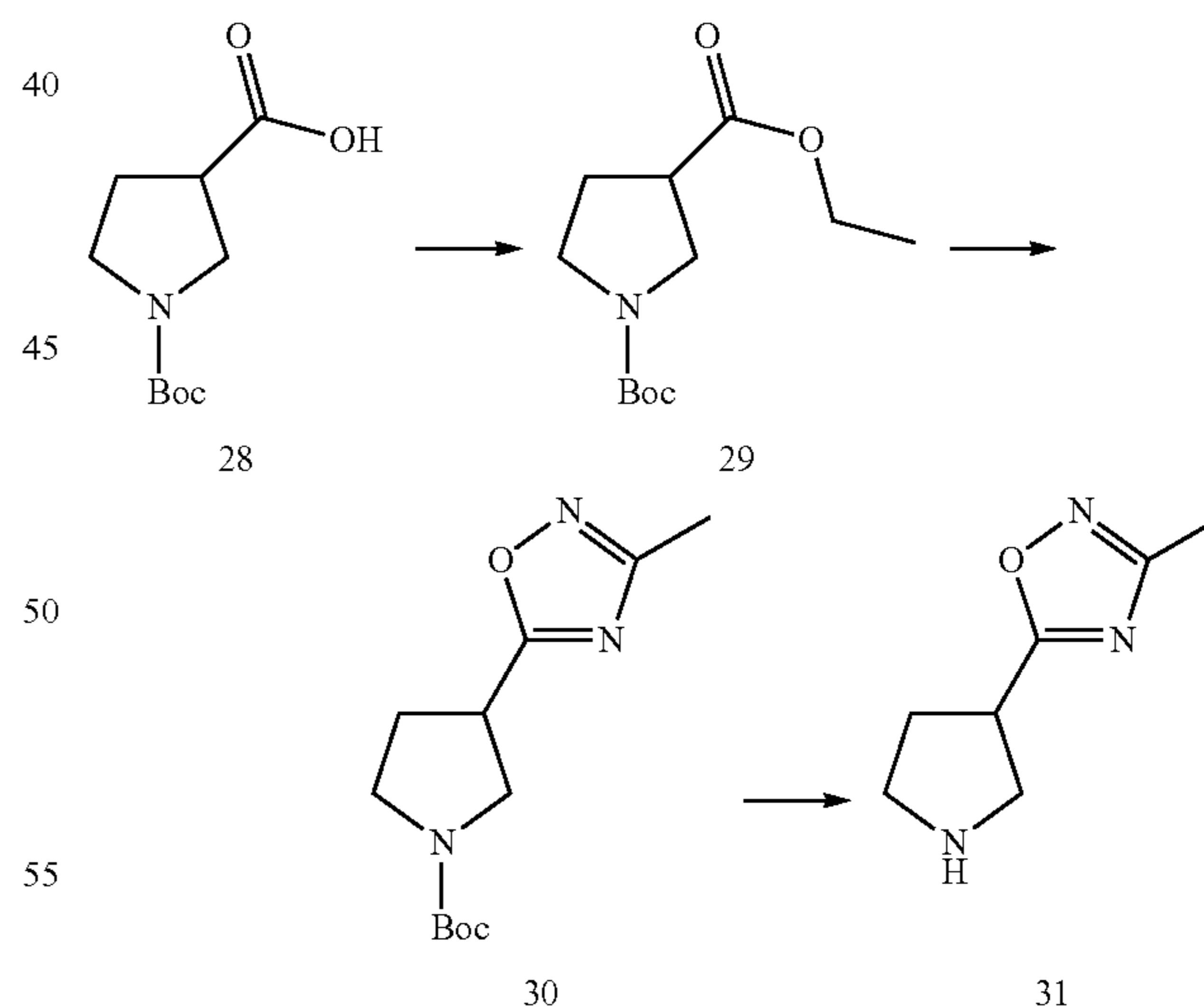
tert-Butyl 3-(3-amino-1,2,4-oxadiazol-5-yl)piperidine-1-carboxylate (26)
