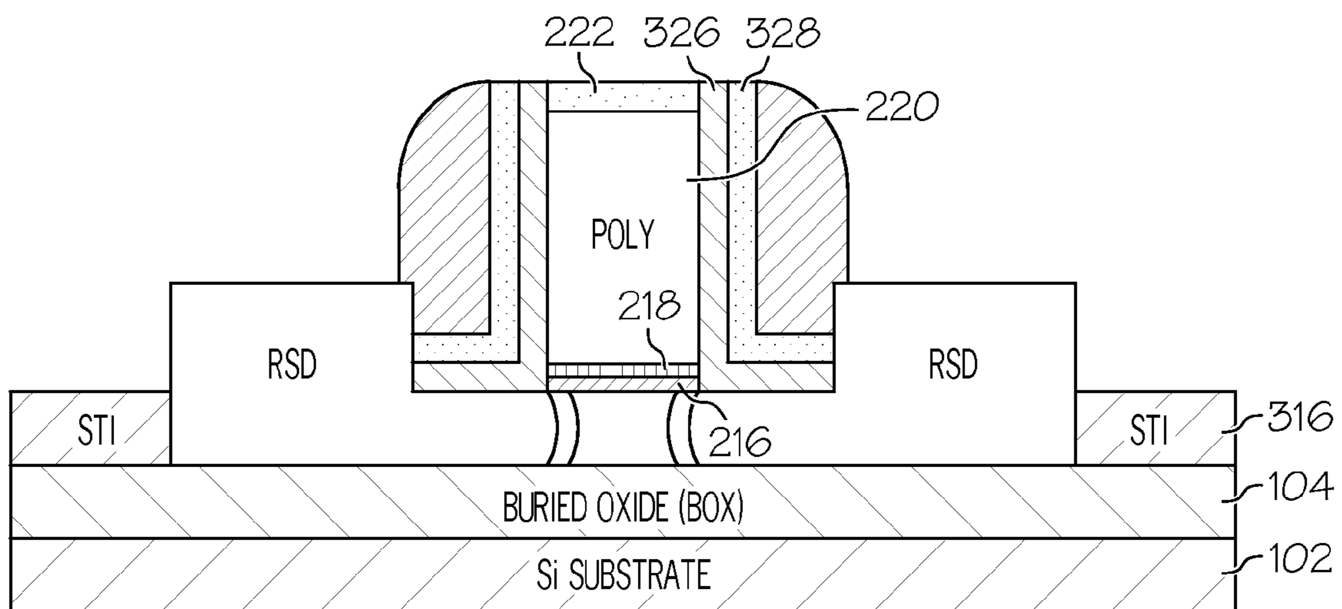
FIG. 10 (PRIOR ART)
